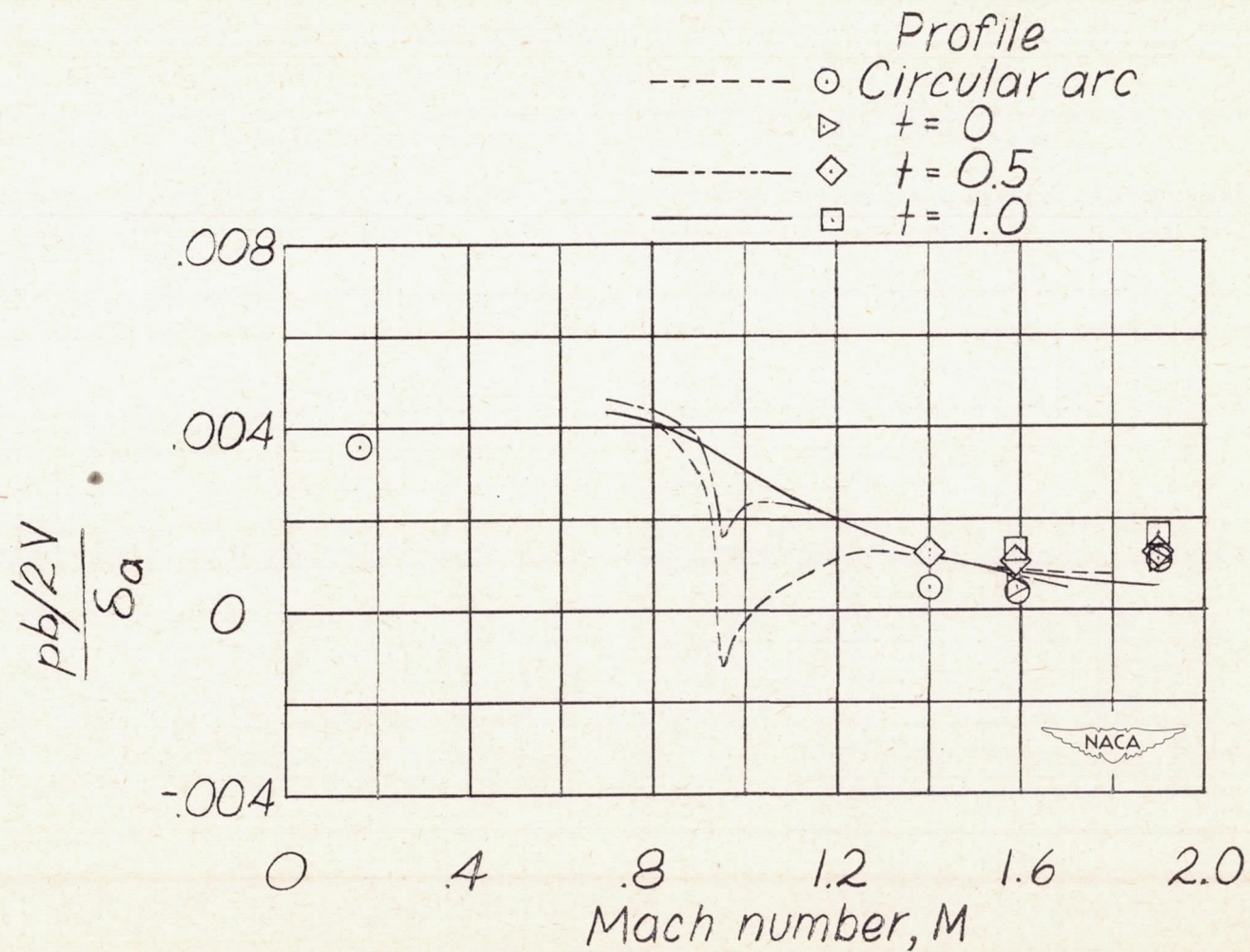
Figure 12.- Variation of \frac{pb/2V}{\delta_a} with Mach number. Faired lines from rocket-model tests, symbols from wind-tunnel tests.
