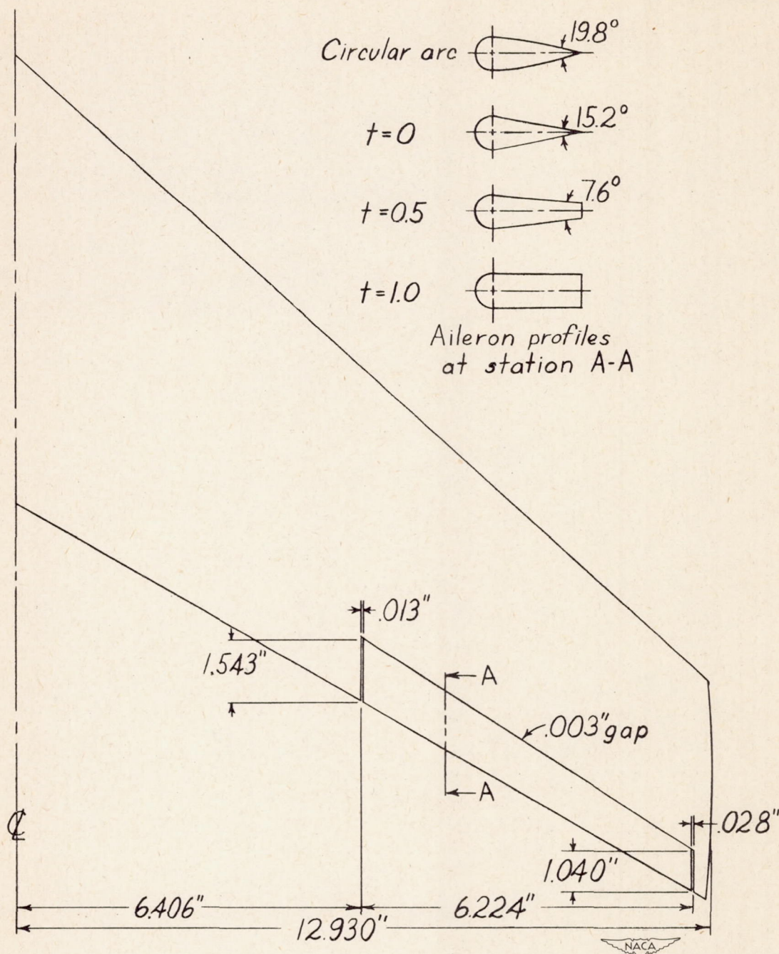
Figure 3.- Details of aileron installation.
