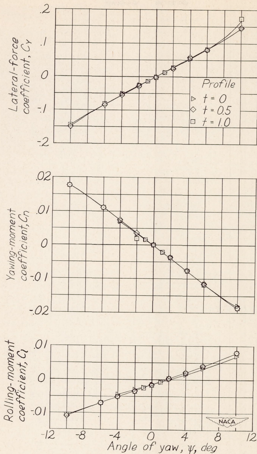
Figure 8.- Effect of aileron profile on the lateral characteristics in yaw. \alpha = 0^\circ ; \delta_a = 0^\circ ; M = 1.59 .
