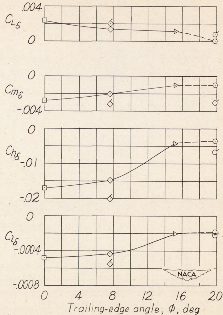
Figure 13.- Effect of trailing-edge angle on various aerodynamic characteristics. Faired line for M = 1.59 ; flagged symbols for M = 1.40 .
