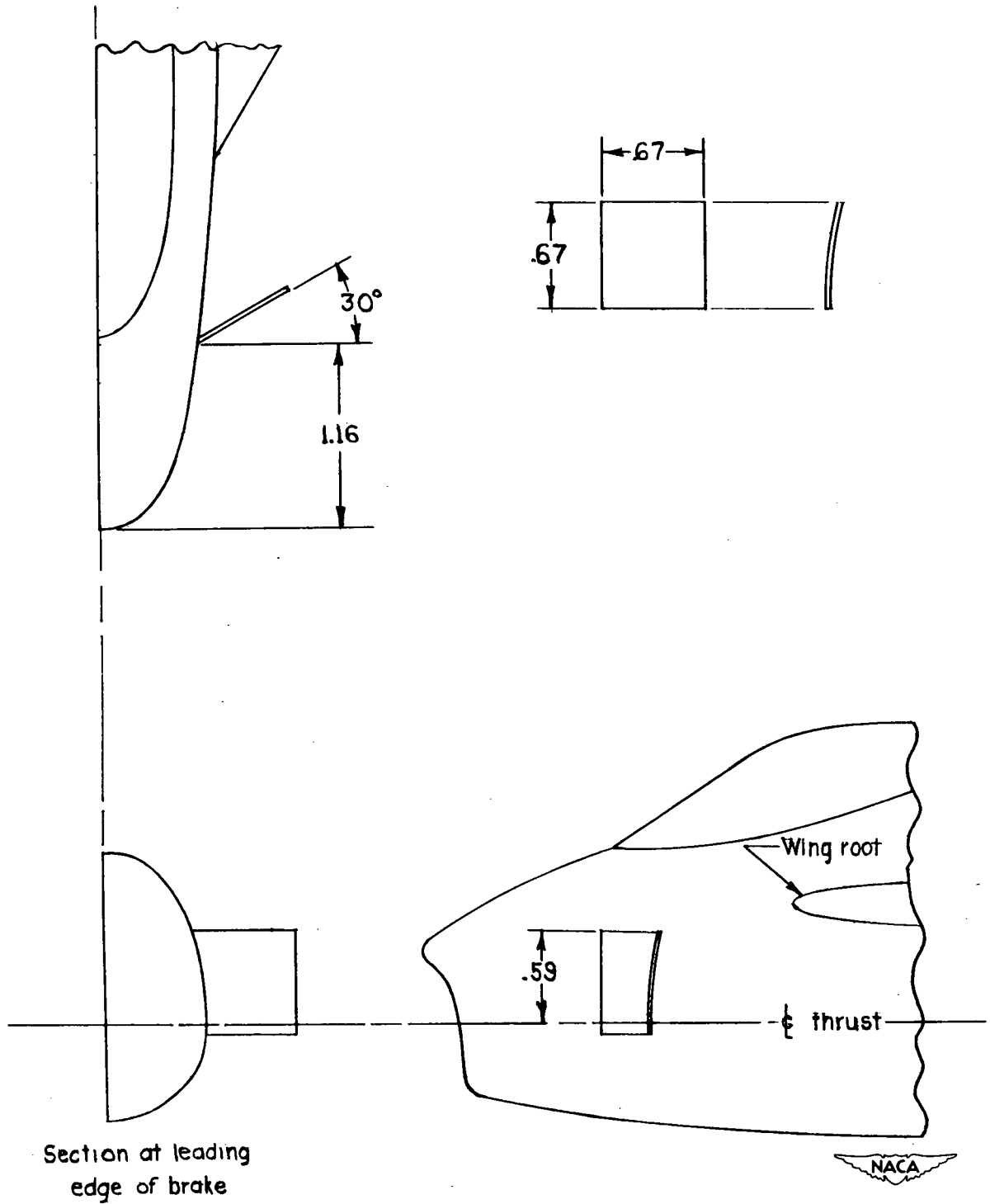
Figure 4.- Fuselage flap dive brake on \frac{1}{30} - scale X-5 model. All dimensions are in inches.
