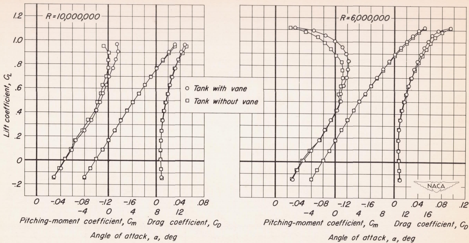
Figure 11.- The effect of the tip-tank vane on the low-speed aerodynamic characteristics of a wing with a tip tank of fineness ratio 6.67. M, 0.25 .
