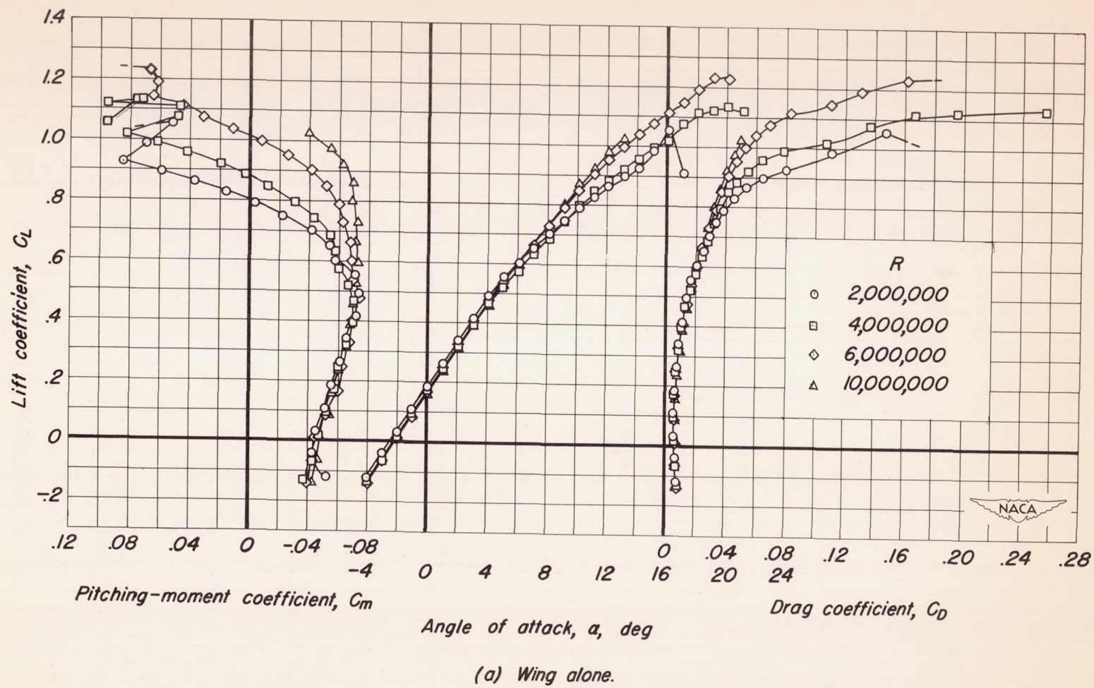
Figure 3.- The effect of Reynolds number on the low-speed aerodynamic characteristics. M , 0.25.
