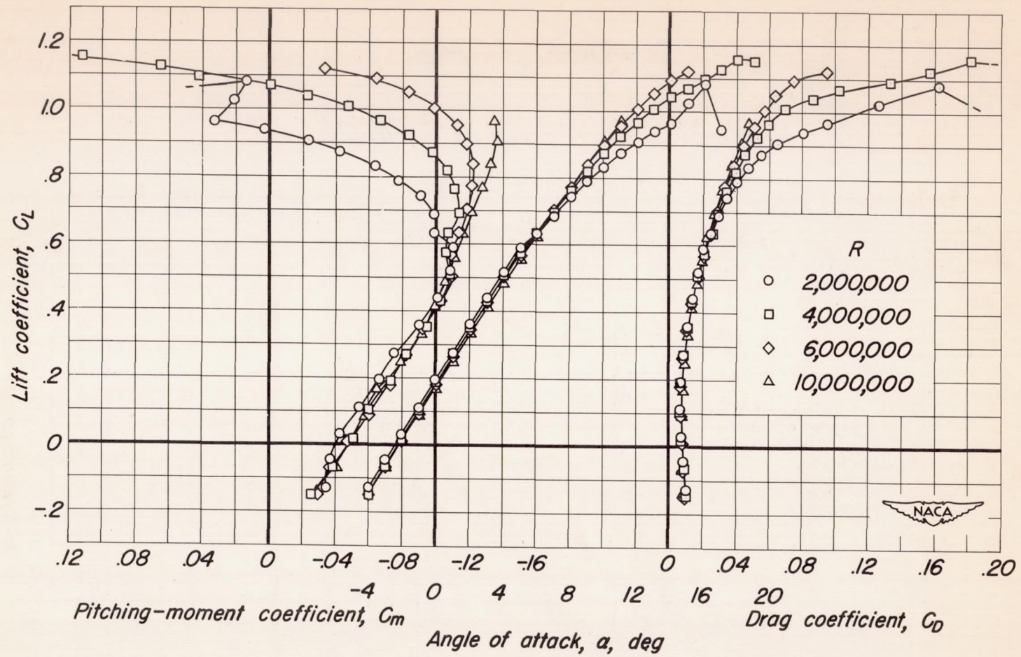
(c) Wing and tip tank of fineness ratio 6.67.
