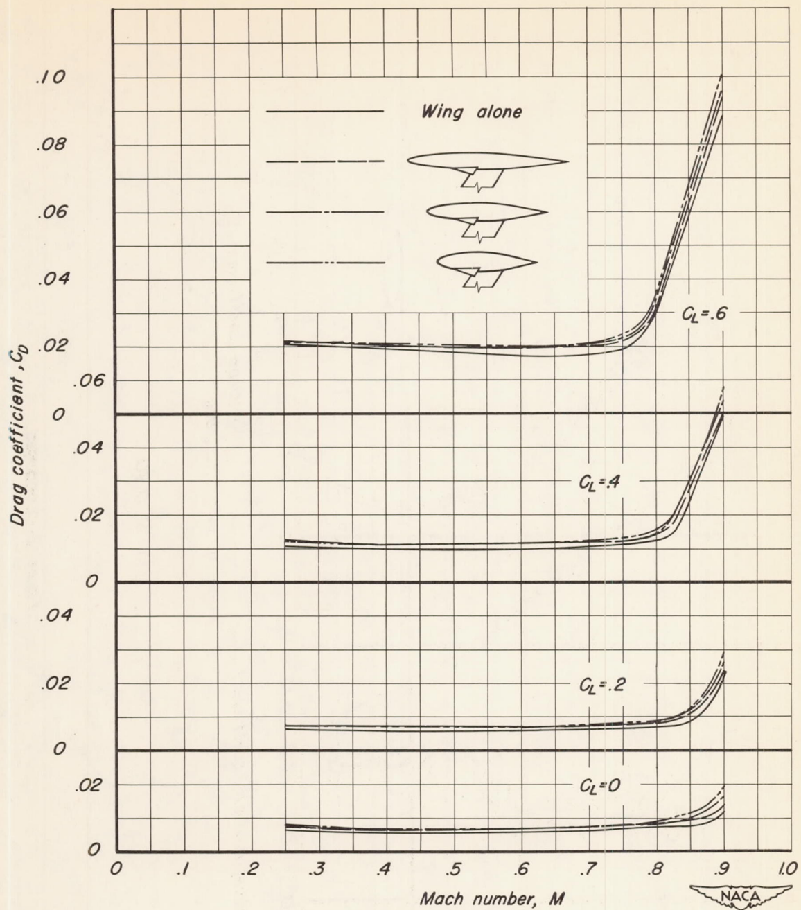
Figure 8.—The variation of drag coefficient with Mach number. R, 2,000,000 .
