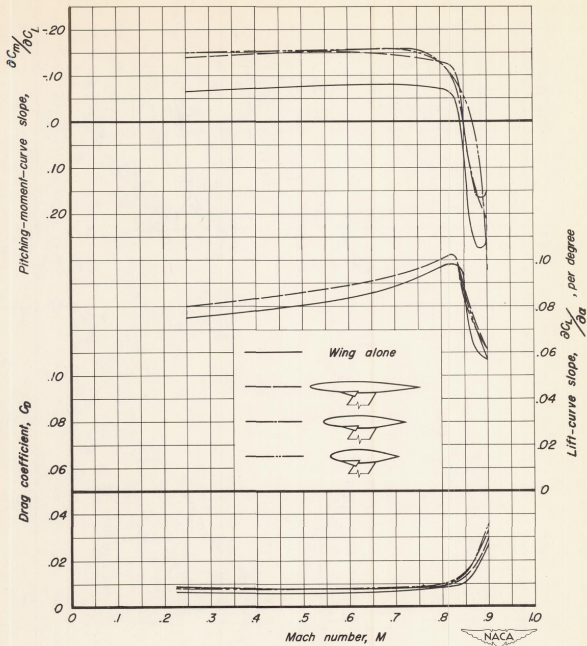
Figure 10.- The variations of pitching-moment-curve slope, lift-curve slope, and drag coefficient with Mach number. C_L , 0.25.
