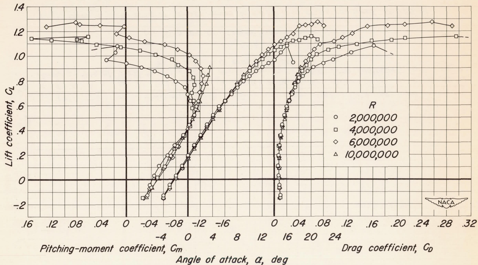
(d) Wing and tip tank of fineness ratio 5.
