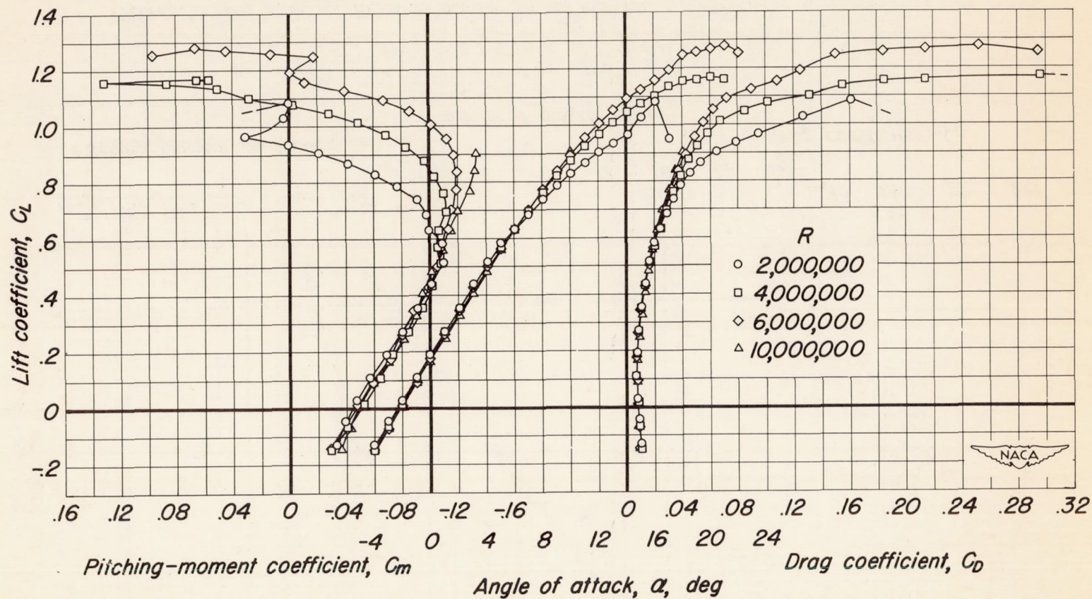
(b) Wing and tip tank of fineness ratio 10.
