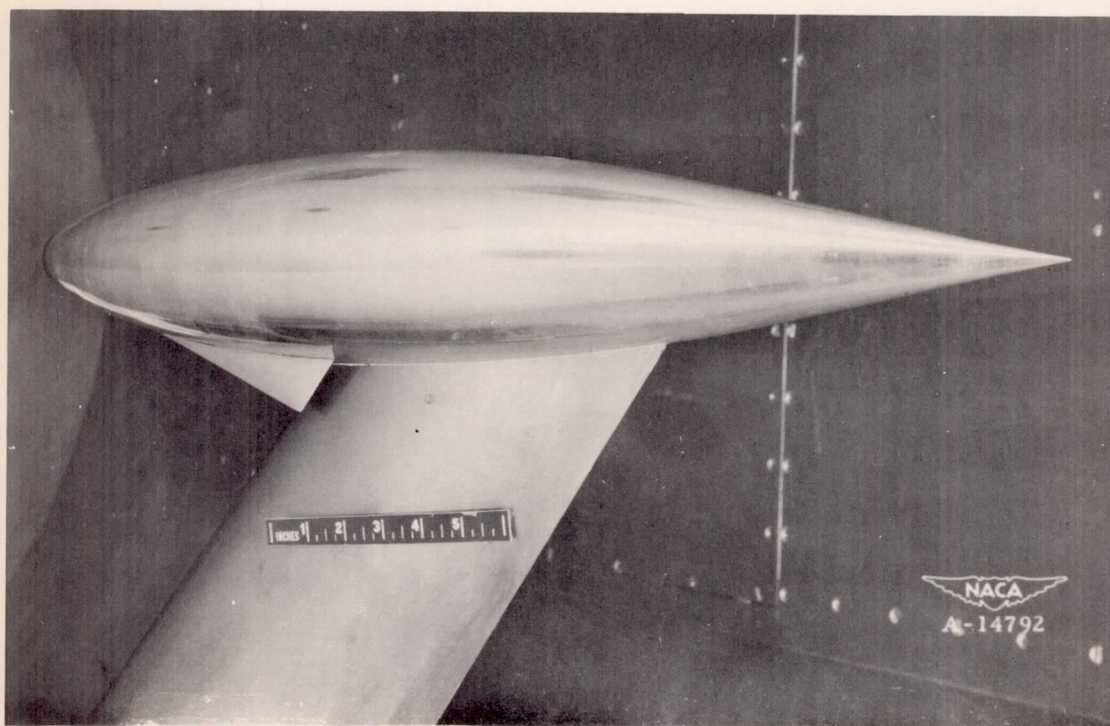
Figure 2.- Photographs of the model mounted in the Ames 12-foot pressure wind tunnel and the tip-tank installation.
