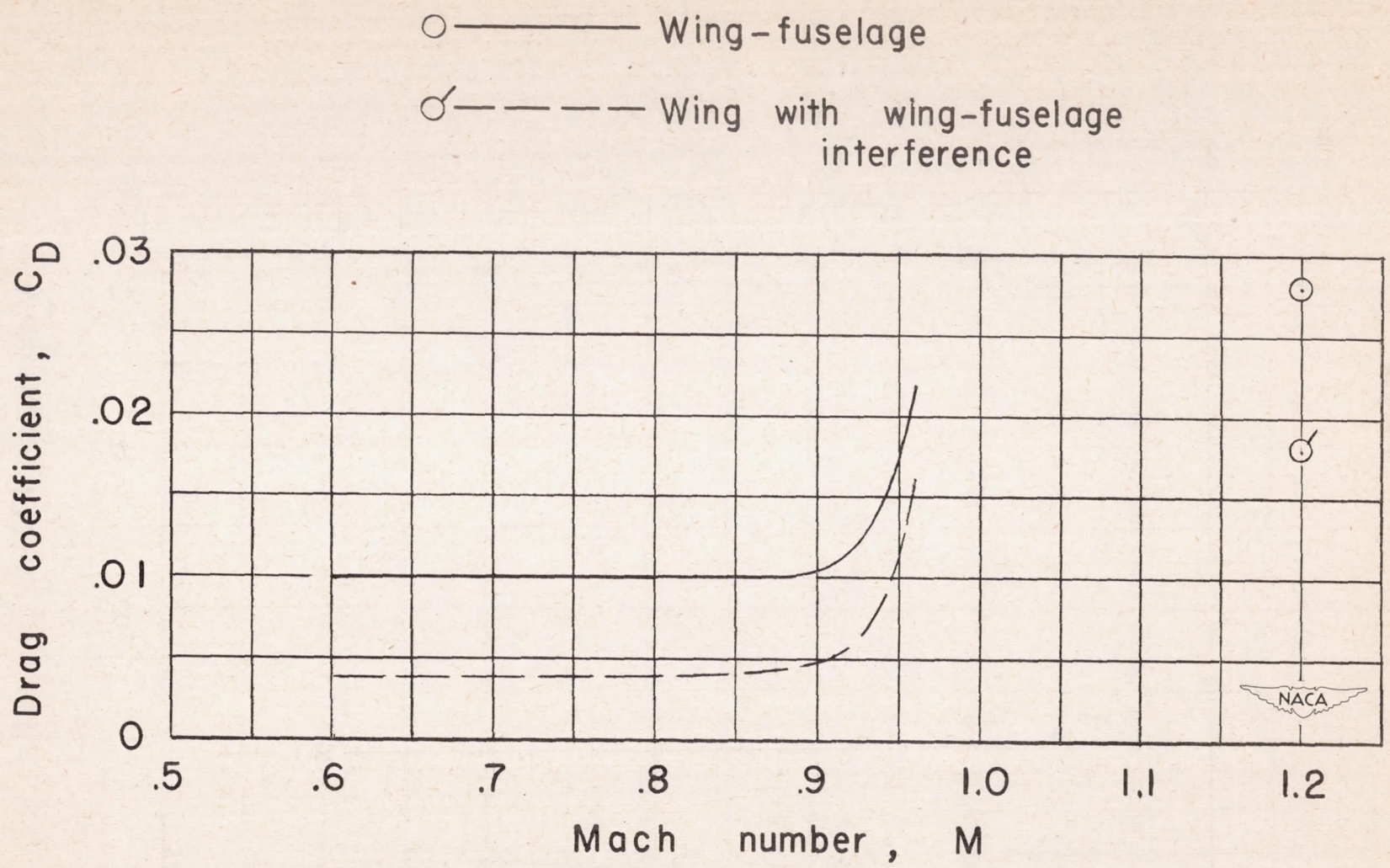
Figure 13.- Drag characteristics at zero lift as a function of Mach number for the wing-fuselage configuration and the wing with wing-fuselage interference.
