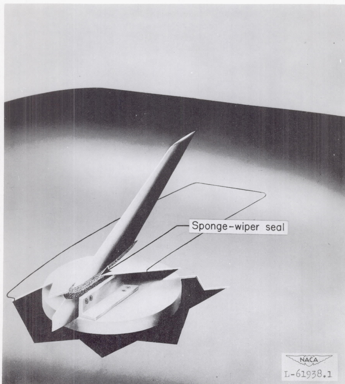
Figure 5.- Pictorial view showing sponge-wiper-seal installation on the model. \alpha = 0^\circ .
