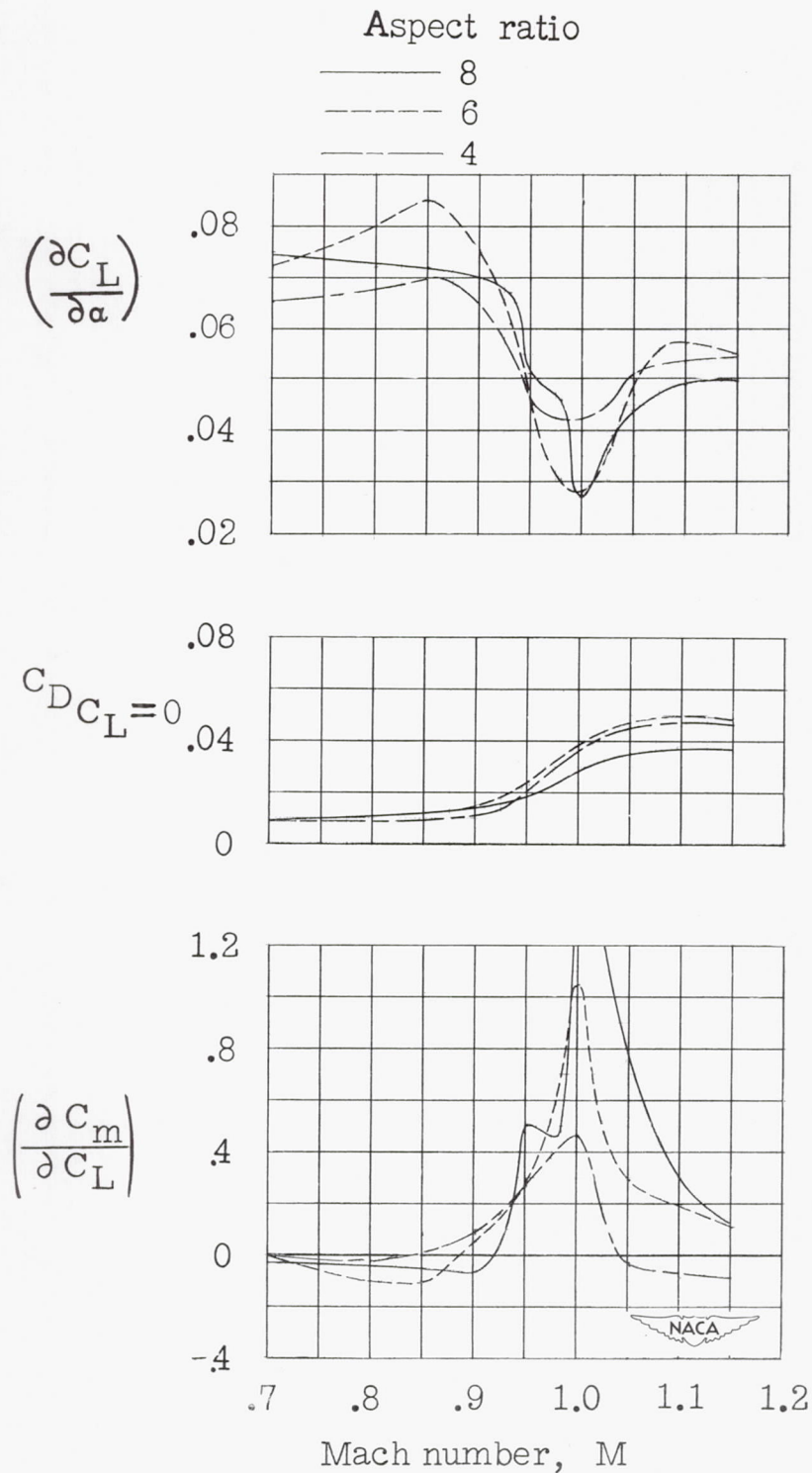
Figure 9.- Lift-curve slopes, drag coefficient at zero lift, and aerodynamic-center location of wings with 45^\circ sweepback and NACA 63 1 A012 airfoil section.
