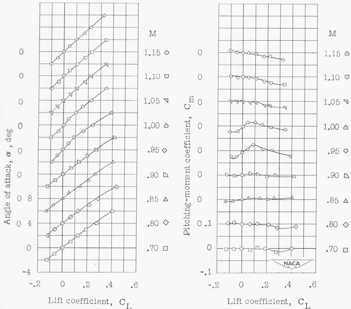
Figure 8.- Aerodynamic characteristics of a 45^\circ sweptback wing with aspect ratio 4, taper ratio 0.68, and NACA 63 1 A012 airfoil.
