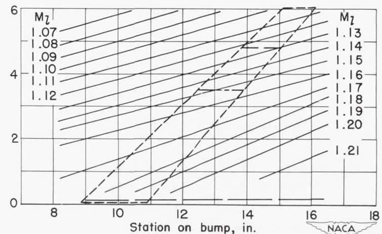
Figure 3.- Typical Mach number contours over transonic bump in region of model location.
