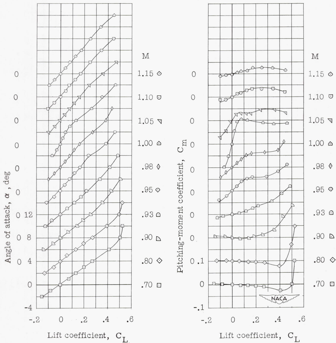
Figure 6.- Aerodynamic characteristics of a 45° sweptback wing with aspect ratio 8, taper ratio 0.45, and NACA 63 1 A012 airfoil.
