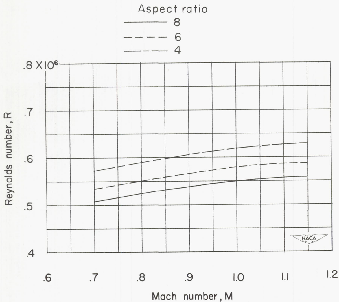
Figure 4.- Variation of test Reynolds number with Mach number for wings with 45^\circ sweepback and NACA 63 1 A012 airfoil section.
