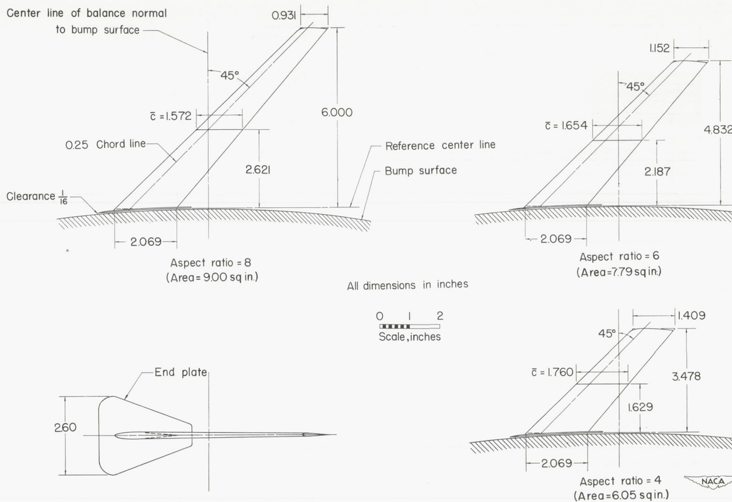
Figure 1.- Plan-form drawings of tapered wings having aspect ratios 4, 6, and 8, quarter-chord lines swept back 45°, and NACA 63 1 A012 airfoil sections.
