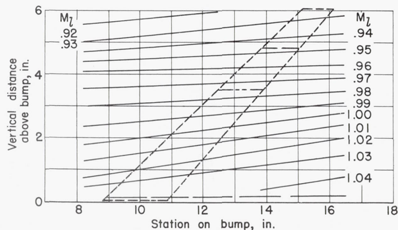
Figure 3.- Typical Mach number contours over transonic bump in region of model location.
