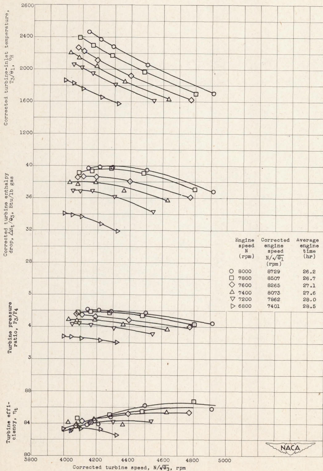
Figure 9. - Continued - Variation of basic turbine-performance parameters with engine speed and corrected turbine speed. Cowl-inlet pressure ratio, 1.025; standard tail-pipe configuration.
