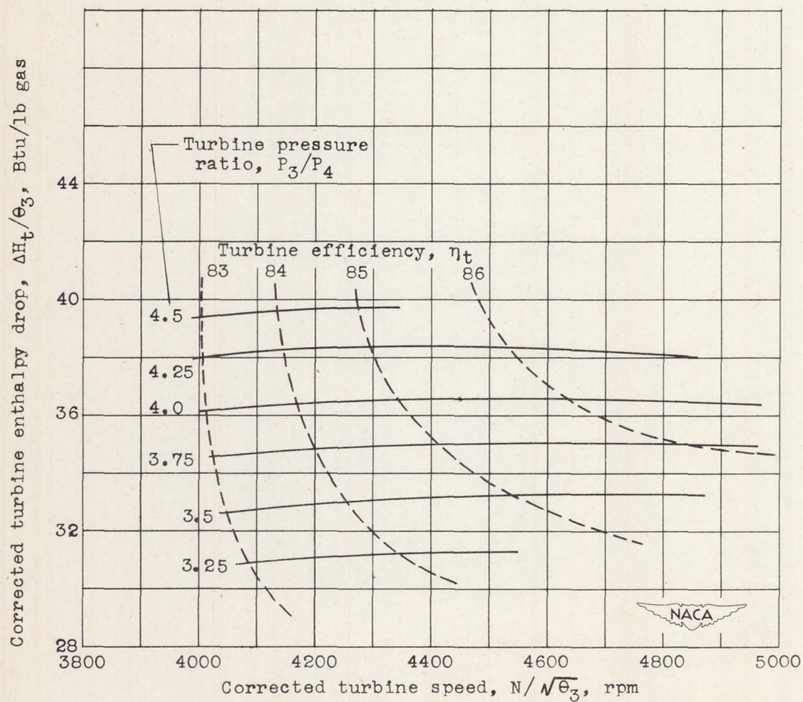
Figure 10. - Turbine-characteristic plot.
