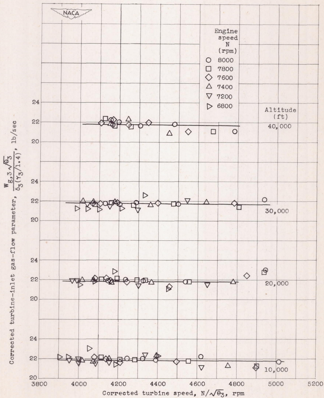
Figure 8. - Variation of corrected turbine-inlet gas-flow parameter with corrected turbine speed at various altitudes. Cowl-inlet pressure ratio, 1.025; standard tail-pipe configuration.
