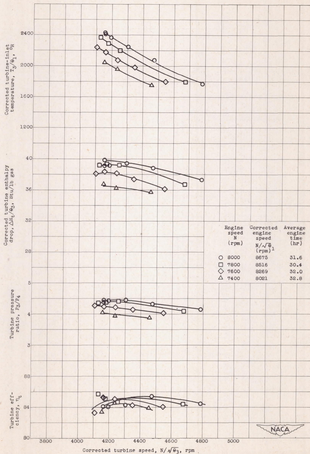
Figure 9. - Concluded - Variation of basic turbine-performance parameters with engine speed and corrected turbine speed. Cowl-inlet pressure ratio, 1.025; standard tail-pipe configuration.
