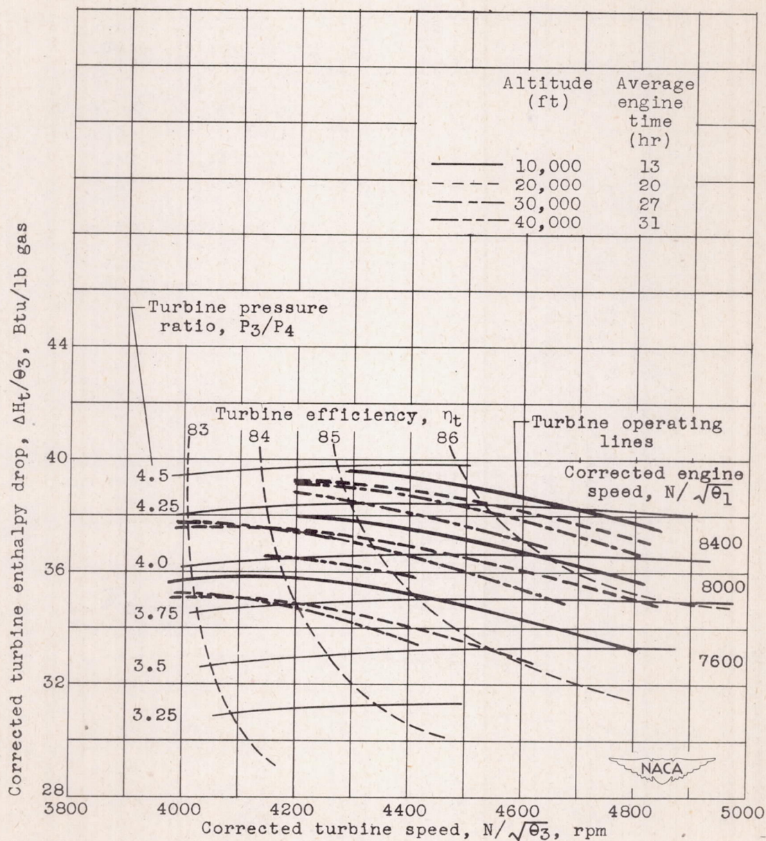
Figure 13. - Effect of altitude on turbine operating lines at several engine speeds. Cowl-inlet pressure ratio, 1.025; standard tail-pipe configuration.
