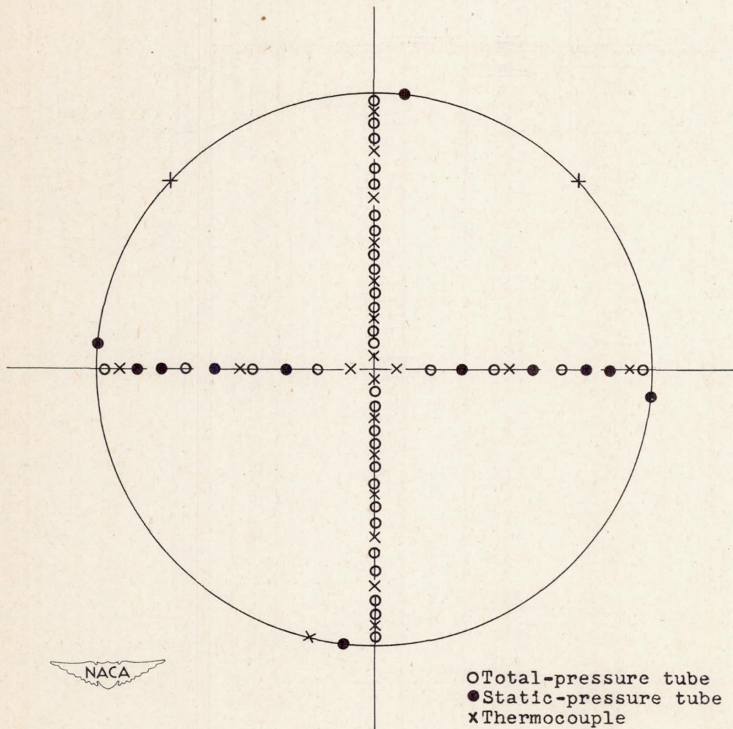
(a) Location of instrumentation. View looking downstream.
