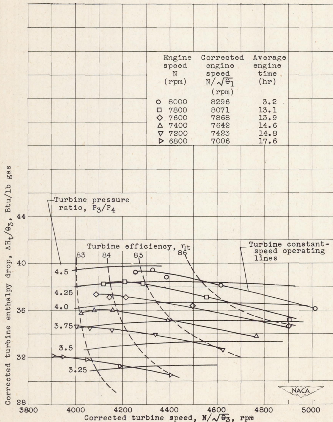
Figure 12. - Turbine operating lines at constant engine speed. Altitude, 10,000 feet; cowl-inlet pressure ratio, 1.025; standard tail-pipe configuration.
