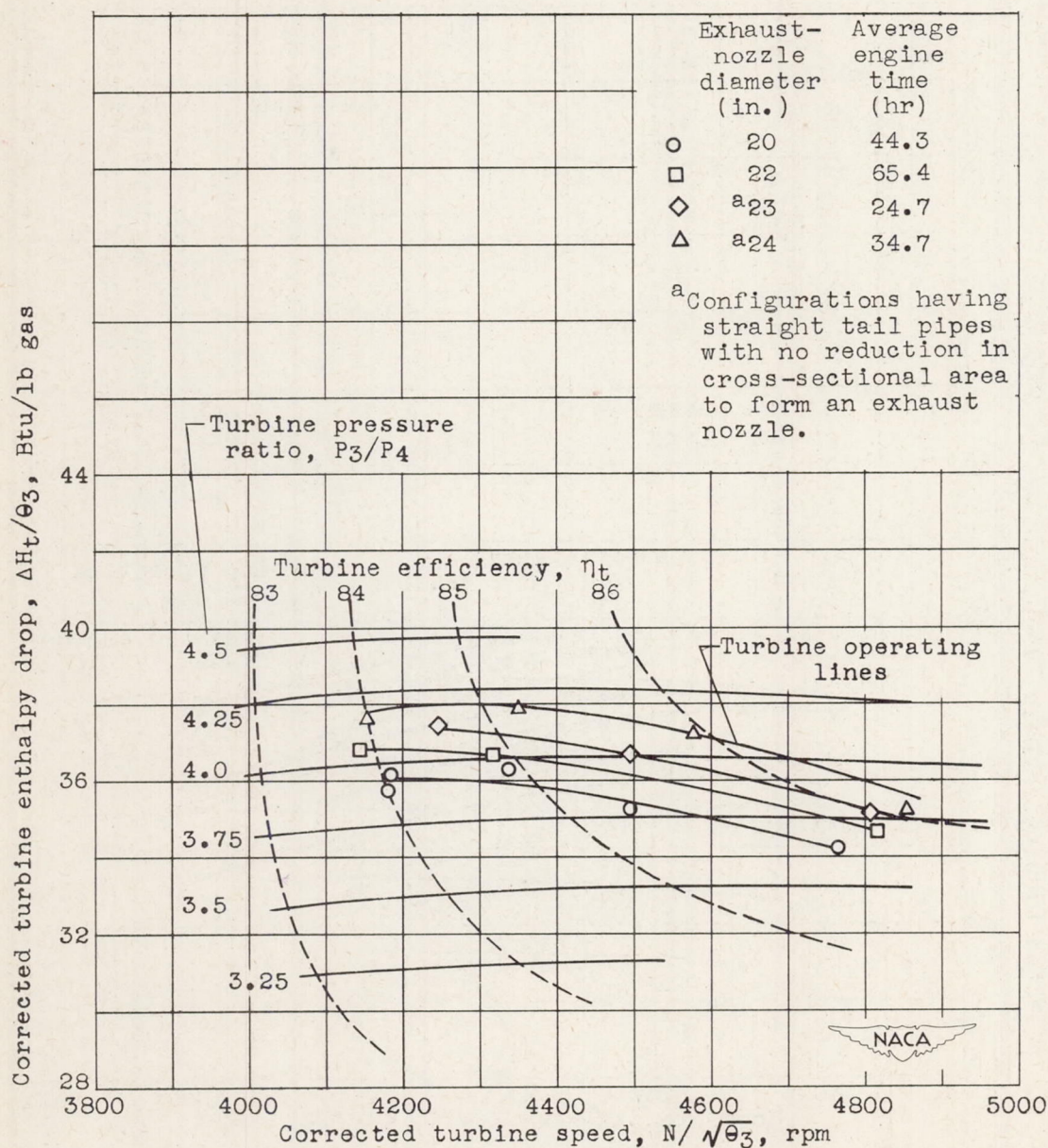
Figure 14. - Effect of tail-pipe configuration on turbine operating lines at altitude of 10,000 feet. Cowl-inlet pressure ratio, 1.025; corrected engine speed, 8000 rpm.
