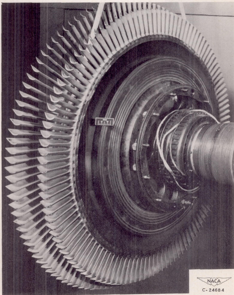
Figure 3. - Turbine rotor of Python turbine-propeller engine.
