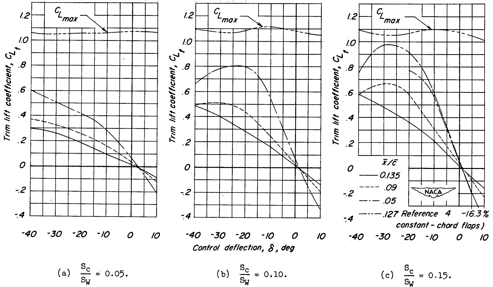
Figure 12.- Effect of static margin on variation of trim lift coefficient with control deflection for the three half-delta tip-control configurations. Wing-fuselage combination.
