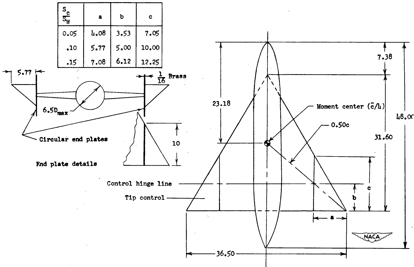
Figure 2.- Sketch of the model used in the investigation. (All dimensions are in inches.)
