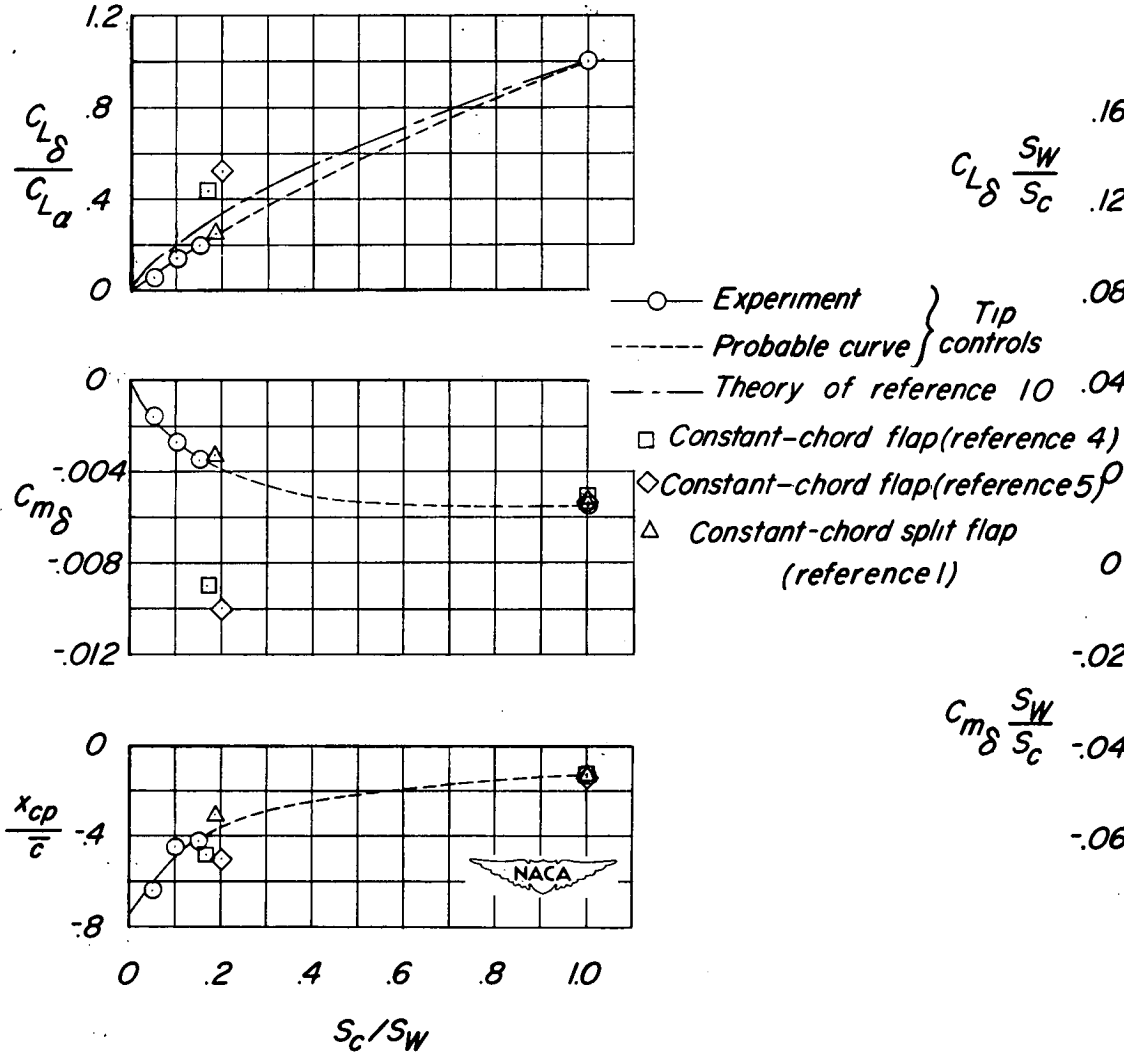
Figure 10.- Effect of control area on control-effectiveness and center-of-pressure characteristics. Wing-fuselage combination; \alpha = 0^\circ ; \delta = 0^\circ .
