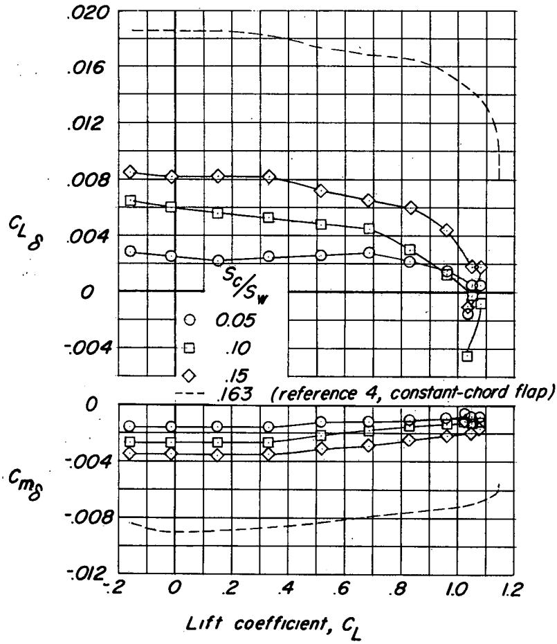
(a) Effect of control area and comparison with constant-chord flap controls. Wing-fuselage combination.
