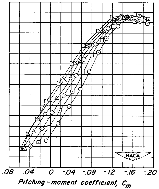
Figure 5.- Longitudinal stability and control characteristics of a 60° triangular wing and fuselage combination with 5-percent-area half-delta tip controls.
