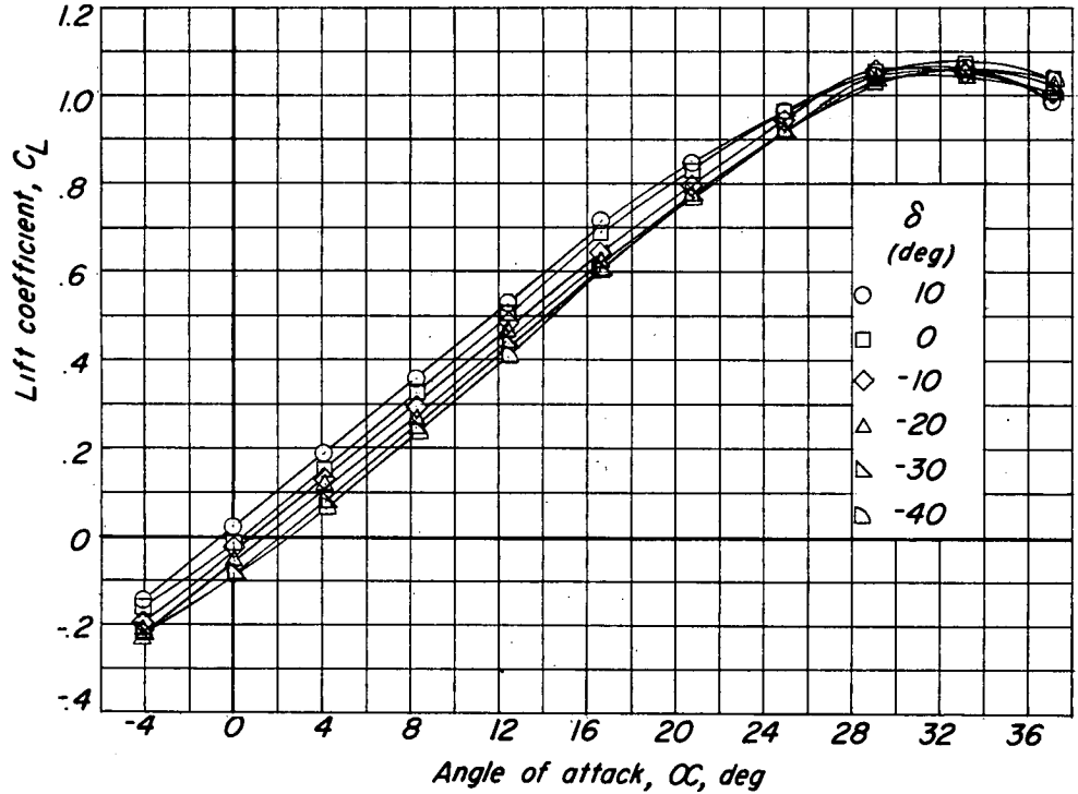
Figure 5.- Longitudinal stability and control characteristics of a 60° triangular wing and fuselage combination with 5-percent-area half-delta tip controls.
