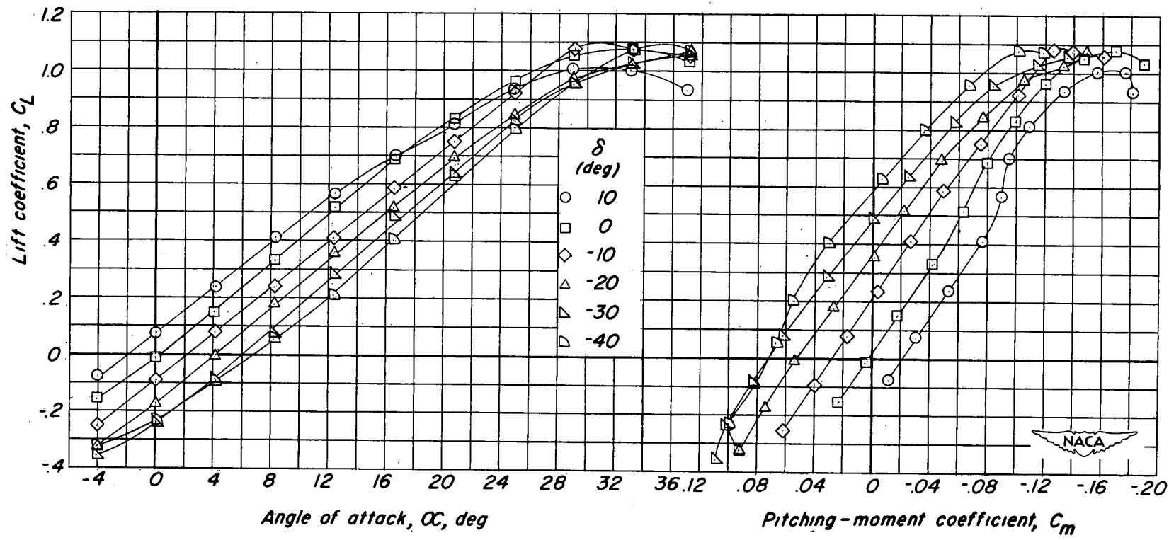
Figure 7.- Longitudinal stability and control characteristics of a 60° triangular wing and fuselage combination with 15-percent-area half-delta tip controls.
