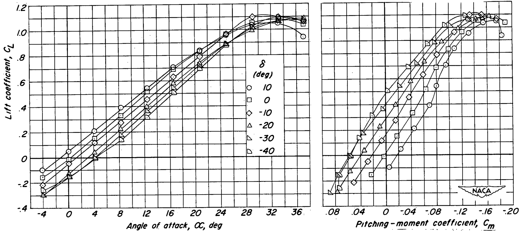
Figure 6.- Longitudinal stability and control characteristics of a 60° triangular wing and fuselage combination with 10-percent-area half-delta tip controls.
