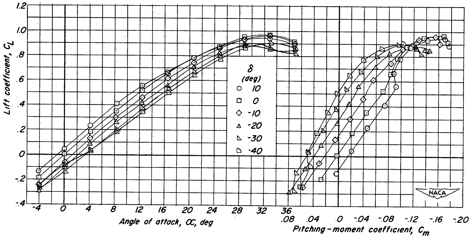
Figure 8.- Longitudinal stability and control characteristics of a 60° triangular wing and fuselage combination with 10-percent-area half-delta tip controls and end plates.
