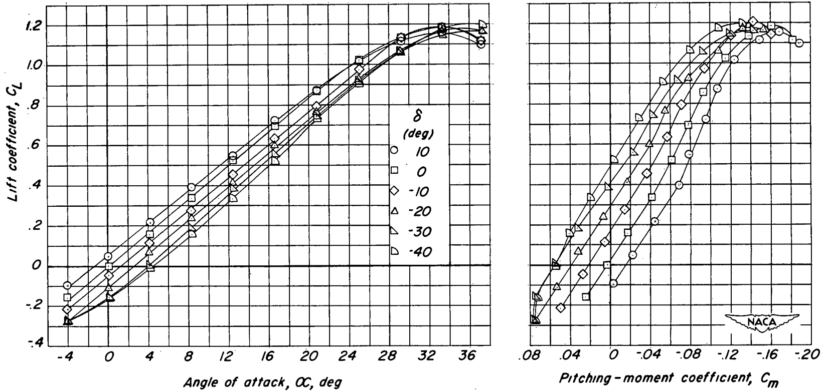
Figure 4.- Longitudinal stability and control characteristics of a 60^\circ triangular wing with 10-percent-area half-delta tip controls.
