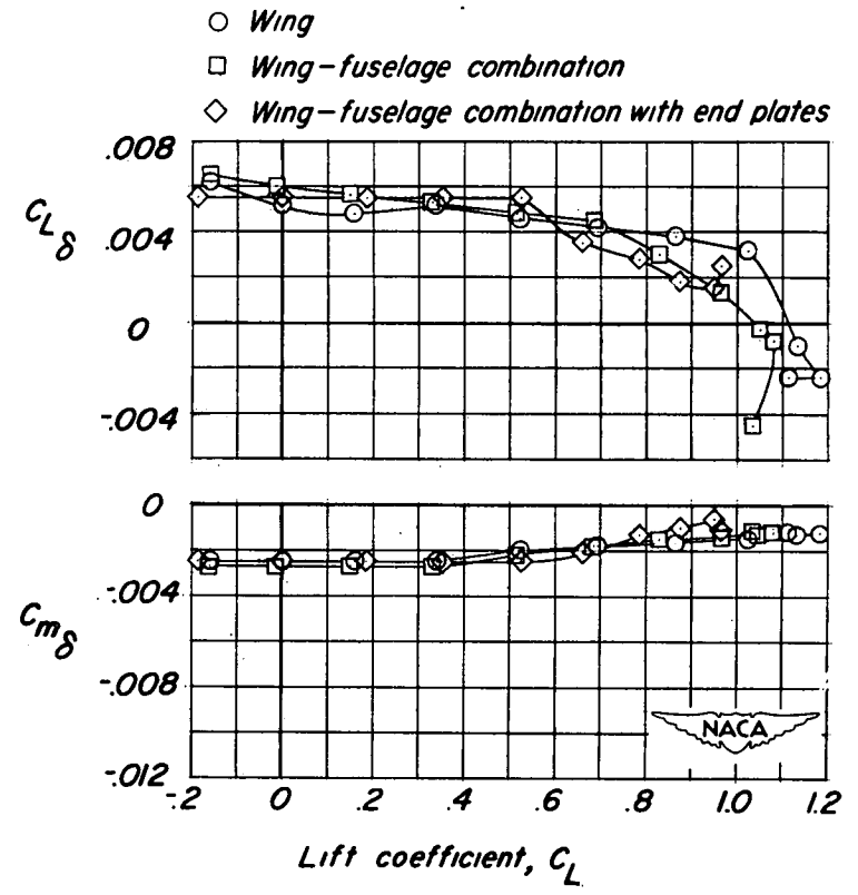
(b) Effect of fuselage and end plates
