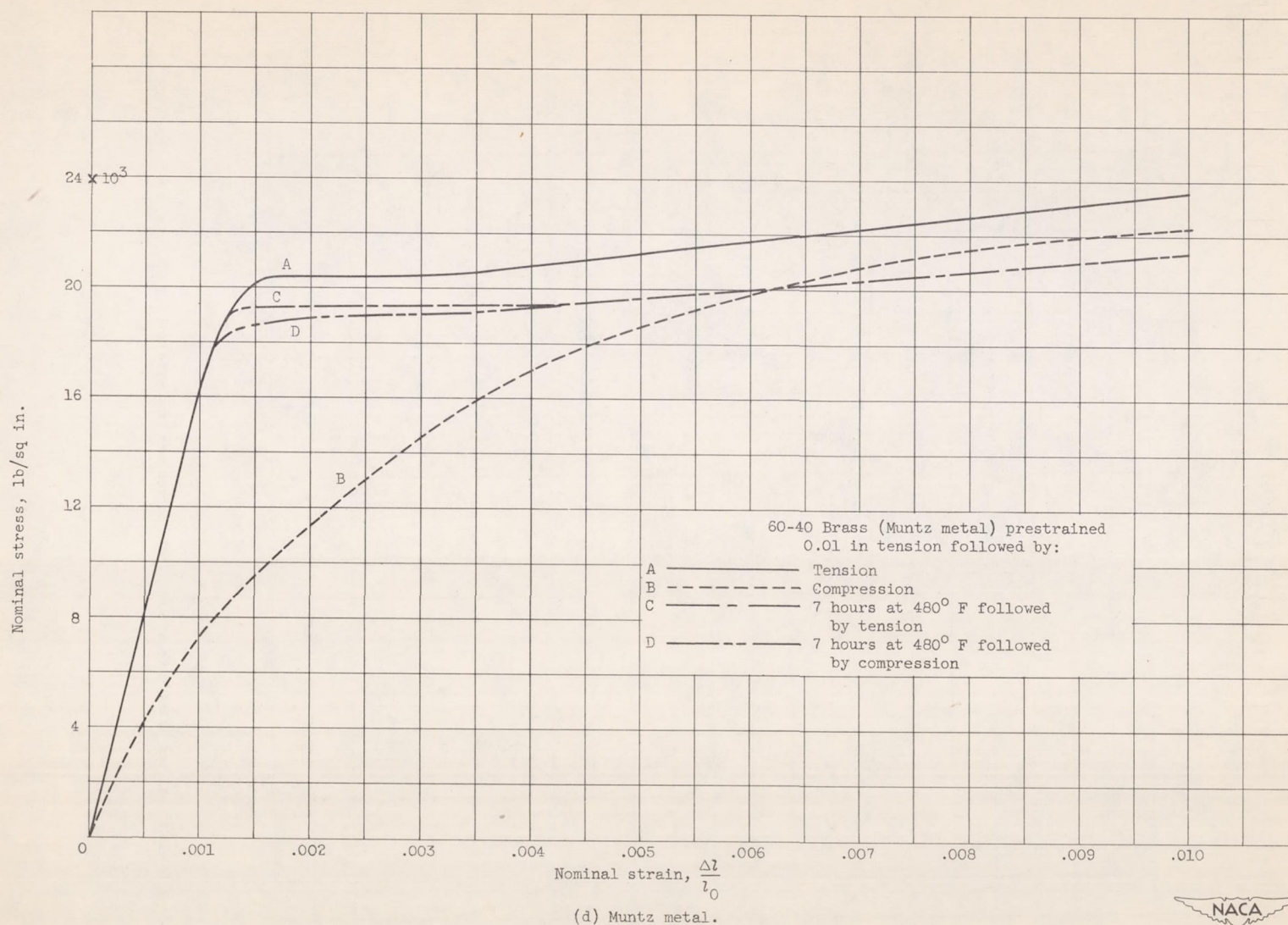
Figure 12. - Concluded. Tension and compression stress-strain curves for tensile prestrained copper and brass and specimens with and without intermediate anneals.
