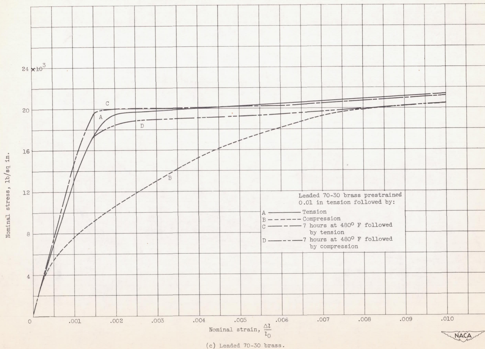
Figure 12. - Continued. Tension and compression stress-strain curves for tensile prestrained copper and brass specimens with and without intermediate anneals.
