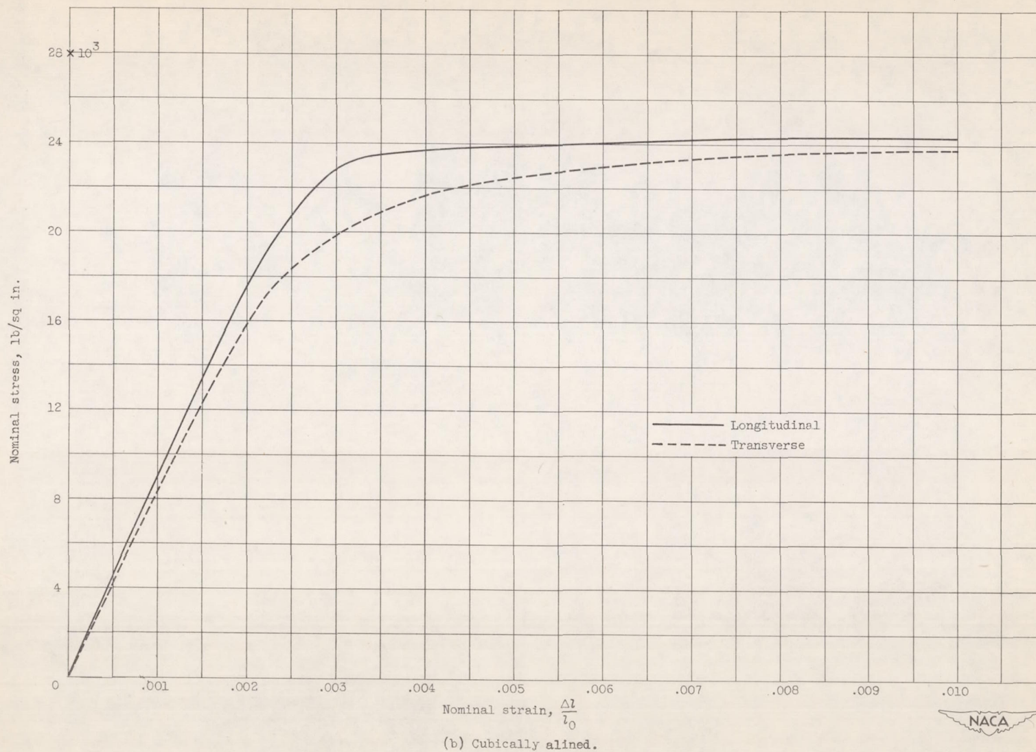
Figure 14. - Concluded. Longitudinal and transverse tension stress-strain curves for specimens cut from isotropic and cubically aligned copper sheet prestrained 10 percent in tension.
