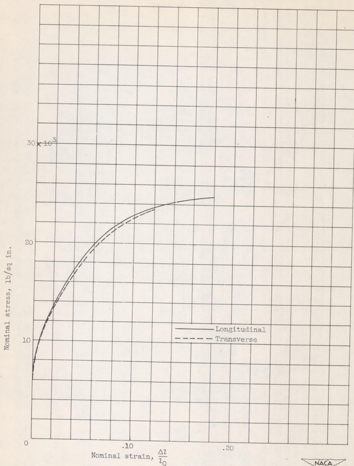
Figure 13. - Concluded. Longitudinal and transverse stress-strain curves for isotropic and cubically aligned copper sheet.
