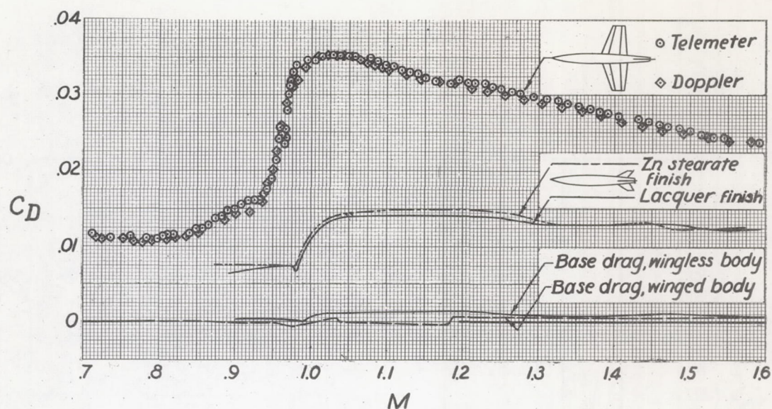
(a) Basic drag data.
