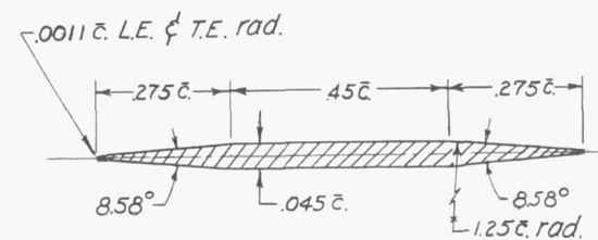
Streamwise wing profile expressed in percent chord
