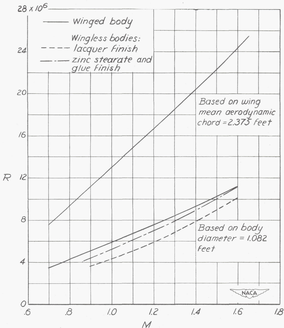
Figure 4.- Variation of Reynolds number with Mach number.
