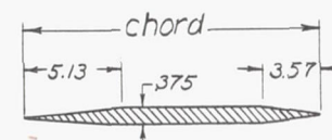
Typical streamwise fin section
