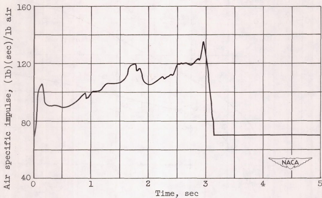
Figure 14. - Air specific impulse obtained with cigarette-type fuel charge evaluated on preflight facility at NACA, Wallops Island. Fuel, MFM-20; inlet-air temperature, 769^{\circ}\text{R} ; simulated flight Mach number, 2.2; combustor length, 48 inches; average specific impulse, 107; air flow, 12.5 pounds per second; total fuel weight, 6.24 pounds.
