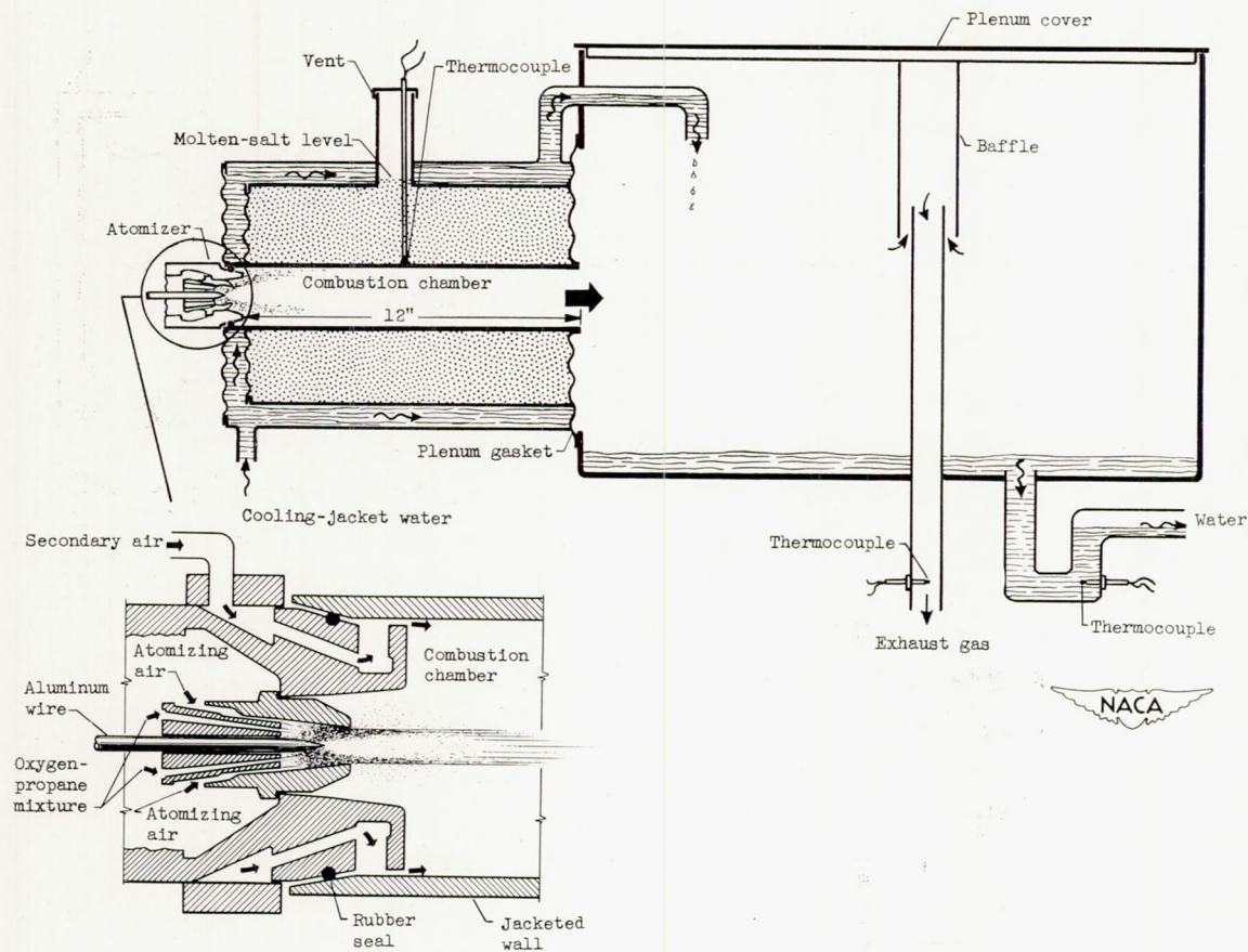
Figure 21. - Experimental setup for NACA 2-inch wire combustor (reference 37).
