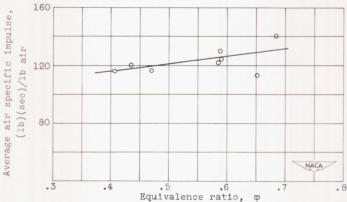
Figure 18. - Average air specific impulse for magnesium solid fuel determined at NACA, Wallops Island. Inlet-air temperature, 679° to 711° R; Mach number, 1.6 and 2.2; L^* , 40 to 51.3.
