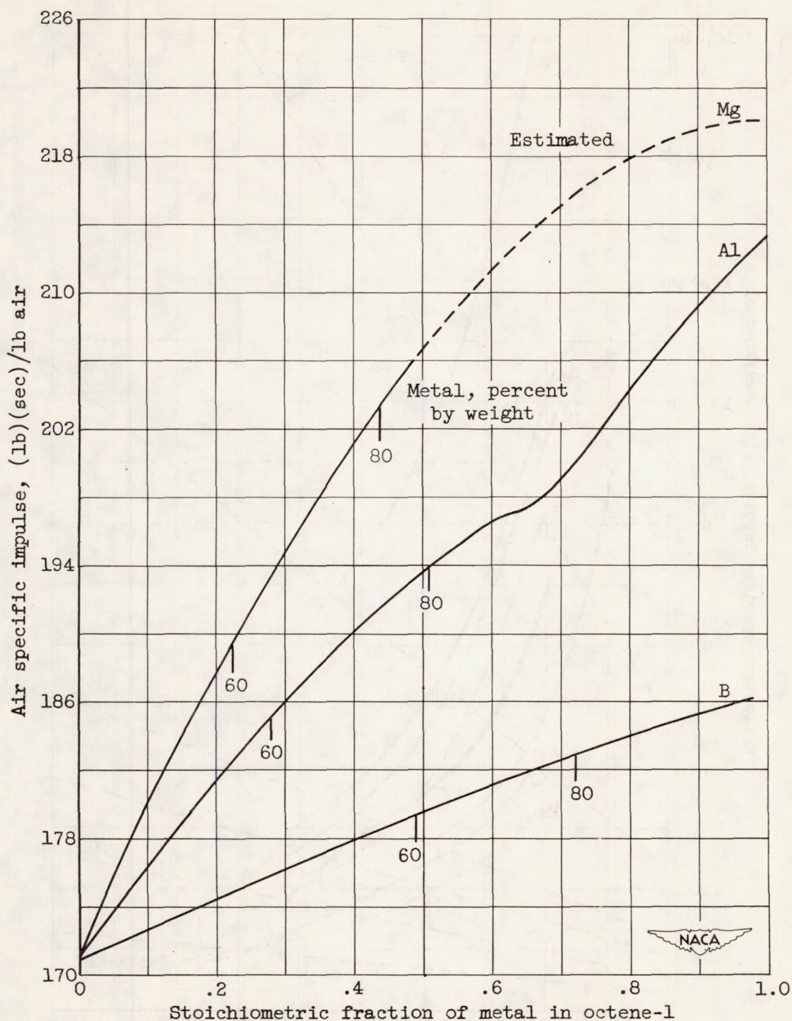
Figure 5. - Air specific impulse of metal slurries in octene-1. Stoichiometric fraction of slurry fixed at 1.0; combustor inlet-air temperature, 560^{\circ}\text{R} ; inlet-air pressure, 2 atmospheres. (From references 26, 27, and 28.)
