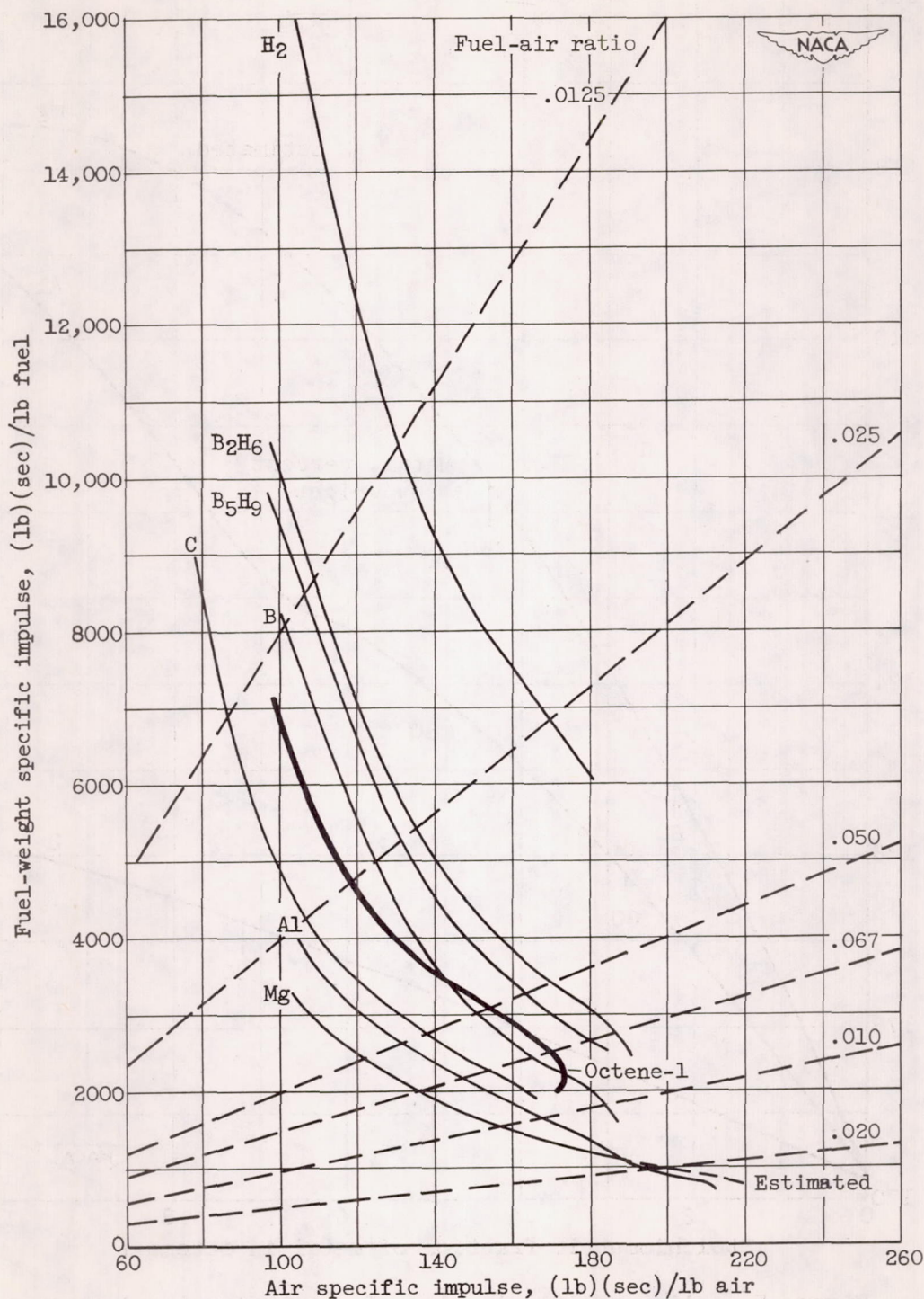
Figure 4. - Variation of fuel-weight specific impulse with air specific impulse for several ram-jet fuels. Combustor inlet-air temperature, 560^\circ\text{R} ; inlet-air pressure, 2 atmospheres. (From references 26, 27, and 28.)
