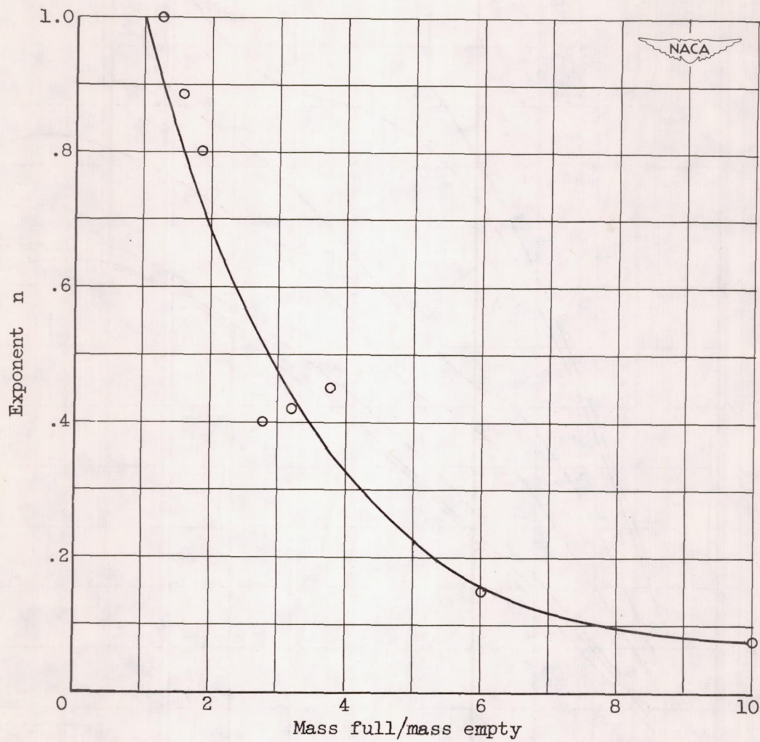
Figure 2. - Variation of exponent n with mass ratio of rocket-propelled vehicles. (From reference 19.)
