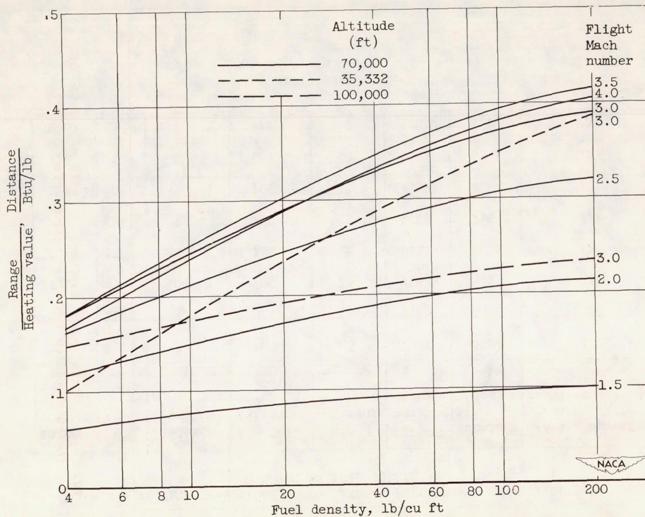
Figure 1. - Effect of fuel heating value and density on range of ram-jet aircraft. Gross weight, 150,000 pounds; pay load, 10,000 pounds.
