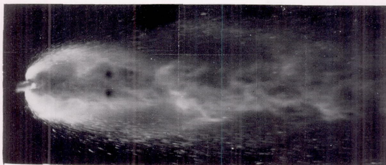
(a) 30-percent nonstabilized slurry of magnesium.
