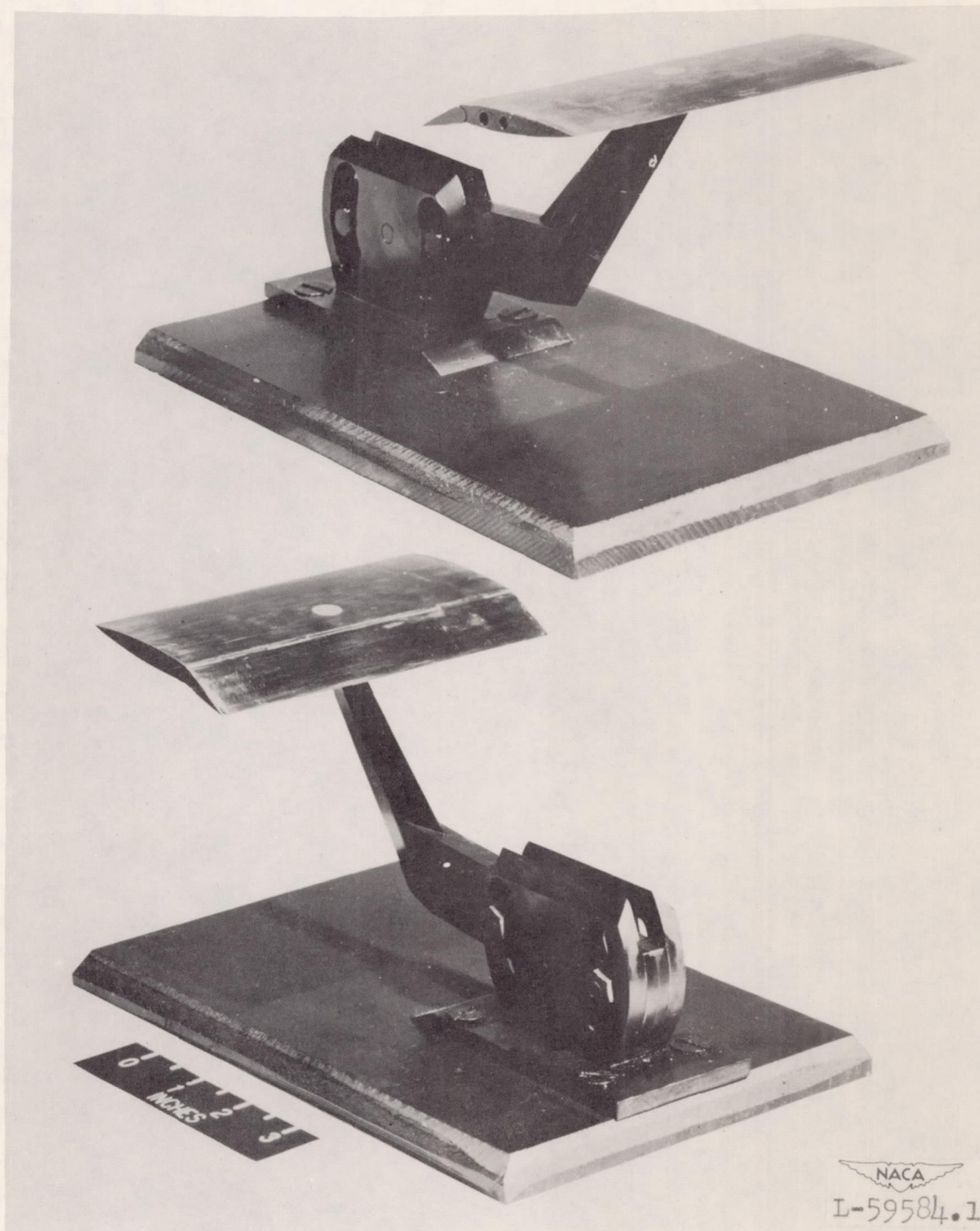
Figure 4.- Front and rear three-quarter views of 9-percent-thick symmetrical circular-arc wing used in schlieren observations.
