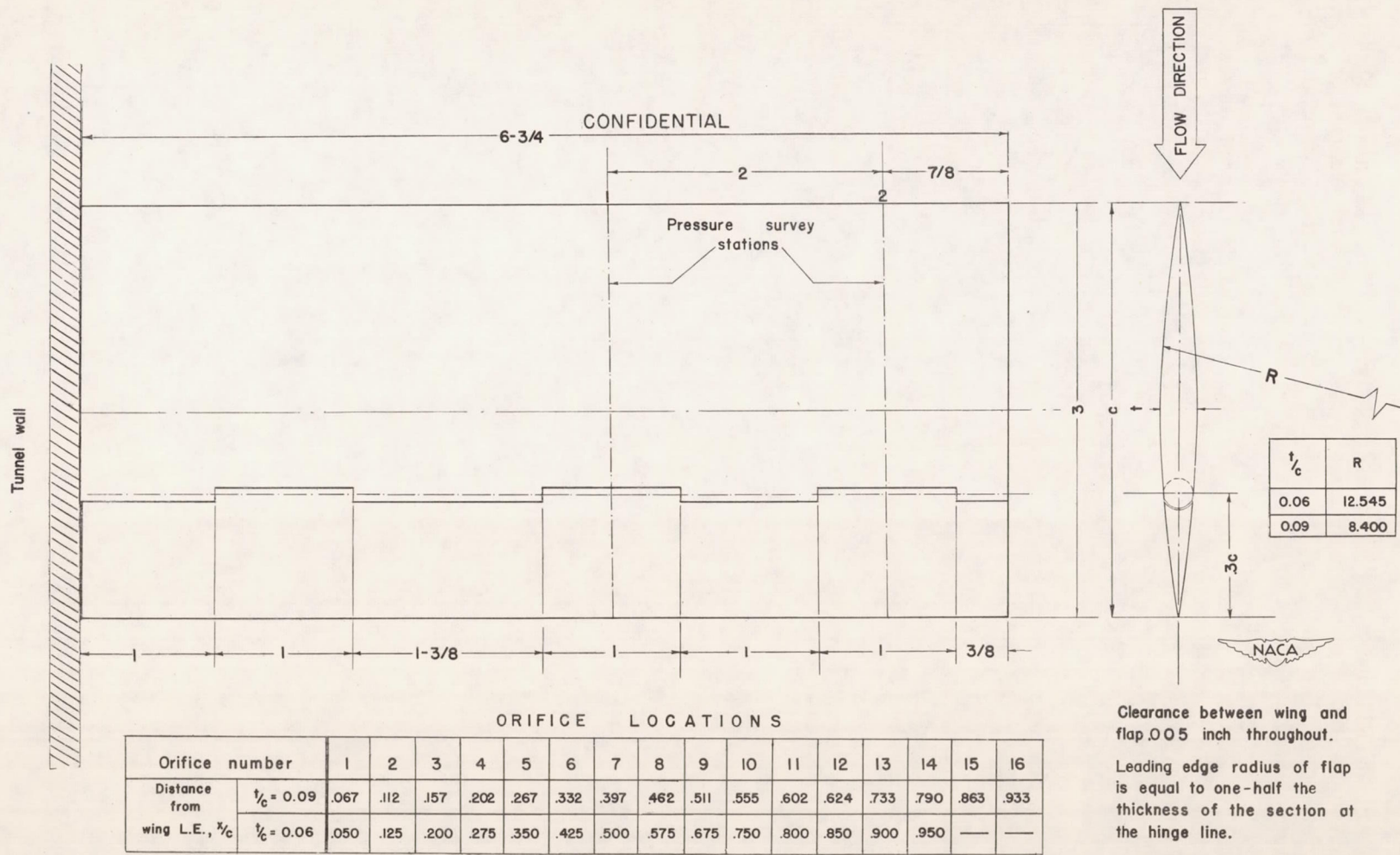
Figure 1.- Sketch showing pertinent dimensions of test models.
