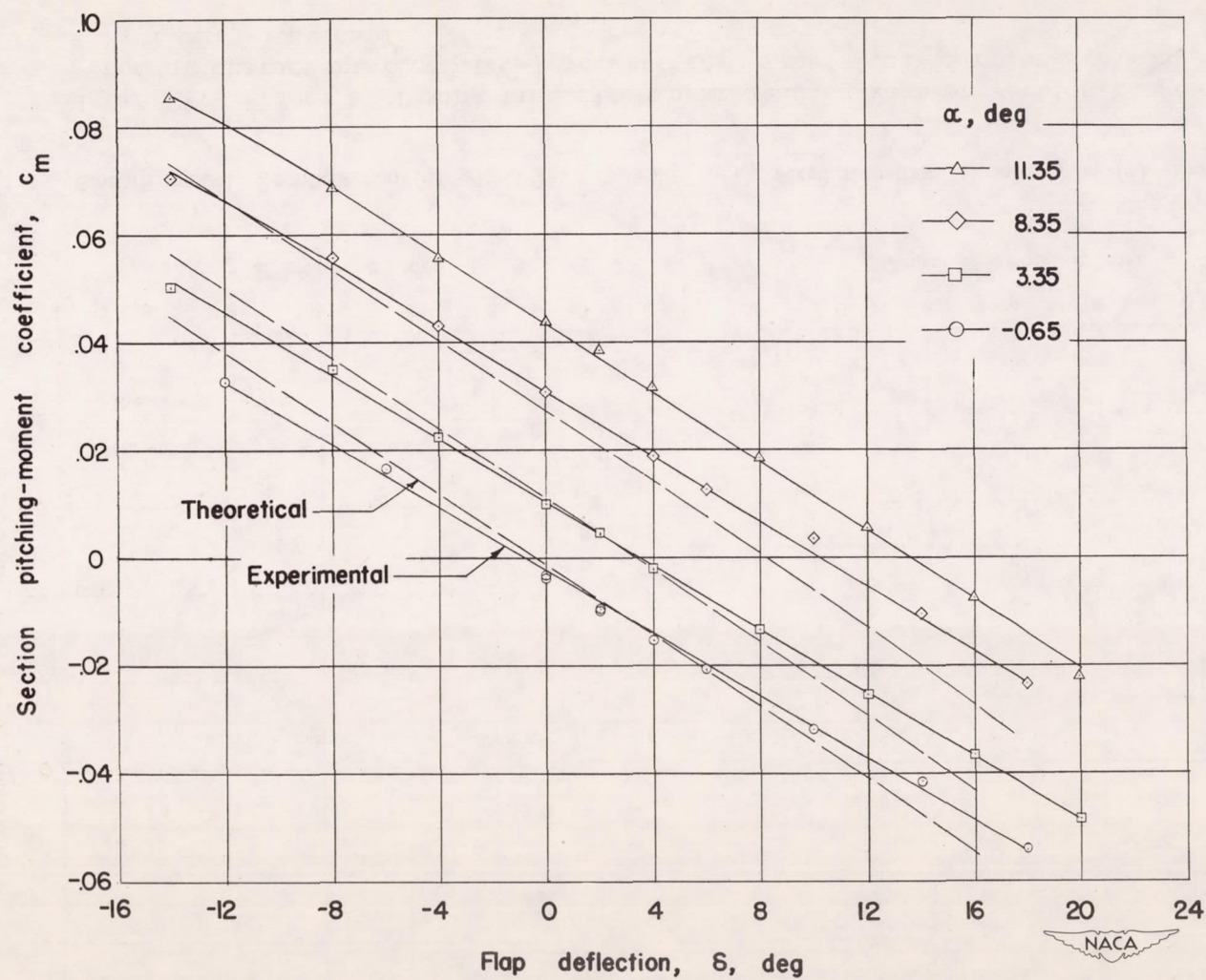
Figure 23.- Section pitching-moment characteristics of 9-percent-thick symmetrical circular-arc wing with fixed transition. Configuration (d), figure 5. M , 1.93. Station 1.
