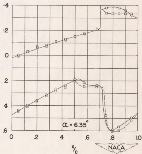
Figure 26.- Effect of sealing hinge gap on experimental pressure distribution over 6-percent-thick symmetrical circular-arc wing. M, 1.62 . Station 1.
