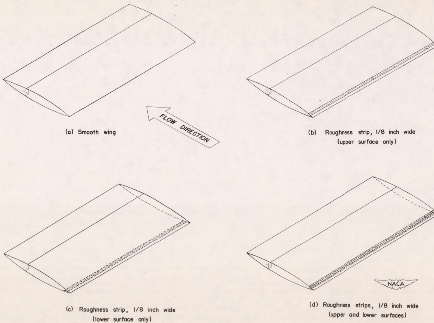
Figure 5.- Locations and extent of wing-surface roughness used in transition studies.
