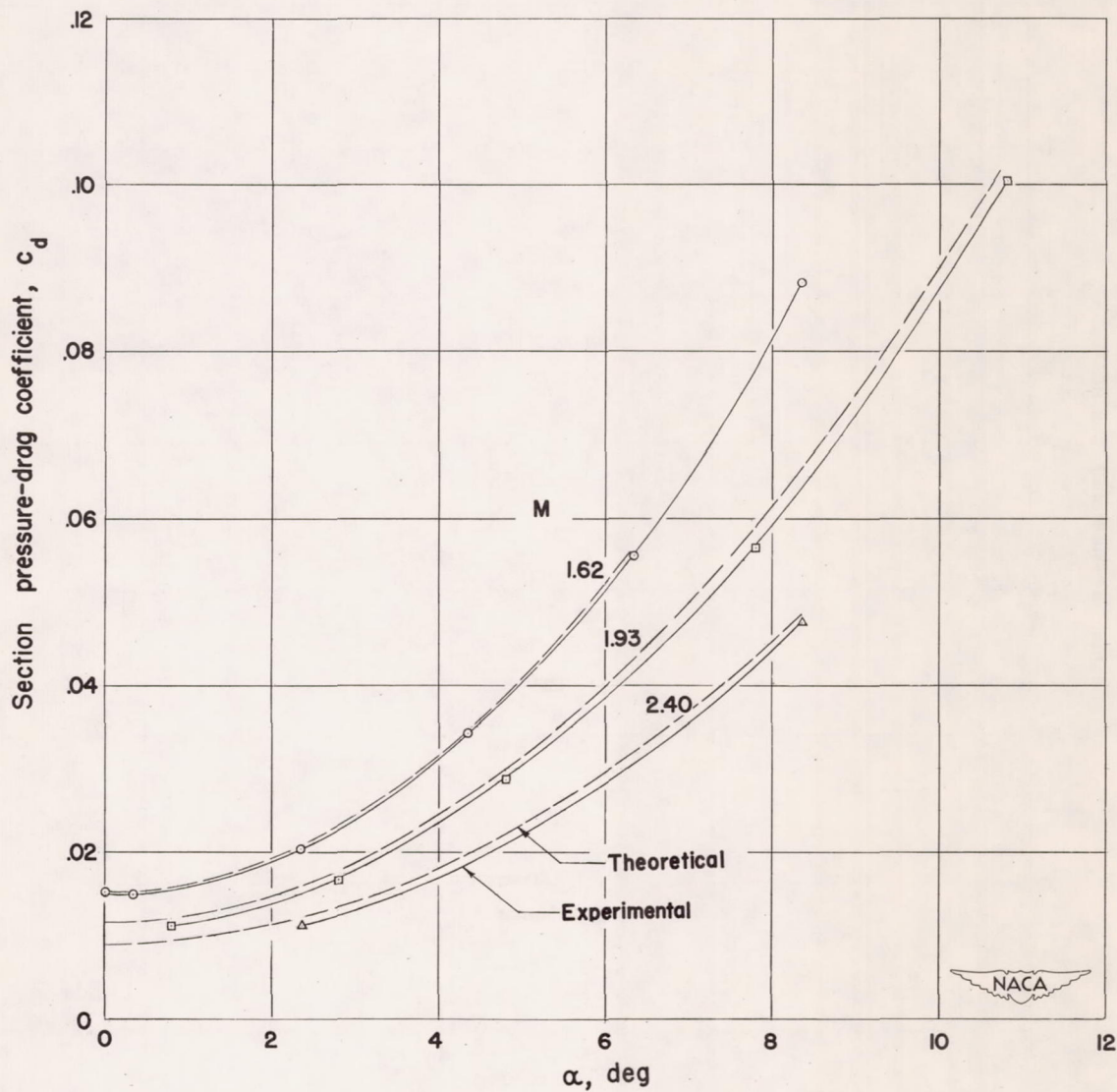
Figure 12.- Effect of Mach number on section pressure-drag coefficient of 6-percent-thick symmetrical circular-arc wing. \delta, 0^\circ . Station 1.
