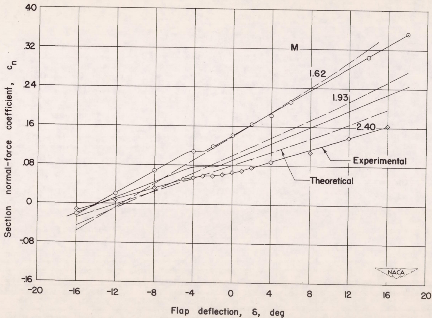
Figure 8.- Effect of Mach number on the section force and moment characteristics of 9-percent-thick symmetrical circular-arc wing. Station 1.
