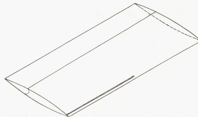
(f) Smooth strip of dope, 1/32 inch wide (upper surface only)
