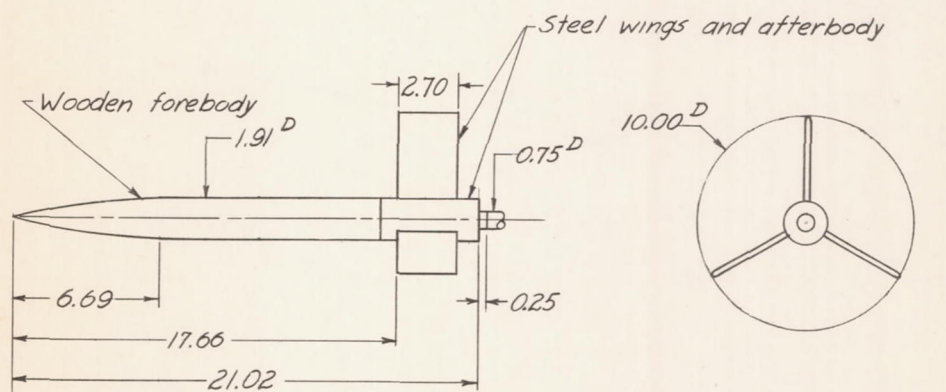
Sting-mounted test configuration
