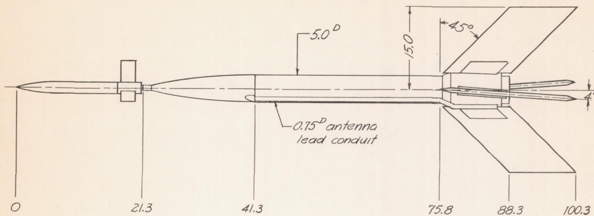
Sting-mount test vehicle
