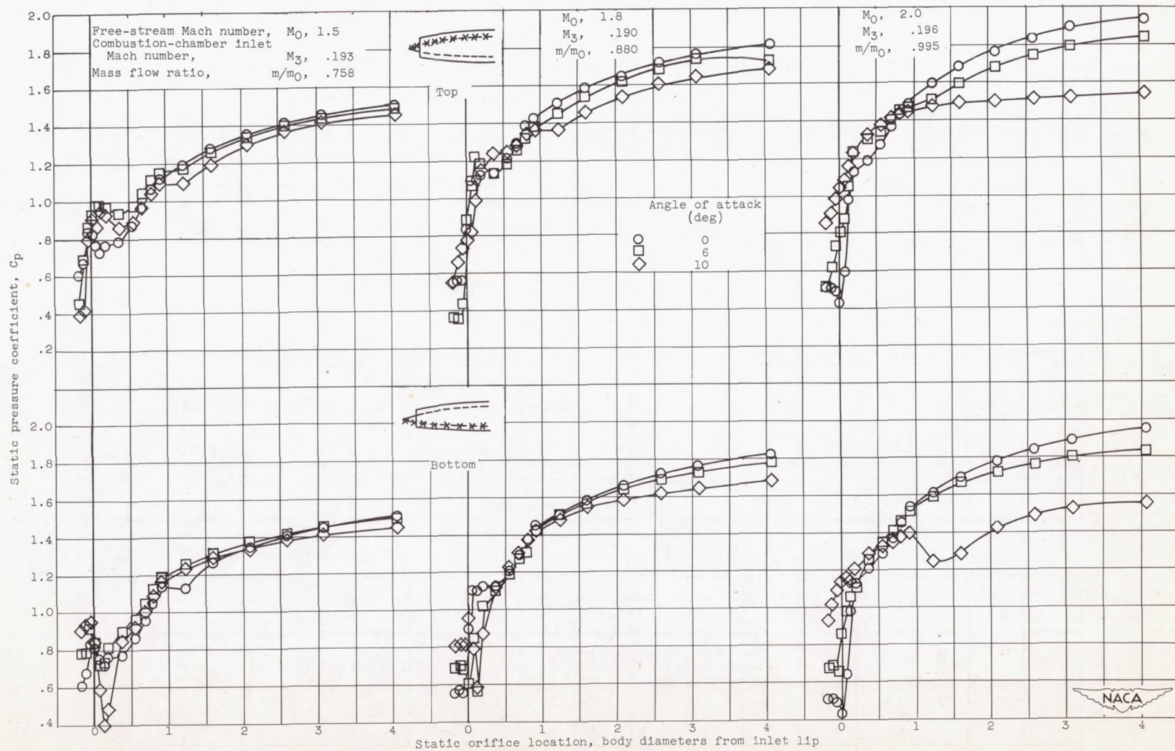
Figure 10. - Concluded. Variation in static pressure coefficients along diffuser at free-stream Mach numbers of 1.5, 1.8, and 2.0.
