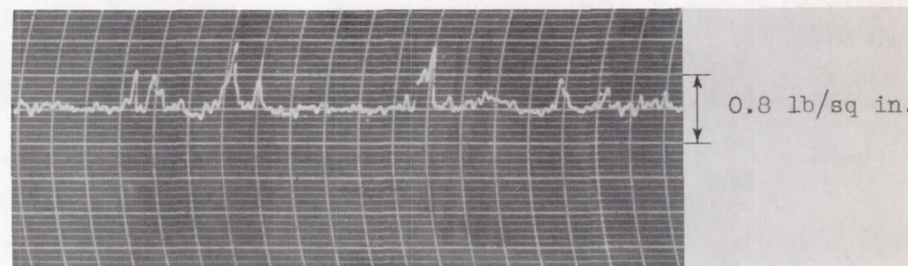
Diffuser exit
