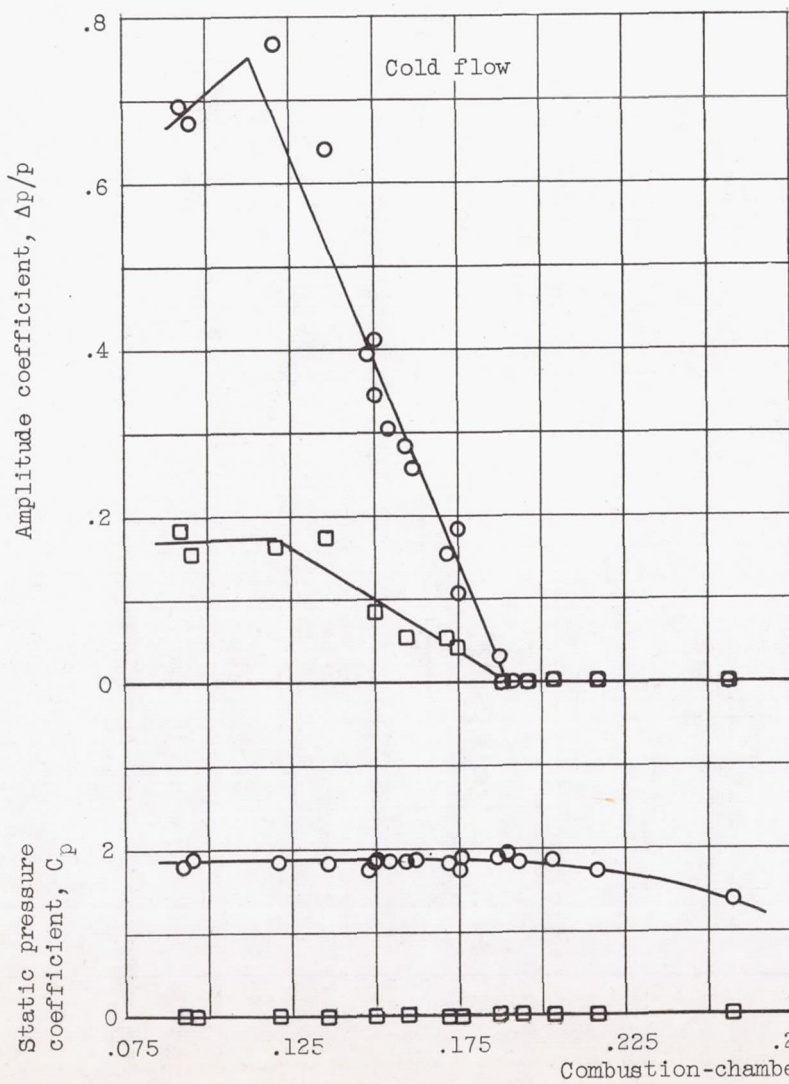
Figure 6. - Static-pressure fluctuation at diffuser exit and external surface of cowl for cold-flow and burning conditions. Mach number, 1.8; angle of attack, 0^\circ .
