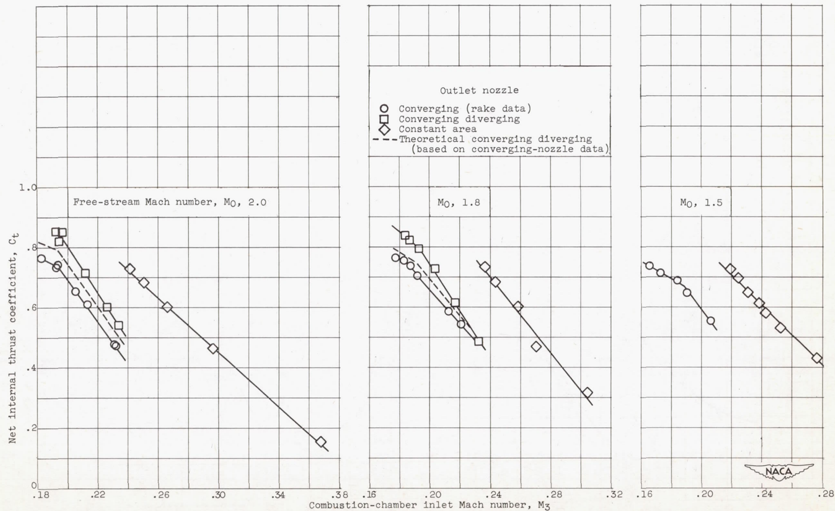
Figure 17. - Net internal thrust coefficients obtained with the three outlet nozzles at Mach numbers of 1.5, 1.8, and 2.0 at 0^\circ angle of attack.
