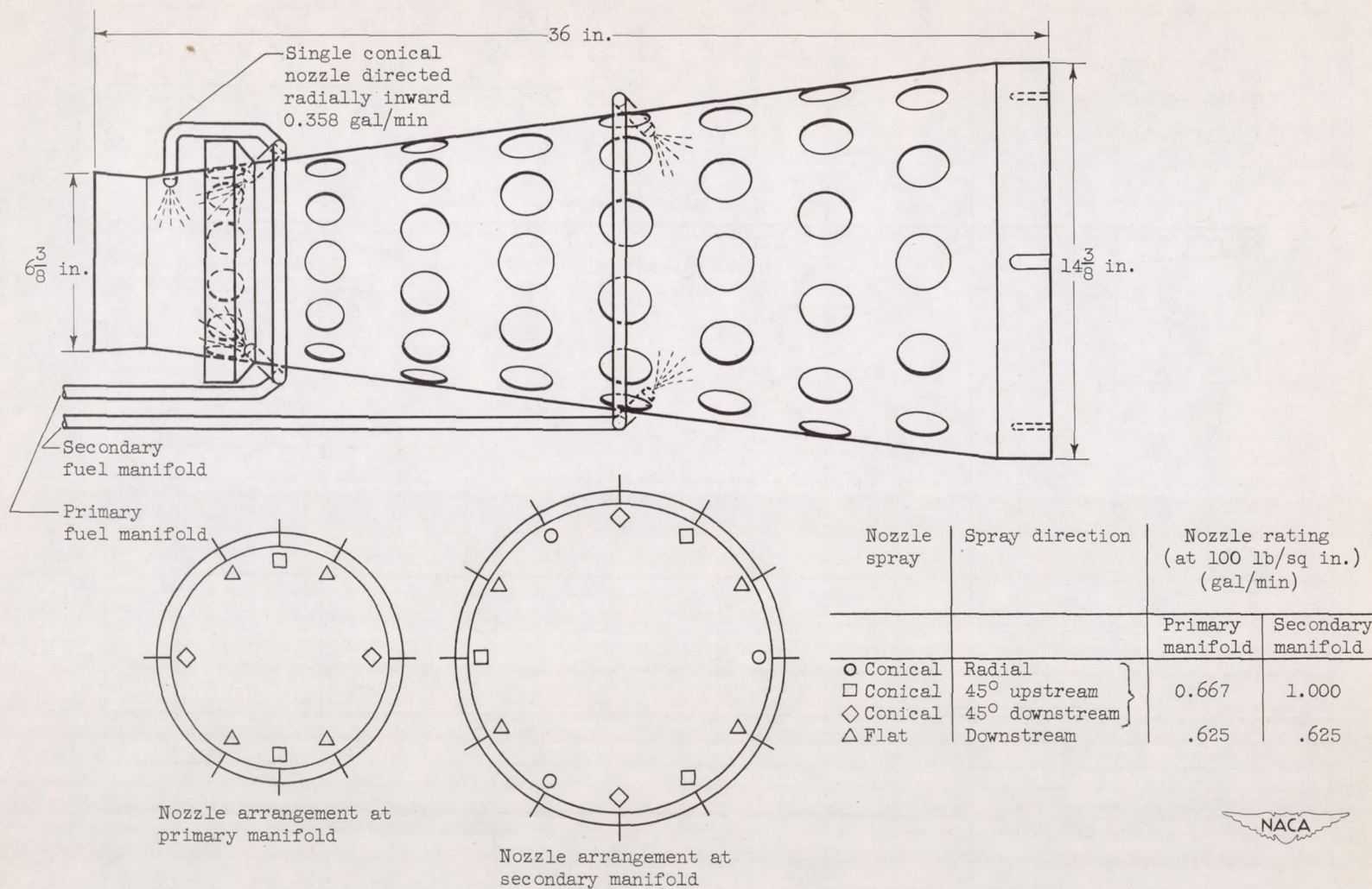
Figure 3. - Burner-configuration details.
