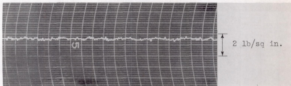
Diffuser exit
