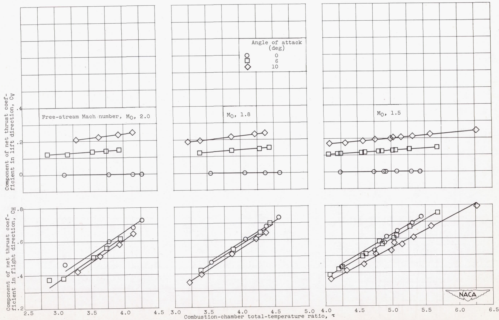
Figure 14. - Components of net thrust coefficients in flight and lift directions at angles of attack of 0^\circ , 6^\circ , and 10^\circ at Mach numbers 1.5, 1.8, and 2.0 for constant-area exhaust nozzle.
