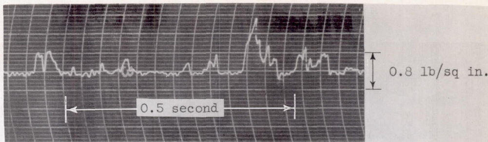
External cowl
