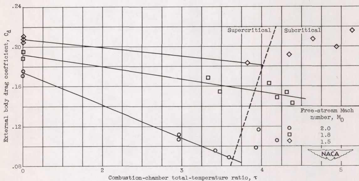
Figure 16. - Effect of burning on body drag coefficient for converging outlet nozzle at free-stream Mach numbers of 1.5, 1.8, and 2.0 and 0° angle of attack.
