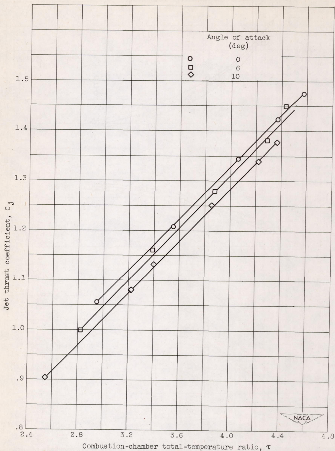
Figure 13. - Jet thrust coefficients obtained with constant-area outlet nozzle at Mach number of 1.8 and angles of attack of 0°, 6°, and 10°.
