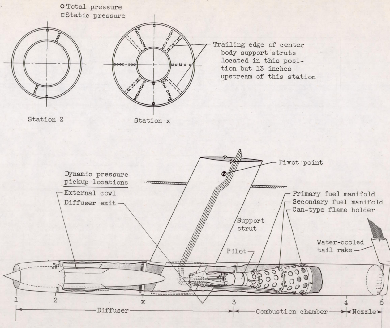
Figure 1. - Diagrammatic sketch of 16-inch ram jet.
