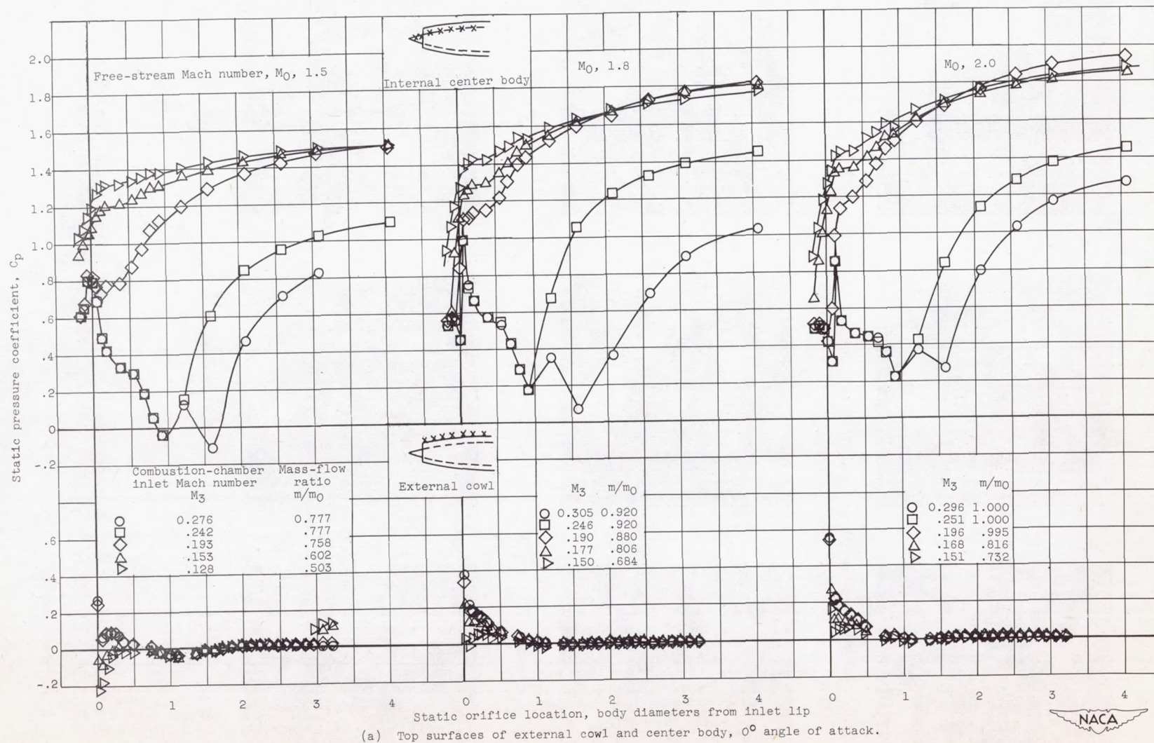
Figure 10. - Variation in static pressure coefficients along diffuser at free-stream Mach numbers of 1.5, 1.8, and 2.0.
