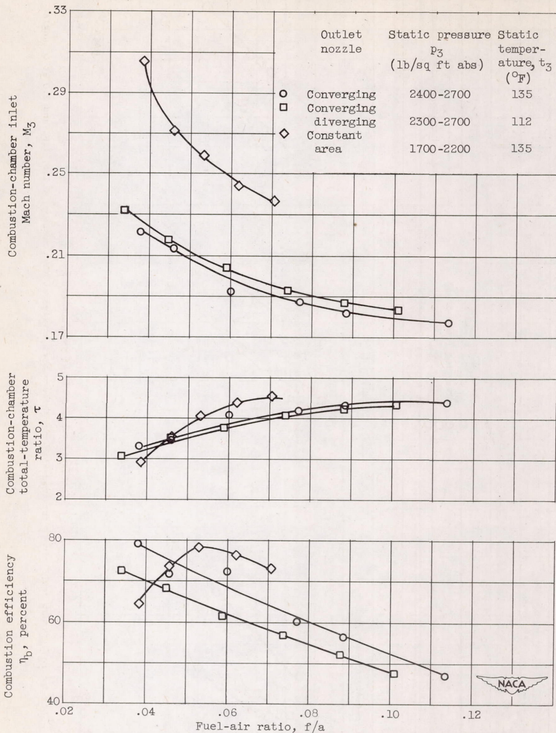
Figure 18. - Effect of outlet nozzle configuration on combustor performance at free-stream Mach number of 1.8 and 0^{\circ} angle of attack.
