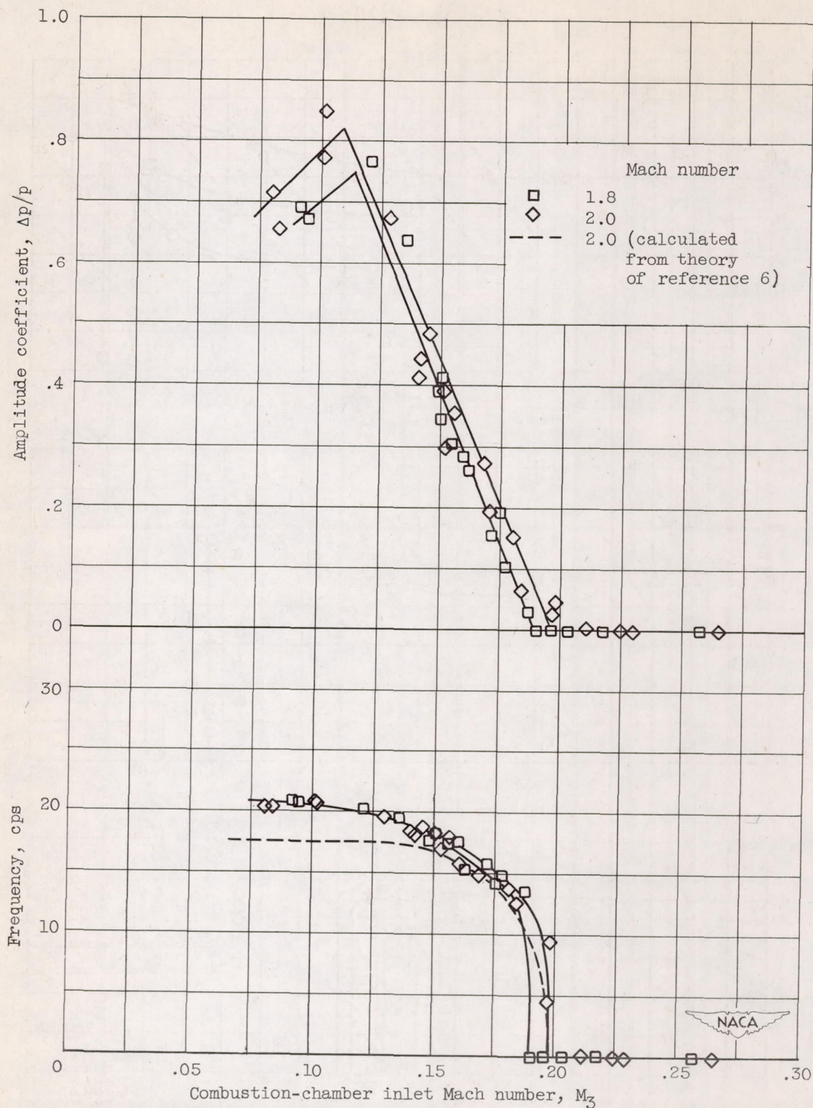
Figure 5. - Cold-flow static pressure fluctuation at diffuser exit; 0^\circ angle of attack.
