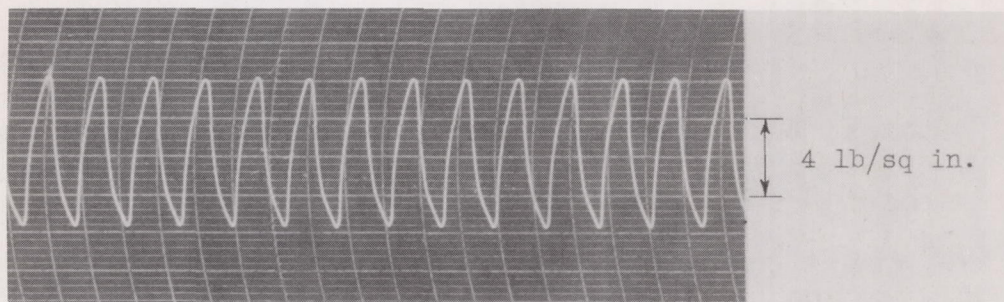
Diffuser exit
