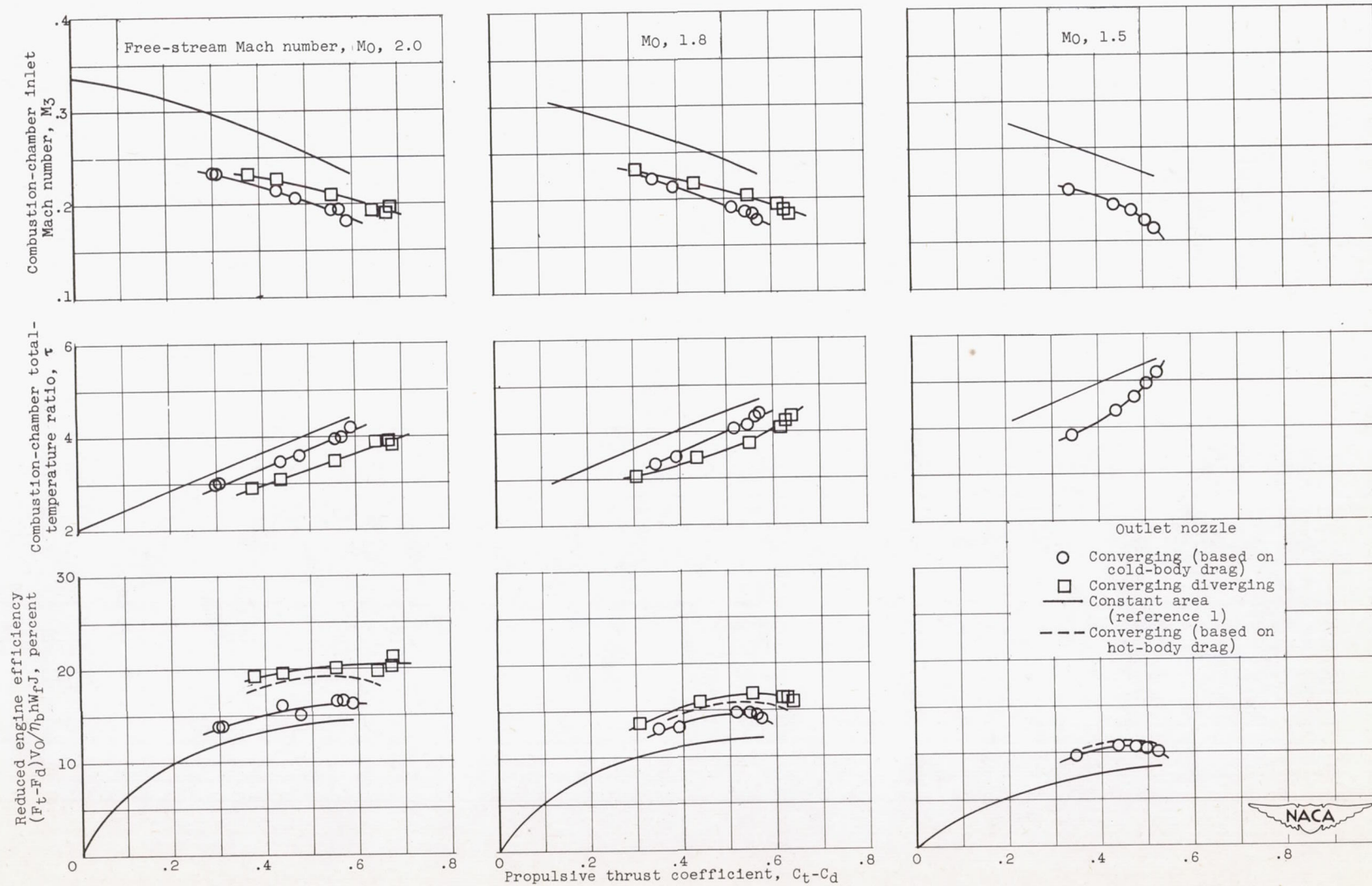
Figure 19. - Variation of reduced engine efficiency with propulsive thrust coefficient for the three outlet nozzles at Mach numbers of 1.5, 1.8, and 2.0 and 0^\circ angle of attack.
