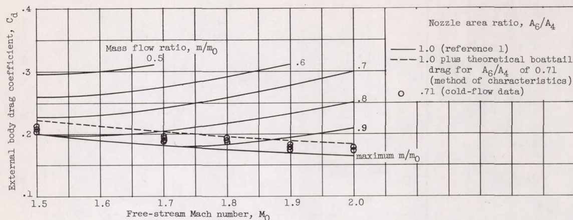
Figure 15. - Cold-flow engine body drag coefficients for 16-inch ram jet with constant area and converging exhaust nozzles.
