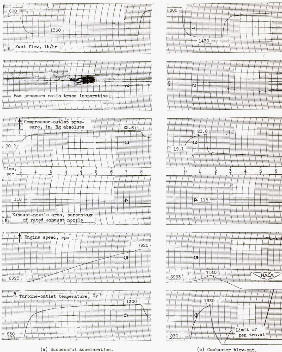
Figure 14. - Behavior of several engine variables during successful and unsuccessful accelerations which resulted from step increase in fuel flow. Altitude, 45,000 feet; flight Mach number, 0.19.
