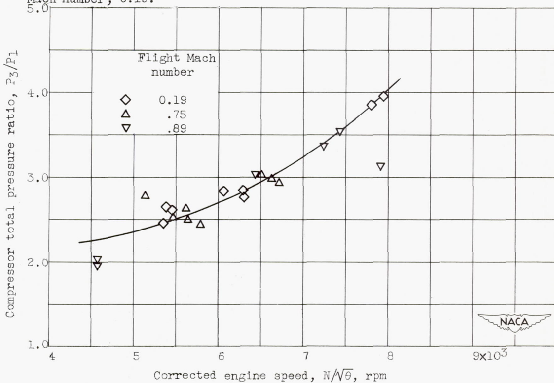
Figure 12. - Effect of flight Mach number on compressor uninstalled characteristics of J47D (RX1-3) engine. Altitude, 25,000 feet.
