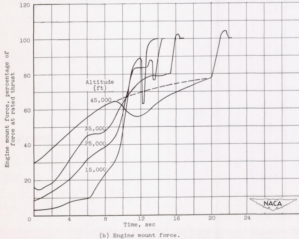
Figure 20. - Effect of altitude on variation of engine speed and engine mount force during thrust selector bursts from 10 to 90 degrees. Flight Mach number, 0.19.
