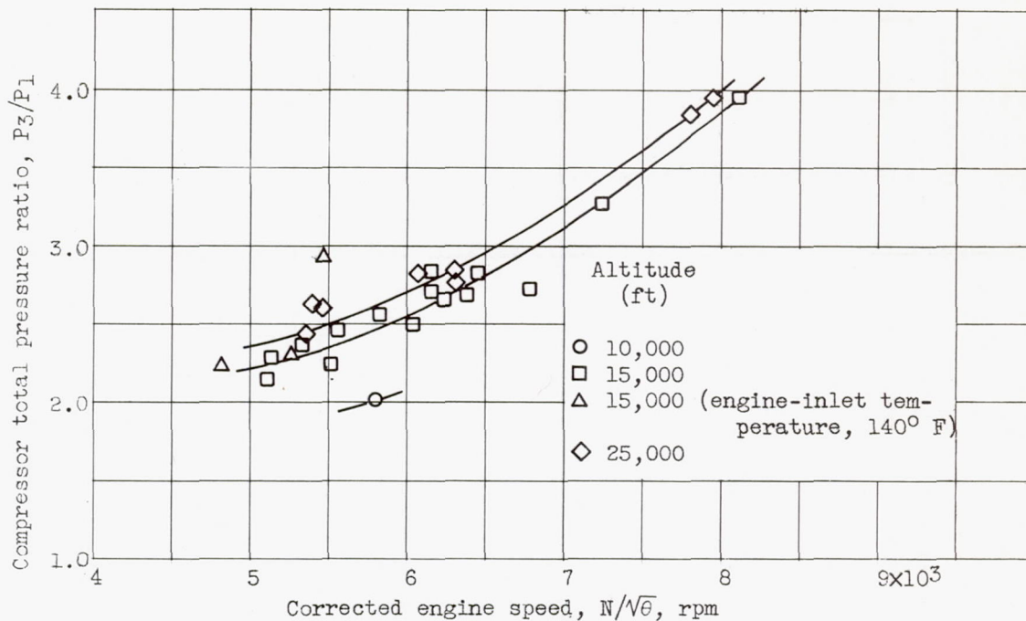
Figure 11. - Effect of altitude and engine-inlet temperature on compressor uninstalled characteristics of J47D (RX1-3) engine. Flight Mach number, 0.19.
