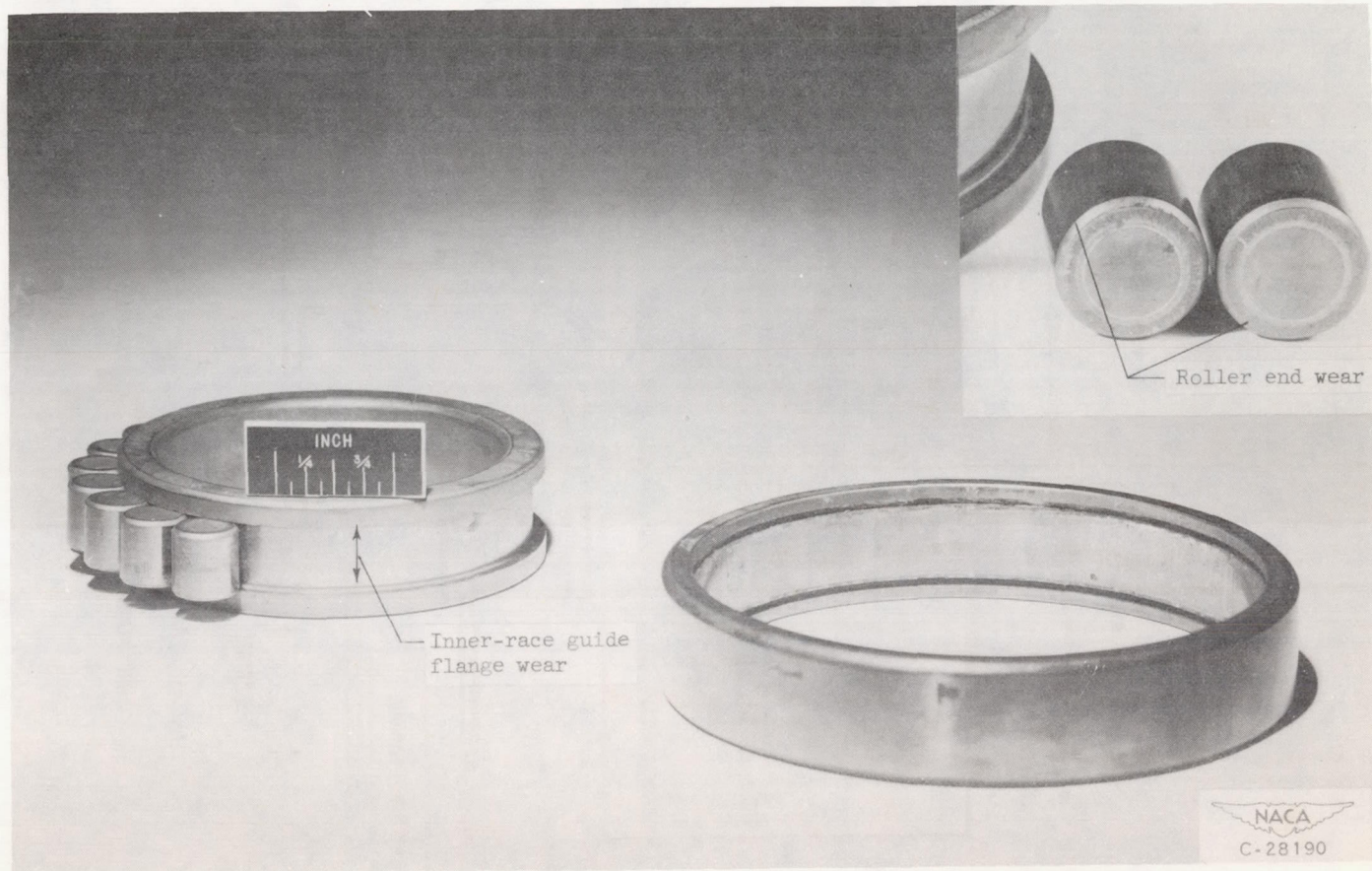
(b) Bearing 13.
