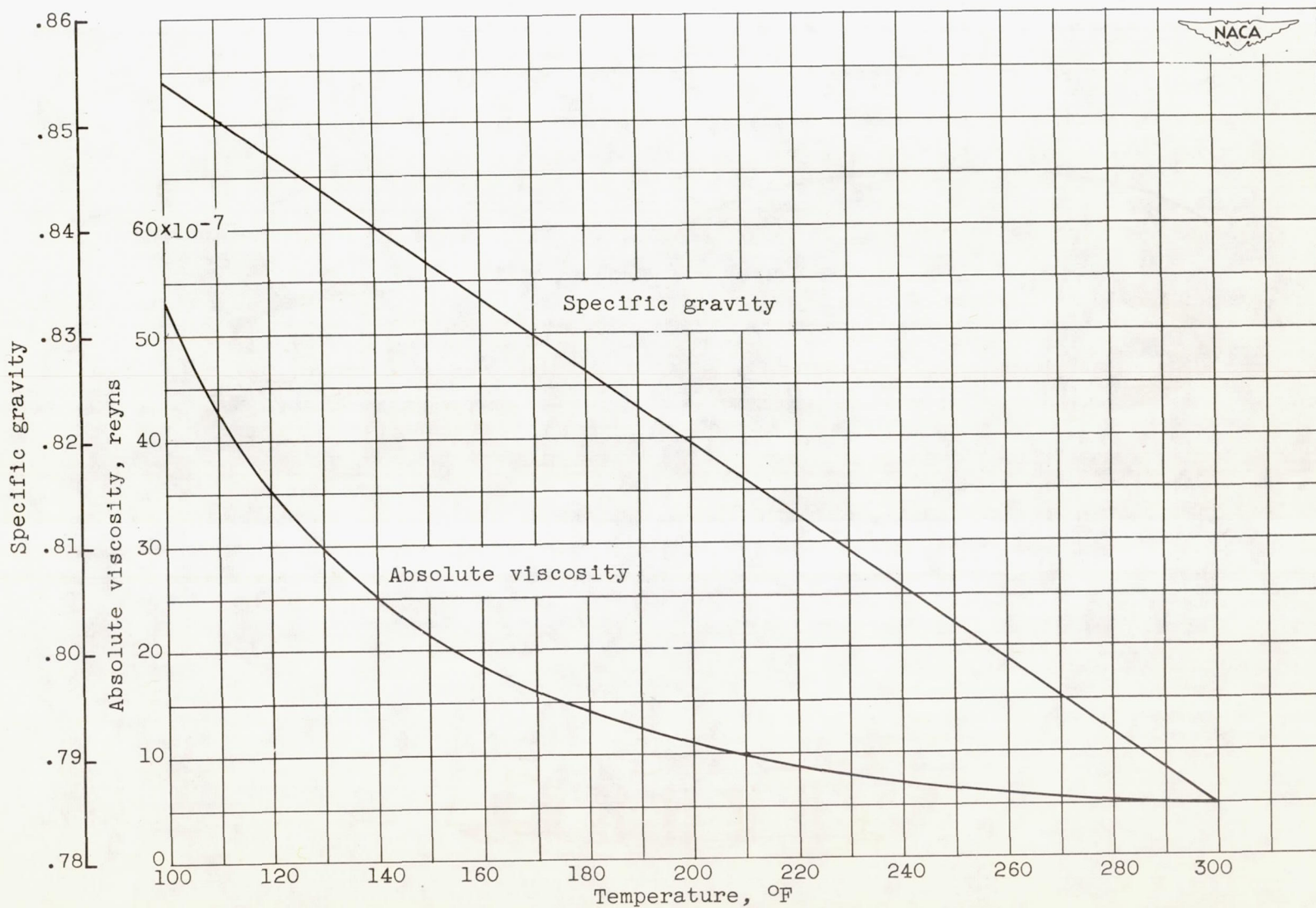
Figure 6. - Absolute viscosity and specific gravity of lubricant. Pour point, -50^{\circ} F; flash point, 310^{\circ} F; viscosity index, 150.
