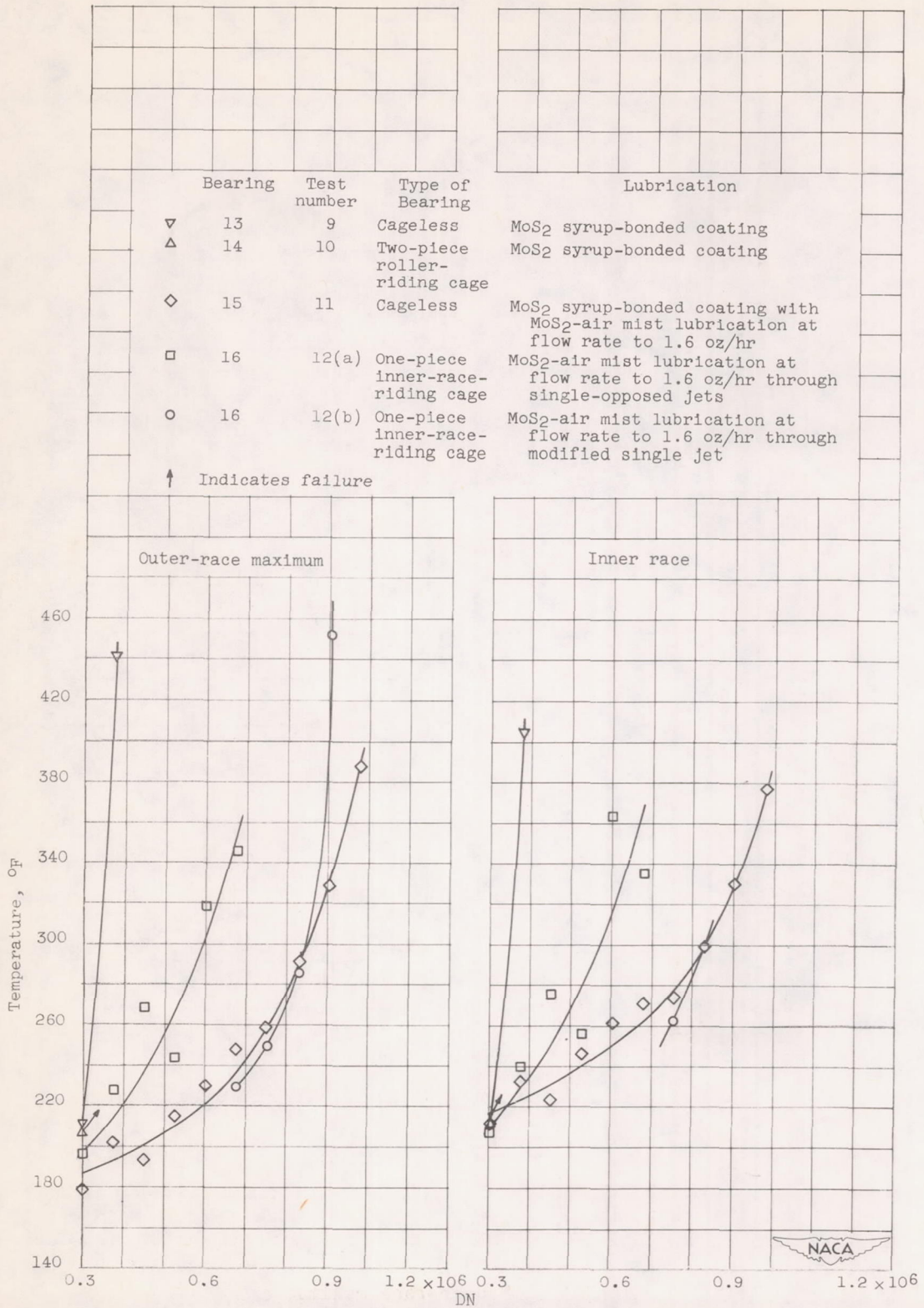
Figure 8. - Effect of DN on outer-race-maximum and inner-race temperatures of bearings 13, 14, 15, and 16 (all with shaft seal). DN, 0.3 \times 10^6 to 0.975 \times 10^6 ; load; 368 pounds.
