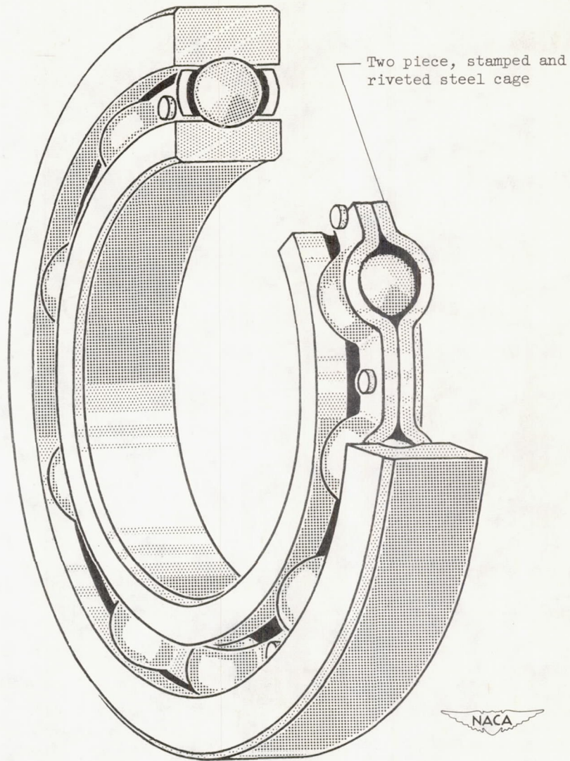
Figure 2. - High-temperature-rig test bearing.
