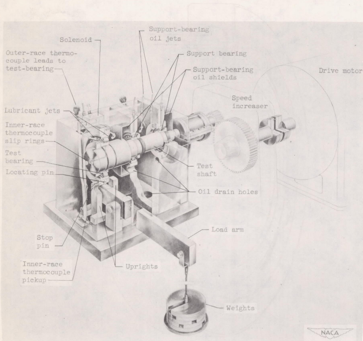
Figure 3. - Cutaway view of high-speed bearing rig.
