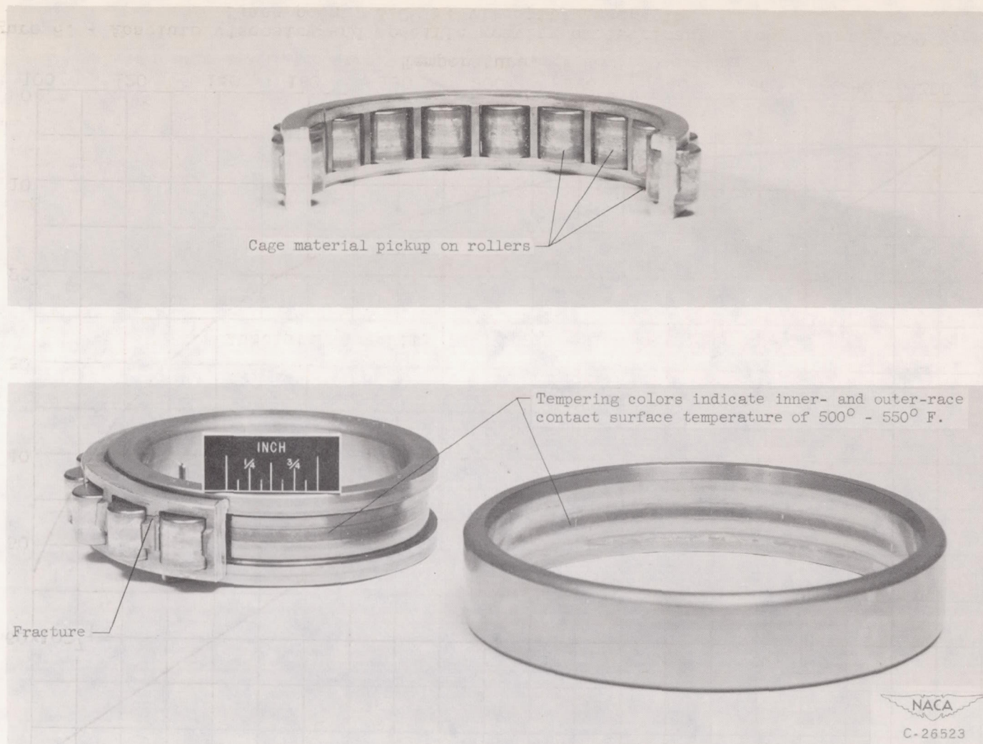
(a) Bearing 10.
