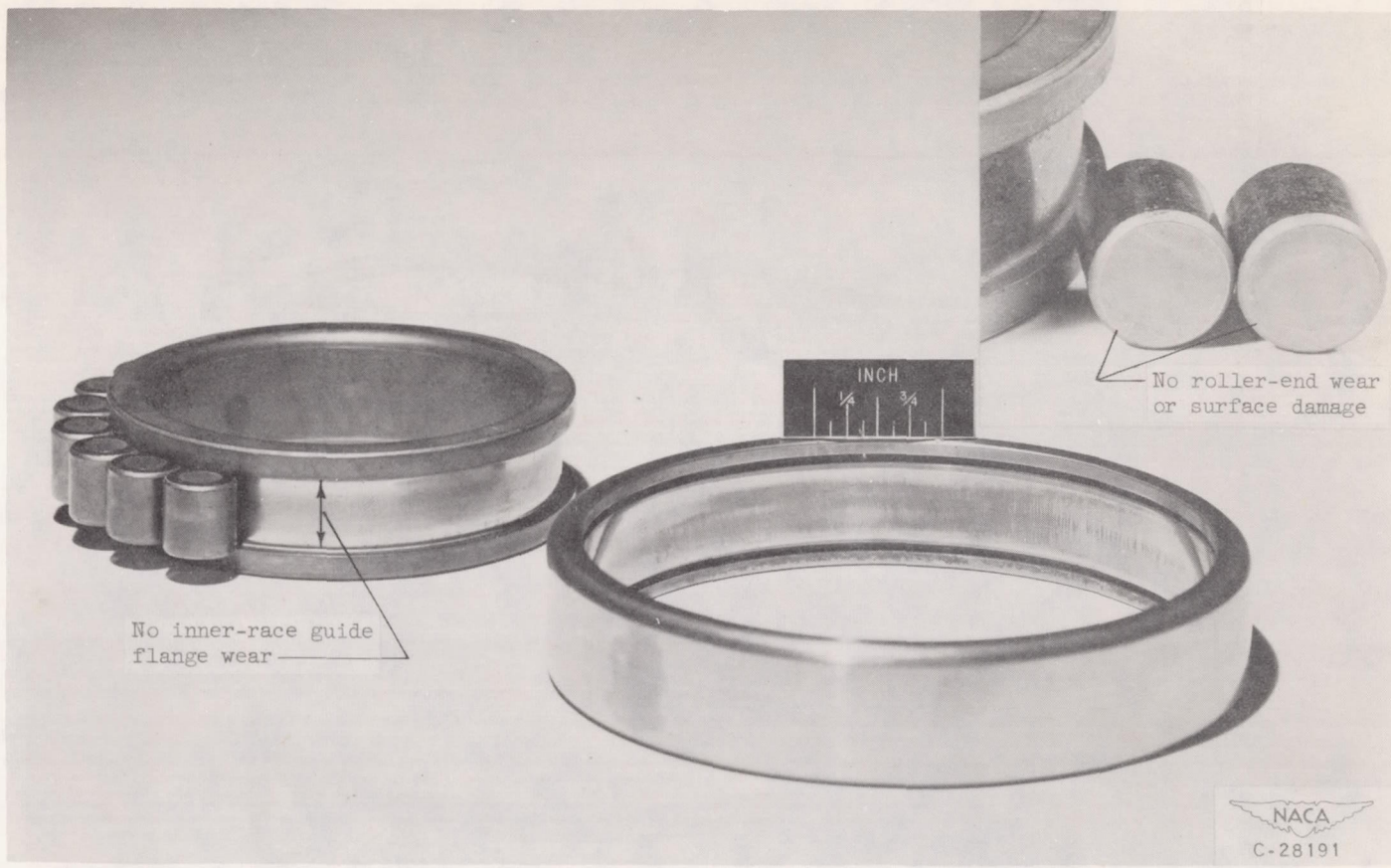
(c) Bearing 15.
