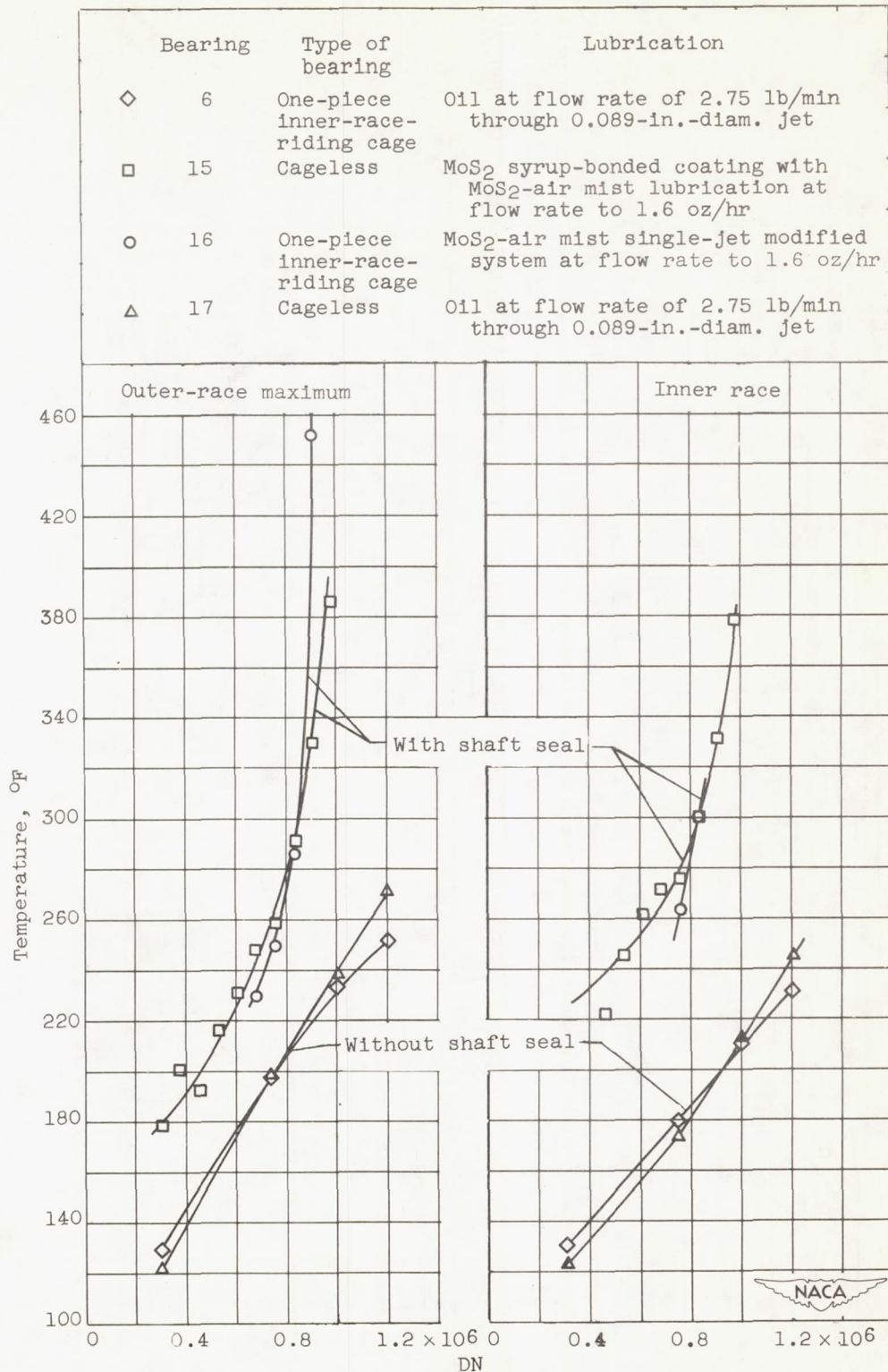
Figure 9. - Effect of DN on outer-race-maximum and inner-race temperatures of bearings 6 (reference 4), 15, 16, and 17. DN, 0.3 \times 10^6 to 1.2 \times 10^6 ; load, 368 pounds.
