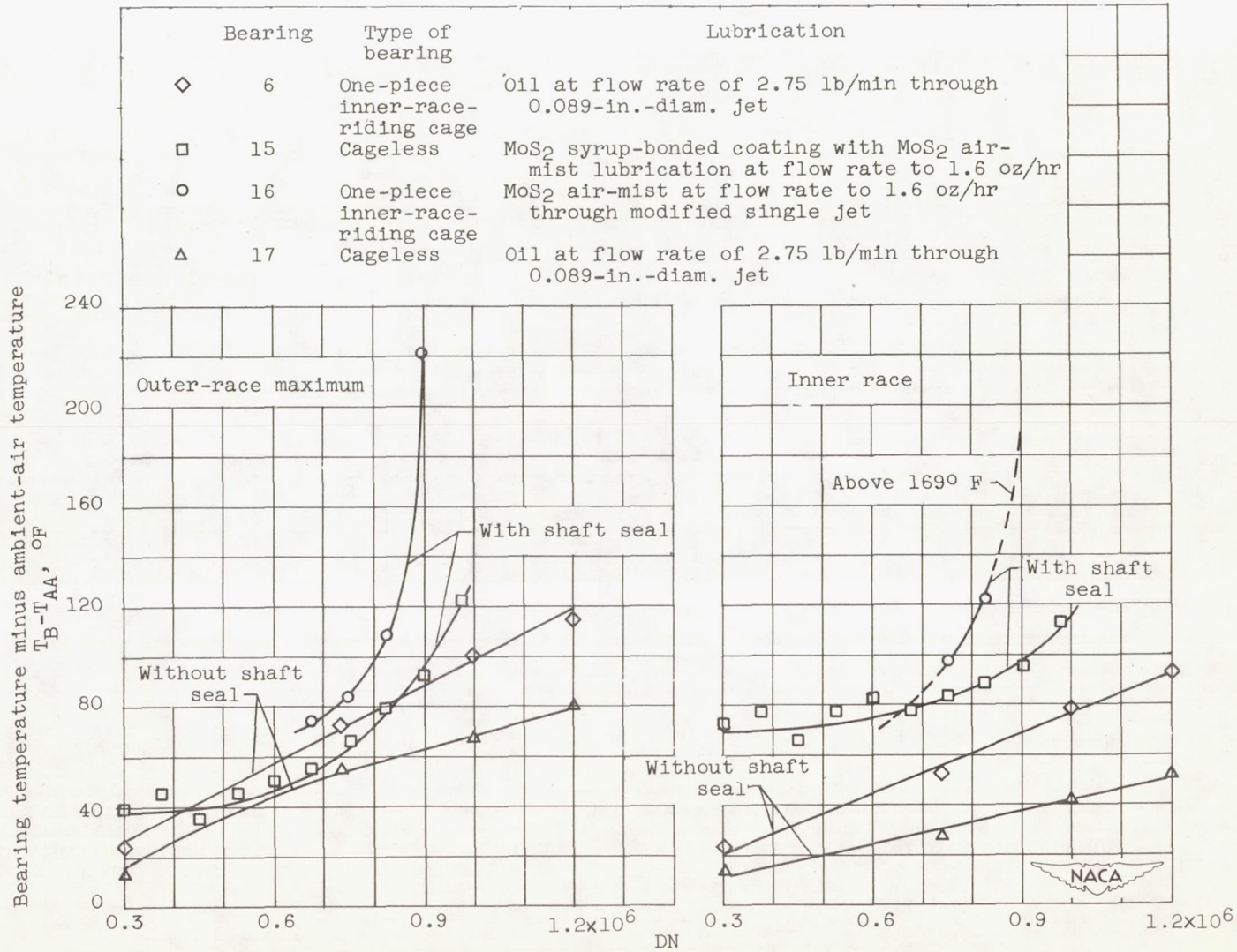
Figure 11. - Effect of DN on outer-race-maximum and inner-race temperatures above ambient-air temperatures for bearings 6, 15, 16, and 17. DN, 0.3 \times 10^6 to 1.2 \times 10^6 ; load, 368 pounds.
