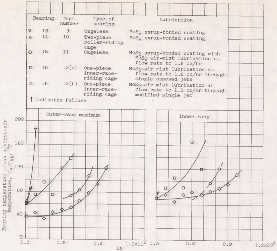
Figure 10. - Effect of DN on outer-race-maximum and inner-race temperatures above ambient-air temperatures for bearings 13, 14, 15, and 16 (with shaft seal). DN, 0.3 \times 10^6 to 0.975 \times 10^6 ; load, 368 pounds.
