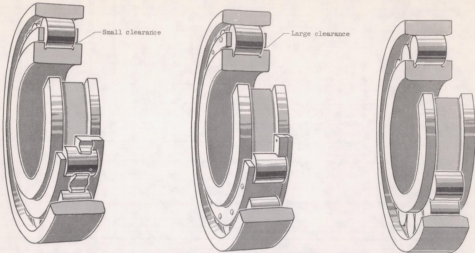
(a) One-piece inner-race-riding cage.
