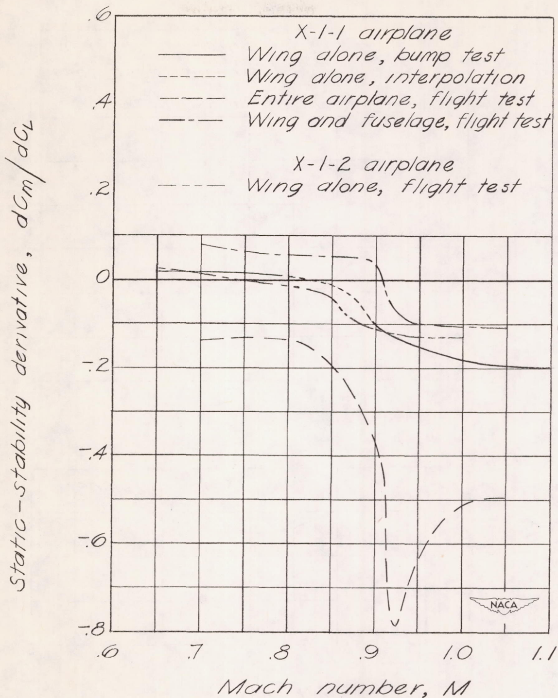
Figure 3.- Variation of the static-stability derivative with Mach number for portions of the X-1 airplanes. C_L = 0.3 ; center of gravity at 23.5 percent mean aerodynamic chord.
