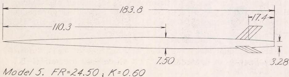
Figure 1.- General arrangements of test models. All dimensions are in inches.
