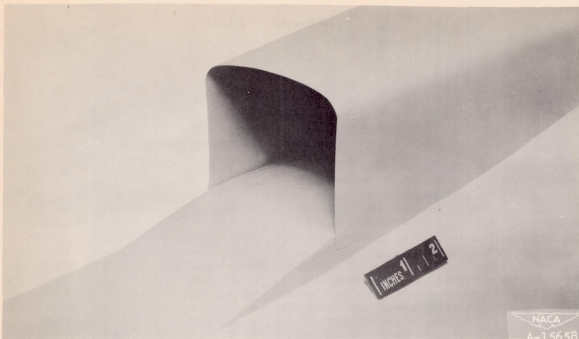
(a) Sharp lip (supersonic type).
