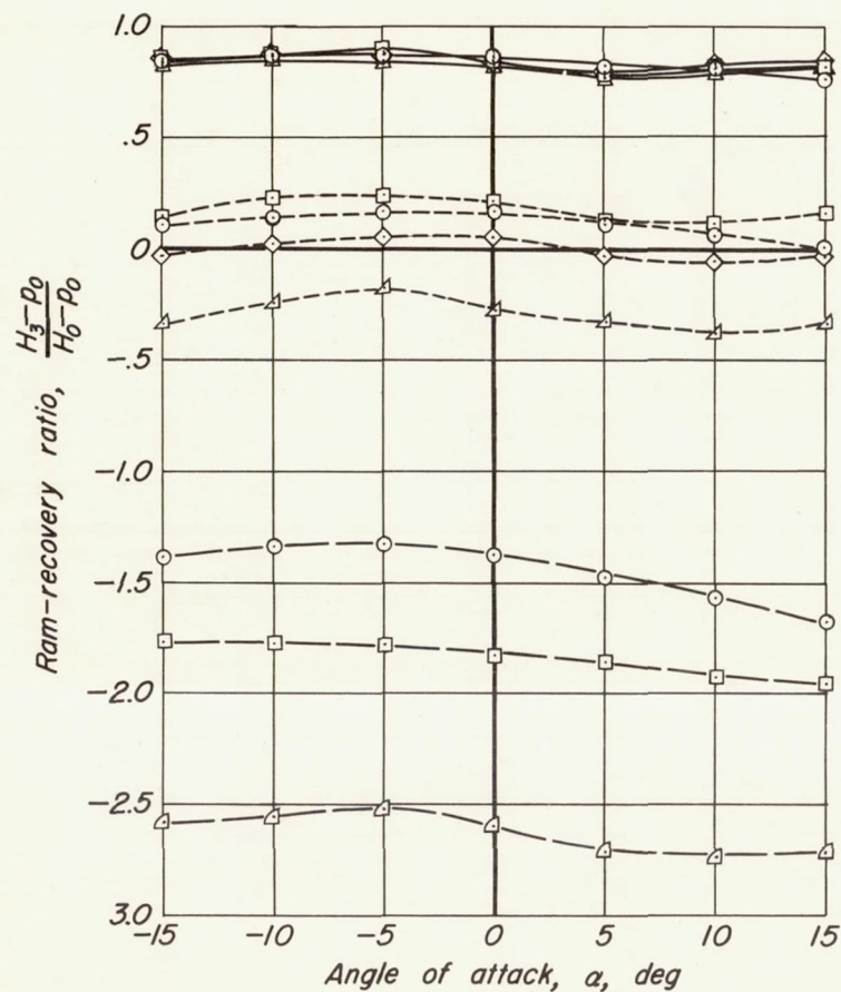
(a) Sharp lip.
