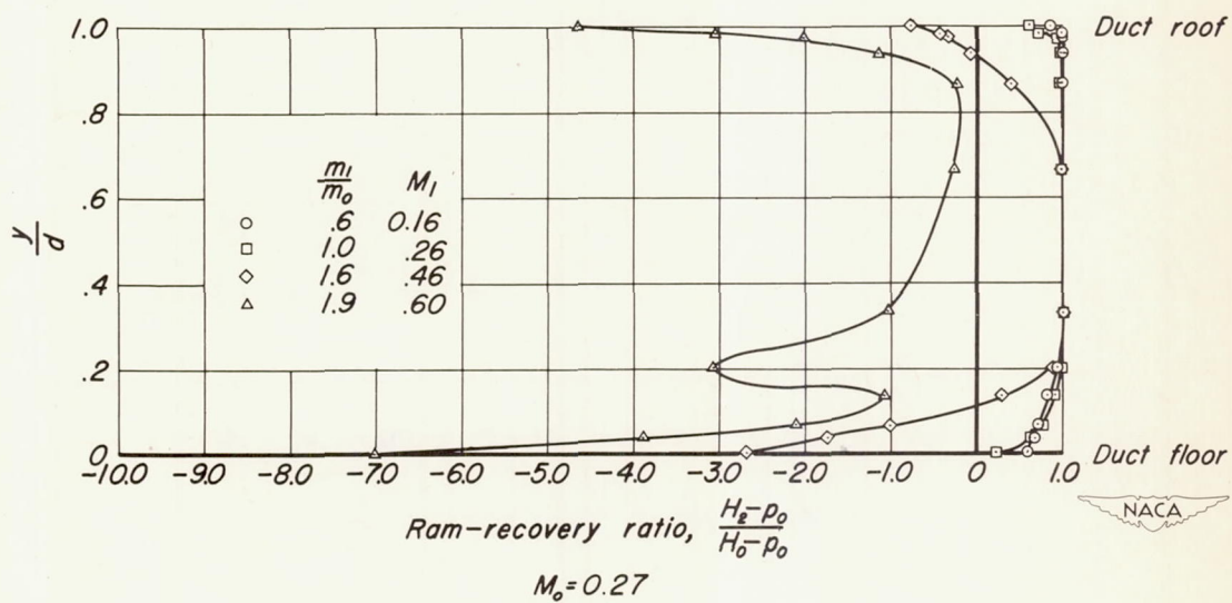
Figure 12.— Distribution of the ram-recovery ratio in the plane of symmetry of the minimum-area station for the intake with the sharp lip. \alpha = 0^\circ
