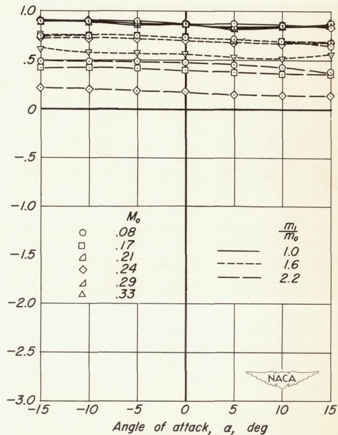
(b) Rounded lip.
