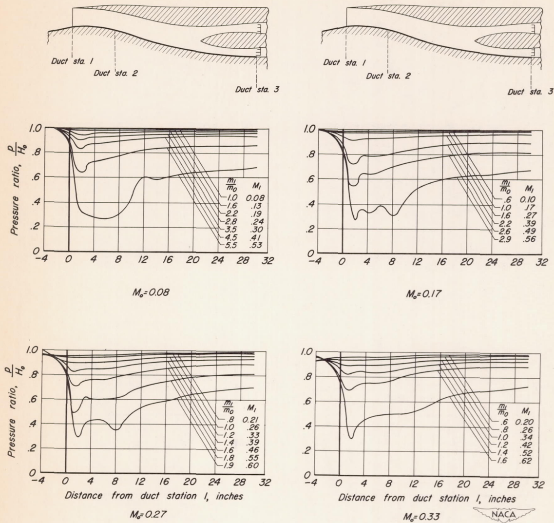
(a) Duct floor.
