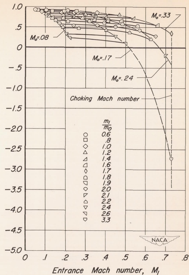
(b) Rounded lip.
