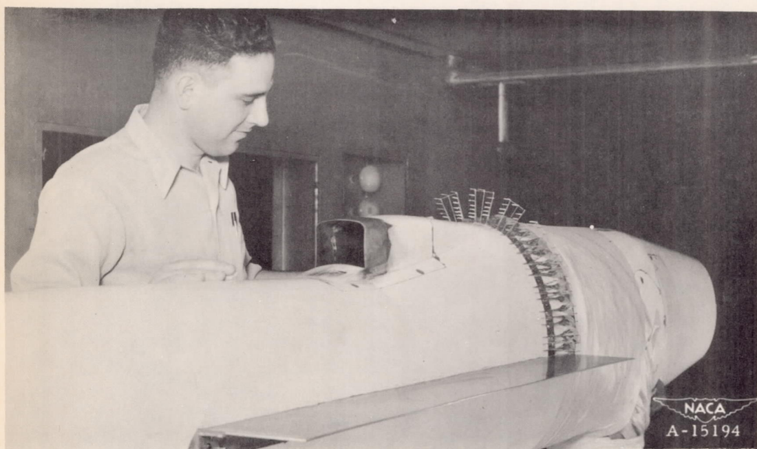
(a) The array of rakes used to measure drag.
