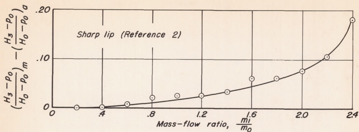
(a) Effect of mass-flow ratio. M_0 = 0.17 .
