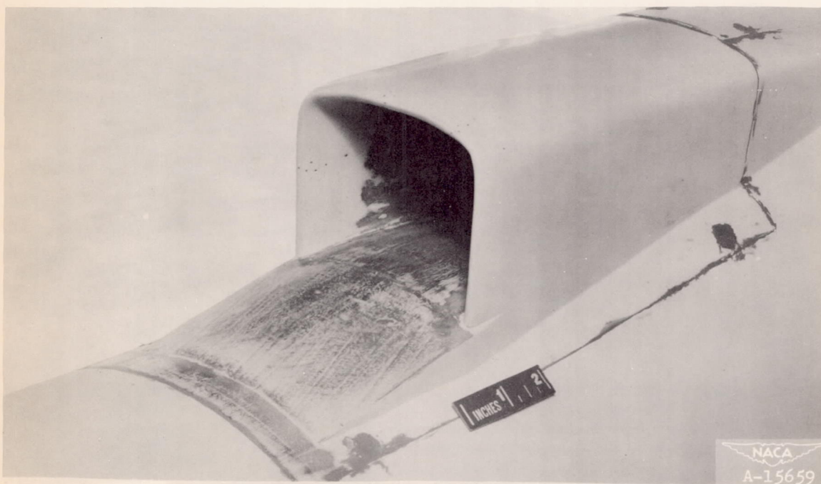
(b) Thick, rounded lip (subsonic type).
