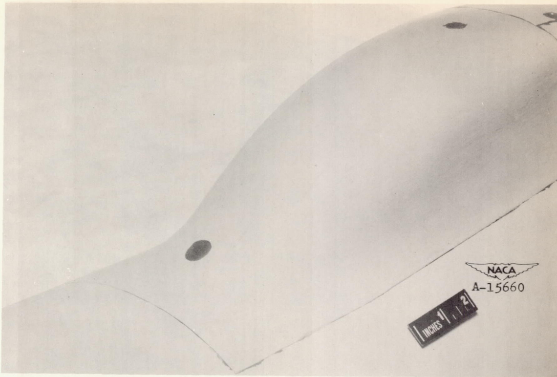
Figure 6.- The intake faired and sealed to form the faired fuselage.
