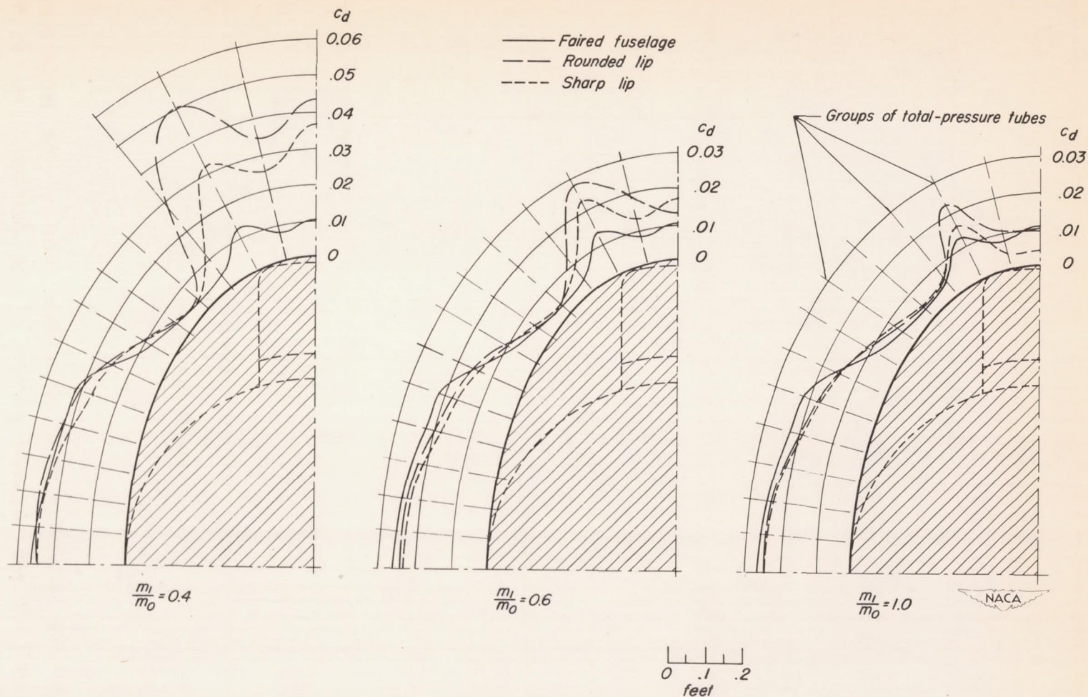
Figure 19.—Distribution of section wake drag coefficients at fuselage station 82 for three configurations. \alpha = 0^\circ , M_0 = 0.24 .
