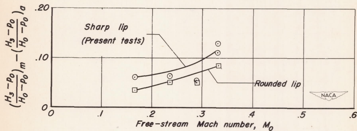
(b) Effect of Mach number. \frac{m_1}{m_0} = 1.6 .
