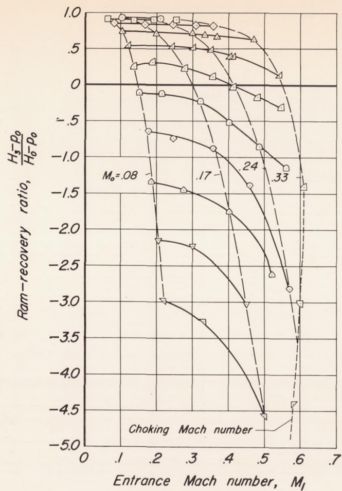
(a) Sharp lip.
