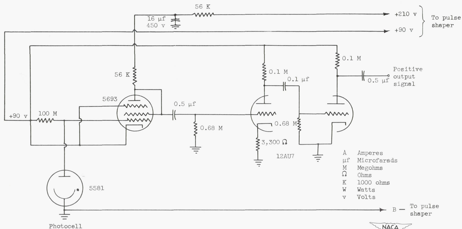
(b) Flame detector.
