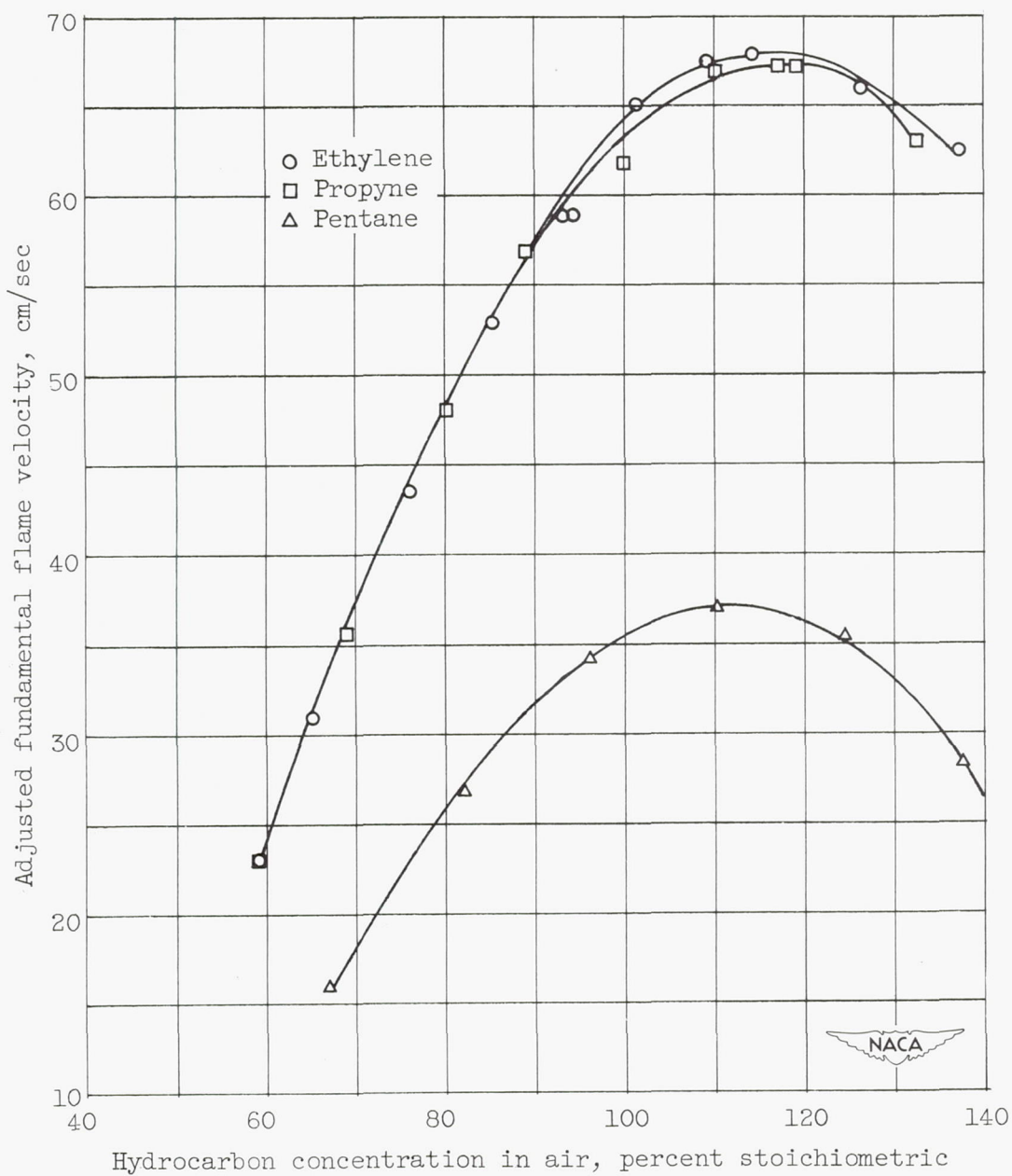
Figure 7. - Fundamental flame velocity.
