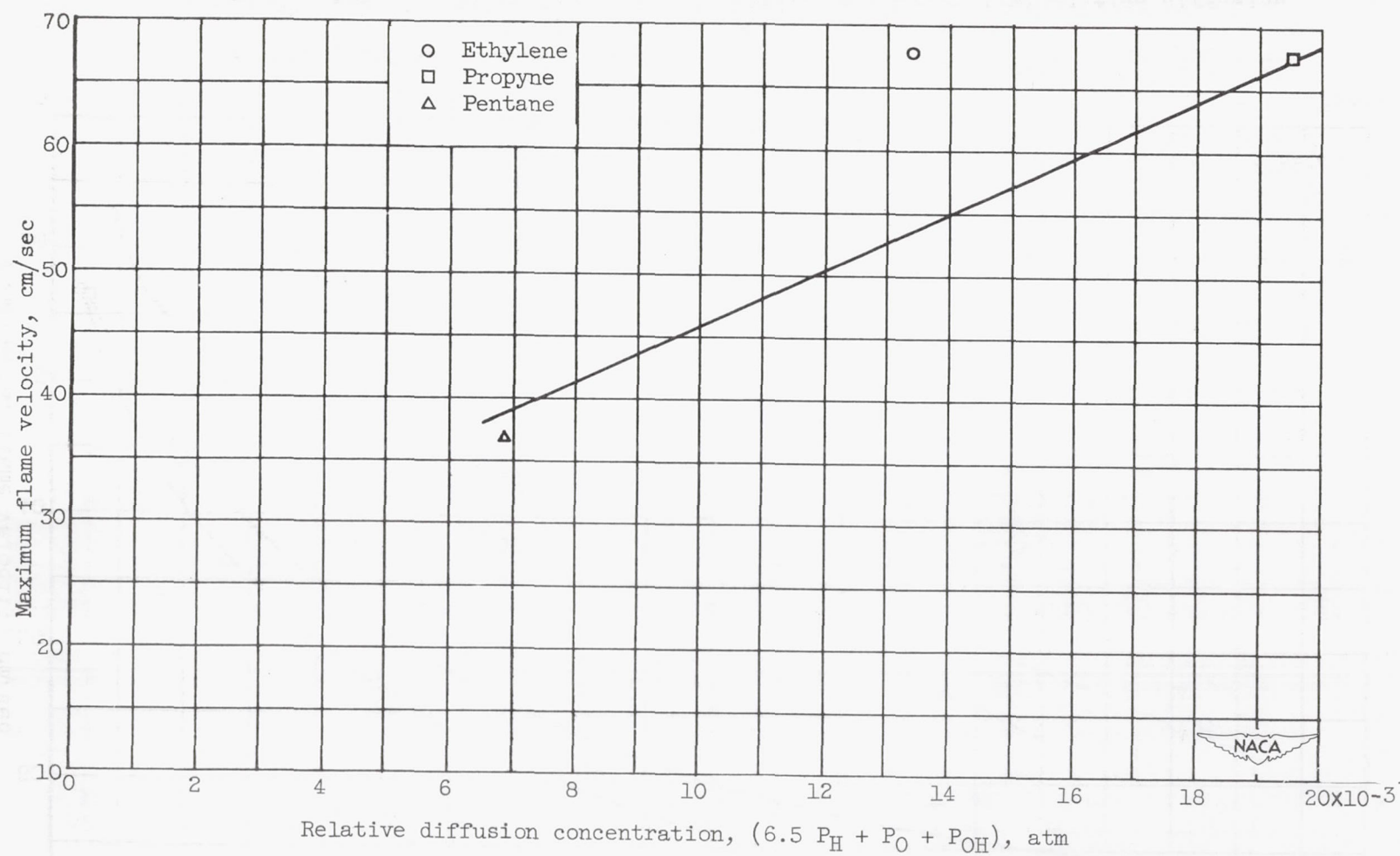
Figure 11. - Correlation for 52 hydrocarbons at maximum flame velocity (reference 2).
