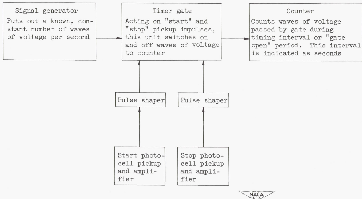
(a) Photoelectric timer.
