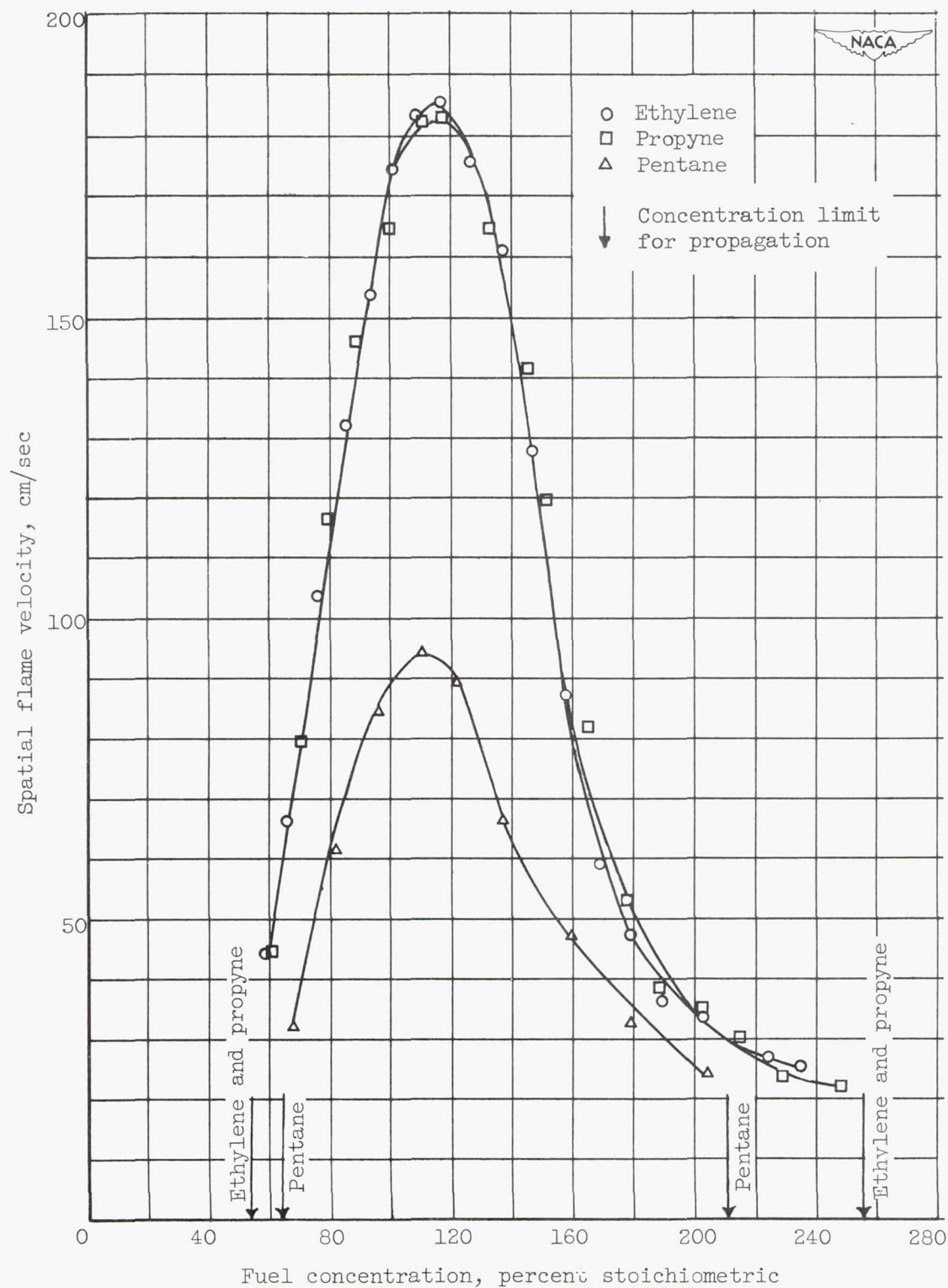
Figure 2. - Change in spatial flame velocity with mixture concentration.
