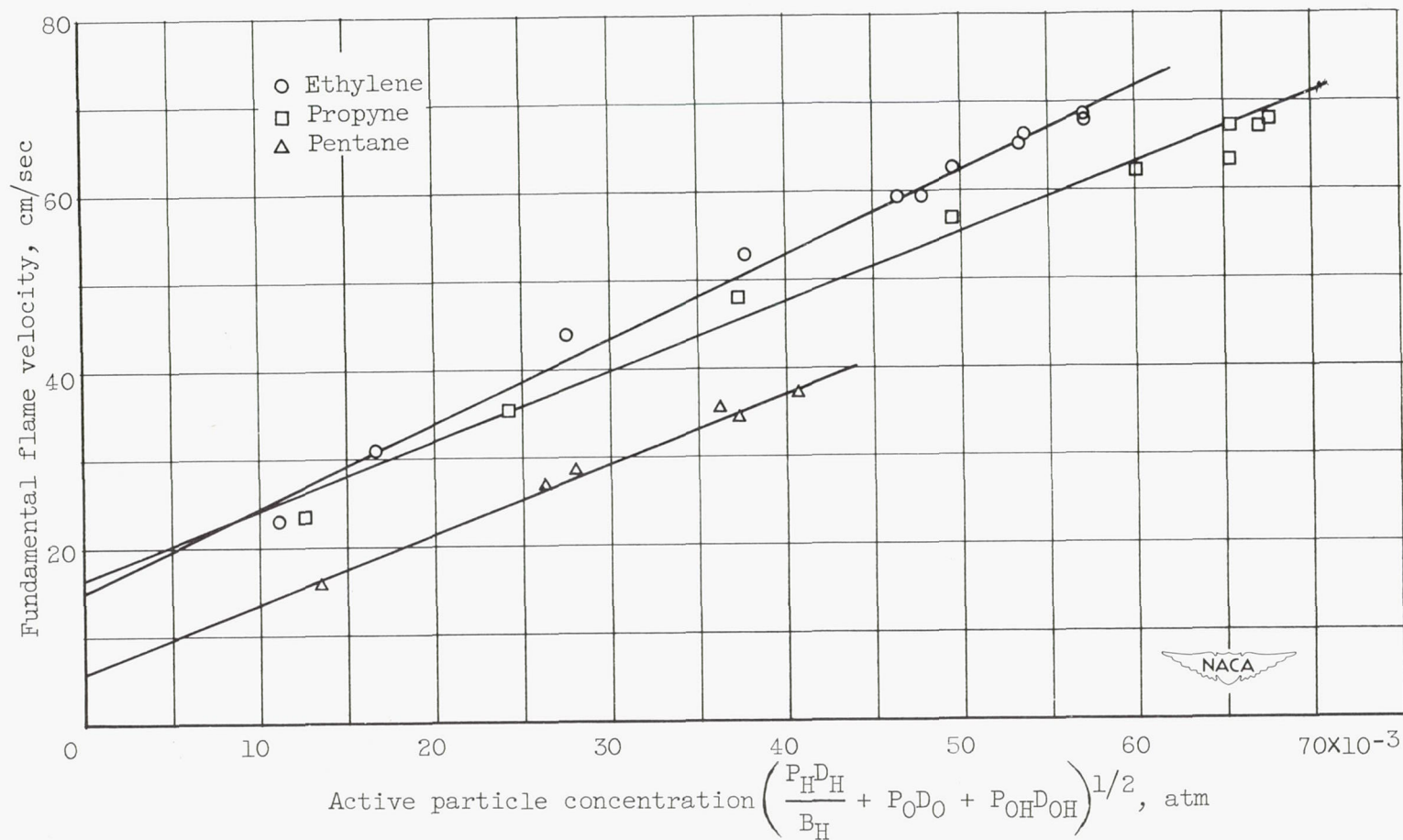
Figure 12. - Variation of flame velocity with square root of diffusion concentration of active particles.
