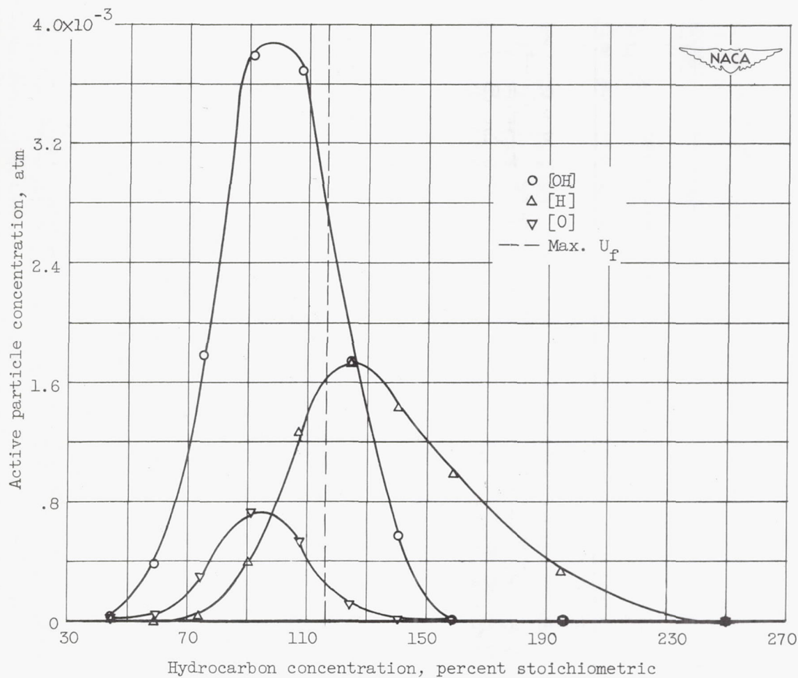
Figure 9. - Continued. Calculated active particle concentrations.
