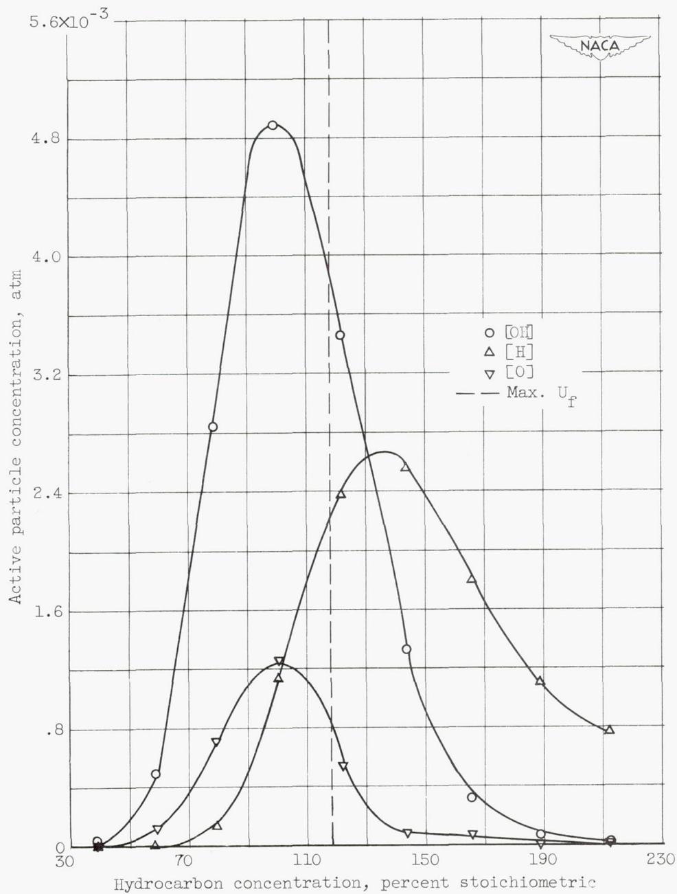
Figure 9. - Continued. Calculated active particle concentrations.
