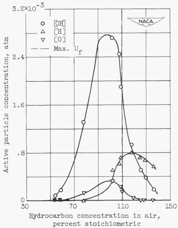
Figure 9. - Calculated active particle concentrations.
