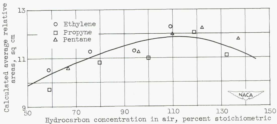
Figure 5. - Change in surface area with composition.
