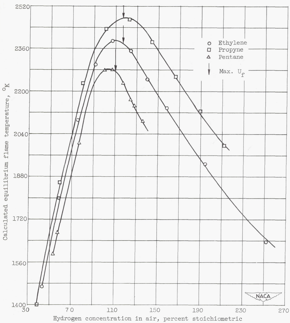
Figure 8. - Calculated equilibrium flame temperatures.
