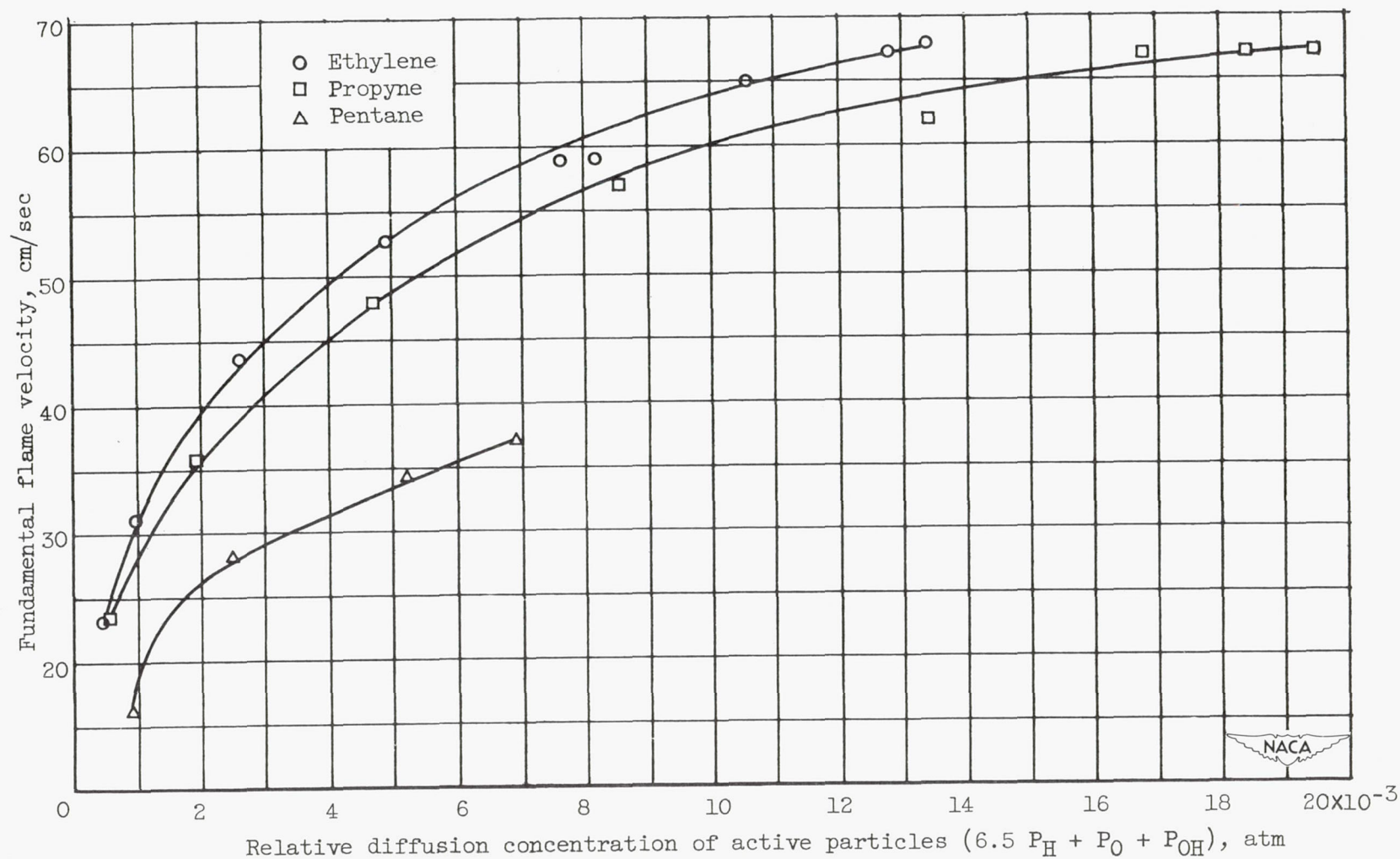
Figure 10. - Variation of fundamental flame velocity with relative diffusion concentration of active particles.
