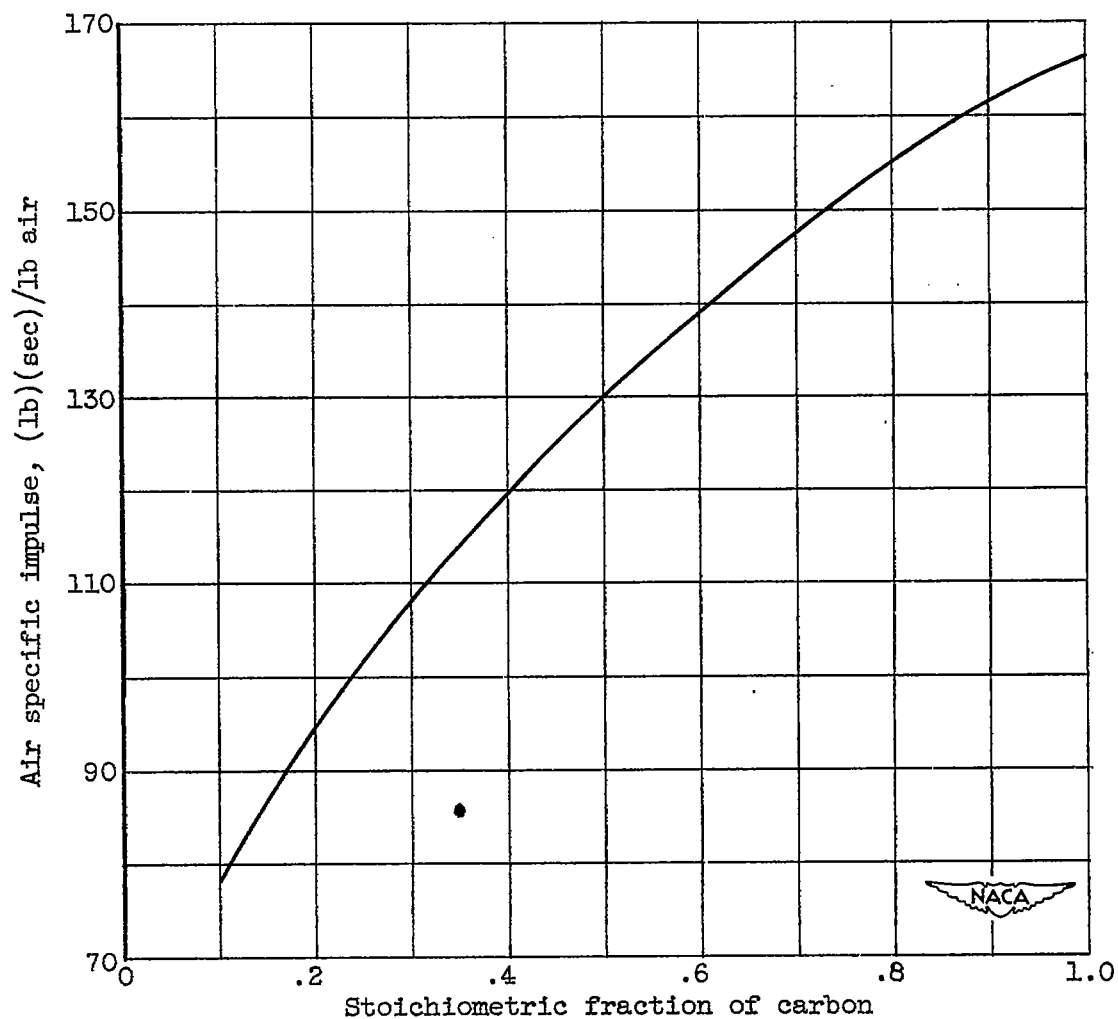
Figure 2. - Concluded. Variation of air specific impulse with stoichiometric fraction of fuel. Combustor inlet-air temperature, 560° R; inlet-air pressure, 2 atmospheres.
