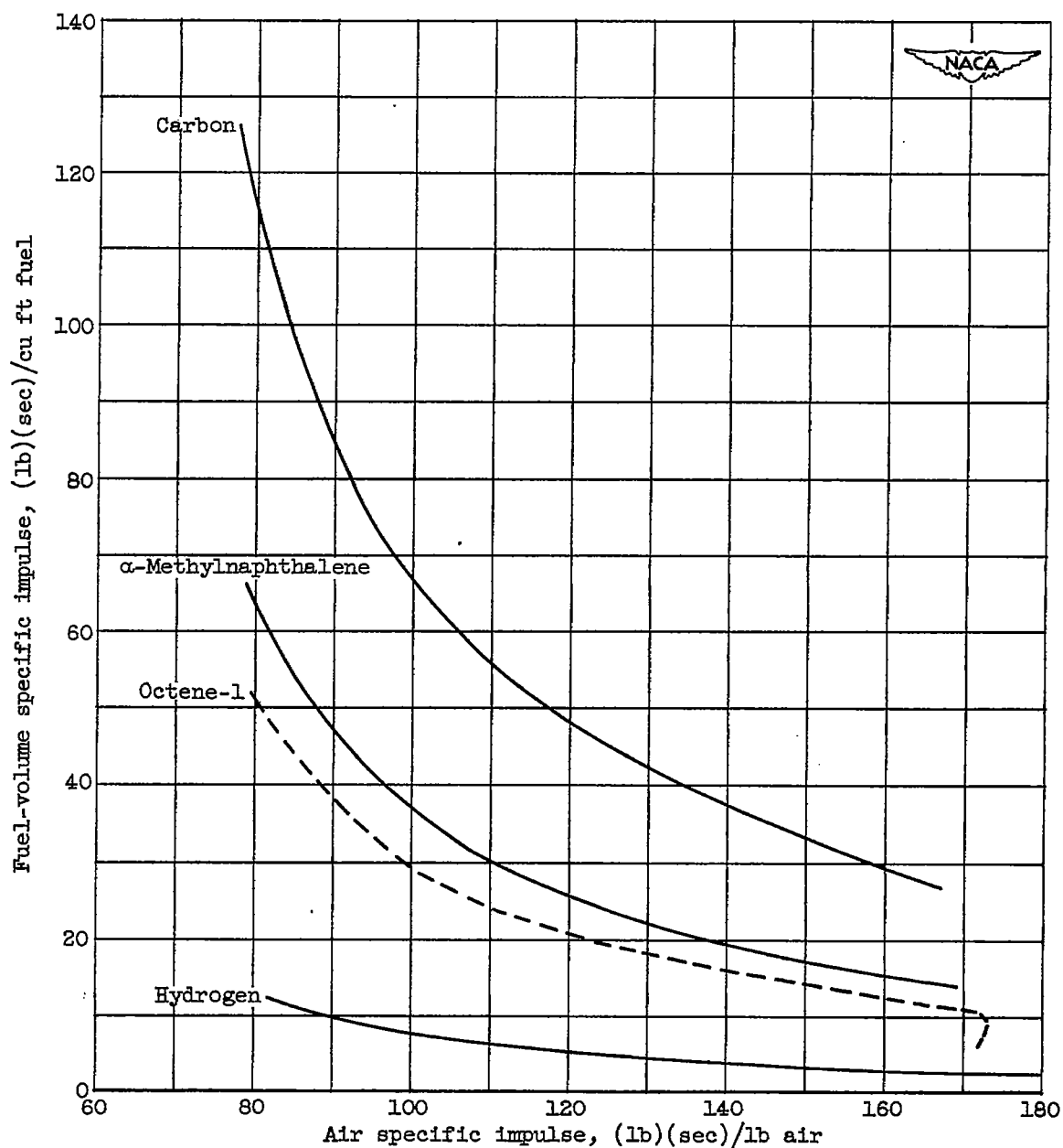
Figure 6. - Comparison of air and fuel-volume specific-impulse characteristics of hydrogen, α-methylnaphthalene, and graphite carbon with octene-1.
