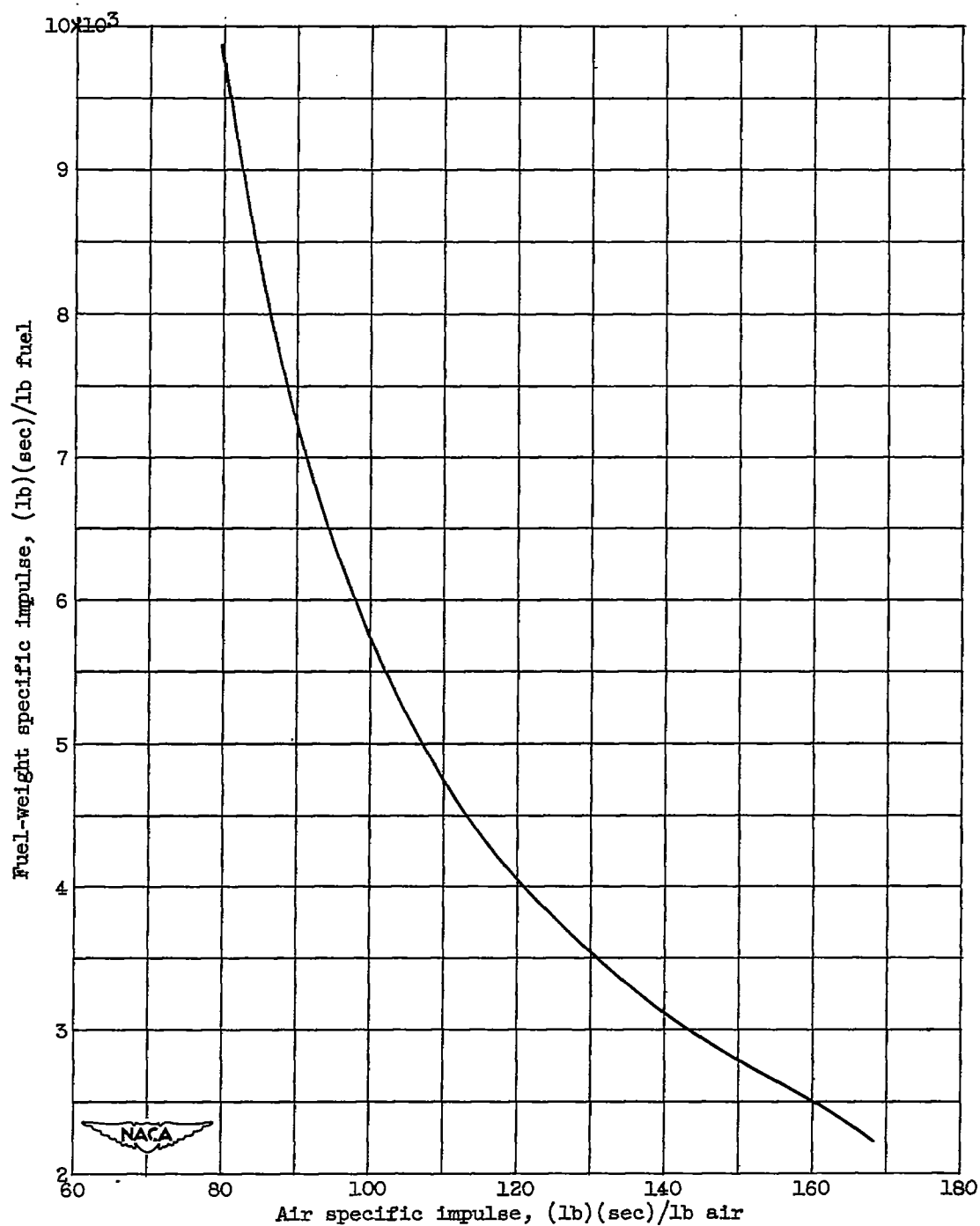
Figure 4. - Continued. Variation of fuel-weight specific impulse with air specific impulse for several fuels. Combustor inlet-air temperature, 560^\circ \text{R} ; inlet-air pressure, 2 atmospheres.
