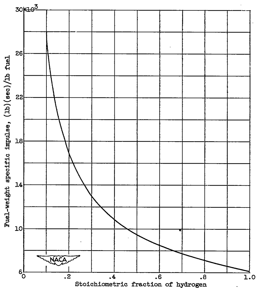
(a) Hydrogen.
