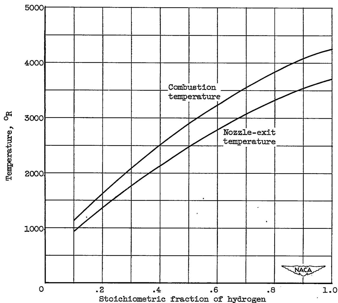
(a) Hydrogen.
