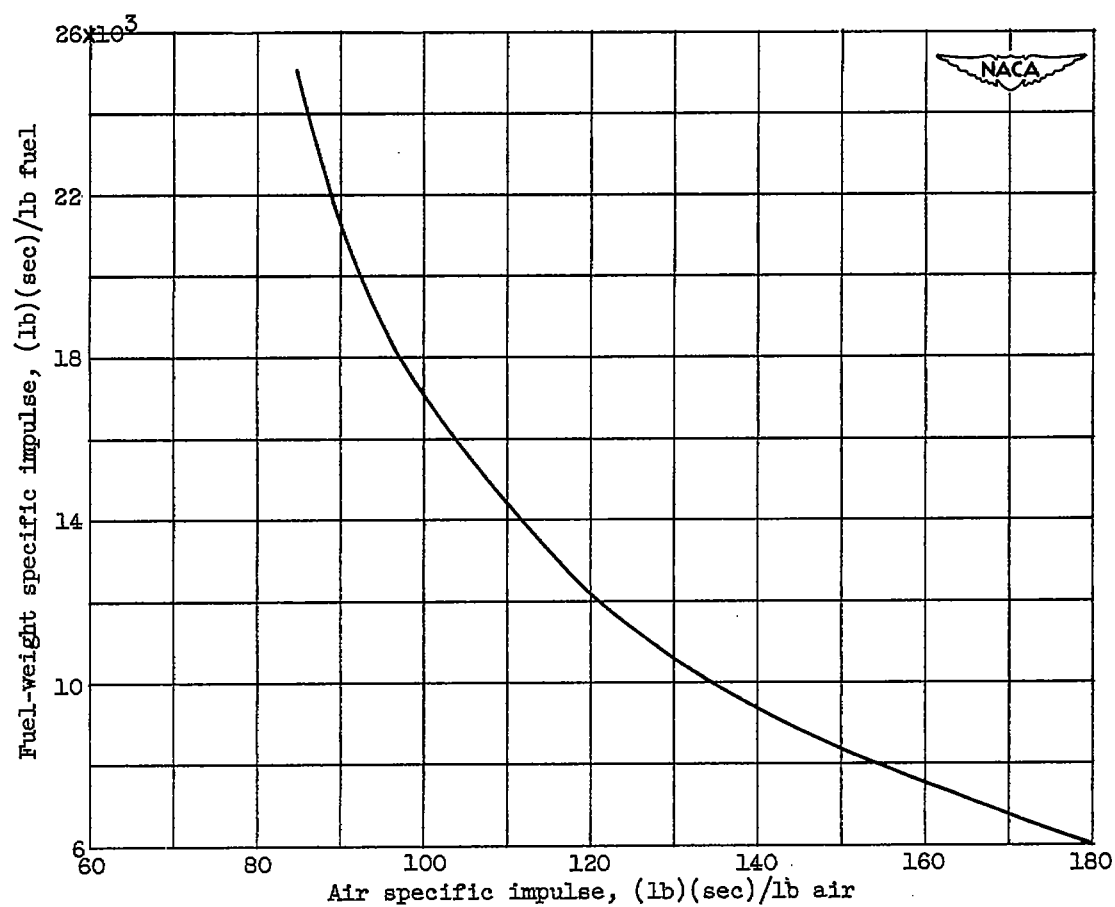
Figure 4. - Variation of fuel-weight specific impulse with air specific impulse for several fuels. Combustor inlet-air temperature, 560^\circ \text{R} ; inlet-air pressure, 2 atmospheres.
