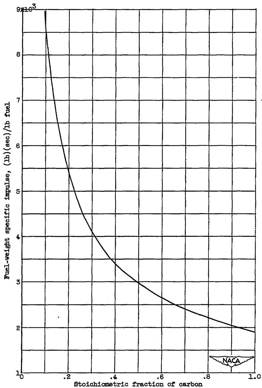
Figure 3. - Concluded. Variation of fuel-weight specific impulse with stoichiometric fraction of fuel. Combustor inlet-air temperature, 560^\circ \text{R} ; inlet-air pressure, 2 atmospheres.
