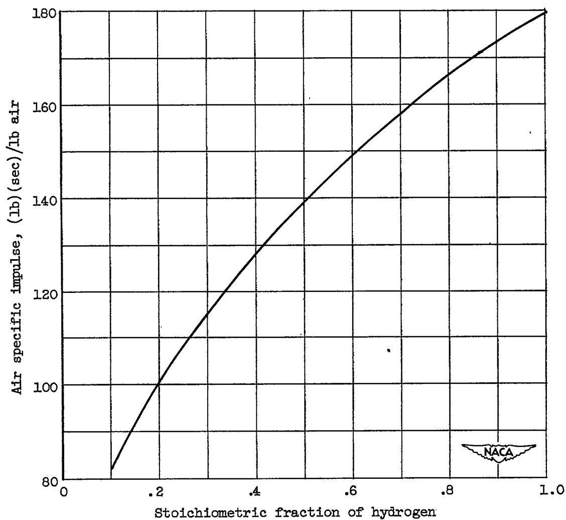
Figure 2. - Variation of air specific impulse with stoichiometric fraction of fuel. Combustor inlet-air temperature, 560° R; inlet-air pressure, 2 atmospheres.
