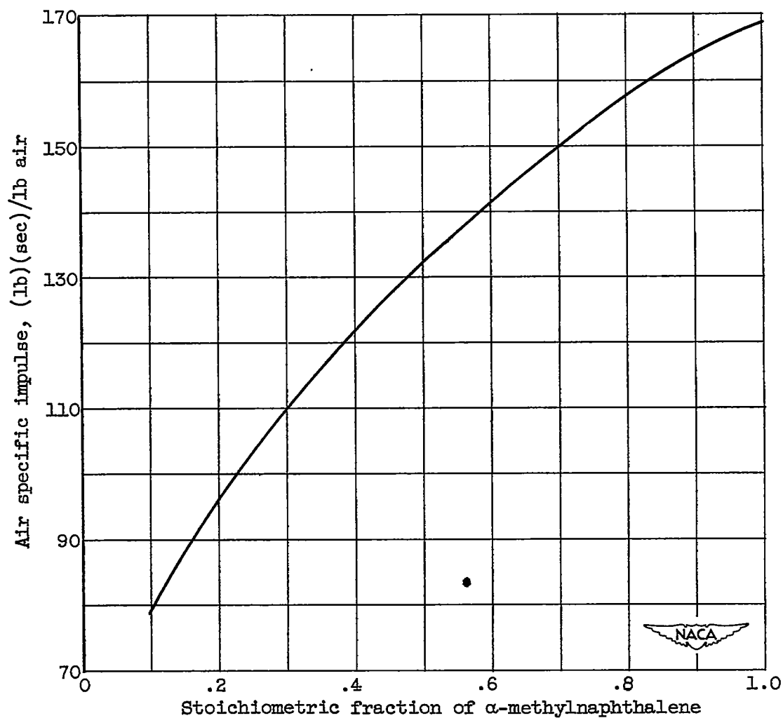
(b) α-Methylnaphthalene.
