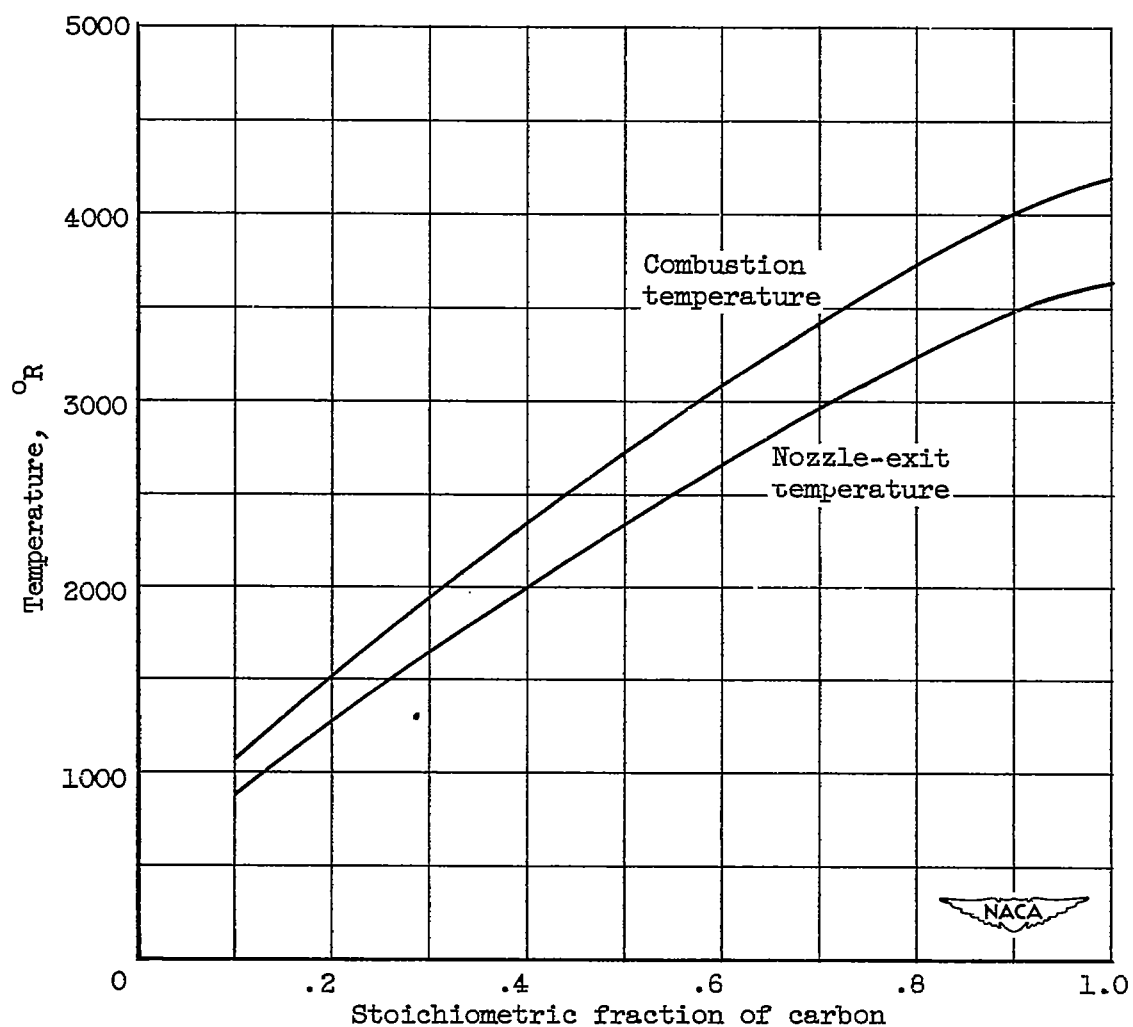
Figure 1. - Concluded. Theoretical variation of combustion and nozzle-exit temperature with stoichiometric fraction of fuel. Combustor inlet-air temperature, 560^{\circ}\text{R} ; inlet-air pressure, 2 atmospheres; expansion ratio, 2.0.
