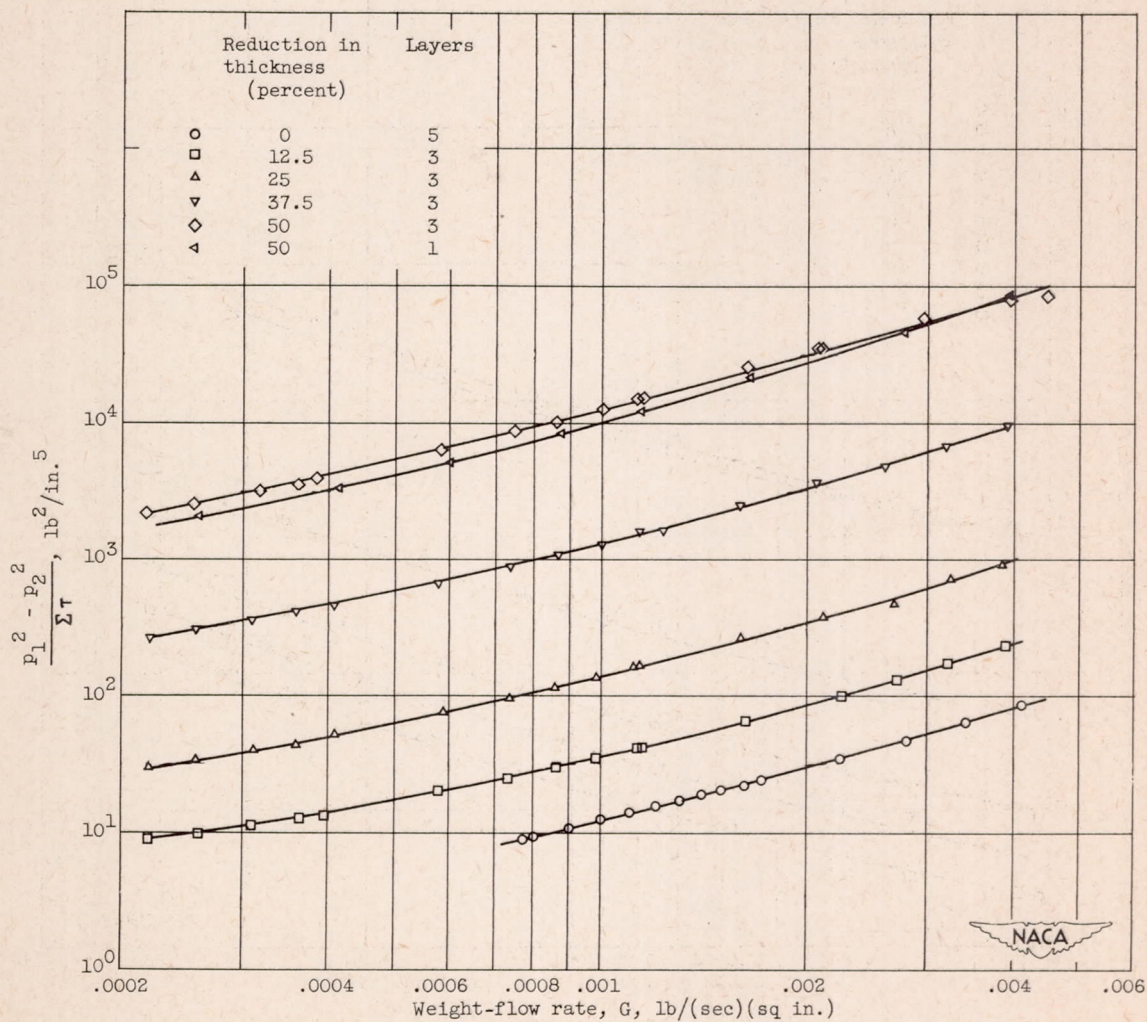
Figure 7. - Concluded. Correlation of air-flow data for unbraided and rolled stainless-steel corduroy wire cloth.
