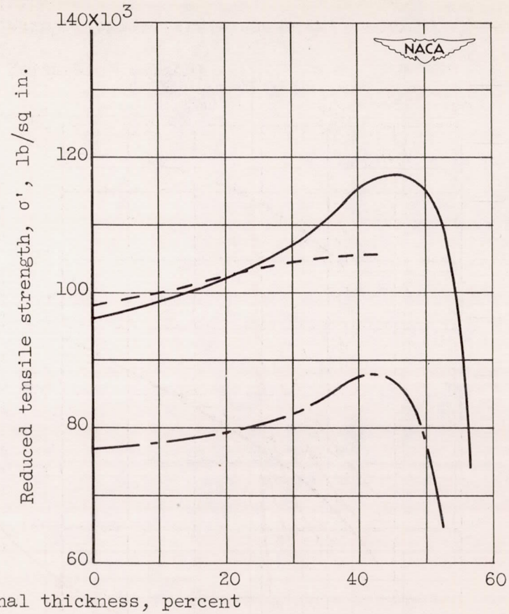
Figure 15. - Effect of rolling on tensile strength of unbrazed stainless-steel corduroy wire cloth.
