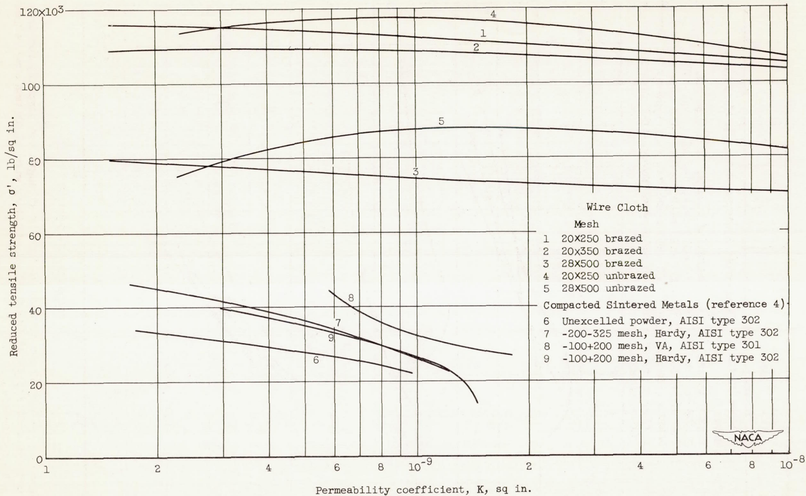
Figure 18. - Comparison of reduced tensile strength and permeability coefficient for braided and unbrazed rolled stainless-steel corduroy wire cloth and some compacted sintered metals.
