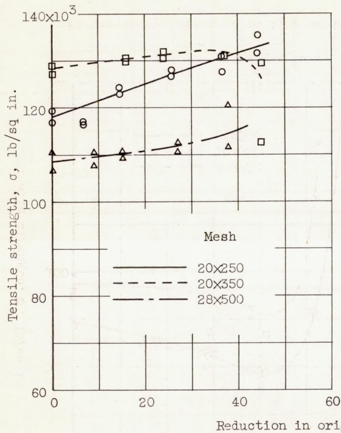
Figure 16. - Effect of rolling on tensile strength of brazed stainless-steel corduroy wire cloth.
