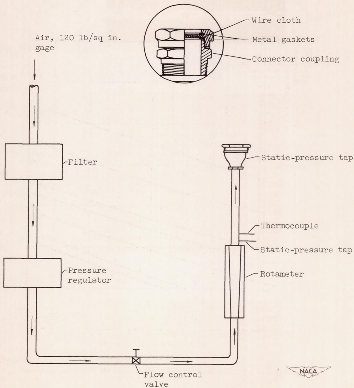
Figure 6. - Schematic diagram of test equipment for measuring air flow through specimens of wire cloth.
