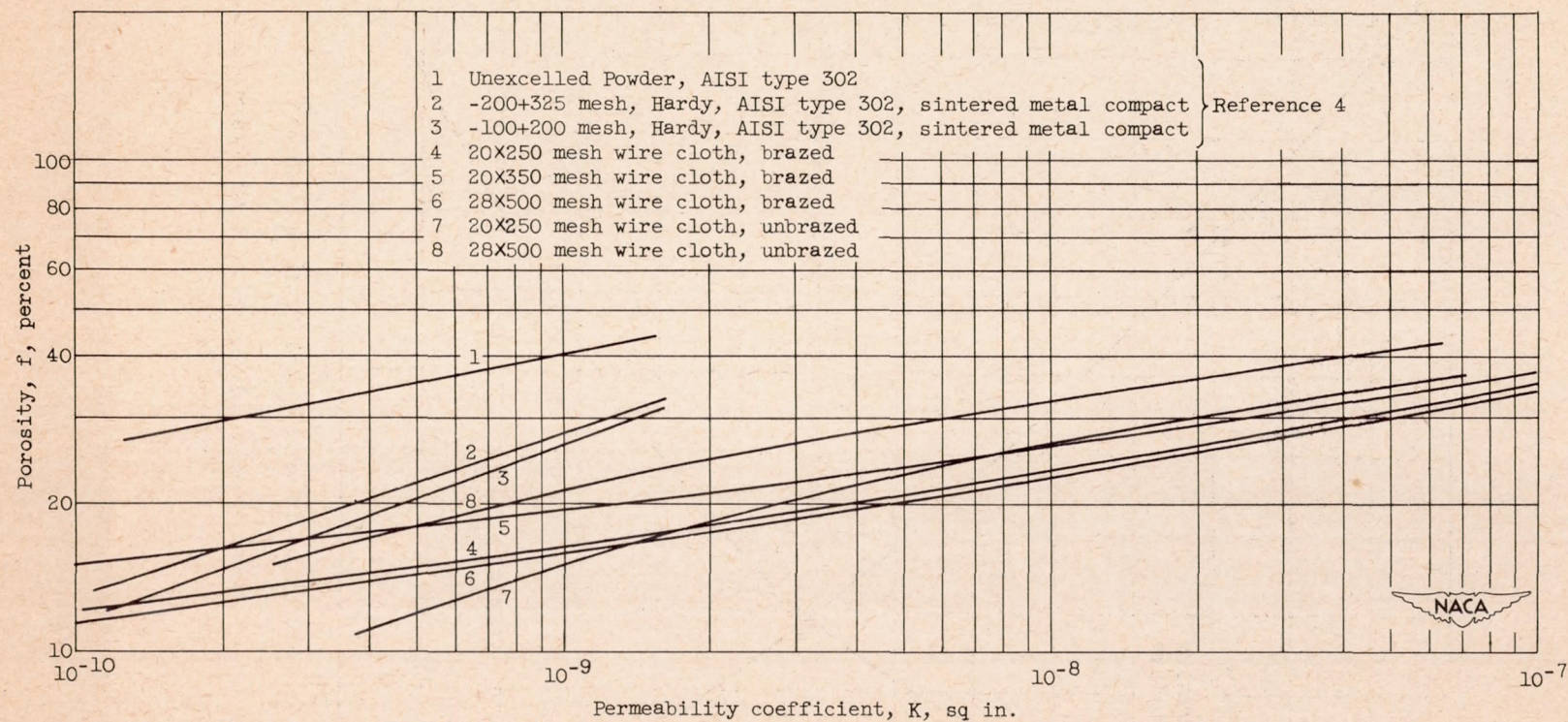
Figure 11. - Comparison of porosity and permeability coefficient for brazed and unbrazed rolled stainless-steel corduroy wire cloth and some sintered-metal compacts.
