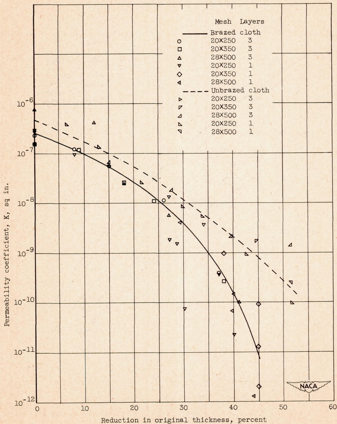
Figure 10. - Effect of rolling on permeability coefficient of braided and unbraided wire cloth in three mesh sizes.
