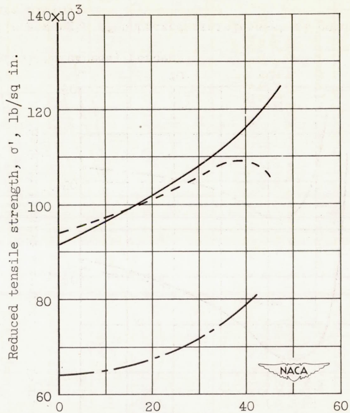
Figure 16. - Effect of rolling on tensile strength of brazed stainless-steel corduroy wire cloth.
