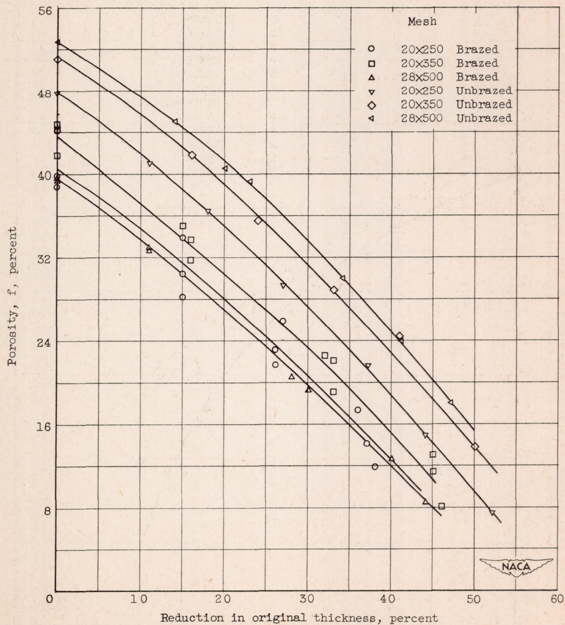
Figure 9. - Effect of rolling on porosity of braided and unbrazed wire cloth in three mesh sizes.
