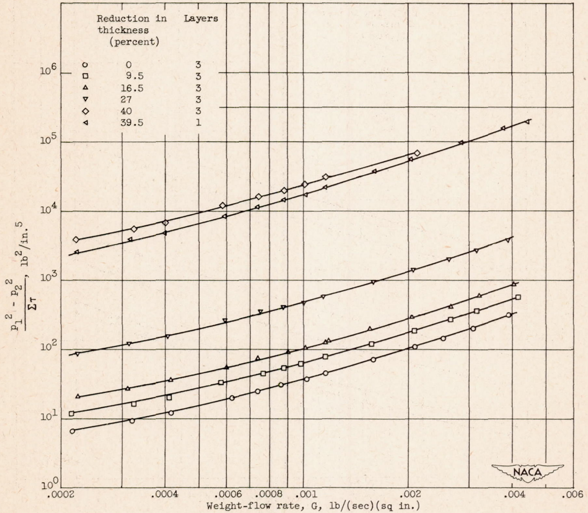
Figure 8. - Concluded. Correlation at air-flow data for brazed and rolled stainless-steel corduroy wire cloth.
