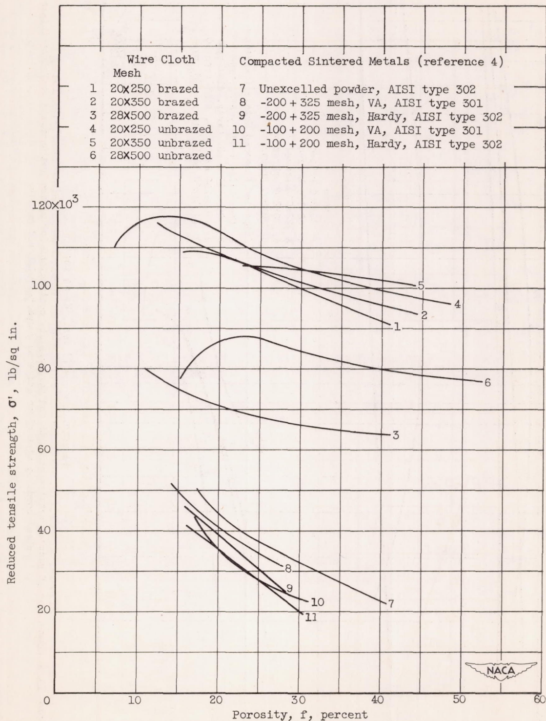
Figure 17. - Comparison of reduced tensile strength and porosity for brazed and unbrazed rolled stainless-steel corduroy wire cloth and some compacted sintered metals.
