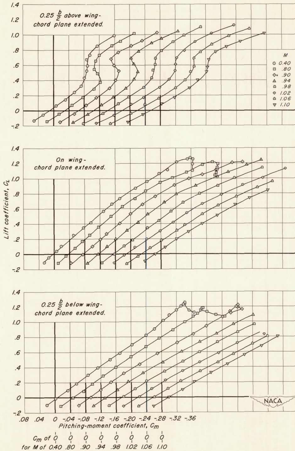
Figure 11.— The pitching-moment characteristics of the model with the tail in each of the three positions. i_1, 0^\circ
