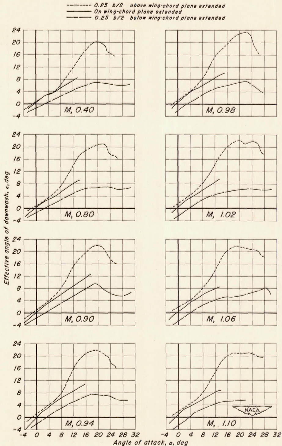
Figure 9.- Variation of downwash with angle of attack.
