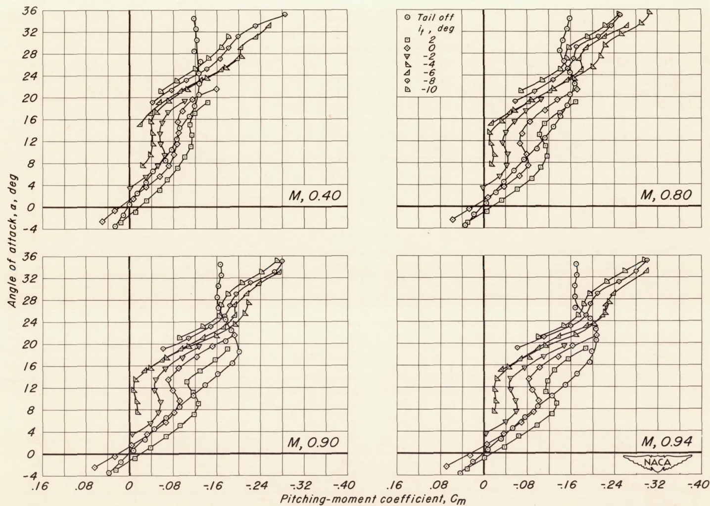
Figure 6.- The effects of the horizontal-tail incidence on the pitching-moment characteristics, tail above the wing-chord plane.
