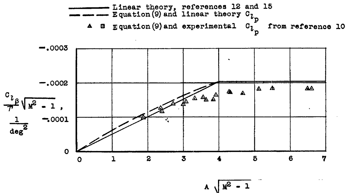
(a) Triangular wings.
