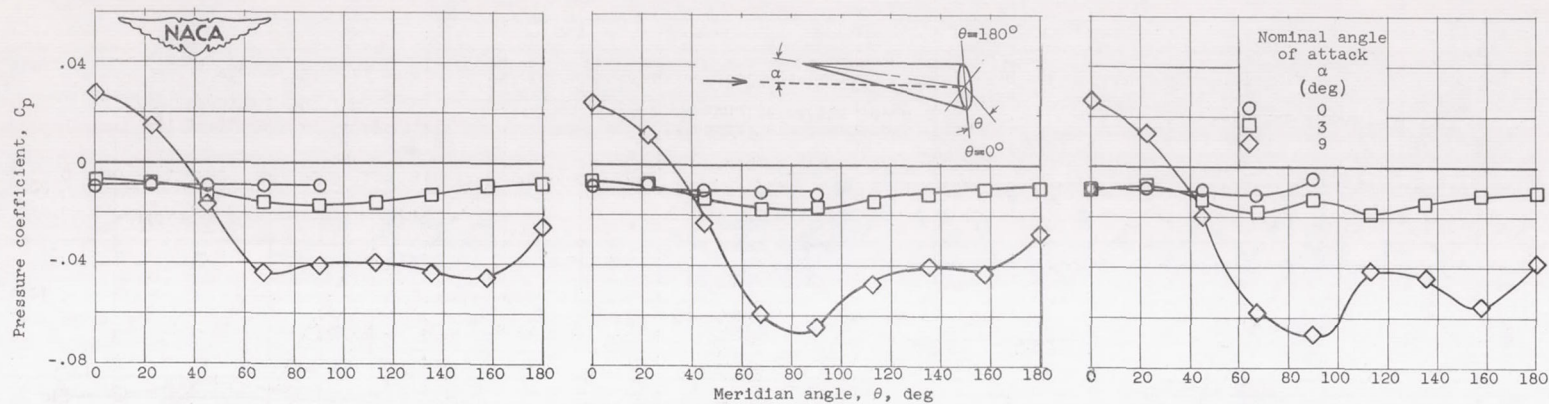
(g) Axial station, 1.708 feet; Reynolds number, 2 \times 10^6 .
