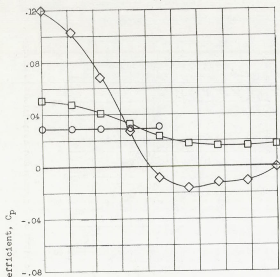
(a) Axial station, 0.584 feet; Reynolds number, 2 \times 10^6 .
