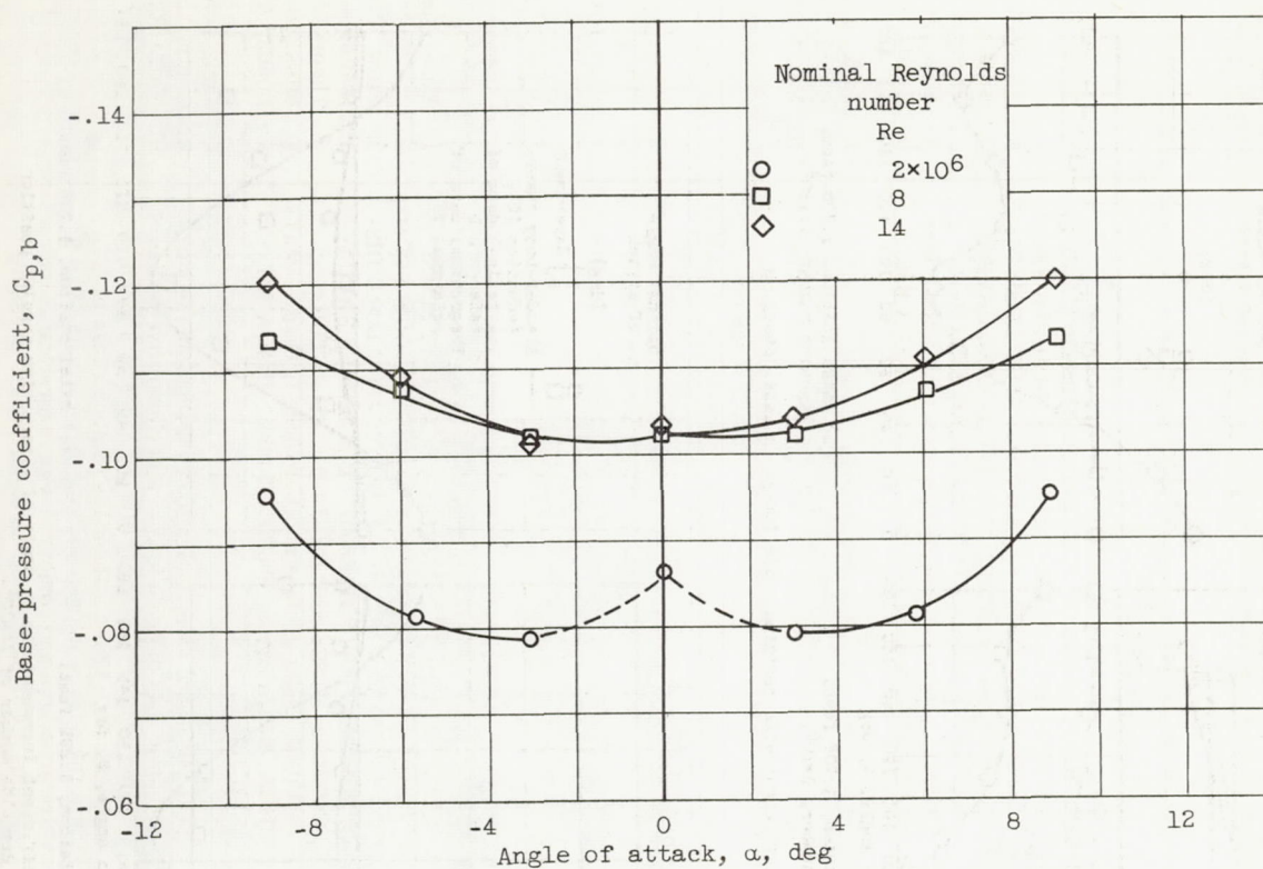
Figure 14. - Variation of base-pressure coefficient with angle of attack for Reynolds numbers of 2 \times 10^6 , 8 \times 10^6 , and 14 \times 10^6 .
