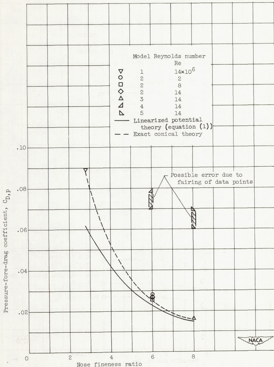
Figure 7. - Experimental and theoretical variation of pressure-fore-drag coefficient with nose fineness ratio.
