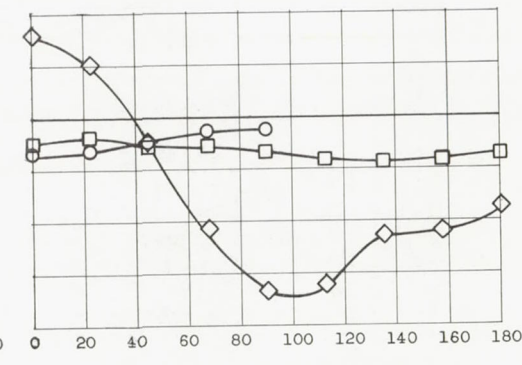
(f) Axial station, 1.291 feet; Reynolds number, 14 \times 10^6 .
