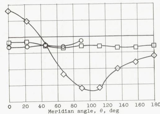
(e) Axial station, 1.291 feet; Reynolds number, 8 \times 10^6 .
