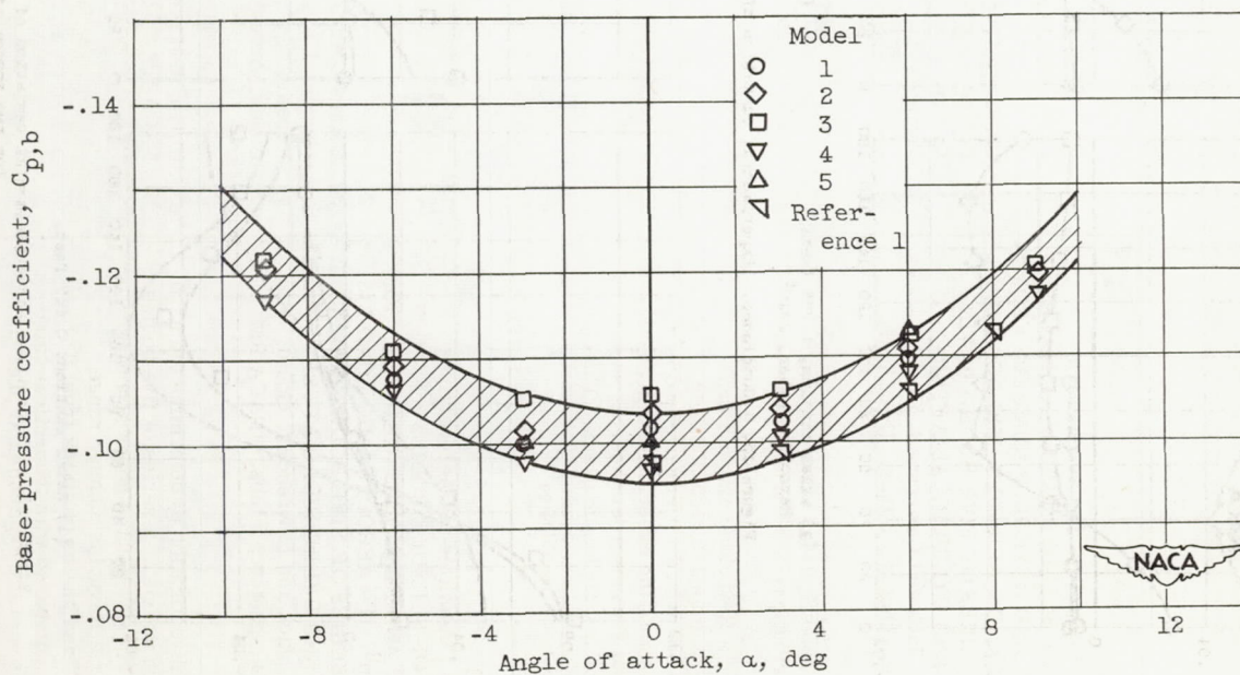
Figure 15. - Variation of base-pressure coefficient with angle of attack for five models at Mach number of 3.12 and Reynolds number of 14 \times 10^6 .
