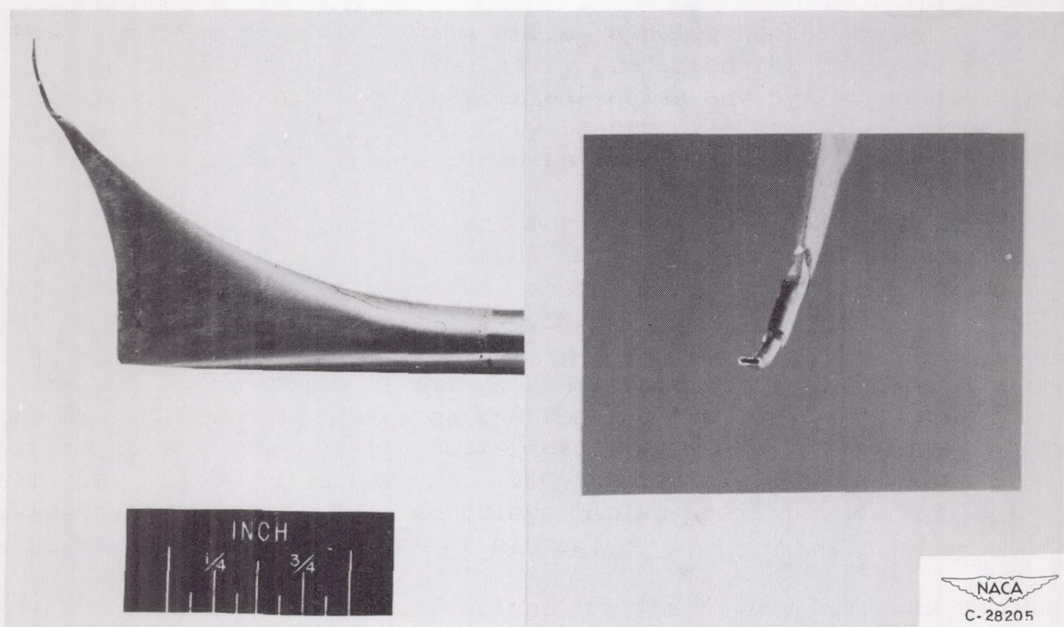
Figure 2. - Probe used to obtain boundary-layer data at zero angle of attack.
