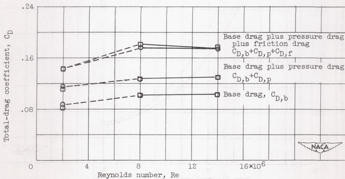
Figure 9. - Variation of total-drag coefficient with Reynolds number for zero angle of attack.
