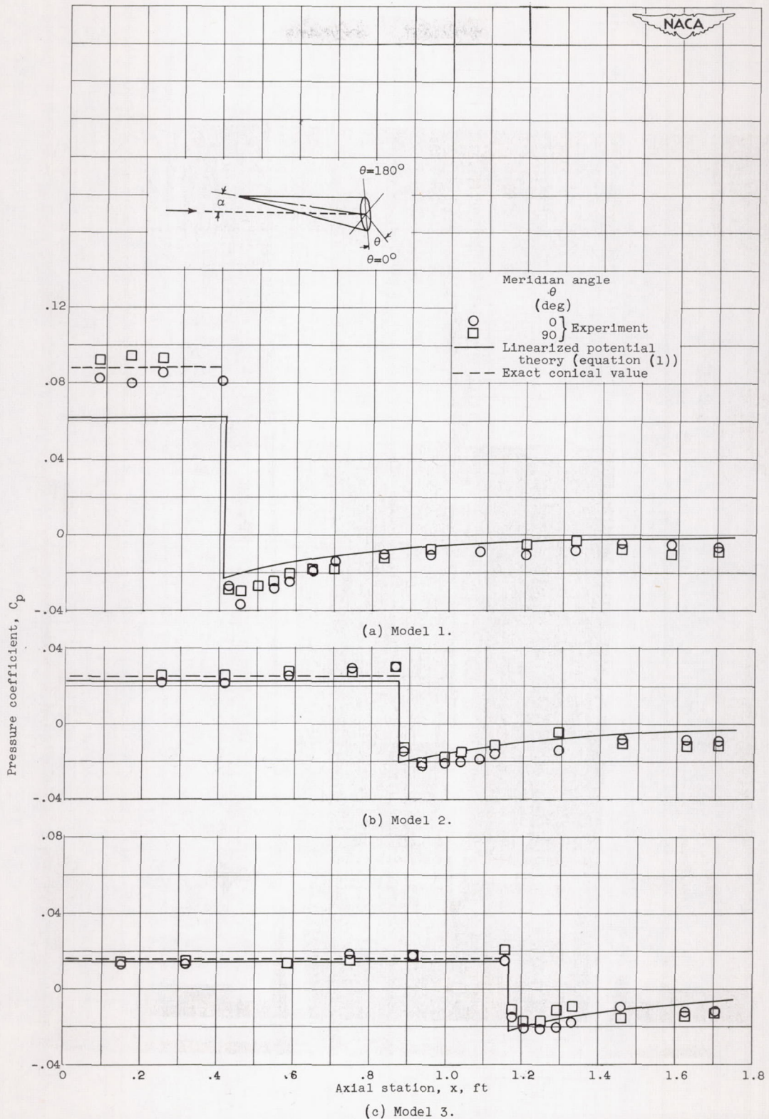
Figure 4. - Experimental and theoretical axial variation of pressure coefficient for model at zero angle of attack and Reynolds number of 14 \times 10^6 .
