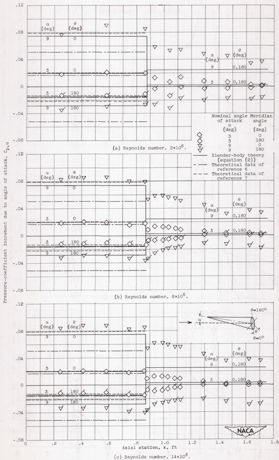
Figure 11. - Experimental and theoretical axial variation of pressure-coefficient increment due to angle of attack.
