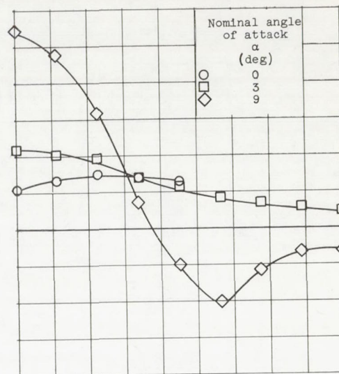
(c) Axial station, 0.417 feet; Reynolds number, 14 \times 10^6 .
