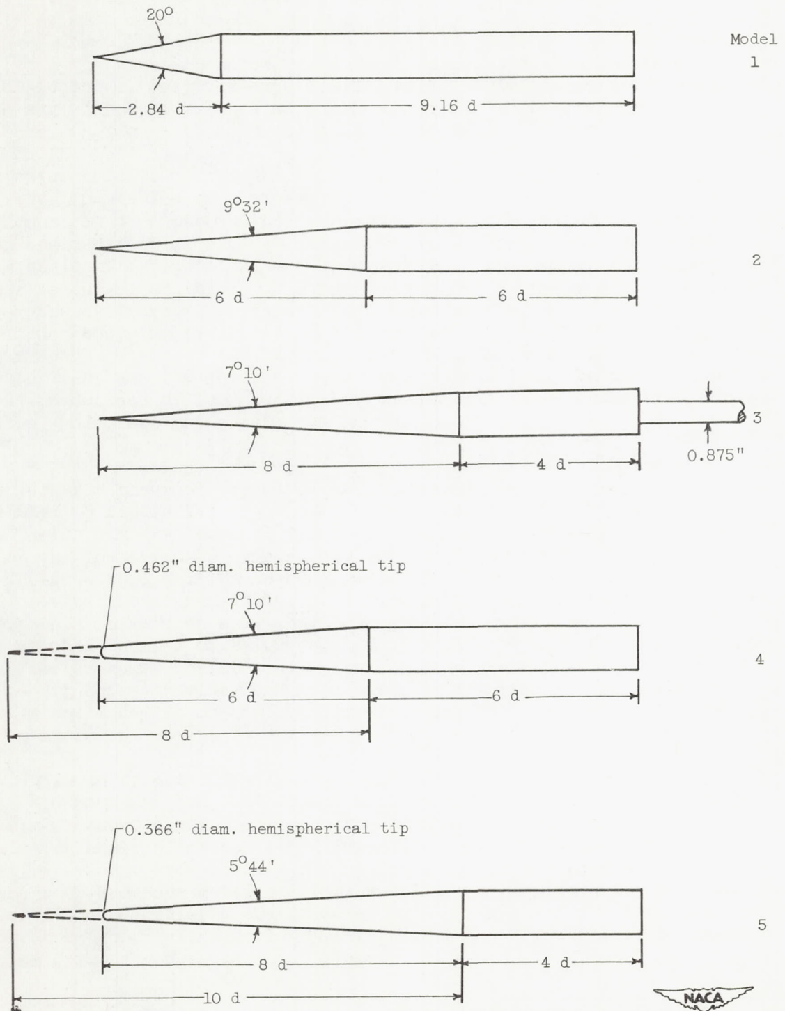
Figure 1. - Schematic drawing of models. Maximum body diameter d , 1.75 inches.
