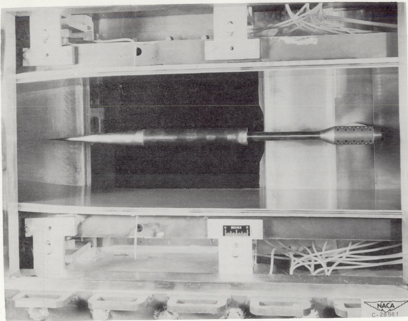
Figure 3. - Representative model 2 installed in Lewis 1- by 1-foot supersonic wind tunnel.
