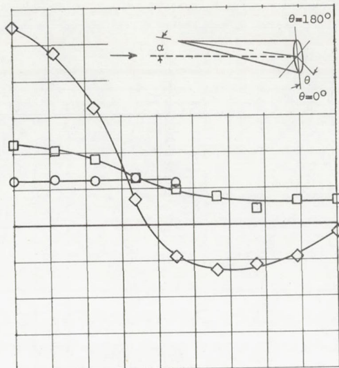
(b) Axial station, 0.417 feet; Reynolds number, 8 \times 10^6 .
