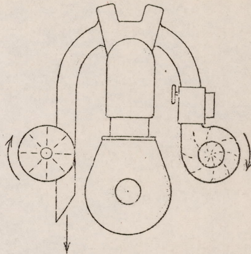
Fig.1 Rateau preliminary compression system.
