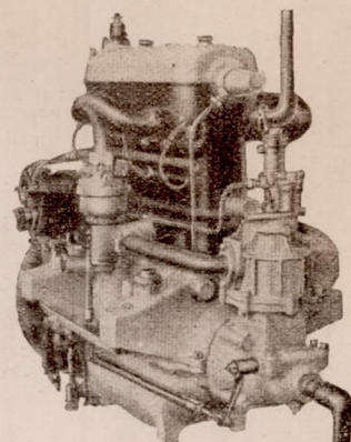
Fig. 11 Oblique view of engine from the compressor end.
