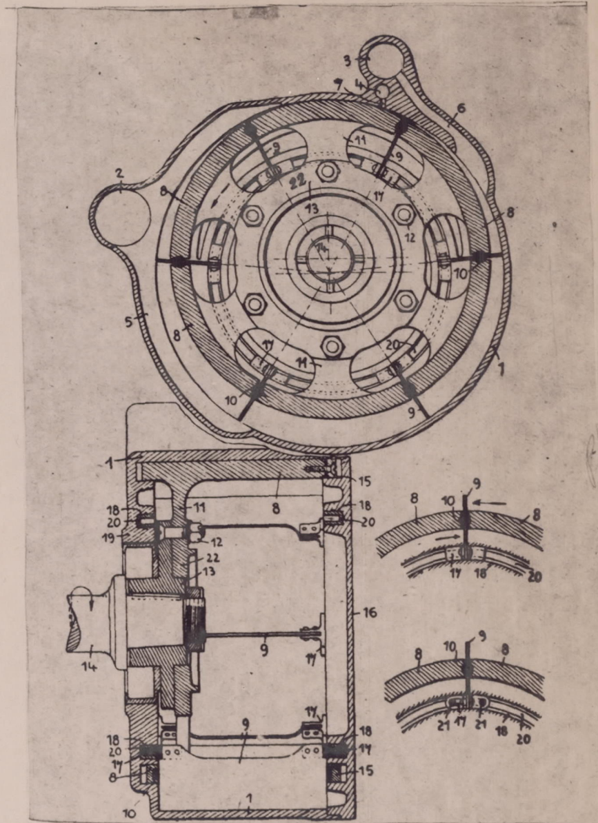
Fig. 6 Zoller Compressor
