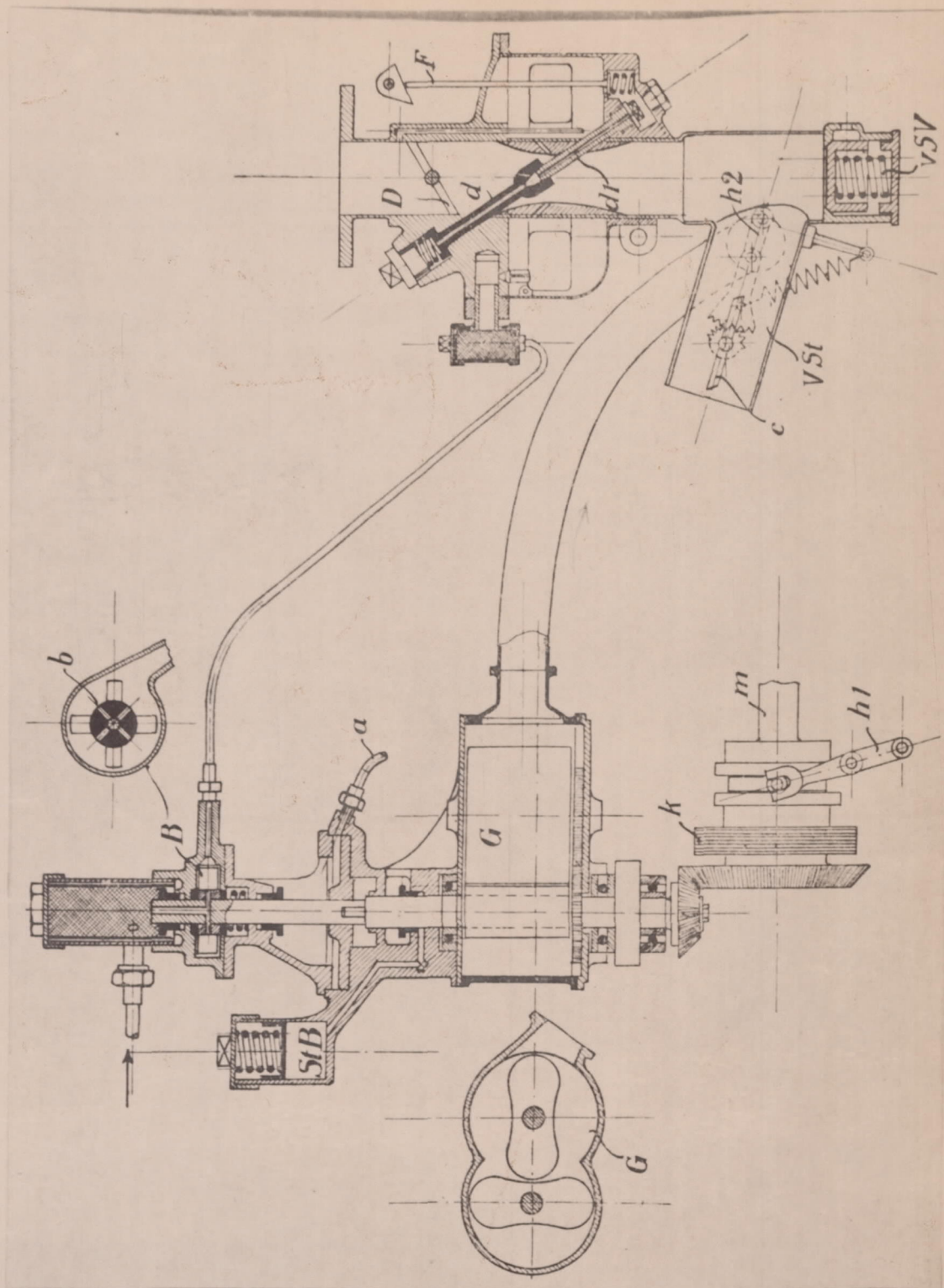
Fig.8 Daimler compressor and fuel delivery system.
