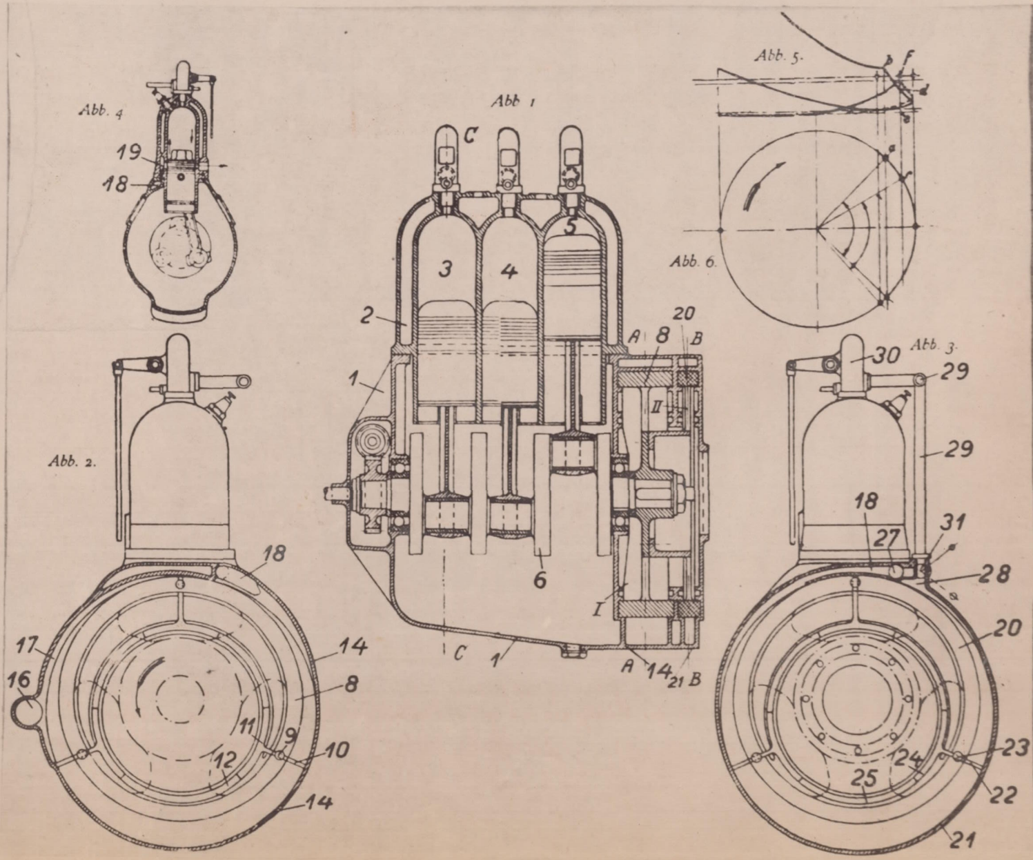
FIG. 7 Zoller compressor on flywheel of a 3-cyl. two-stroke engine.
