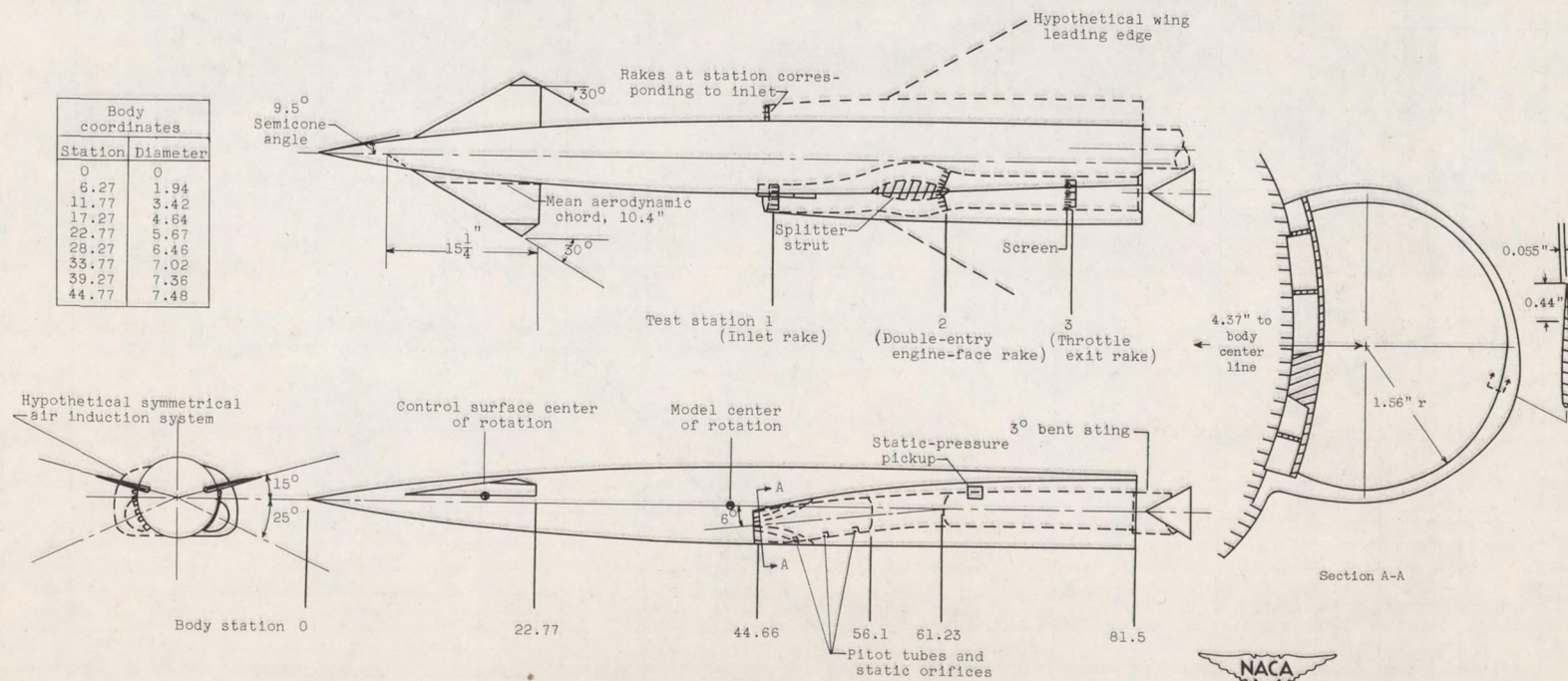
Figure 2. - Schematic drawing of test model showing normal-shock side inlet and subsonic diffuser.
