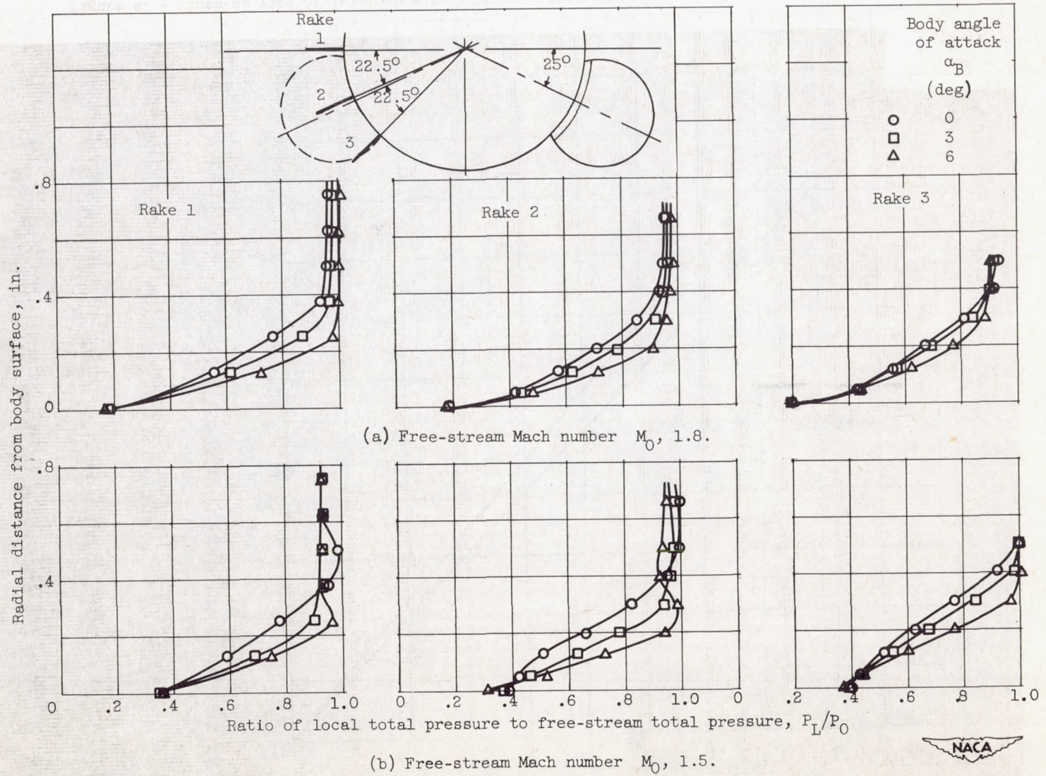
Figure 7. - Boundary-layer profiles at inlet station. Control surface deflection \delta , 0.
