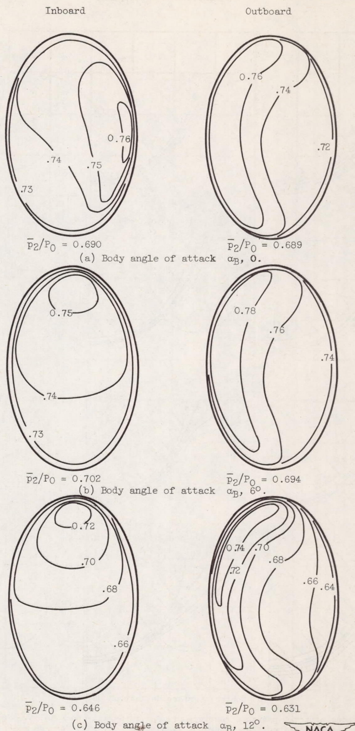
Figure 9. - Contours of total pressure recovery at engine twin intake faces at 0.95 engine rated mass flow. Free-stream Mach number M_0 , 1.8; control surface deflection \delta , 0; angle of yaw \psi , 0.
