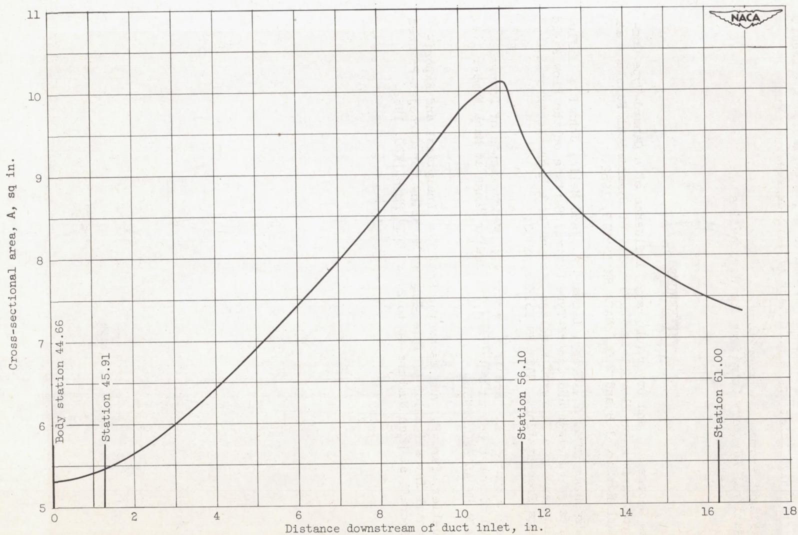
Figure 3. - Variation of duct cross-sectional area (normal to center line of flow) with distance downstream of inlet.
