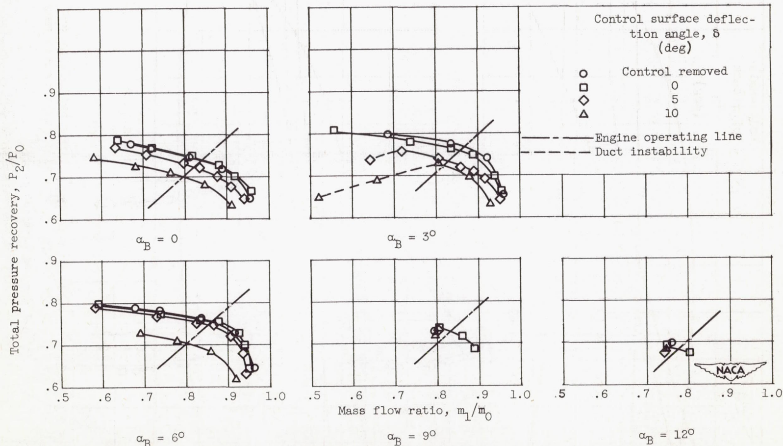
Figure 11. - Concluded. Total-pressure-recovery mass-flow relationships for various control surface deflection angles. Angle of yaw \Psi , 0.
