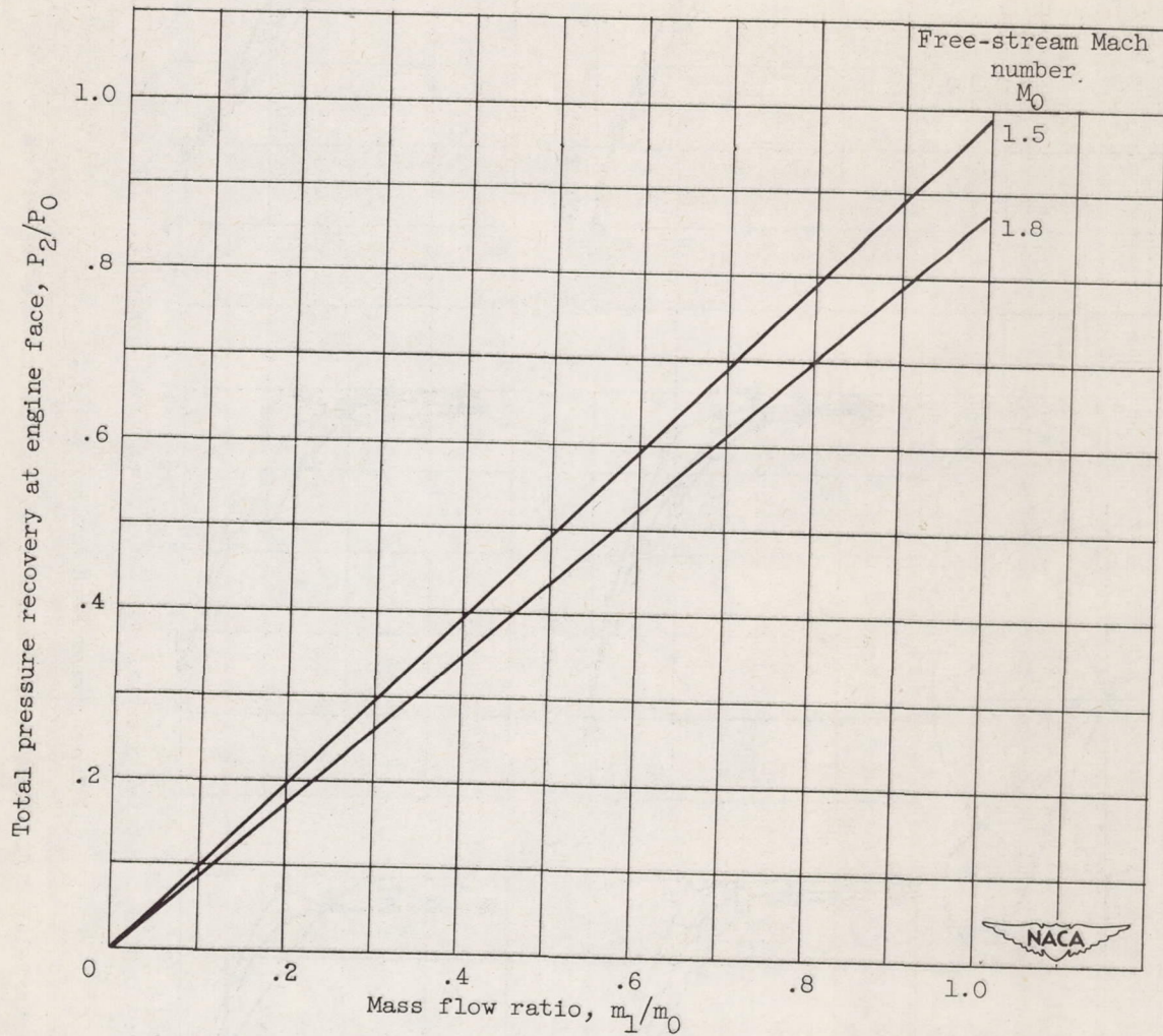
Figure 6. - Engine operating lines for given altitude (tropopause) and hypothetical turbojet engine (at rated engine speed).
