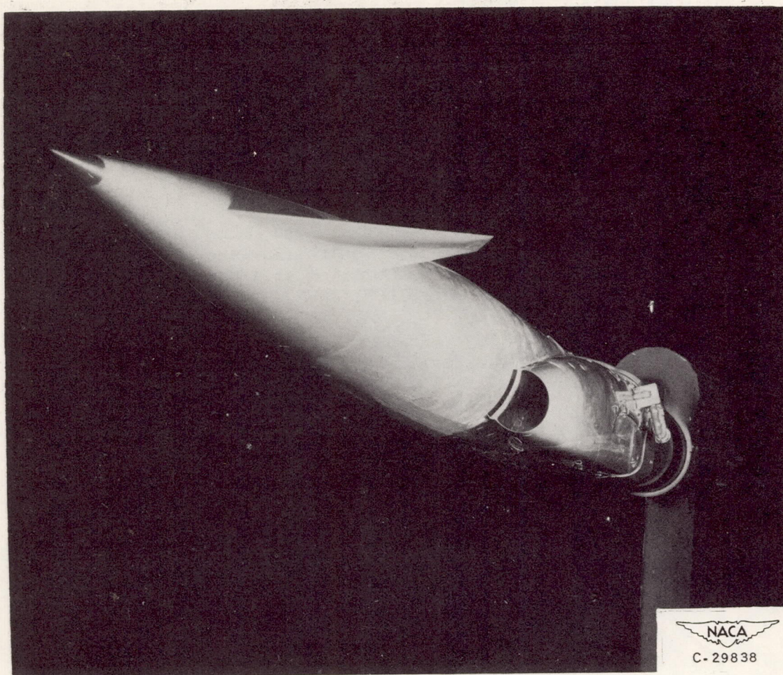
Figure 1. - Inlet-body-control surface configuration mounted in 8- by 6-foot supersonic tunnel. Inlet survey rake removed.
