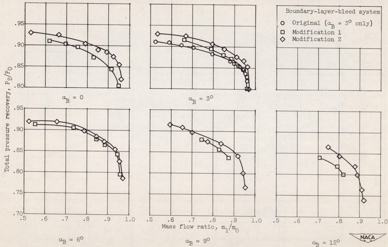
(a) Free-stream Mach number M_0 , 1.5.
