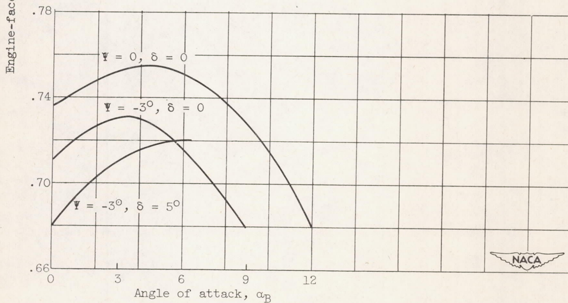
(b) Free-stream Mach number M_0, 1.8 .
