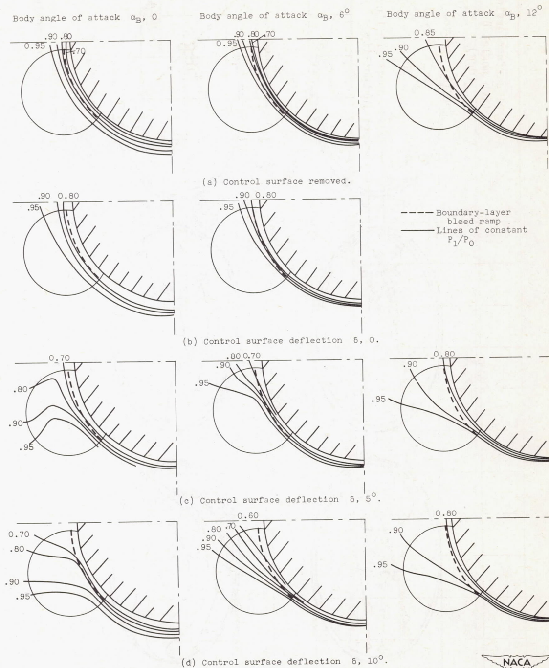
Figure 10. - Contours of total pressure recovery P_1/P_0 at normal-shock inlet. Free-stream Mach number M_0, 1.8 . (Data obtained from reference 1; data not obtained for \alpha_B = 12^\circ, \delta = 0 .)
