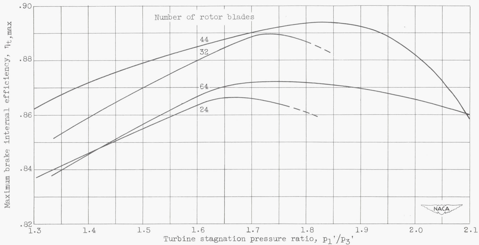
Figure 5. - Maximum brake internal efficiency obtainable at each stagnation pressure ratio.
