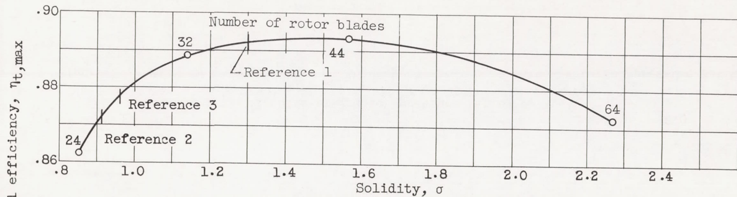
(a) Variation with solidity.
