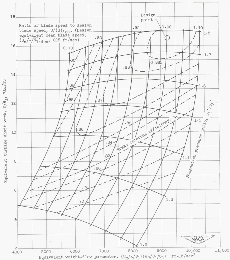
(c) 32-blade-rotor-turbine configuration.
