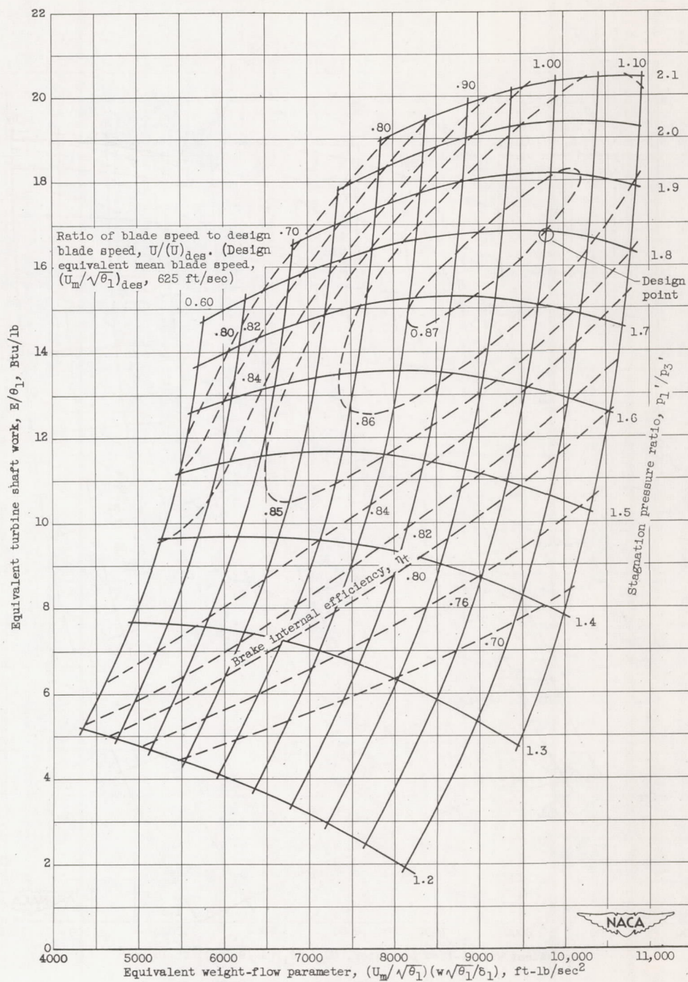
Figure 4. - Continued. Over-all turbine performance.
