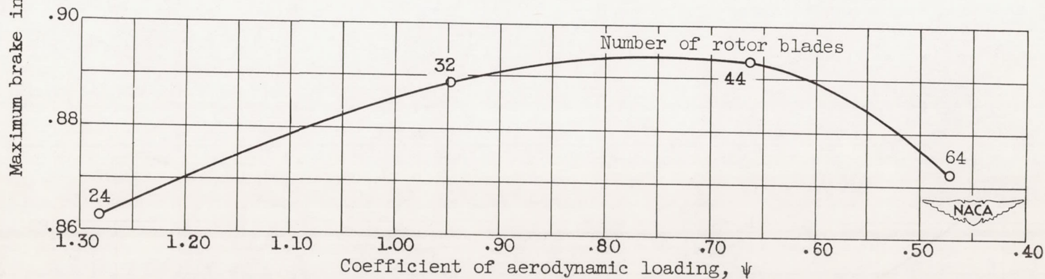
(b) Variation with coefficient of aerodynamic loading.
