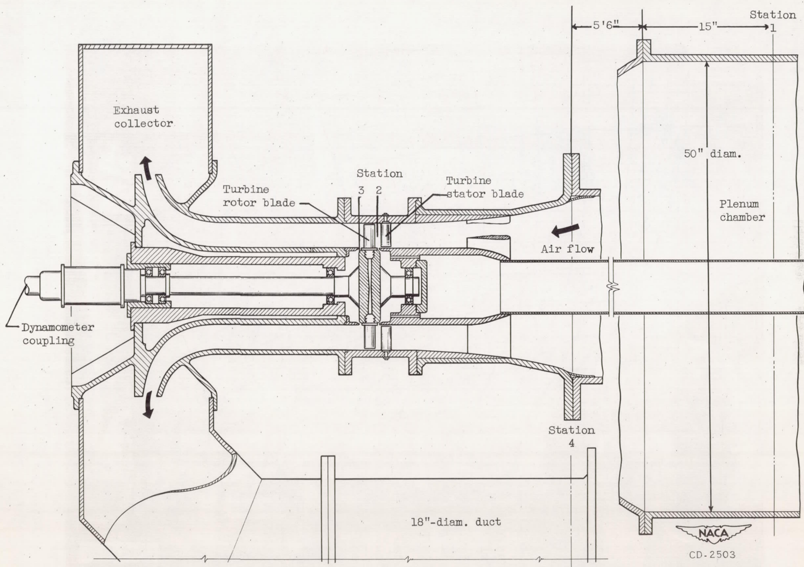
Figure 3. - Schematic section of turbine installation showing measuring stations.
