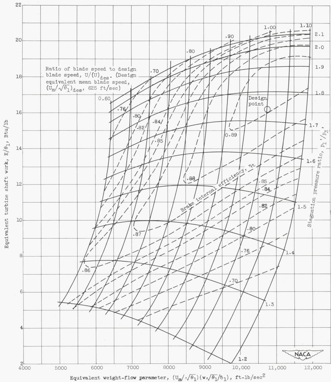
Figure 4. - Over-all turbine performance.
