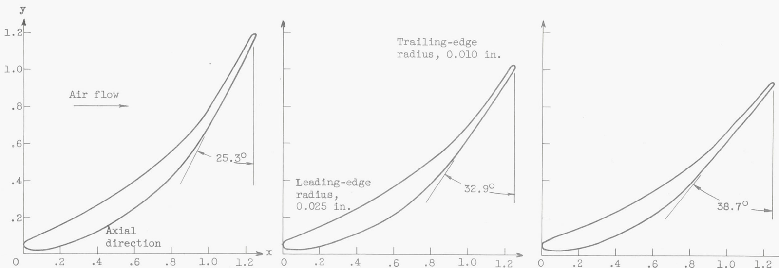
Hub-section radius, 4.20 in.
