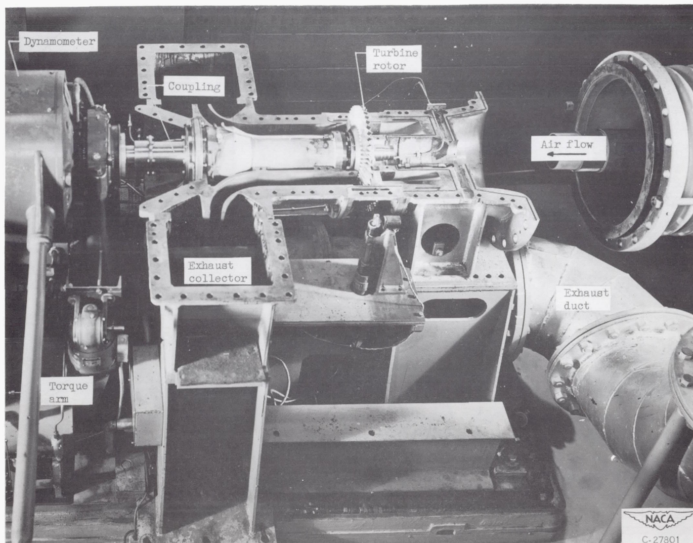
Figure 2. - Turbine installation with top half of casing removed.
