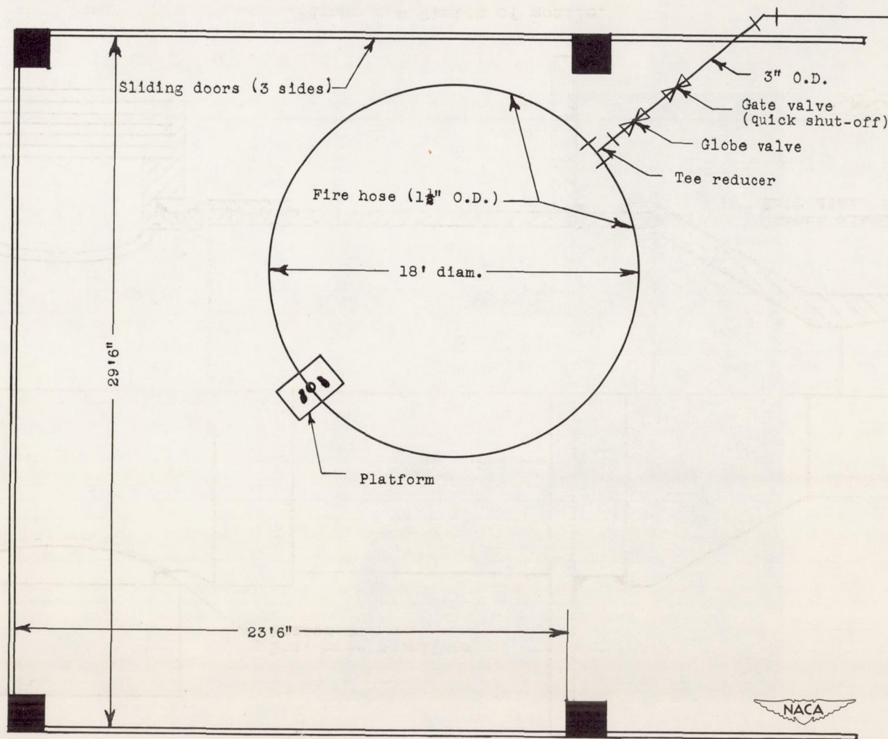
Figure 2.- Test layout.
