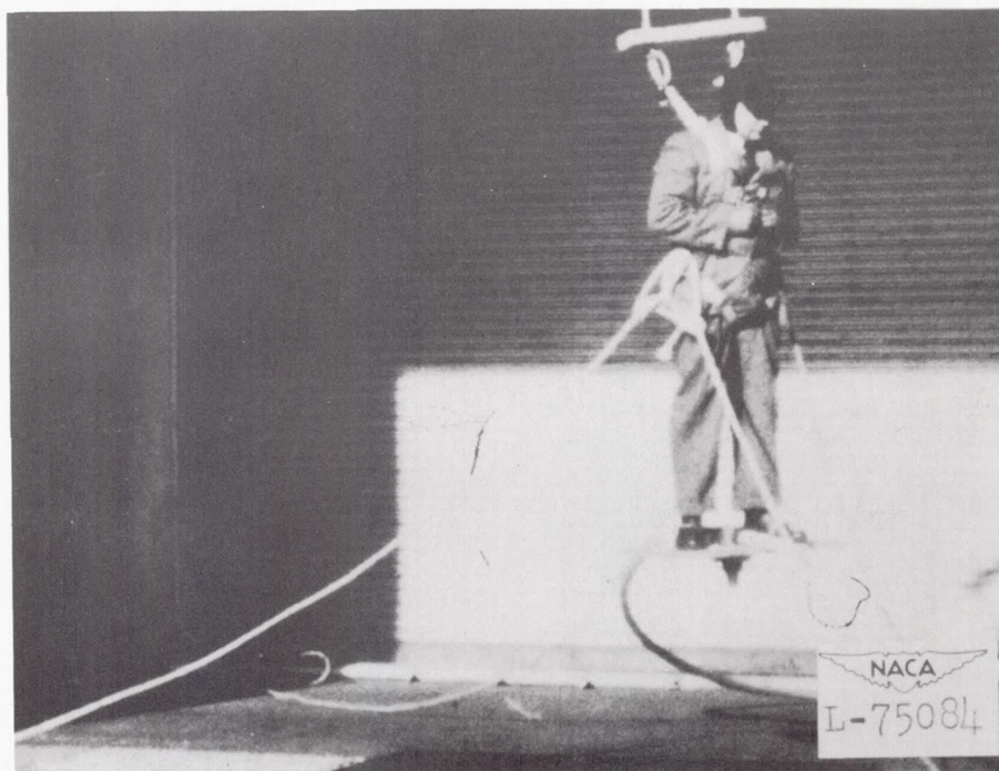
Figure 15.- Flyer A in flight.
