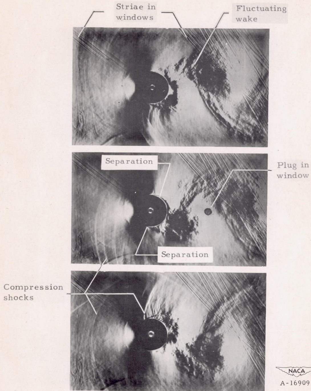
Figure 3. - Schlieren pictures of the flow about a 1.97-inch cylinder in the Ames 1- by 3 \frac{1}{2} -foot wind tunnel at a Mach number of 0.51.
