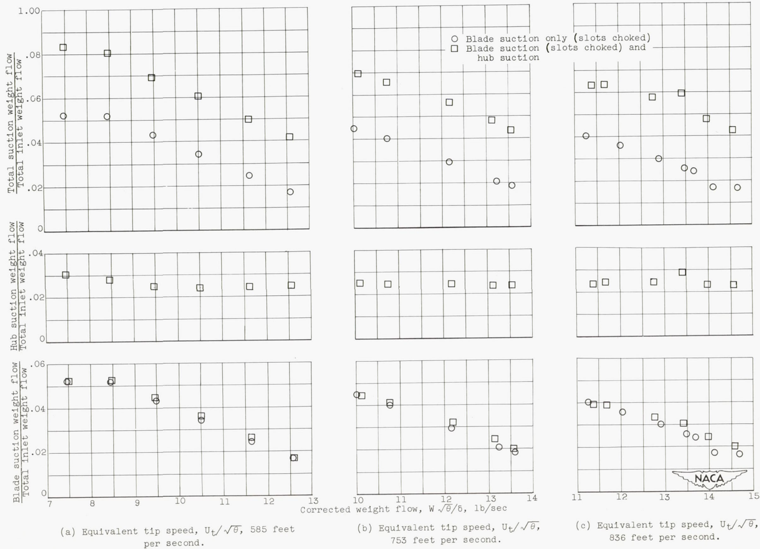
Figure 9. - Variation of suction weight flows with compressor weight flow for three tip speeds.
