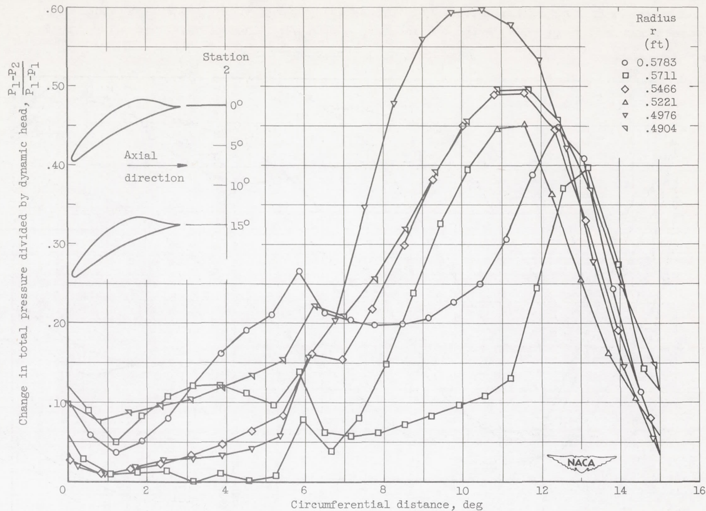
Figure 10. - Stator-loss survey. U_t/\sqrt{\theta} , 836 feet per second; W\sqrt{\theta}/\delta , 13.47 pounds per second; blade suction weight flow, 0.35 pound per second; without hub suction.
