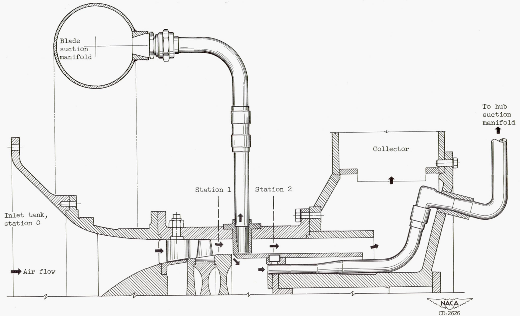
Figure 5. - Cross section of compressor flow passage.
