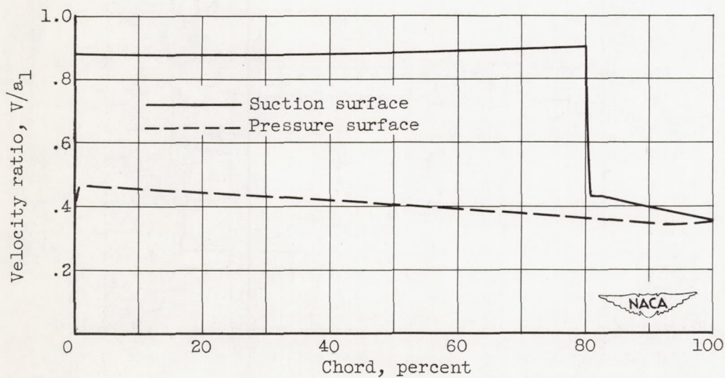
Figure 4. - Two-dimensional potential-flow velocity distribution on hub section of stator blade.
