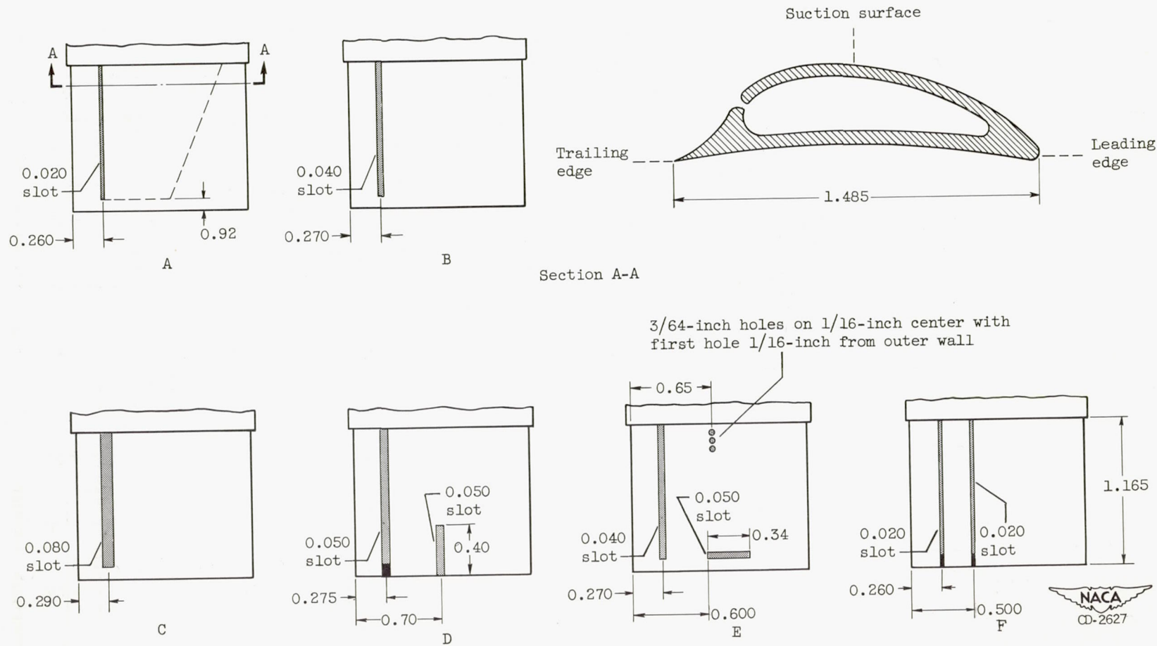
Figure 7. - Suction slot configurations.
