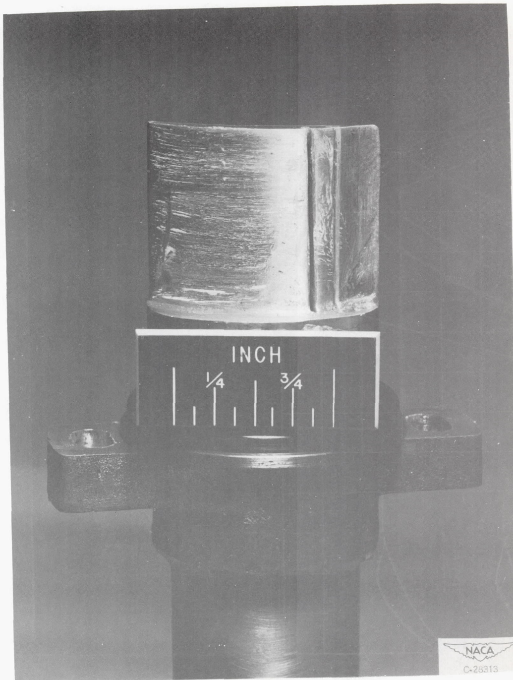
Figure 13. - Flow traces on blade without blade suction.
