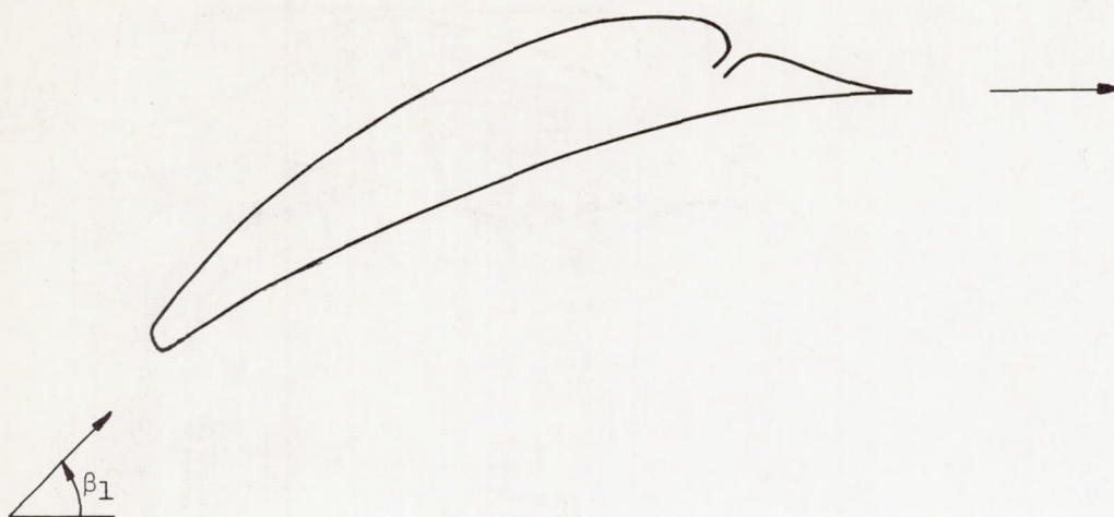
Figure 3. - Stator-blade profile at hub. r , 0.4854 feet; c , 0.1238 feet; \sigma , 0.97; M_1 , 0.7; \beta_1 , 45^\circ ; \beta_2 , 0^\circ .
