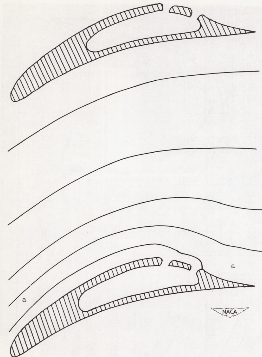
Figure 12. - Approximate streamlines in two-dimensional potential flow past hub section of stator blade.
