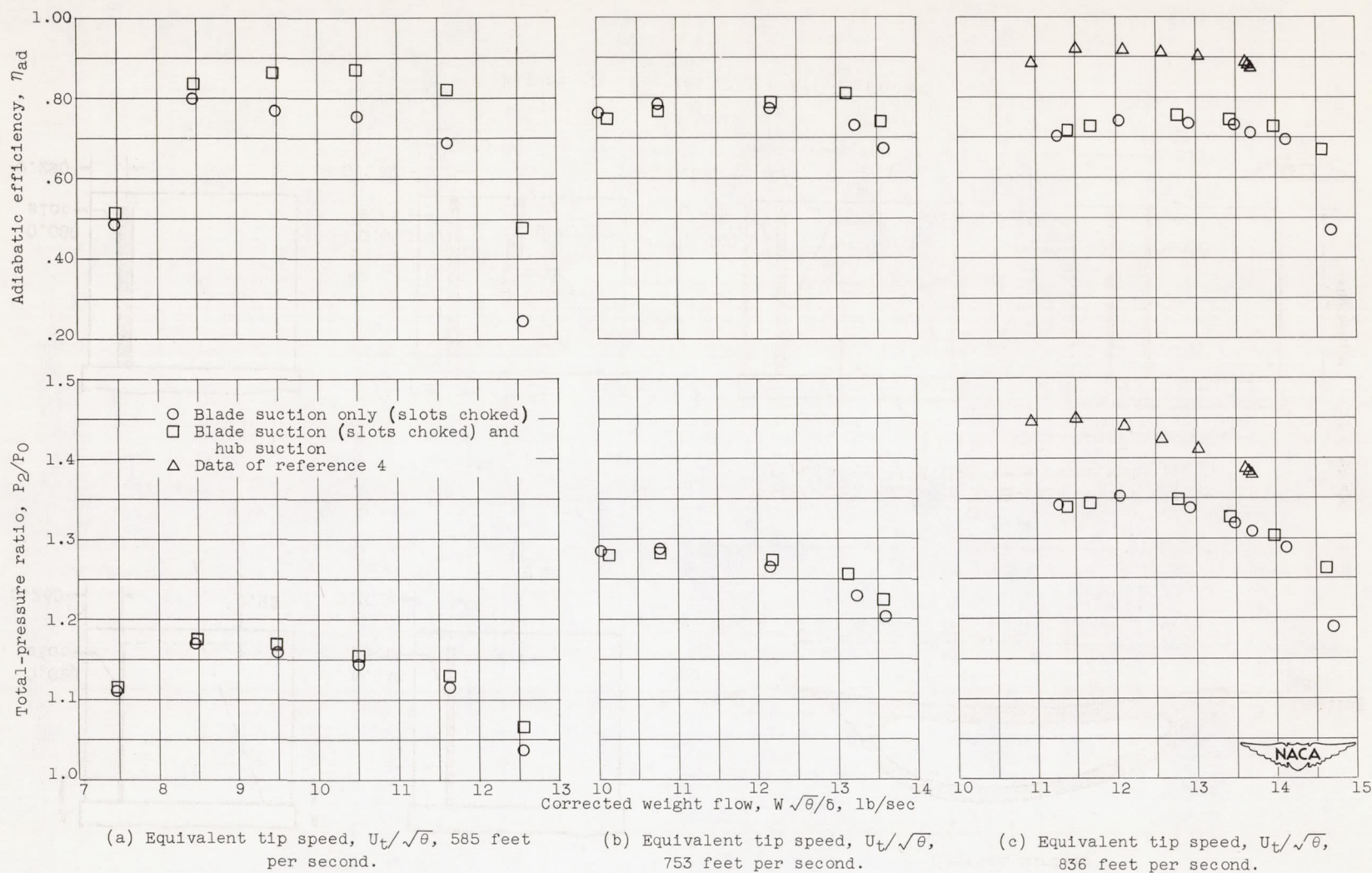
Figure 8. - Variation of total-pressure ratio and efficiency with compressor weight flow for three tip speeds.
