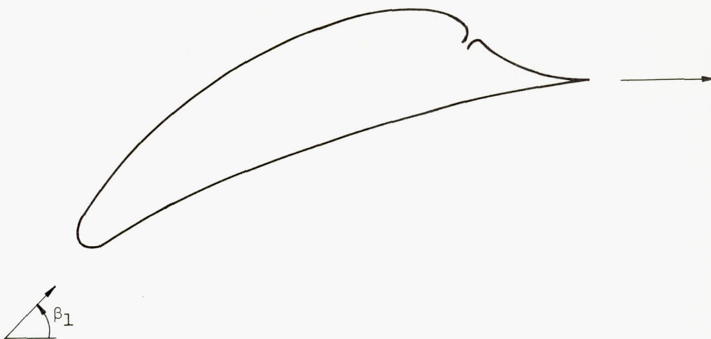
Figure 1. - Stator-blade profile at tip. r , 0.5833 feet; c , 0.1238 feet; \sigma , 0.81; M_1 , 0.6; \beta_1 , 45^\circ ; \beta_2 , 0^\circ .
