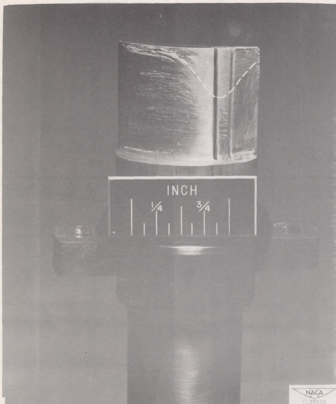
Figure 14. - Flow traces on blade with blade suction.
