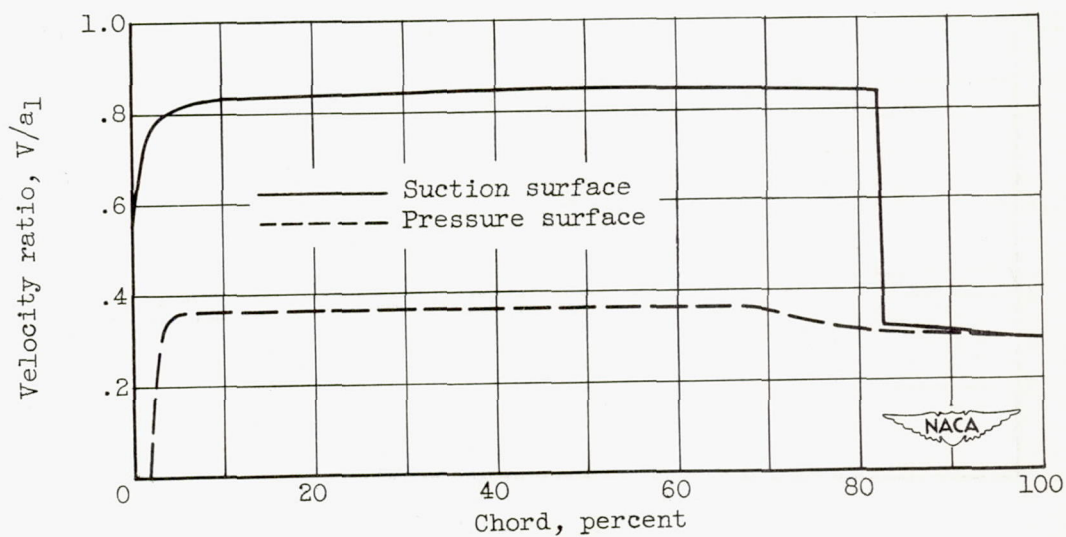
Figure 2. - Two-dimensional potential-flow velocity distribution on tip section of stator blade.
