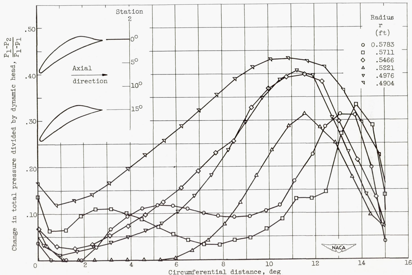
Figure 11. - Stator-loss survey. U_t/\sqrt{\theta} , 836 feet per second; W\sqrt{\theta}/\delta , 13.42 pounds per second; blade suction weight flow, 0.39 pound per second; hub suction weight flow, 0.41 pound per second.
