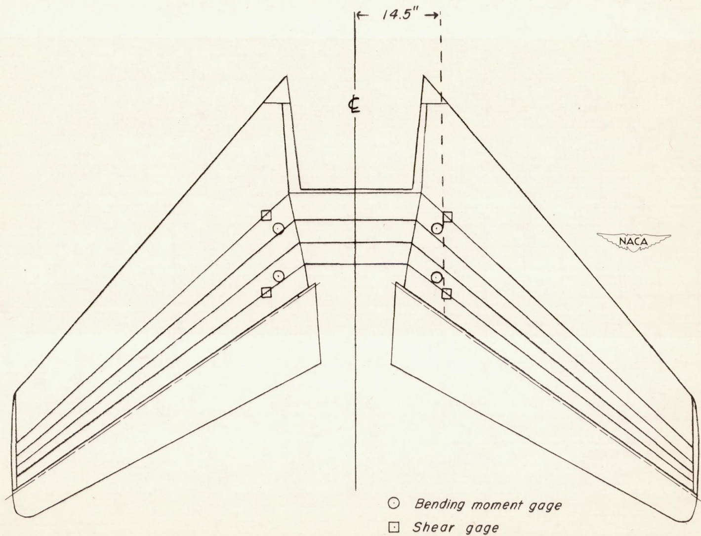
Figure 6.- Horizontal tail of X-5 airplane showing the location of the strain gages.
