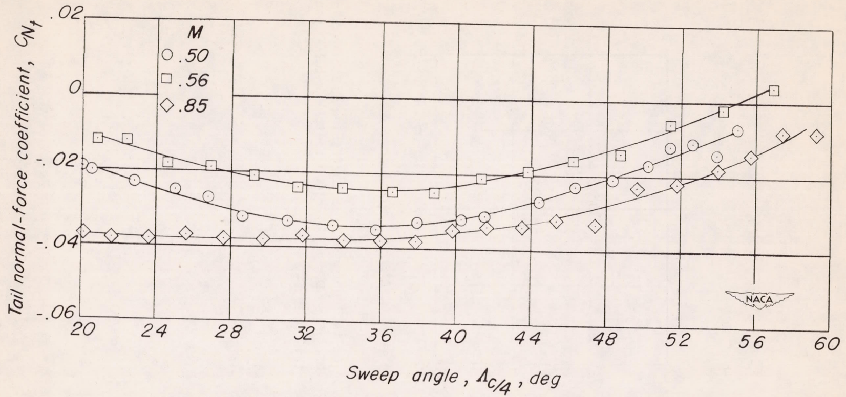
Figure 7.- Variation of tail normal-force coefficient with sweep angle for level flight. h_p \approx 20,000 feet; W \approx 8,500 pounds; c.g. \approx fuselage station 155.0.
