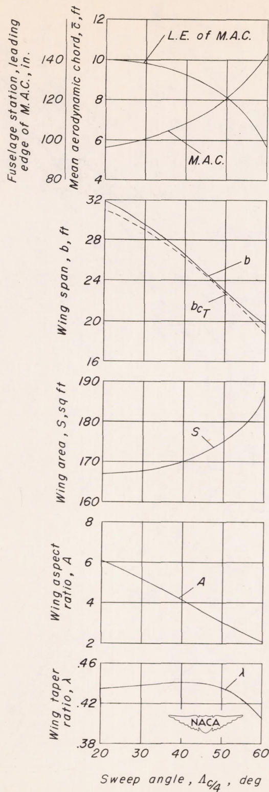
Figure 5.- Dimensional characteristics of X-5 airplane plotted against wing sweep angle.
