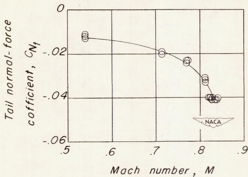
Figure 8.- Variation of tail normal-force coefficient with Mach number during level flight. \Lambda = 20^\circ ; h_p \approx 24,000 feet; W \approx 8,800 pounds; c.g. \approx fuselage station 155.4.
