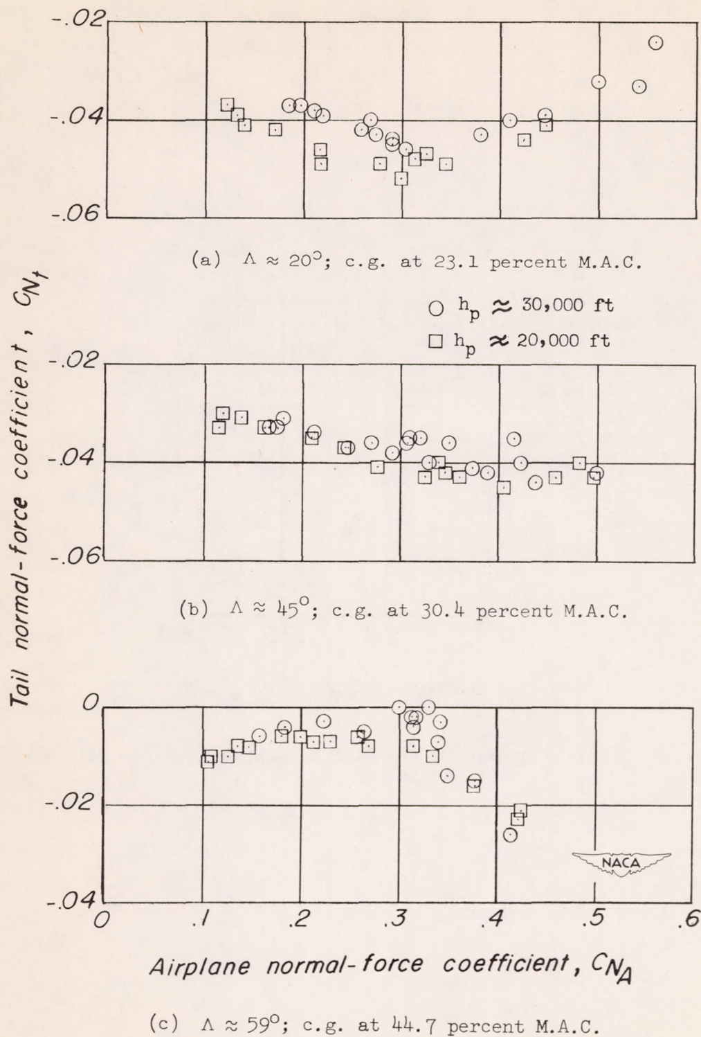
Figure 9.- Variation of tail normal-force coefficient with airplane normal-force coefficient during pull-ups. M \approx 0.83 .
