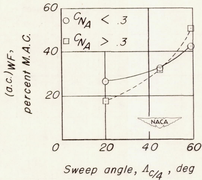
Figure 10.- Variation of wing-fuselage aerodynamic center with wing sweep angle for M \approx 0.83 .
