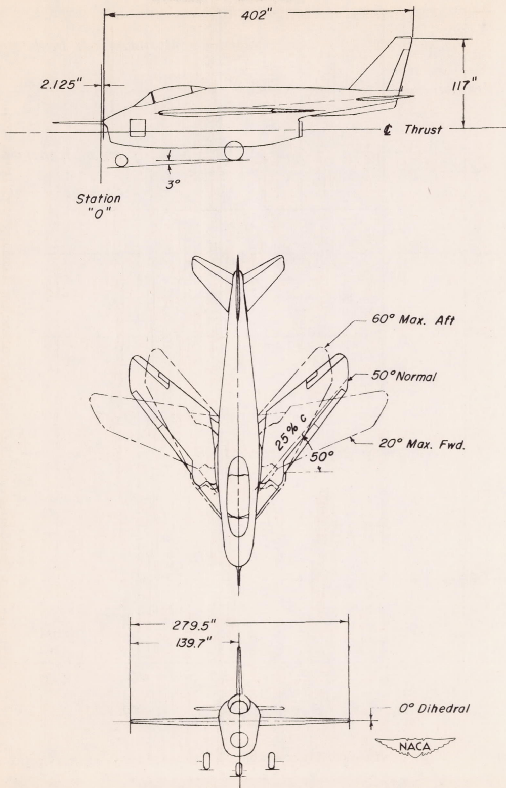
Figure 3.- Three-view drawing of the Bell X-5 airplane.
