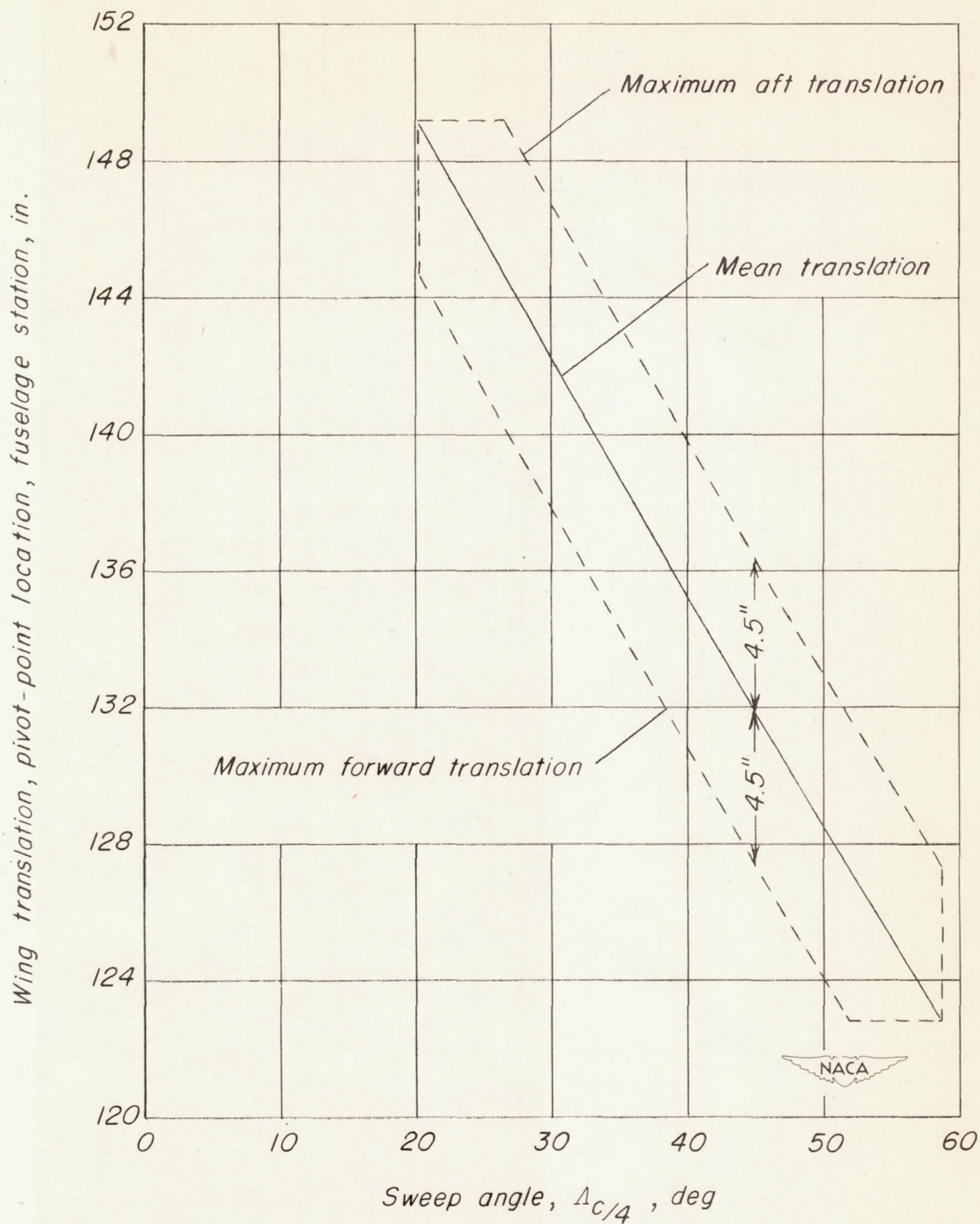
Figure 4.- Wing pivot-point location plotted against wing sweep angle X-5 airplane.
