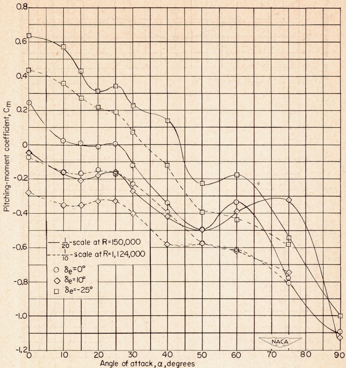
Figure 7.- Comparison of the pitching-moment characteristics of the modified \frac{1}{20} -scale model (sting nose installed) used in the current investigation and the larger scale model reported in reference 1. \psi = 0^\circ . (Small horizontal tail on both models.)
