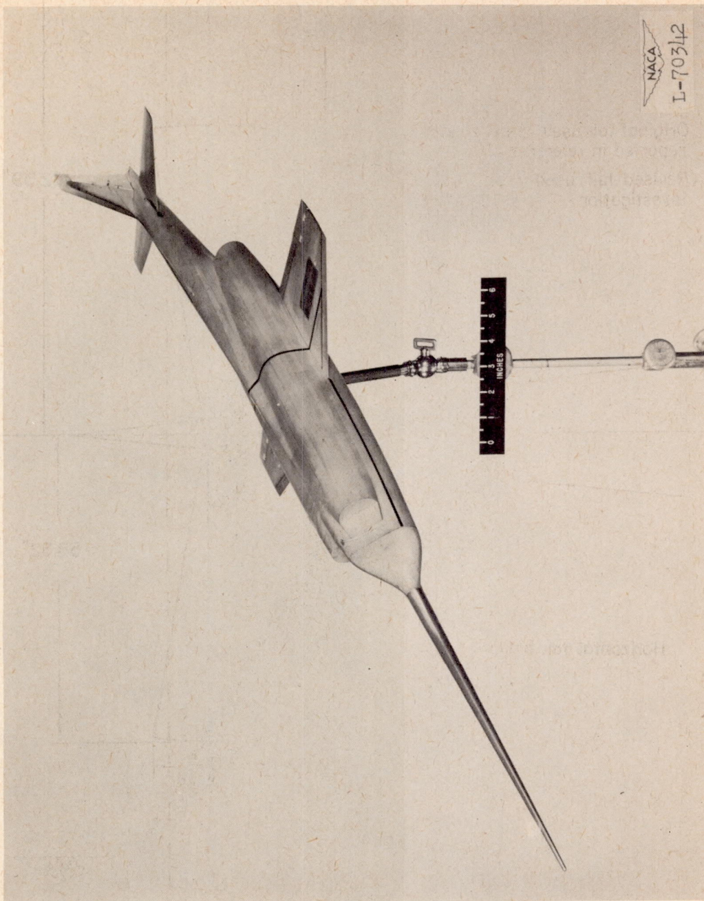
Figure 3.- Photograph of modified model - sting nose installed.
