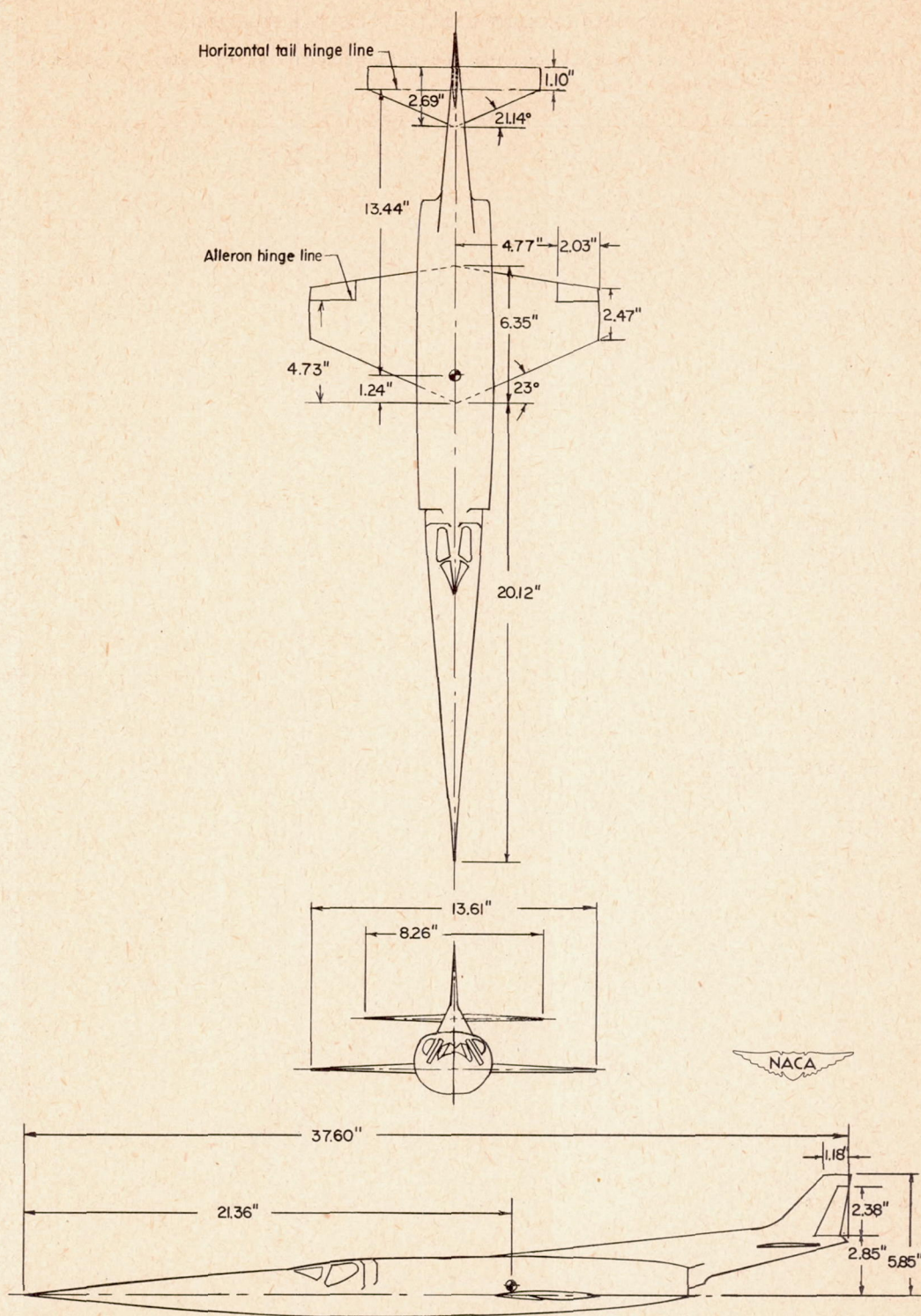
Figure 1.- Three-view drawing of the unmodified \frac{1}{20} -scale model investigated. (Large horizontal tail installed.)
