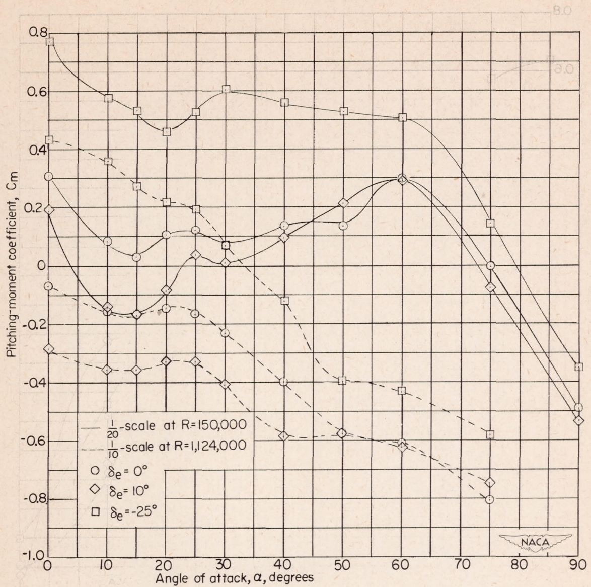
Figure 6.- Comparison of the pitching-moment characteristics of the the unmodified \frac{1}{20} -scale model used in the current investigation and the larger scale model reported in reference 1. \psi = 0^\circ . (Small horizontal tail on both models.)
