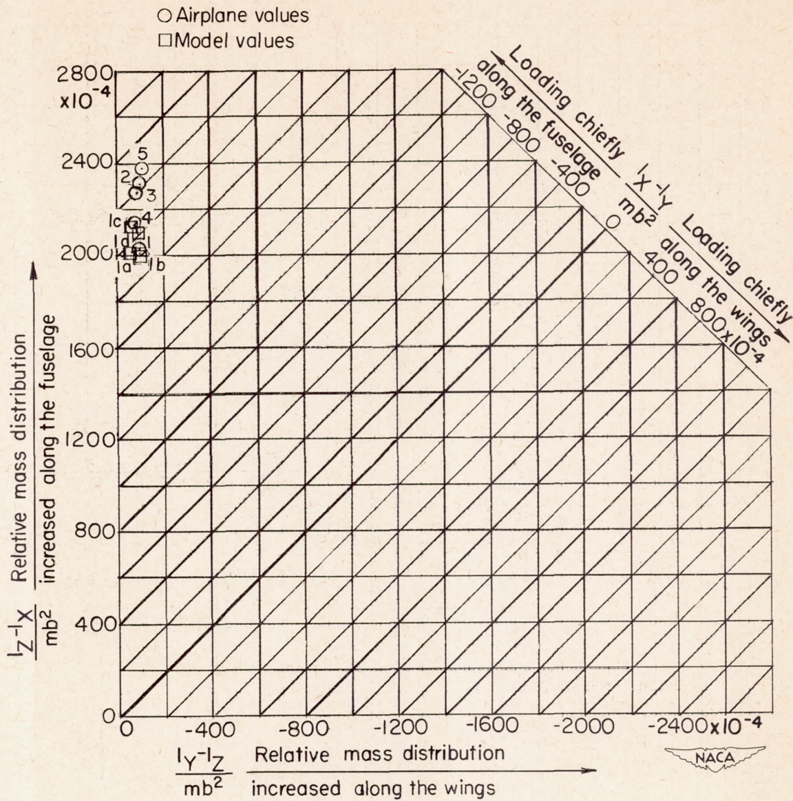
Figure 5.- Mass parameter plot for the various airplane loading conditions and for the conditions tested on the model as tabulated in table II.
