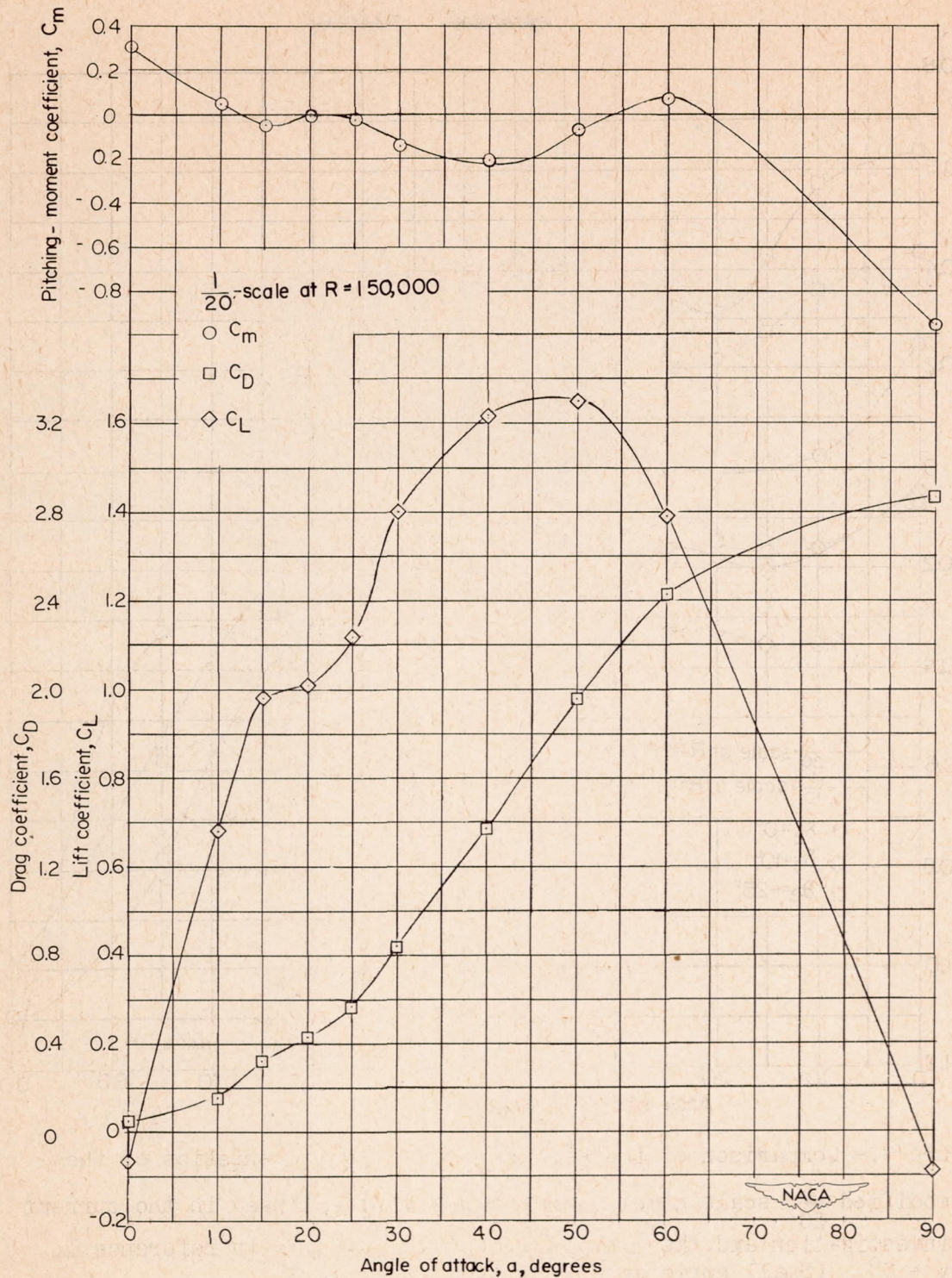
Figure 8.- Aerodynamic characteristics of the unmodified \frac{1}{20} -scale model with large horizontal tail installed. \psi = 0^\circ . \delta_e = 0^\circ .
