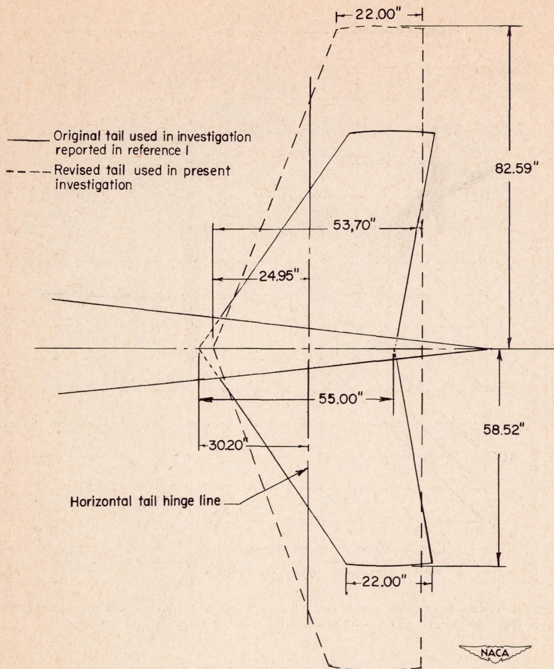
Figure 4.- Comparison of small horizontal tail used in the investigation of reference 1 and the horizontal tail used for the present dynamic tests. Dimensions are full scale.
