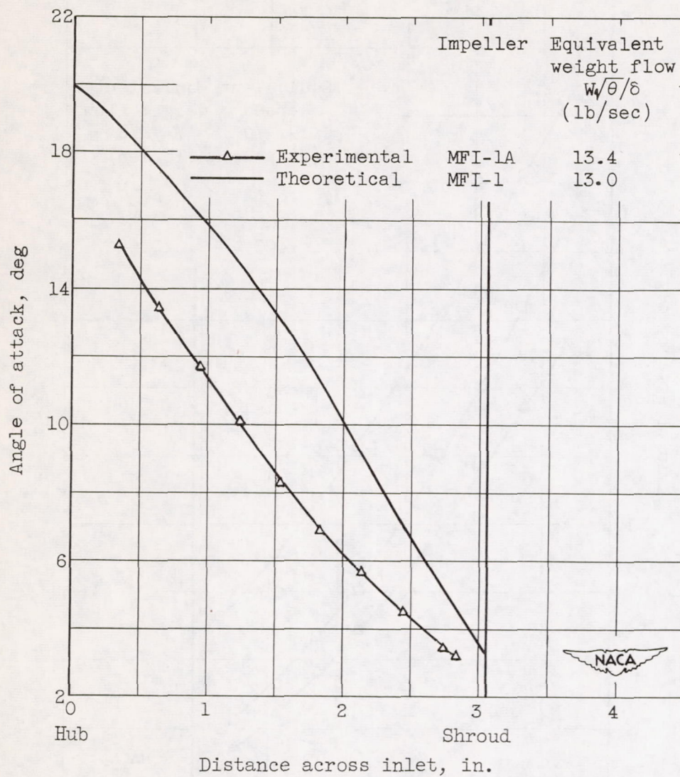
Figure 12. - Angle of attack at equivalent speed of 1400 feet per second.
