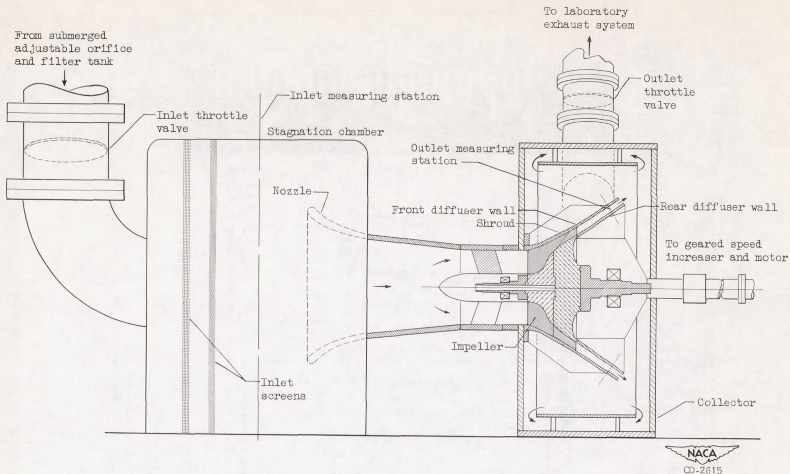
Figure 4. - Experimental setup used in investigation of 14-inch mixed-flow impeller.
