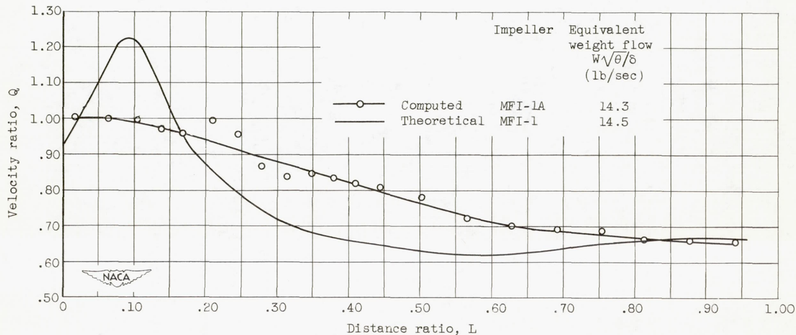
Figure 10. - Mean velocity distribution along shroud at equivalent speed of 1400 feet per second. Computed values are based on experimental static pressures.
