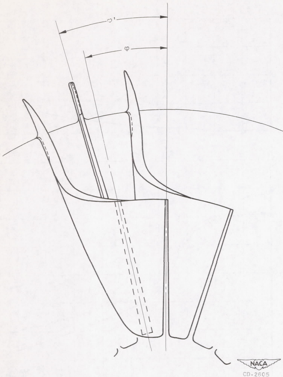
Figure 2. - Front view of MFI-1A impeller showing orientation of angles \varphi and \varphi' .
