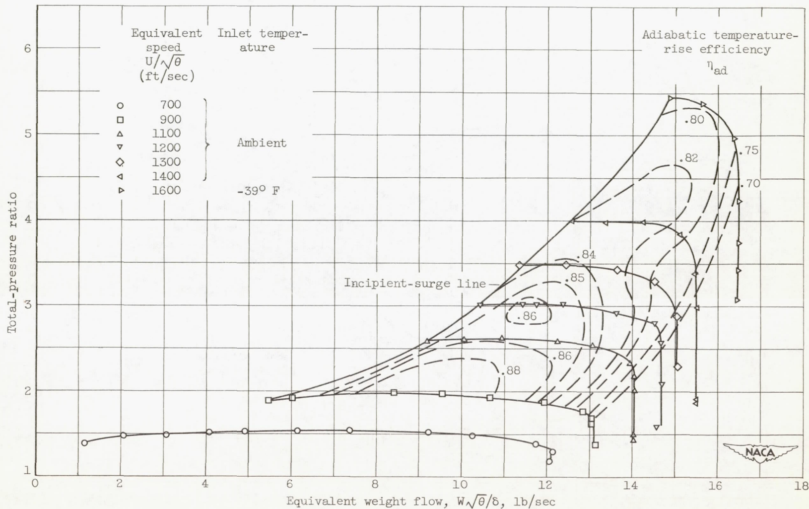
Figure 7. - Over-all performance characteristics of MFI-1A impeller at inlet air pressure of 14 inches of mercury absolute. Ambient inlet air temperature varied from 77^\circ to 82^\circ\text{F} .
