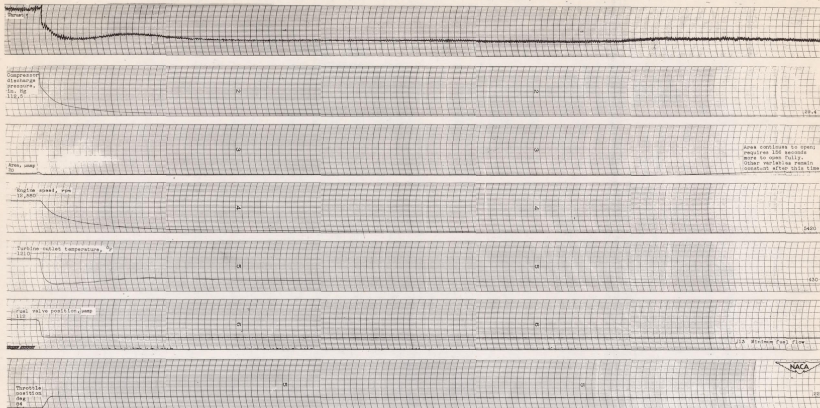
Figure 6. - Continued. Transient operation of automatically controlled engine at a nominal ram pressure ratio of 1.2.
