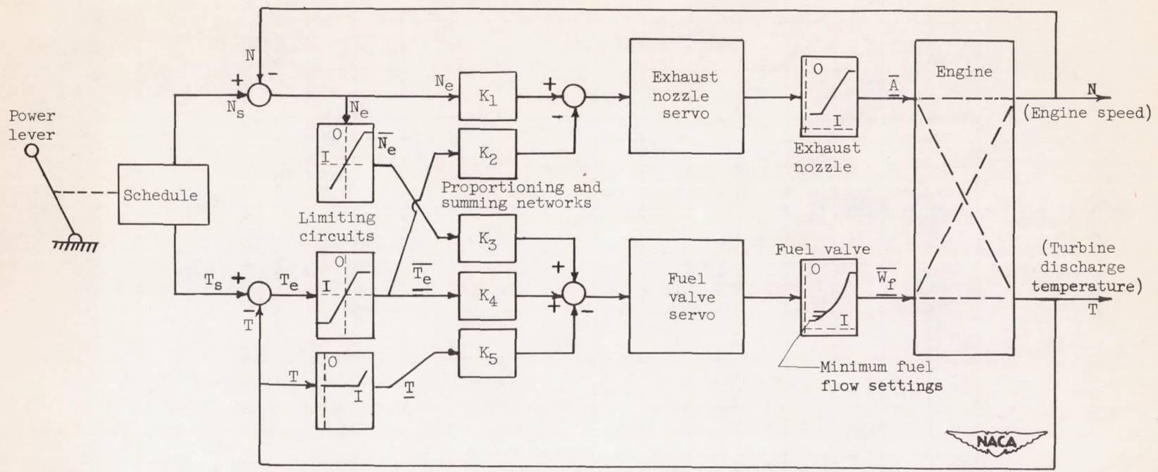
Figure 1. - Block diagram of Westinghouse J34-WE-32 primary control system.
