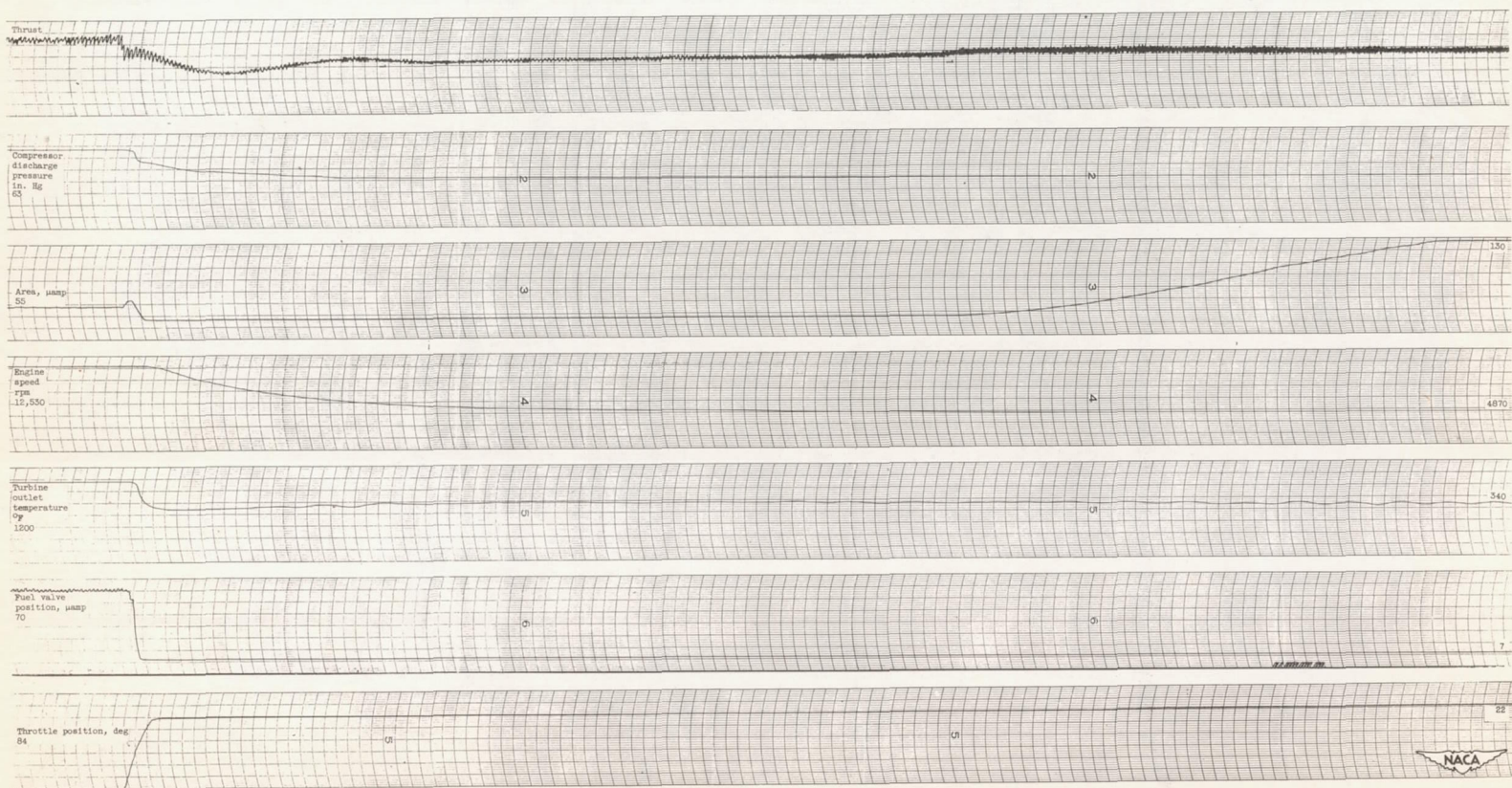
Figure 6. - Continued. Transient operation of automatically controlled engine at a nominal ram pressure ratio of 1.2.
