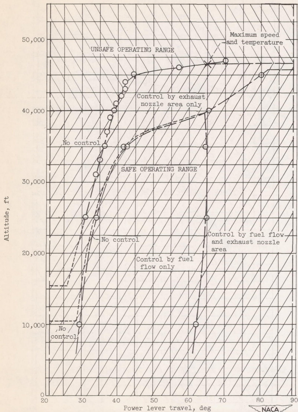
Figure 4. - Effect of altitude and power lever position on safe and unsafe operating ranges of controlled engine and on type of control existing in safe operating range. Minimum fuel flow, 550 pounds per hour; ram pressure ratio, 1.2.
