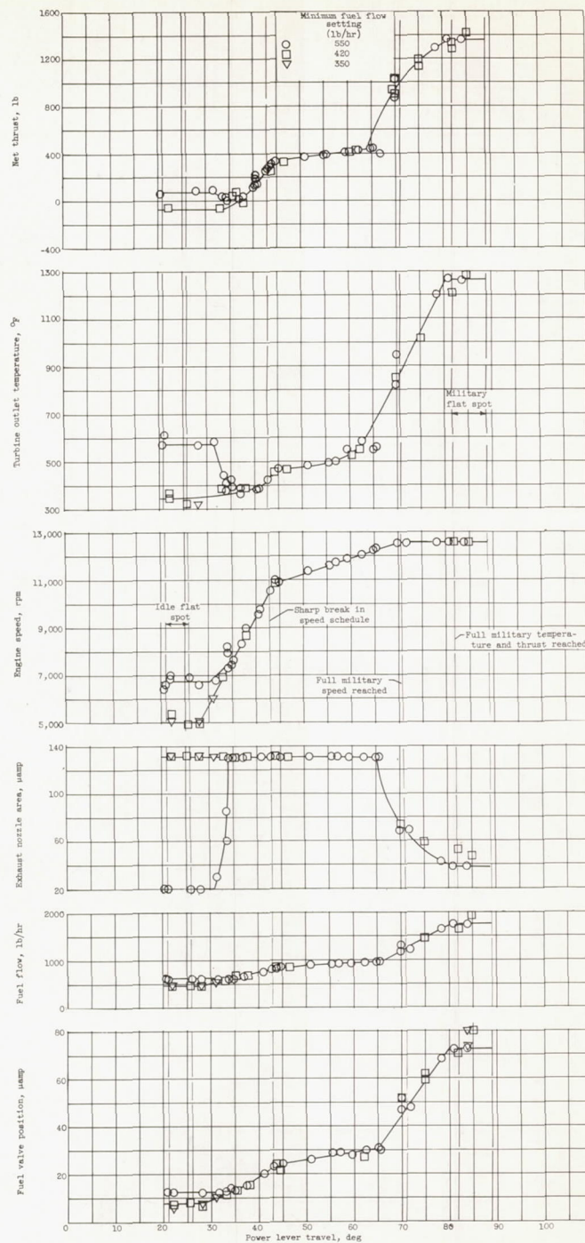
Figure 3. - Continued. Variation of net thrust, turbine outlet temperature, engine speed, exhaust nozzle area, fuel flow, and fuel valve position with power lever travel for different values of minimum fuel flow setting. Ram pressure ratio, 1.2.
