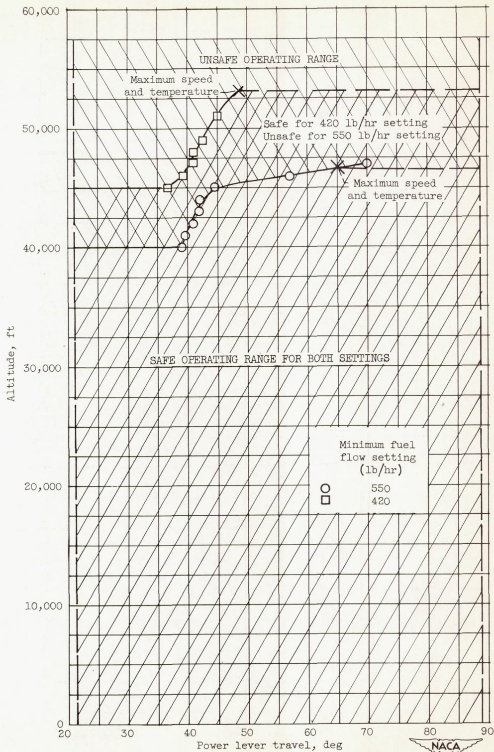
Figure 5. - Power lever travel for controlled engine showing safe and unsafe operating ranges as a function of altitude with different minimum fuel flow settings. Ram pressure ratio, 1.2.
