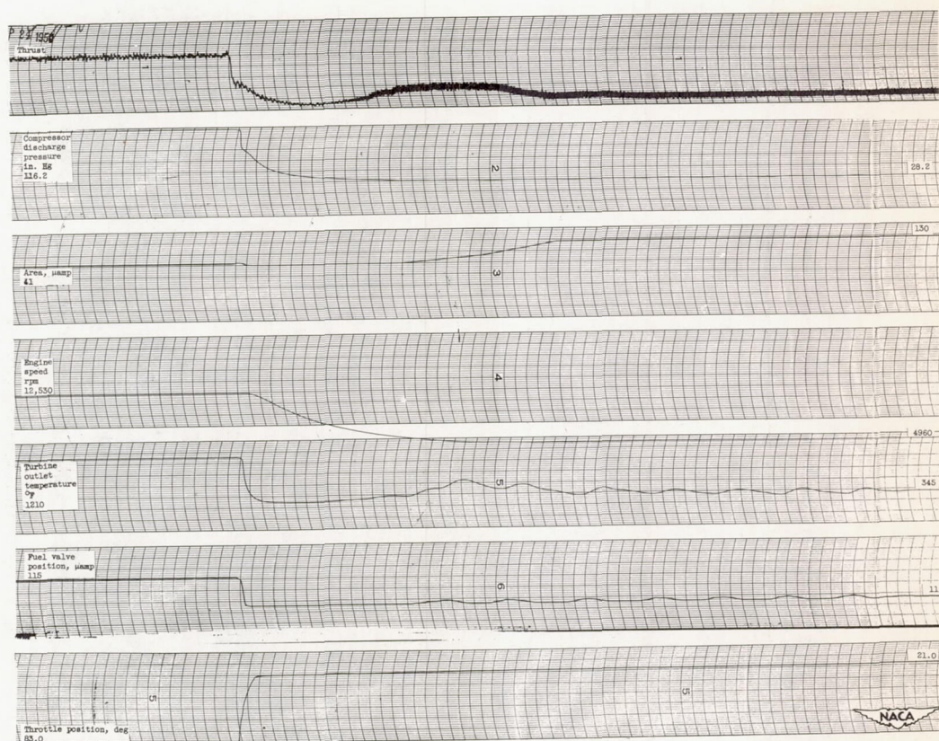
Figure 6. - Continued. Transient operation of automatically controlled engine at a nominal ram pressure ratio of 1.2.
