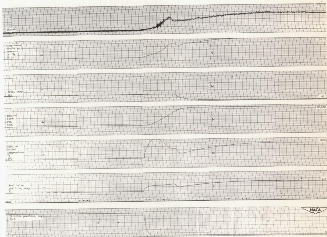
Figure 6. - Continued. Transient operation of automatically controlled engine at a nominal ram pressure ratio of 1.2.
