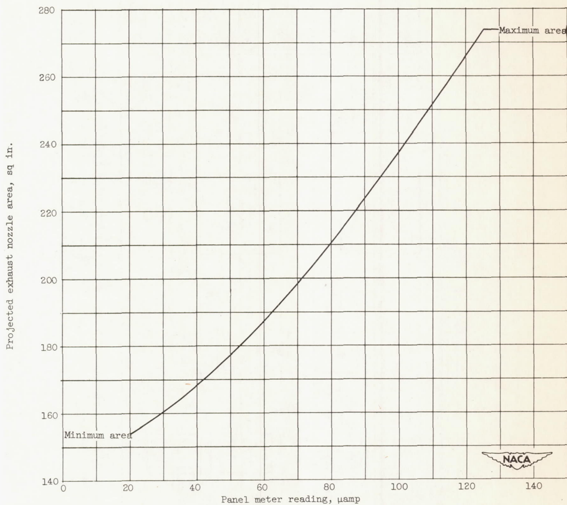
Figure 2. - Calibration of Westinghouse variable-area nozzle for J34-WE-32 turbojet engine.
