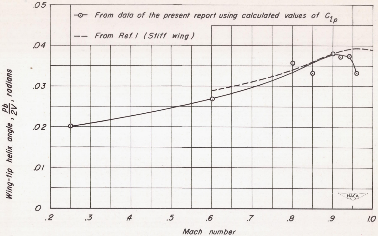
Figure 16.— Variation with Mach number of wing-tip helix angle due to projection of the perforated spoiler. \alpha = 0^\circ , R = 1,500,000 .
