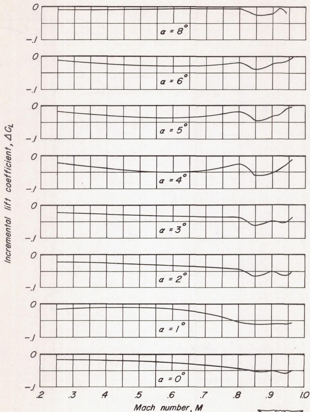
Figure 12.-Variation with Mach number of incremental lift coefficient for a model with a perforated spoiler. R = 1,500,000 .
