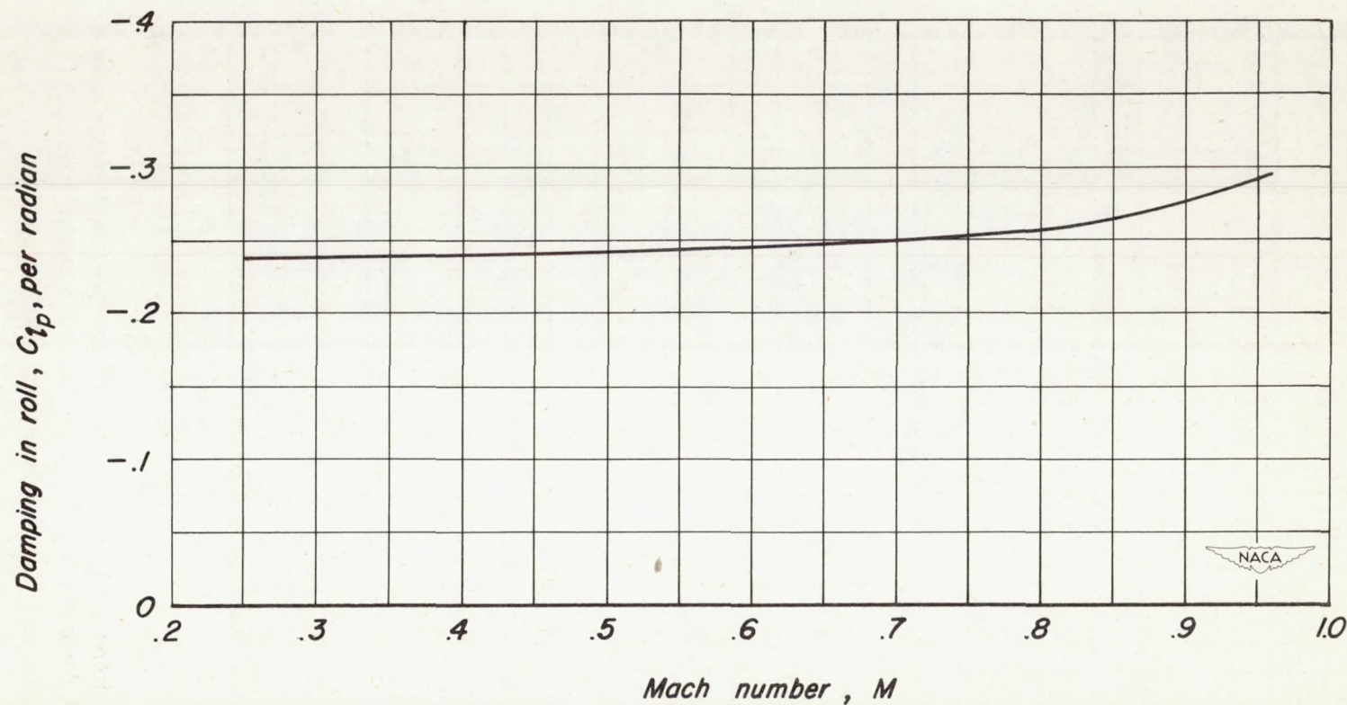
Figure 15.— Variation with Mach number of the calculated damping in roll for a wing of aspect ratio 3 and having 45^\circ of sweepback. \alpha = 0^\circ .
