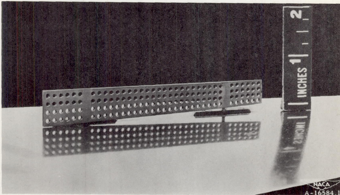
(b) Front and close-up views of spoiler.
