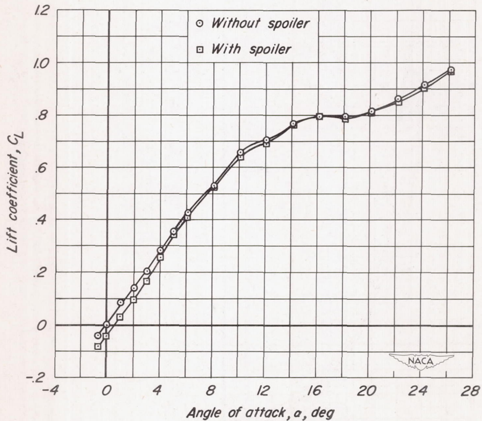
Figure 5.— The aerodynamic characteristics at a Mach number of 0.80. R=1,500,000 .
