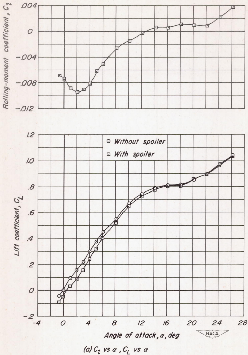
Figure 6.—The aerodynamic characteristics at a Mach number of 0.85. R = 1,500,000 .
