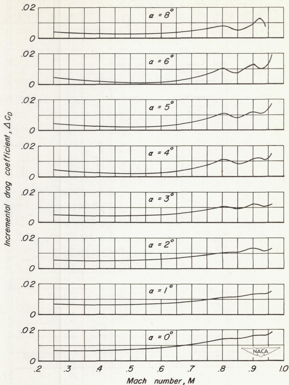
Figure 13.-Variation with Mach number of incremental drag coefficient for a model with a perforated spoiler. R = 1,500,000 .
