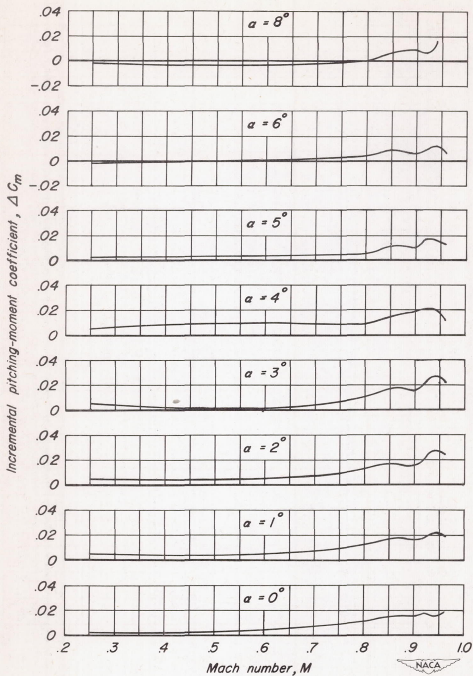
Figure 14.—Variation with Mach number of incremental pitching-moment coefficient for a model with a perforated spoiler. R=1,500,000 .
