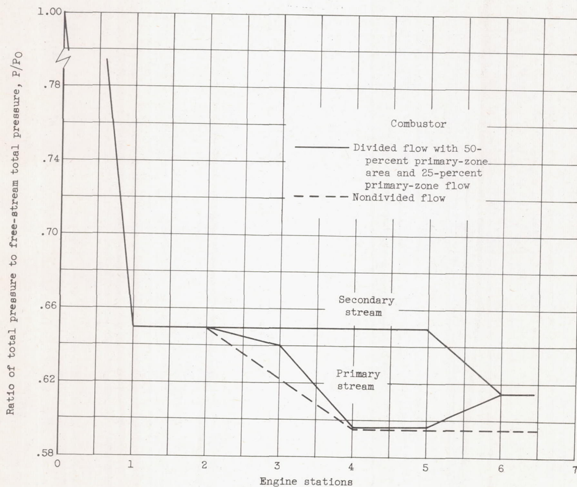
Figure 2. - Variations in total-pressure ratio through analytical model engine. Free-stream Mach number, 3.0; diffuser efficiency, 65 percent; combustor-inlet Mach number, 0.18; over-all combustor total-temperature ratio, 1.875.
