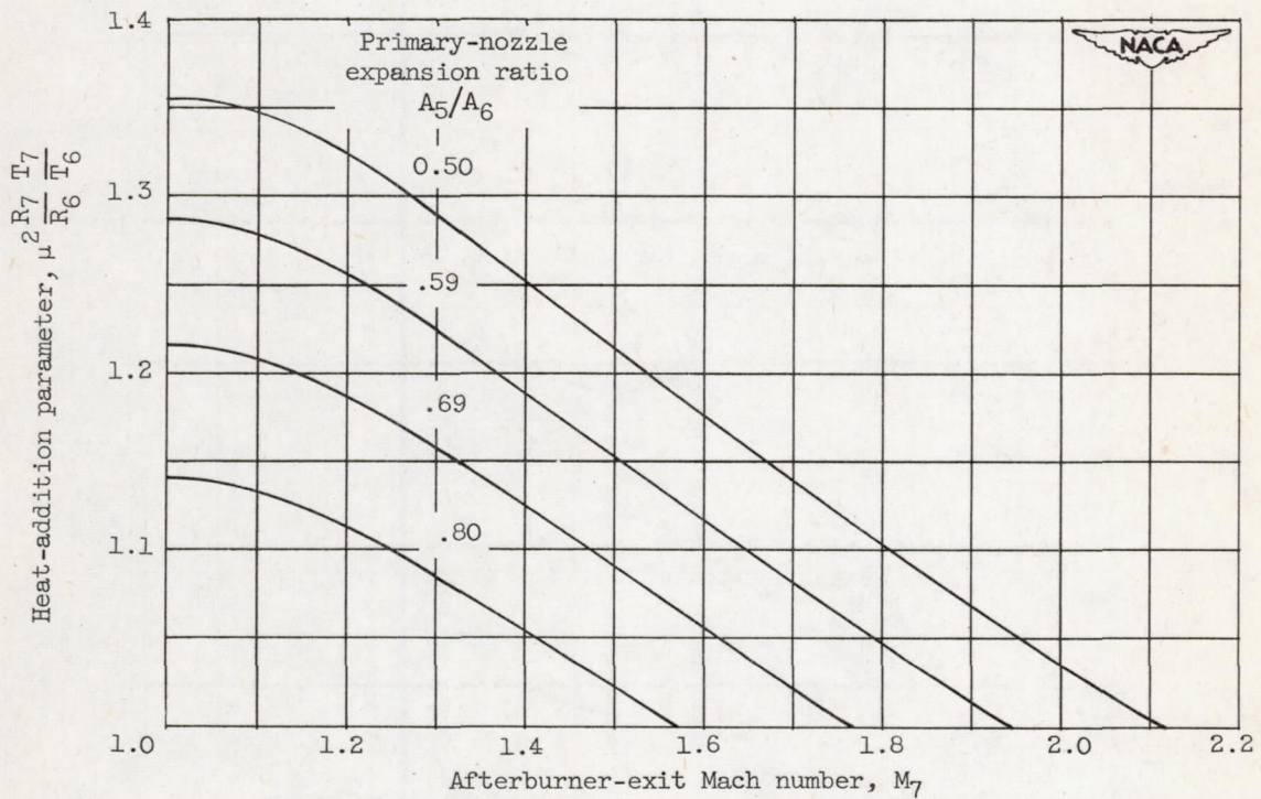
(a) Effect of primary-nozzle-expansion ratio and afterburner-exit Mach number on heat-addition parameter. Initial transition region.
