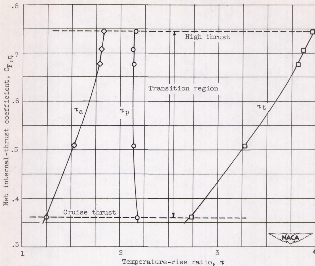
Figure 8. - Variation of net internal-thrust coefficient with total and component temperature-rise ratios. Free-stream Mach number M_0 , 2.0; diffuser-exit Mach number M_3 , 0.219 \pm 0.006 ; transition region primary fuel-air ratio, 0.038.
