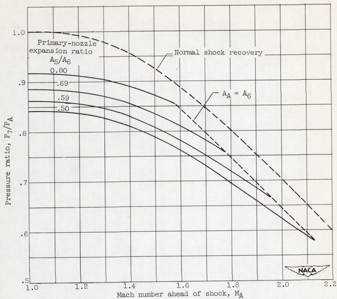
(c) Effect of primary-nozzle-expansion ratio and Mach number ahead of normal shock on total-pressure ratio across the afterburner. Transition region. M_5 = 1 ; M_7 = 1 ; T_5 = T_6 ; \gamma = 1.3 .
