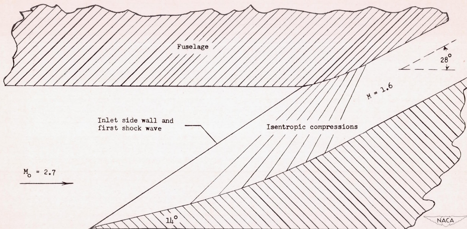
Figure 15.- Proposed modification of design flow pattern for swept, rectangular scoop inlet.
