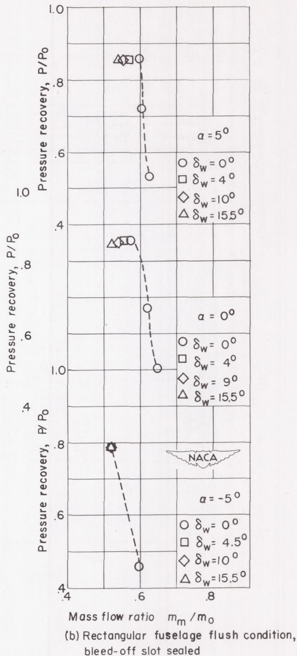
Figure 19.- Variation of pressure recovery with mass-flow ratio for various wedge deflections and angles of attack. M_0 = 2.03 .
