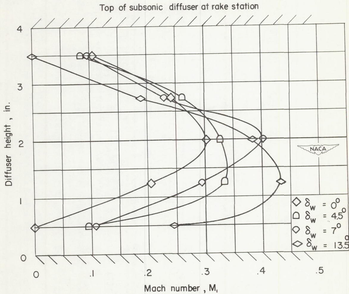
Figure 23.- Mach number distribution at the rake station in the subsonic diffuser. \alpha = 0^\circ ; M_0 = 2.03 .
