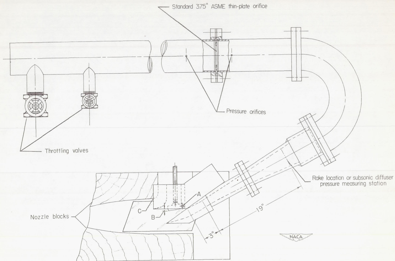
Figure 6.- Schematic drawing of test installation.
