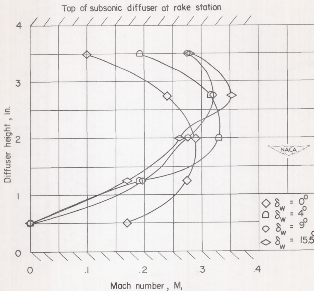
(b) Rectangular fuselage, flush condition, bleed-off slot sealed.
