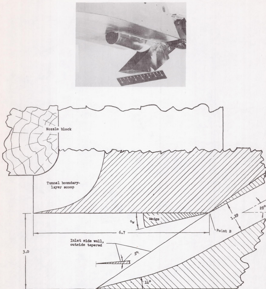
Figure 5.- Details of model with circular fuselage. L-76080
