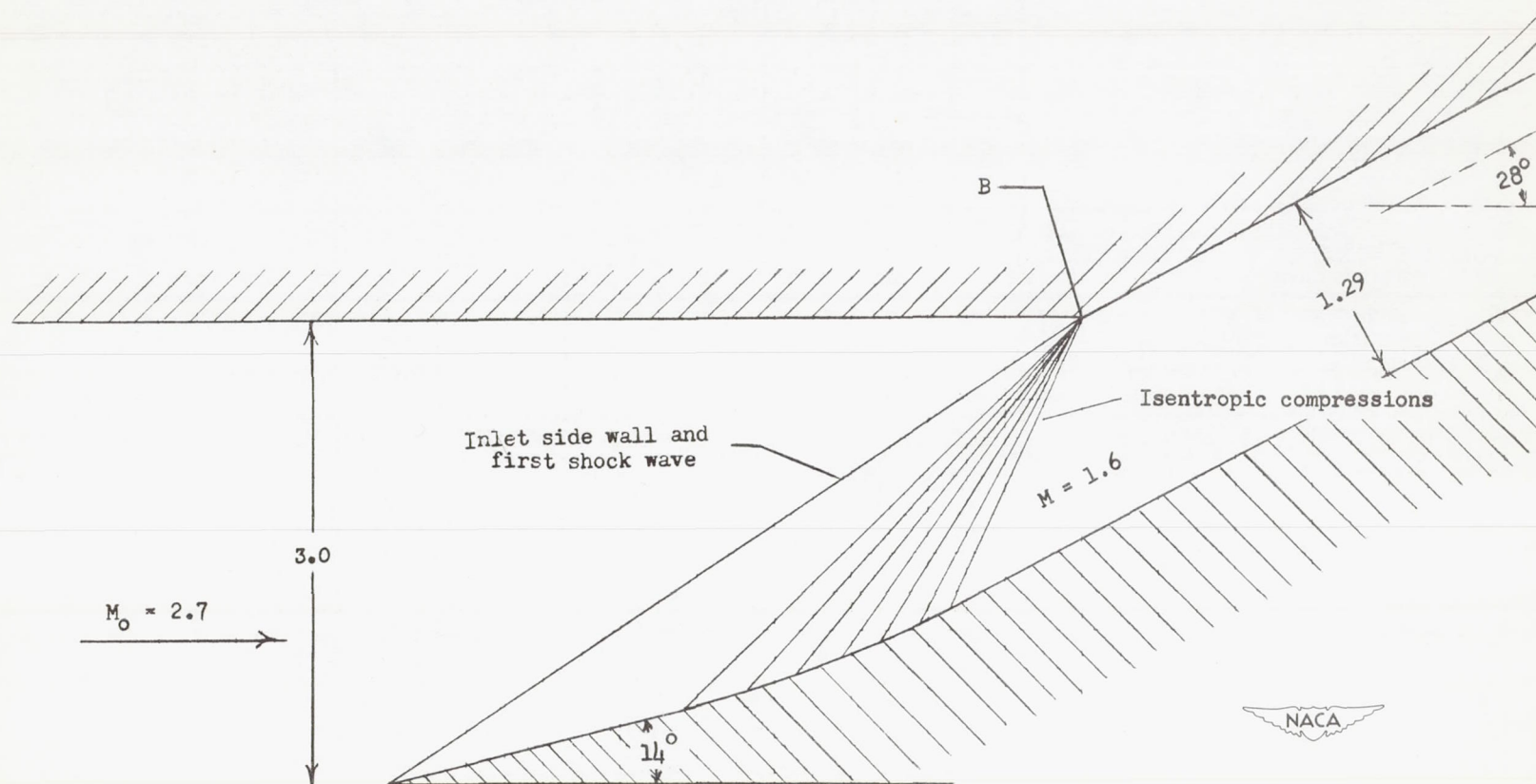
Figure 3.- Design flow pattern for swept, rectangular scoop inlet.
