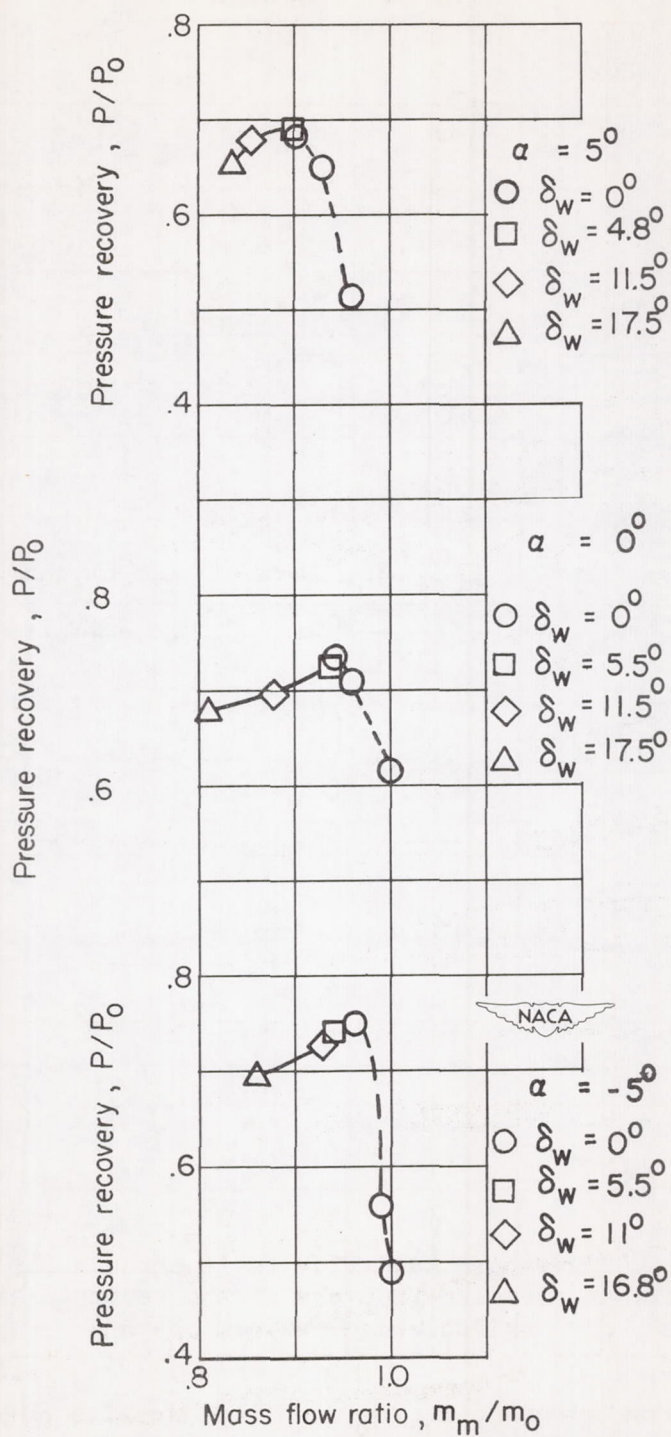
(e) Rectangular fuselage, offset condition, bleed-off slot open to atmospheric pressure.
