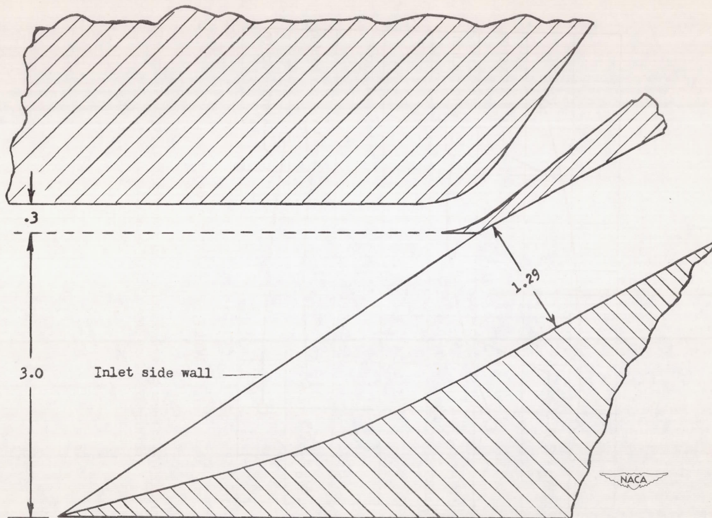
Figure 26.- Proposed modification of inlet to aid starting.
