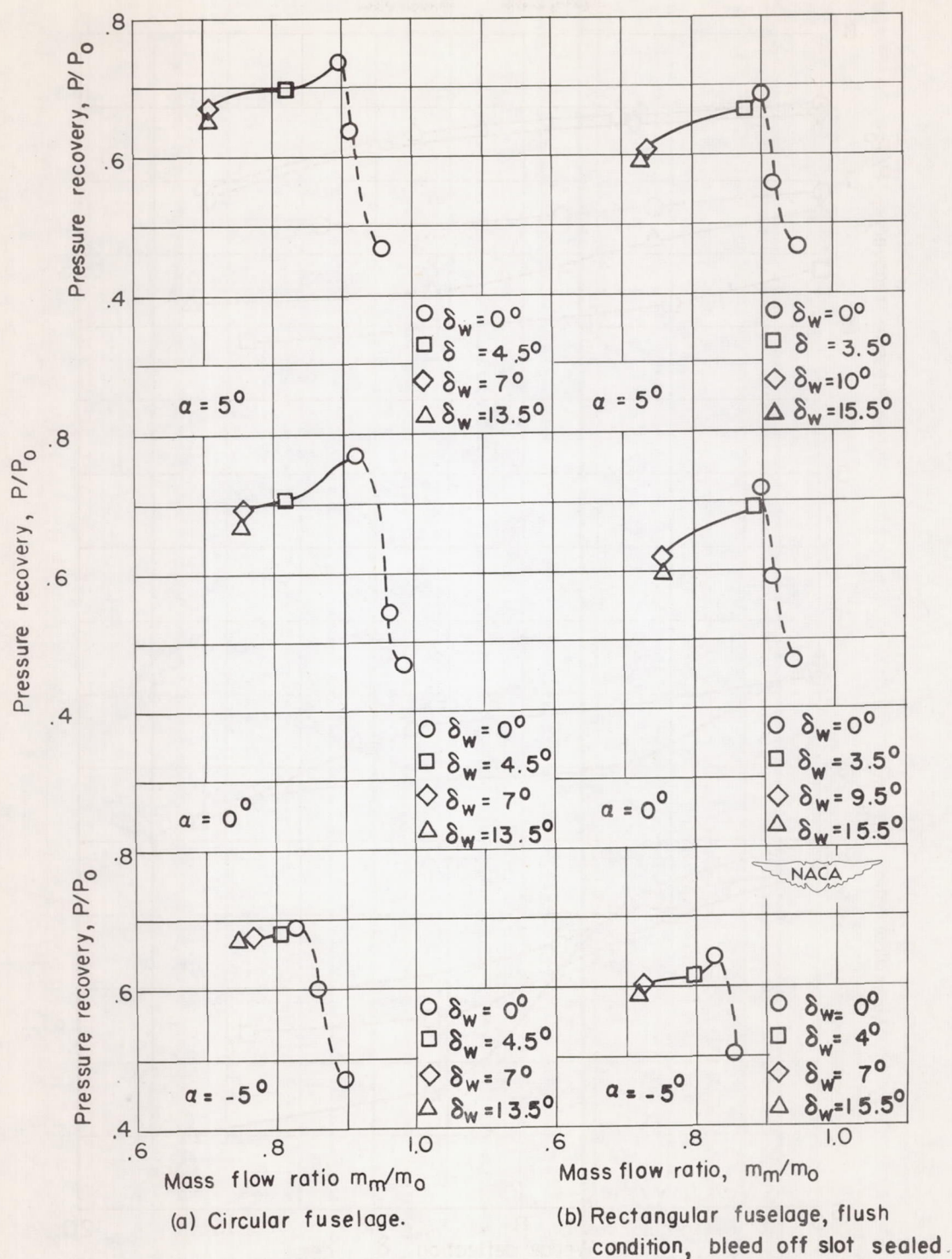
Figure 21.- Variation of pressure recovery with mass-flow ratio for various wedge deflections and angles of attack. M_0 = 2.71 .
