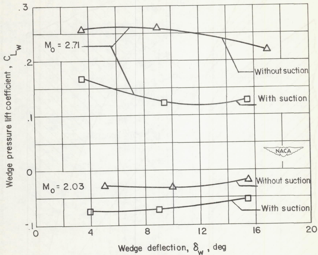
Figure 25.- Effect of wedge deflection on wedge lift coefficient, rectangular fuselage, flush condition. \alpha = 0^\circ .
