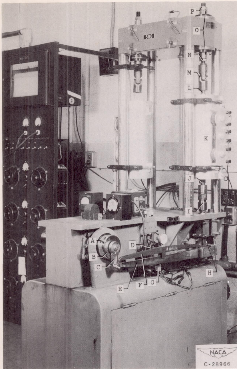
Figure 3. - Fatigue machine modified for testing at elevated temperatures.
