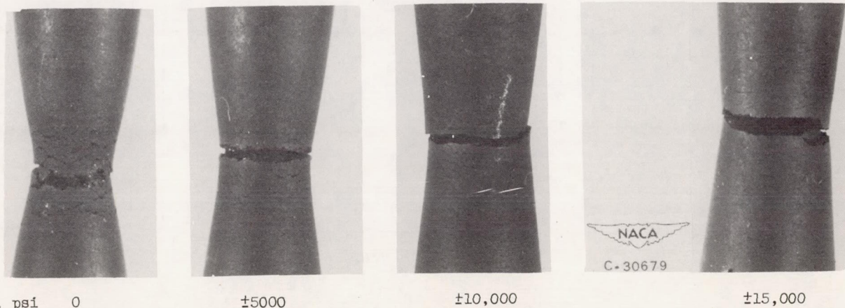
(b) Round cross-sectional specimens; X3.87
