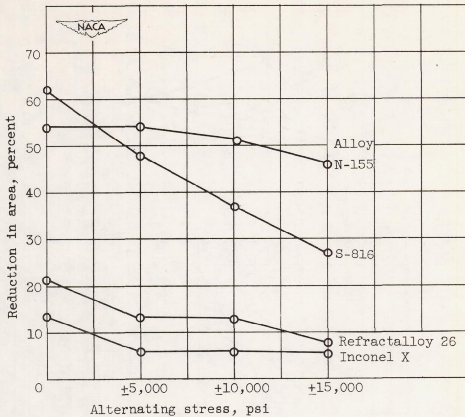
Figure 7. - Effect of alternating stress on reduction of area of fractured specimens.
