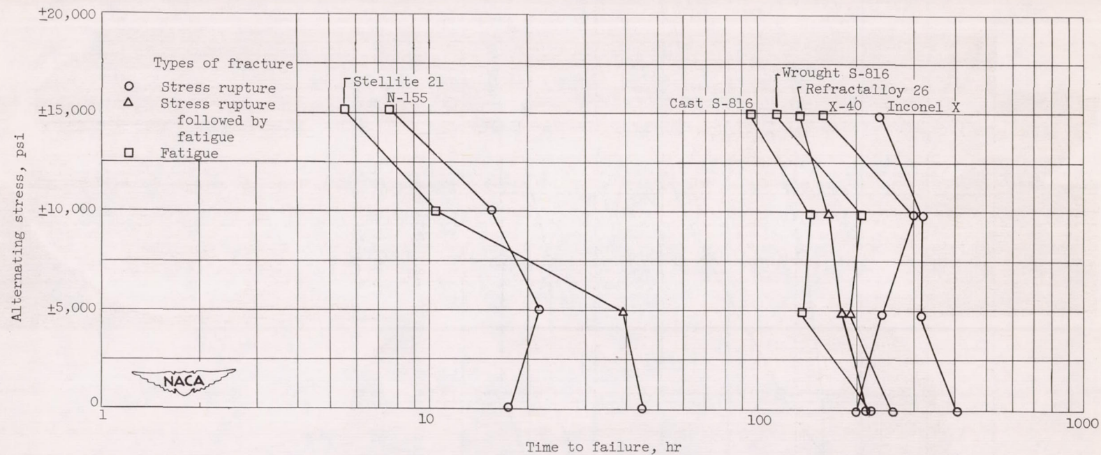
Figure 6. - Effect of alternating stress on type of fracture and time to failure. Temperature, 1500° F; mean stress, 22,000 pounds per square inch.
