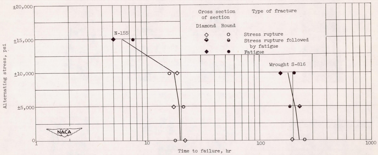
Figure 8. - Effect of specimen shape on time to failure. Temperature, 1500° F; mean stress, 22,000 pounds per square inch.
