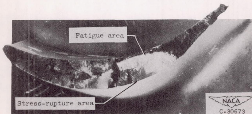
(c) Stress rupture followed by fatigue fracture.
