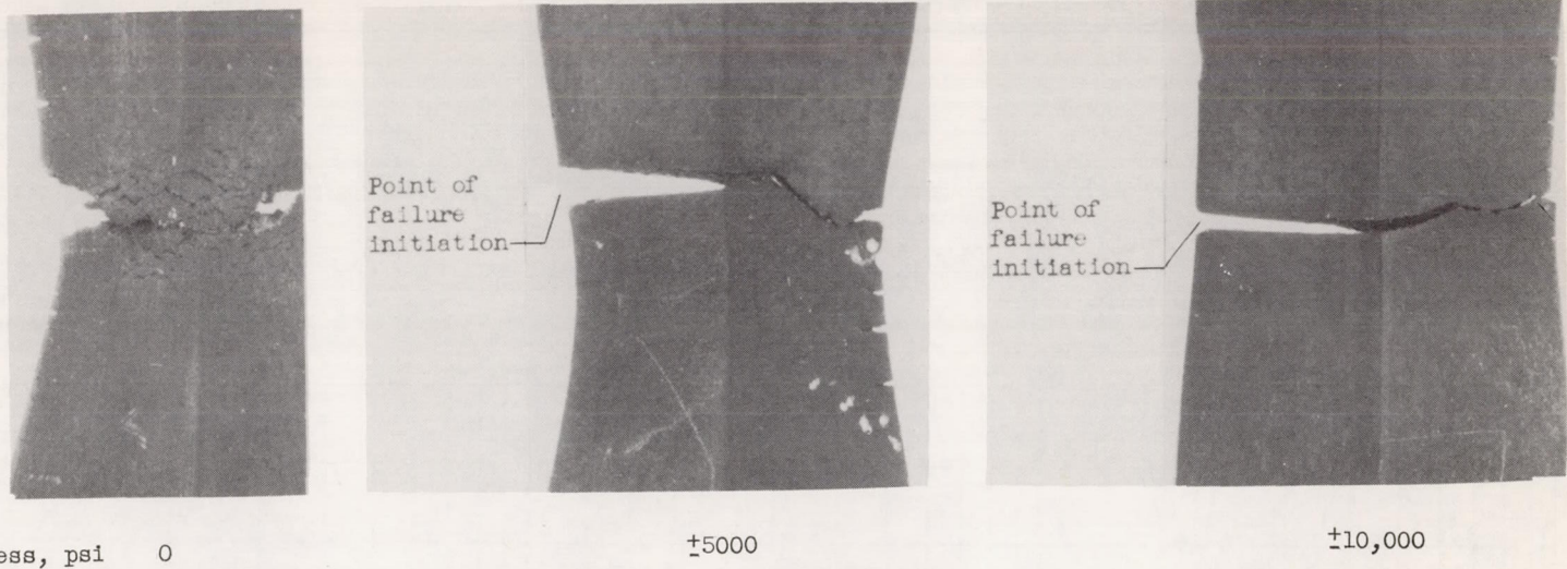
(a) Diamond cross-sectional specimens; X3.75
