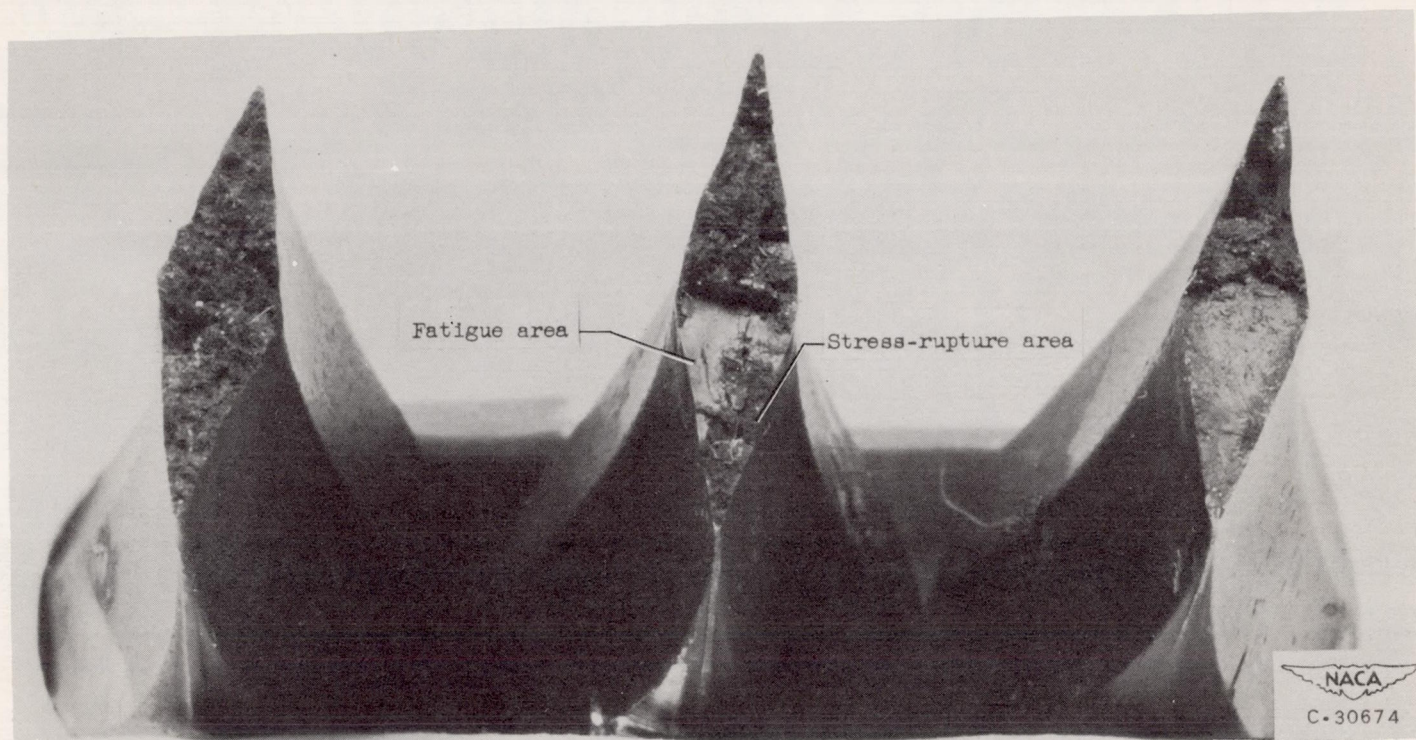
(c) Fatigue.
