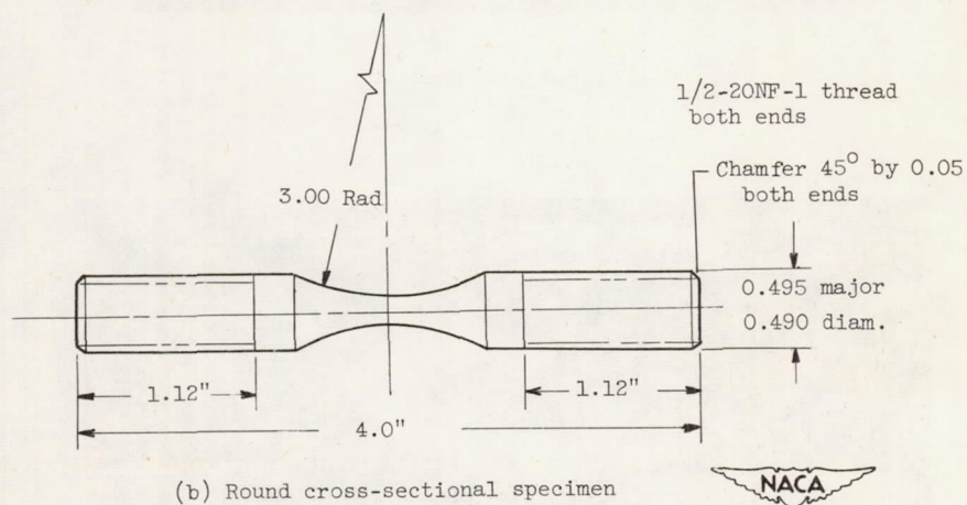
Figure 2. - Fatigue specimens used.
