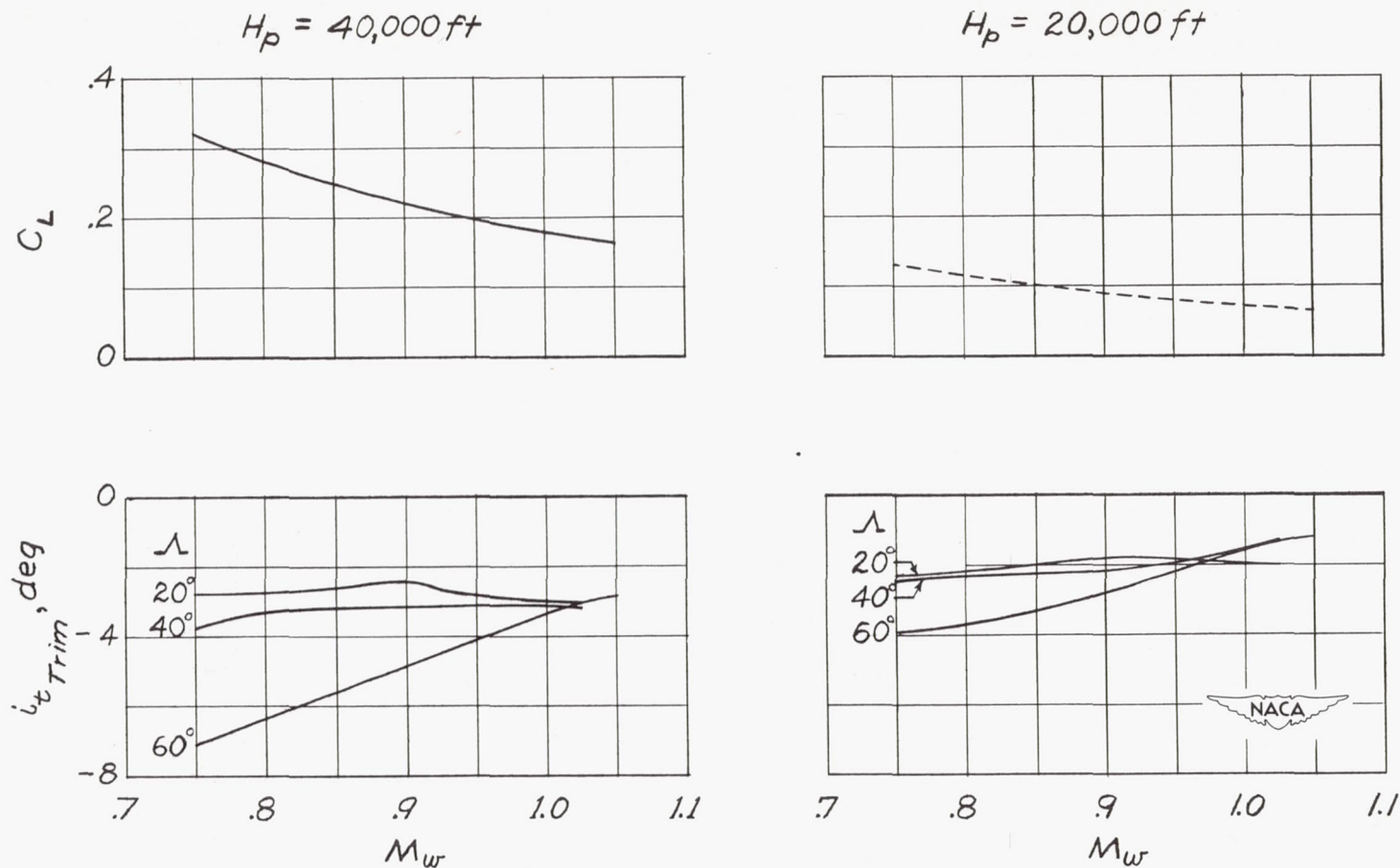
Figure 17.- Variation with Mach number of stabilizer angle required for trim in level flight at altitudes of 20,000 and 40,000 feet with wing loading of 50 and center of gravity located at 26 percent mean aerodynamic chord of 60^\circ sweptback wing and at 35 percent mean aerodynamic chord of the 40^\circ and 20^\circ sweptback wings. Lift coefficient for level flight also shown.
