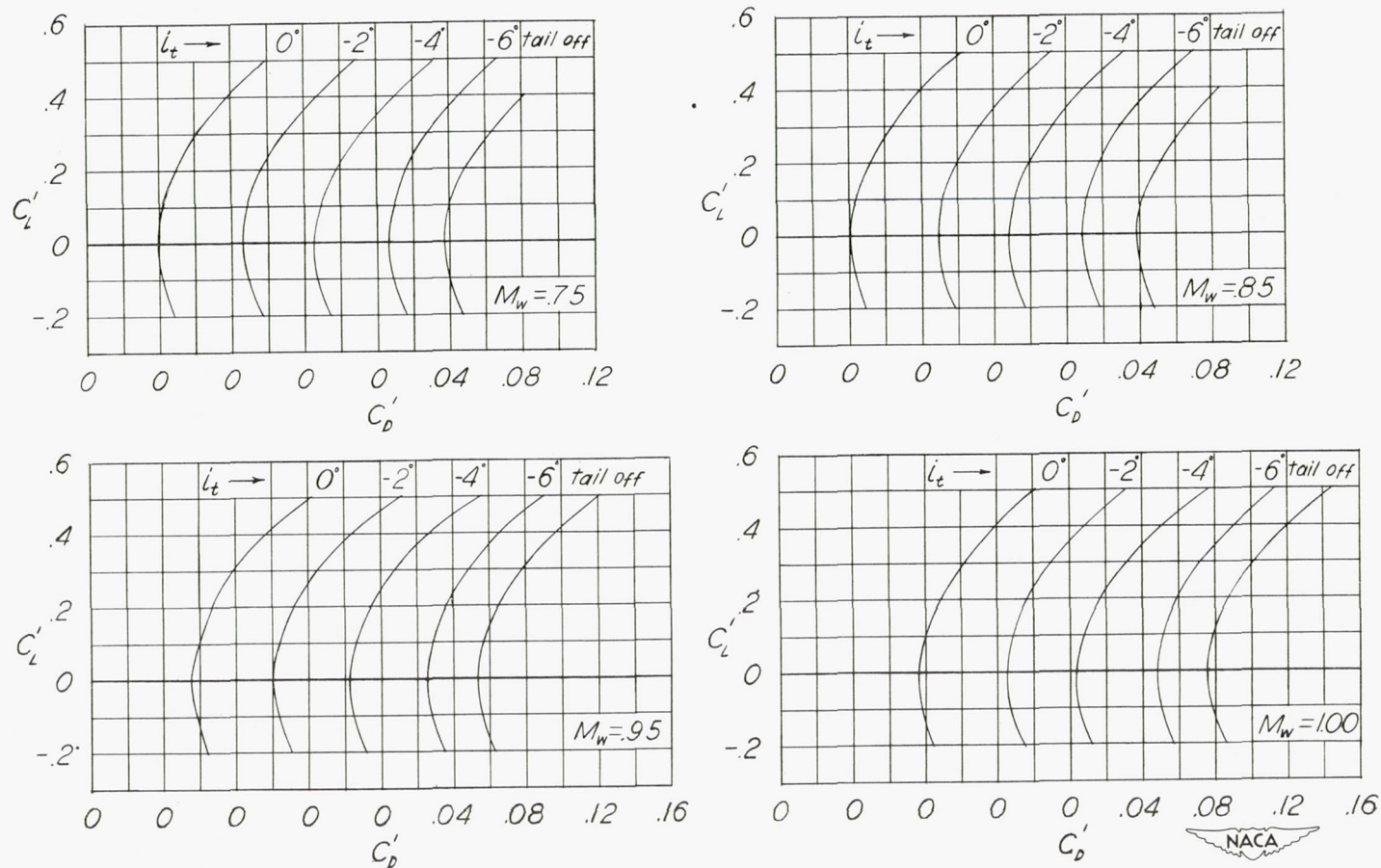
Figure 12.- Variation of lift coefficient with drag coefficient for several tail incidences and wing sweepback angles at several Mach numbers for semispan model of Bell X-5 airplane. Results from reference 6 ( i_t = -2^\circ ) are also shown. (Coefficients based on 60^\circ sweptback-wing dimensions.)
