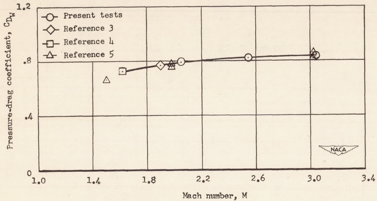
Figure 5.- Variation of pressure-drag coefficient with Mach number for a hemisphere.
