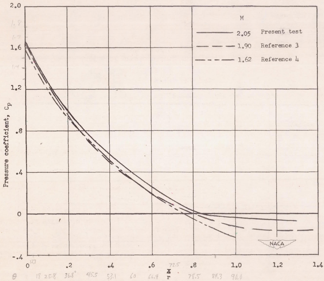
Figure 4.- Pressure distribution on a hemisphere for M = 2.05 test and references 3 and 4.
