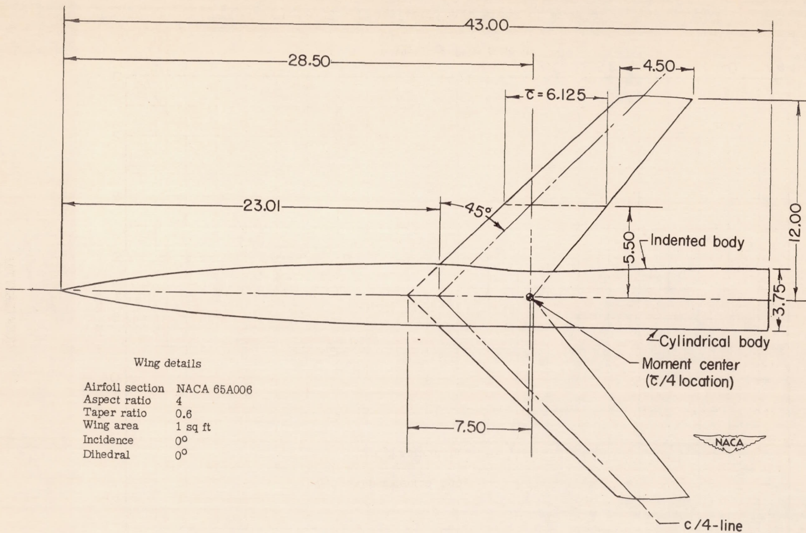
Figure 1.- Model details. All dimensions in inches.
