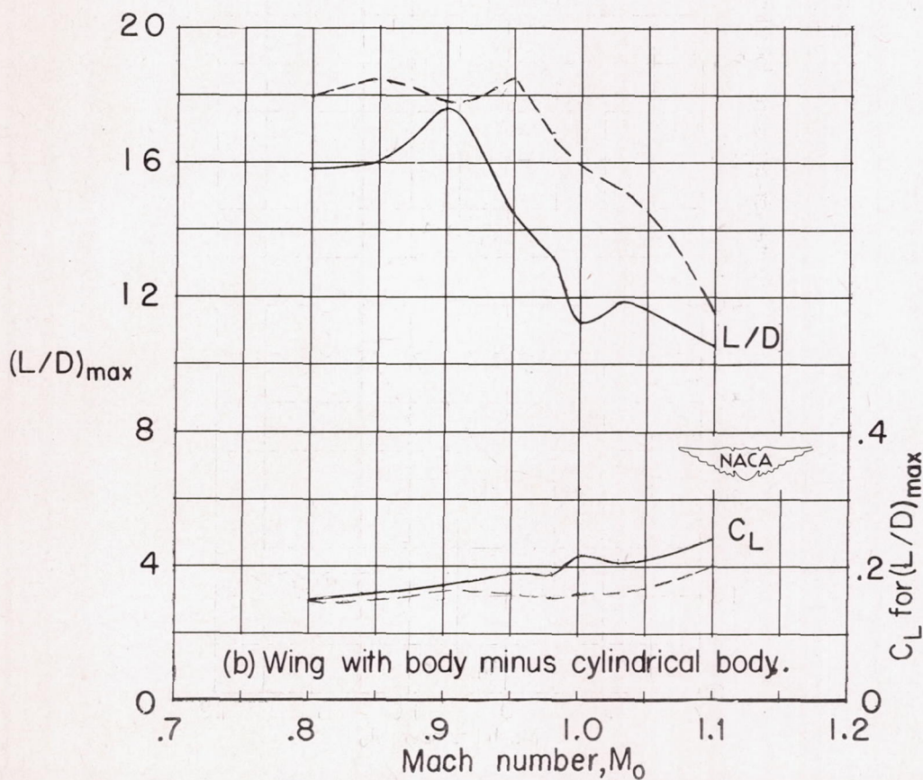
Figure 7.- Comparison of maximum lift-drag ratio and lift coefficient for maximum lift-drag ratio.
