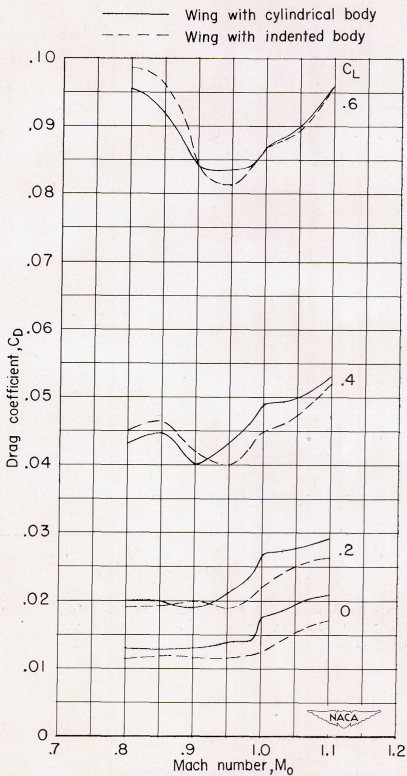
Figure 5.- Variation of drag coefficient with Mach number. Wing with body.
