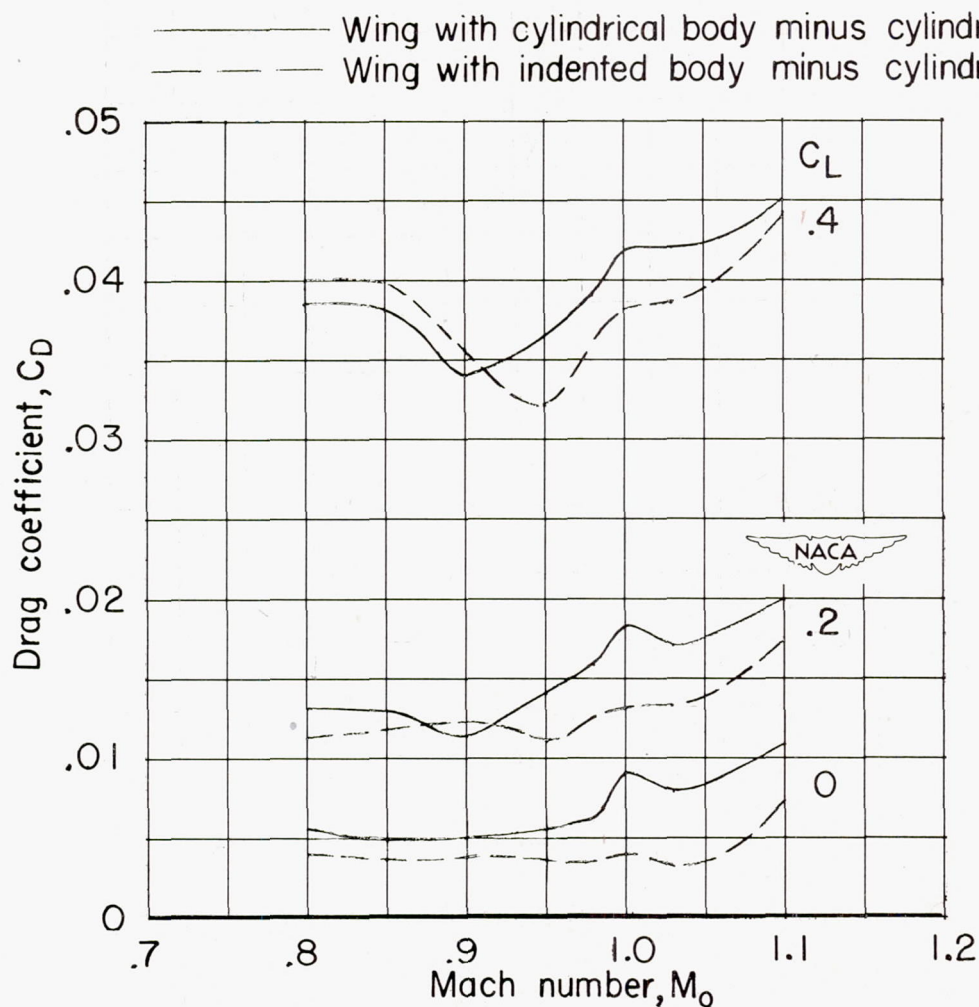
Figure 6.- Variation with Mach number of the wing with interference drag coefficient illustrating effect of body indentation on the transonic drag rise.
