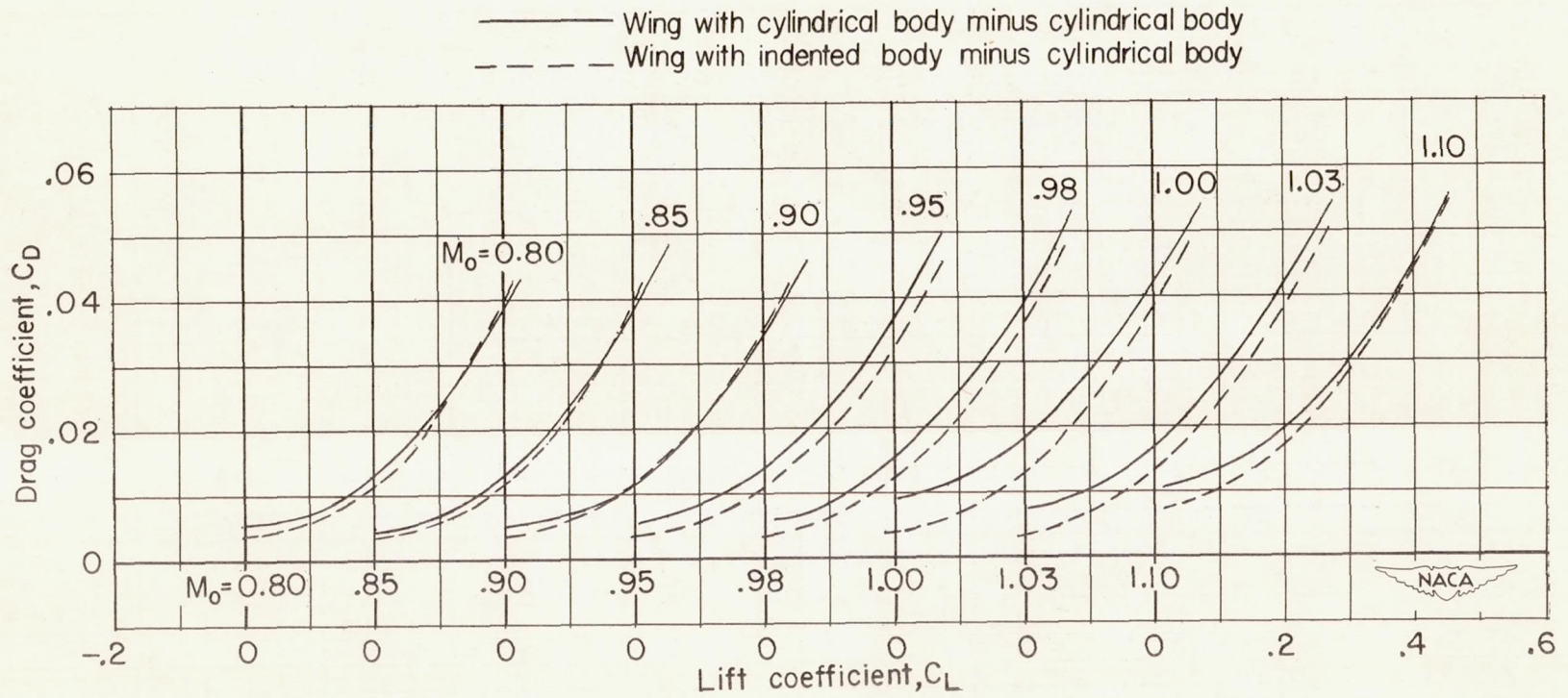
Figure 4.- Variation of drag coefficient with lift coefficient. Wing with interference.
