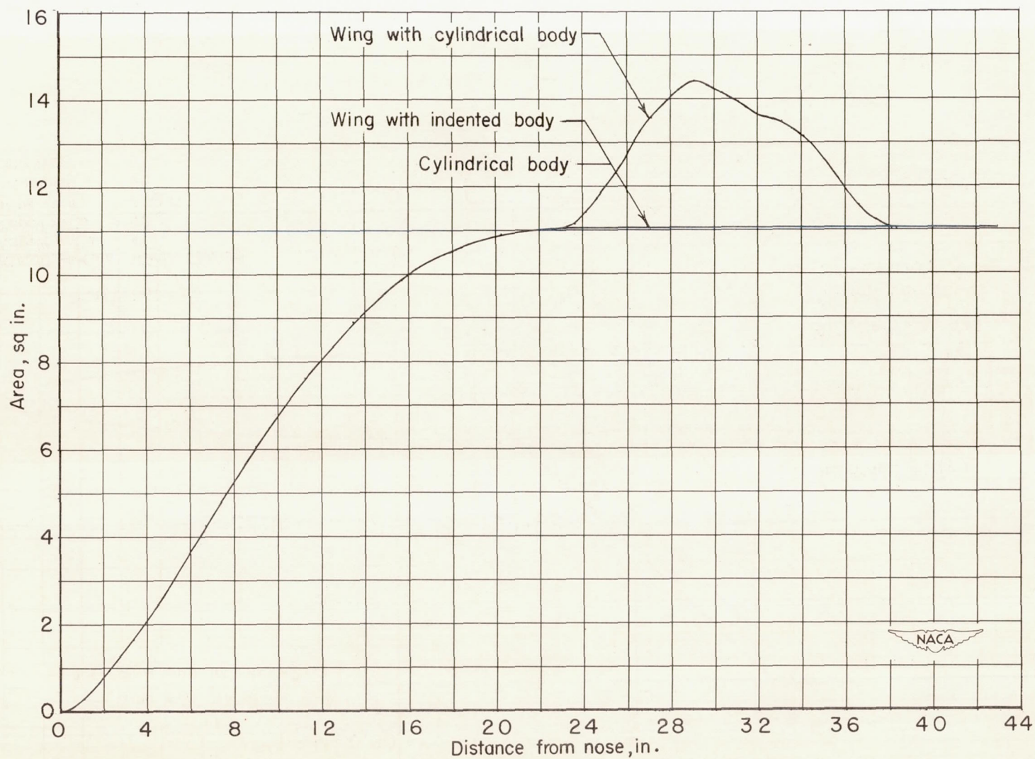
Figure 2.- Cross-sectional areas of models.
