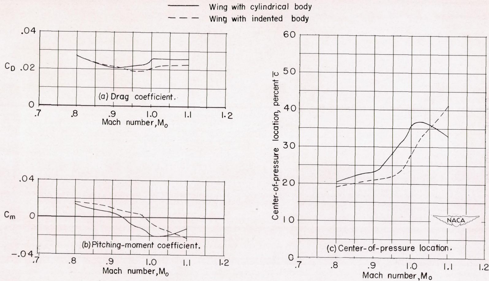
Figure 9.- Comparison of various performance parameters for level-flight condition at an altitude of 40,000 feet and a wing loading of 50 pounds per square foot.
