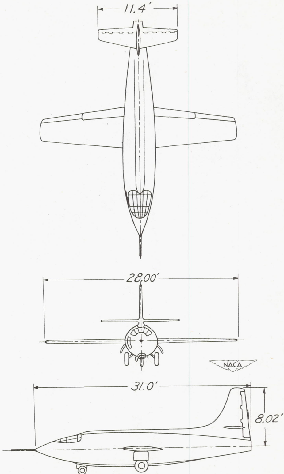
Figure 2.- Three-view drawing of Bell X-1 airplane.
