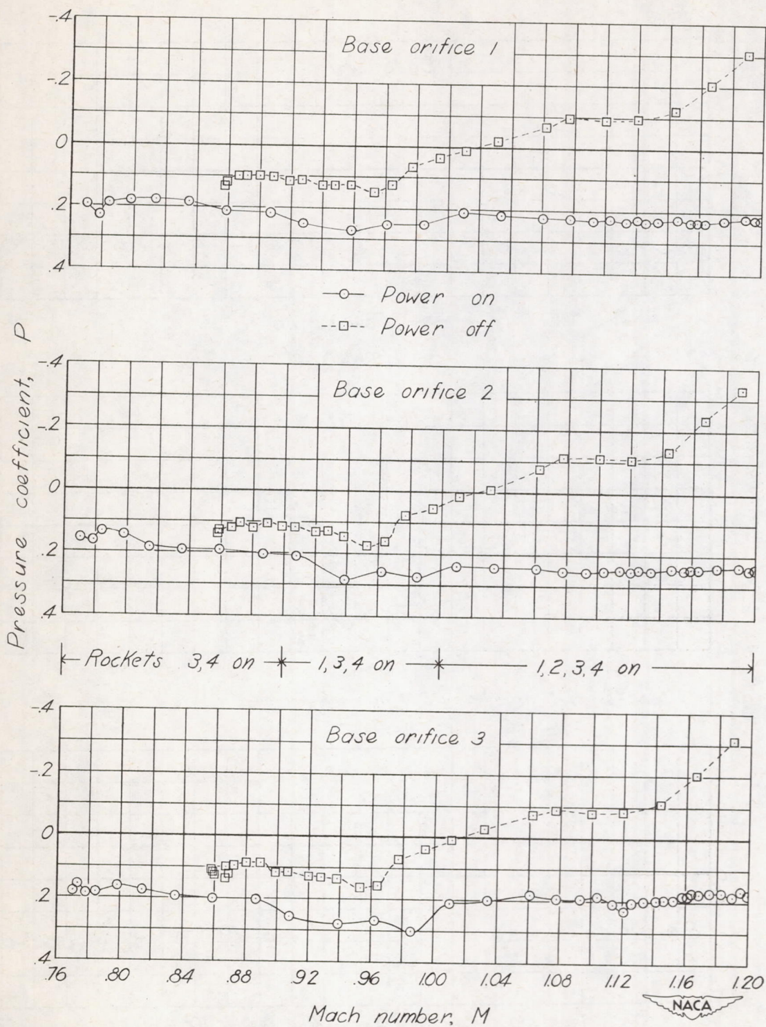
Figure 7.- Variation of pressure coefficient on fuselage base with Mach number in power-on and power-off flight on Bell X-1 airplane. C_{NA} \approx 0.4 .
