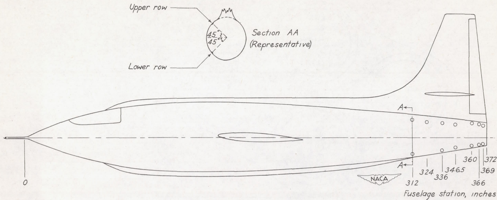
(a) Fuselage side near base.
