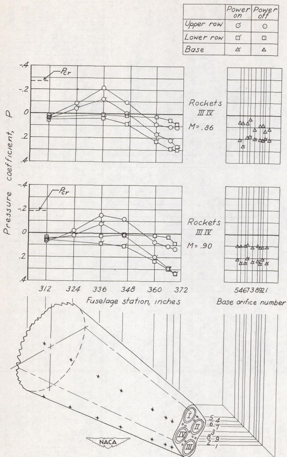
Figure 10.- Pressure distribution on and near fuselage base in power-on and power-off flight at various Mach numbers. C_{NA} \approx 0.4 .
