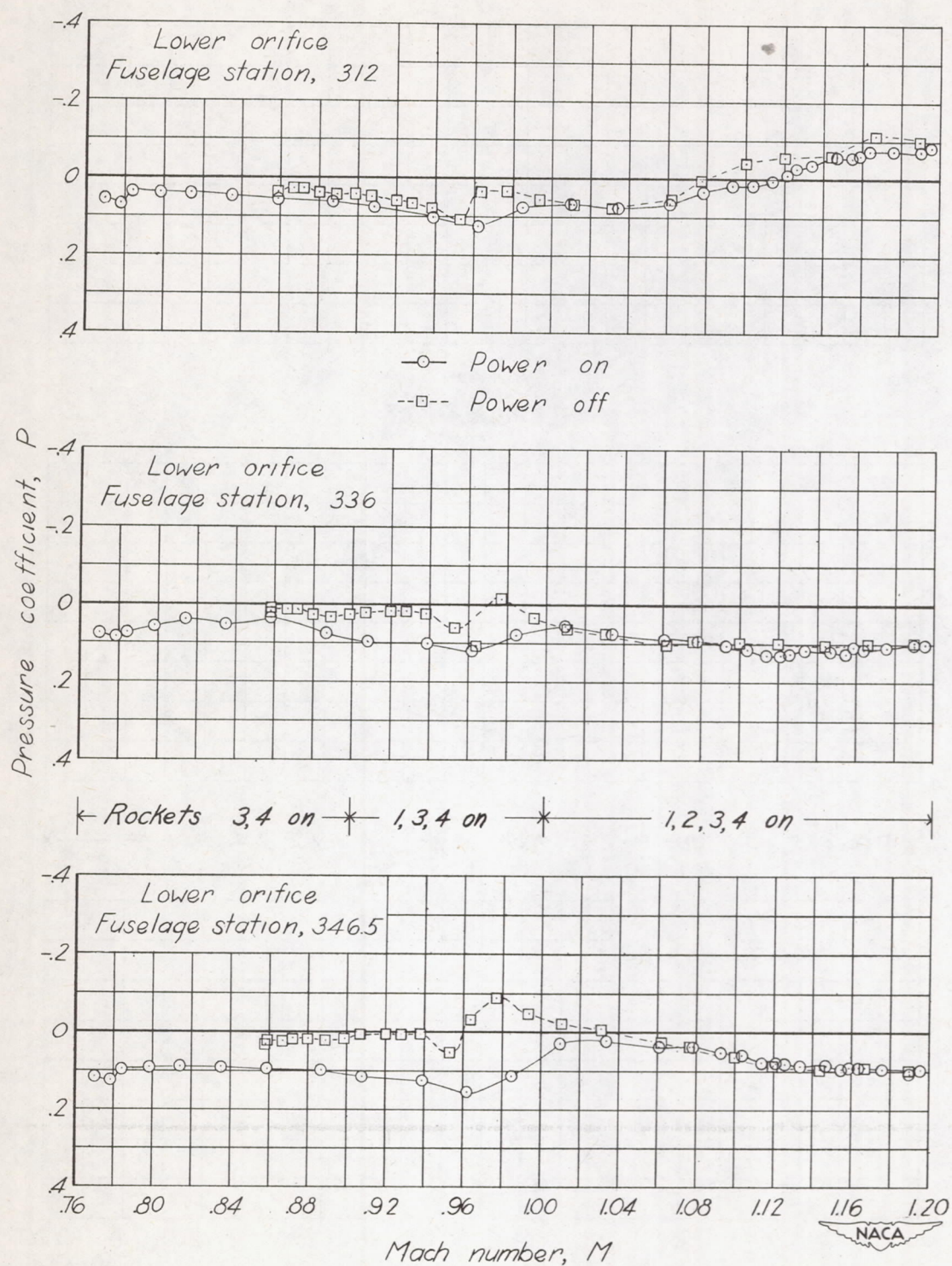
Figure 9.- Variation of pressure coefficient on fuselage side near base with Mach number in power-on and power-off flight of Bell X-1 airplane. Lower orifice row; C_{NA} \approx 0.4 .
