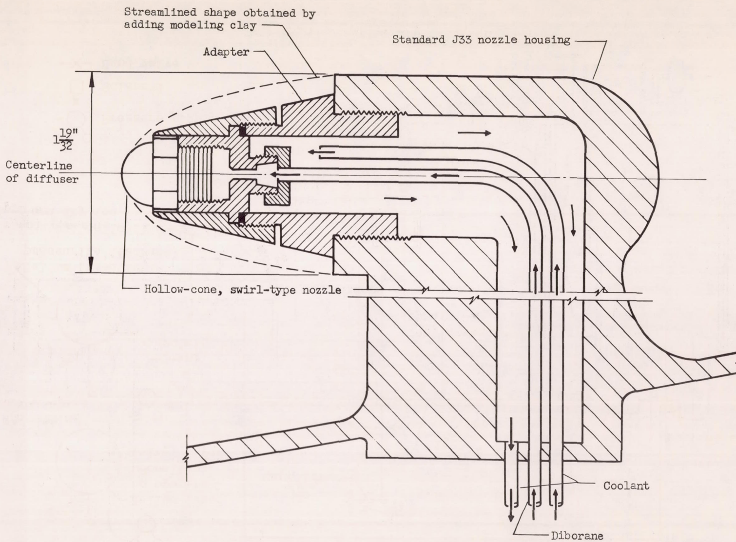
Figure 2. - Diborane injection nozzle.
