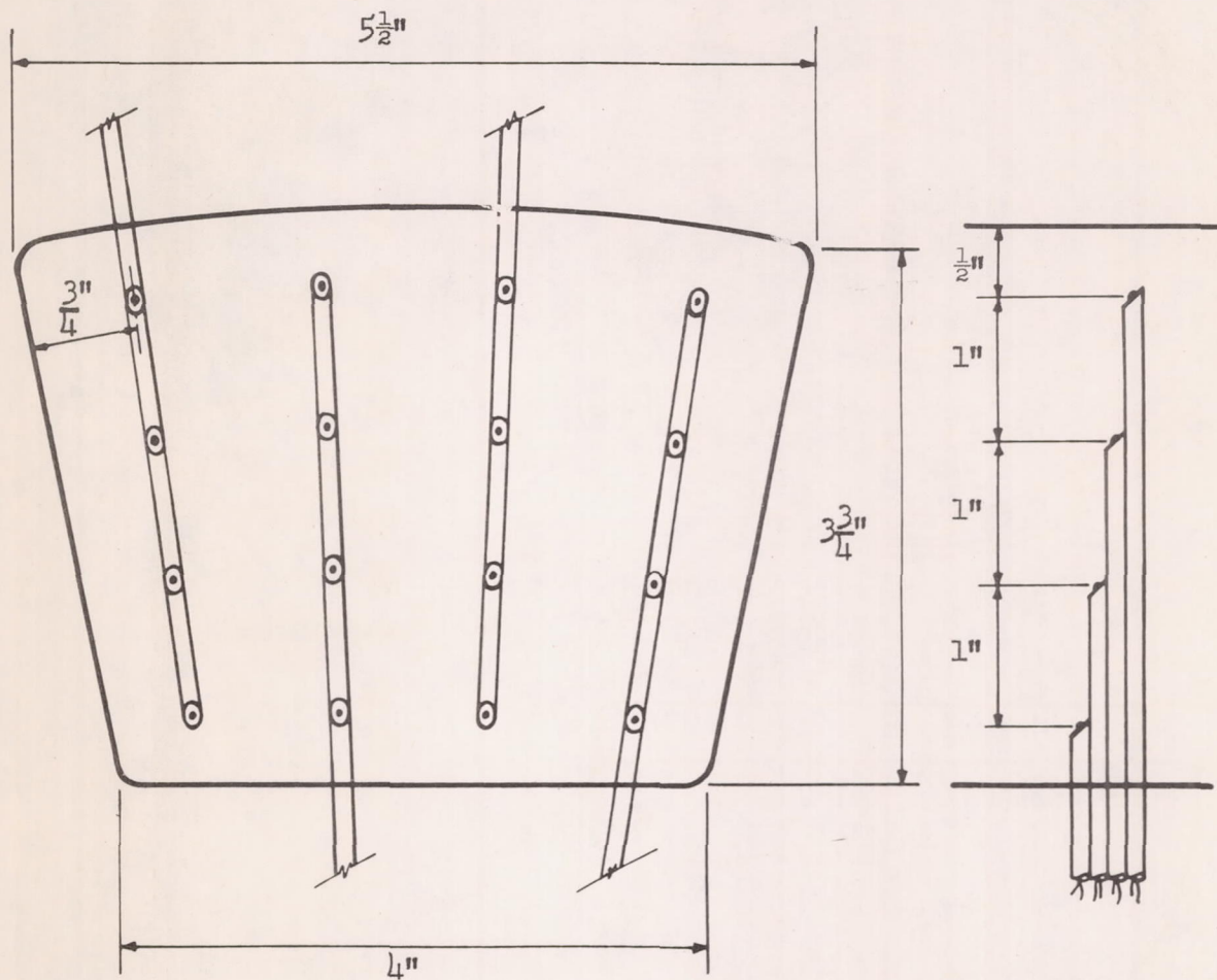
Figure 6. - Combustor-outlet instrumentation.
