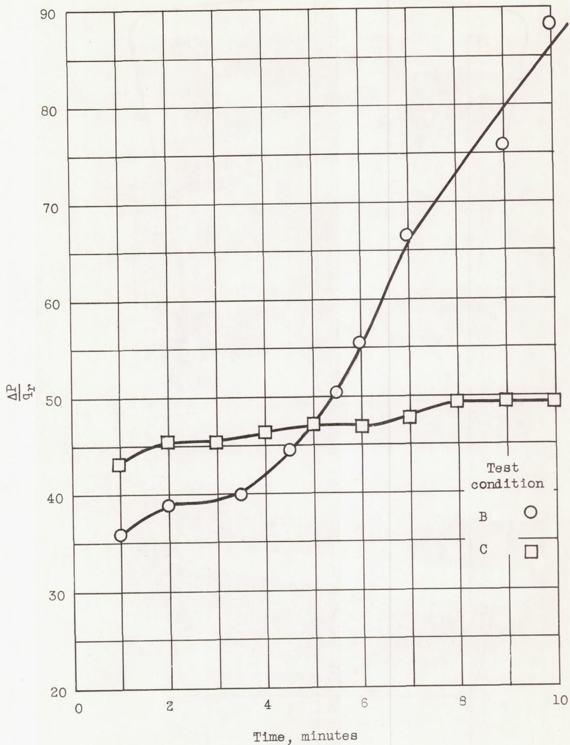
Figure 12. - Variation with time of the total pressure drop through the model 6 combustor plus obstructions in the exhaust duct.
