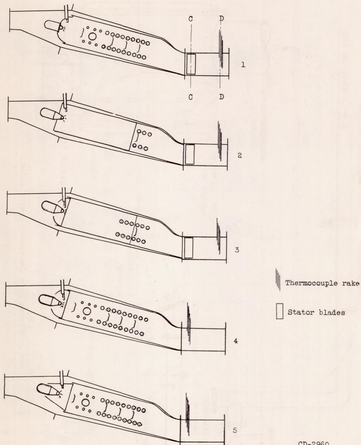
Figure 4. - Combustors.
