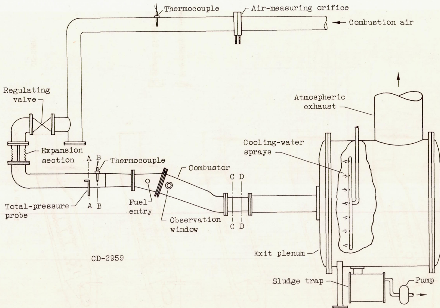
Figure 3. - Combustor installation.
