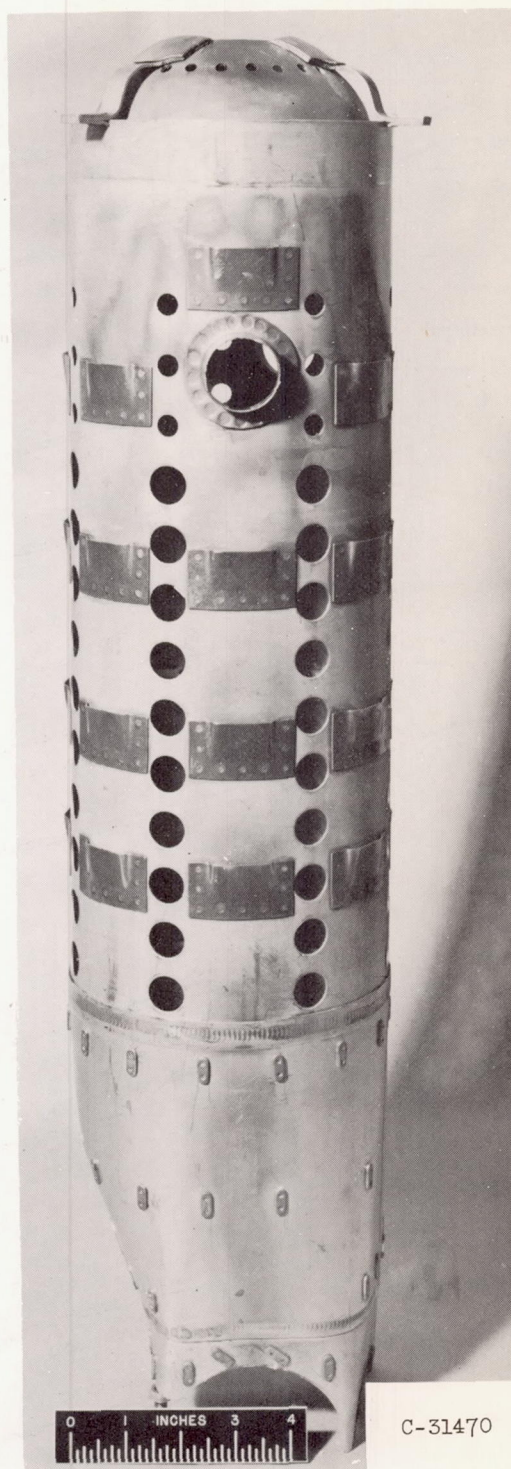
(a) Dome. (b) Photograph of dome and liner assembly.
