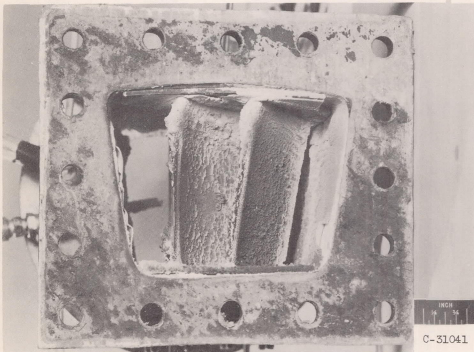
Figure 8. - Deposits with model 2 combustor.
