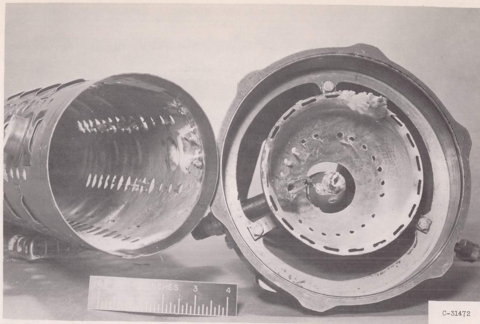
Figure 9. - Concluded. Deposits on liner and dome of model 6 combustor.
