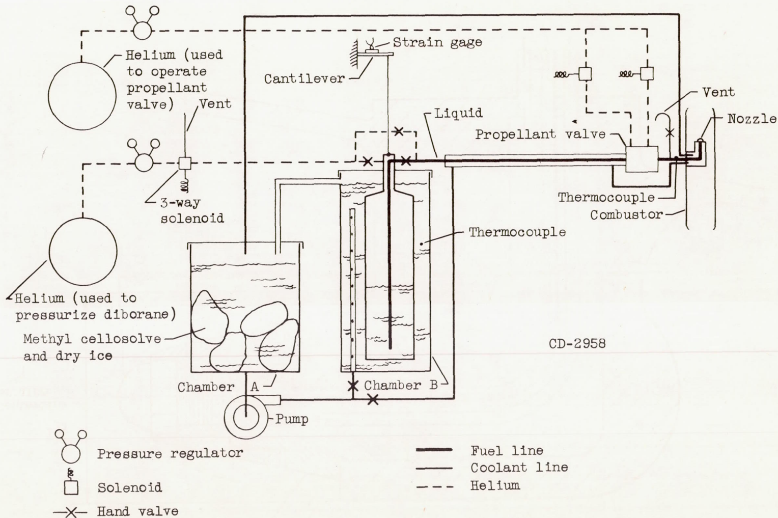
Figure 1. - Fuel system.
