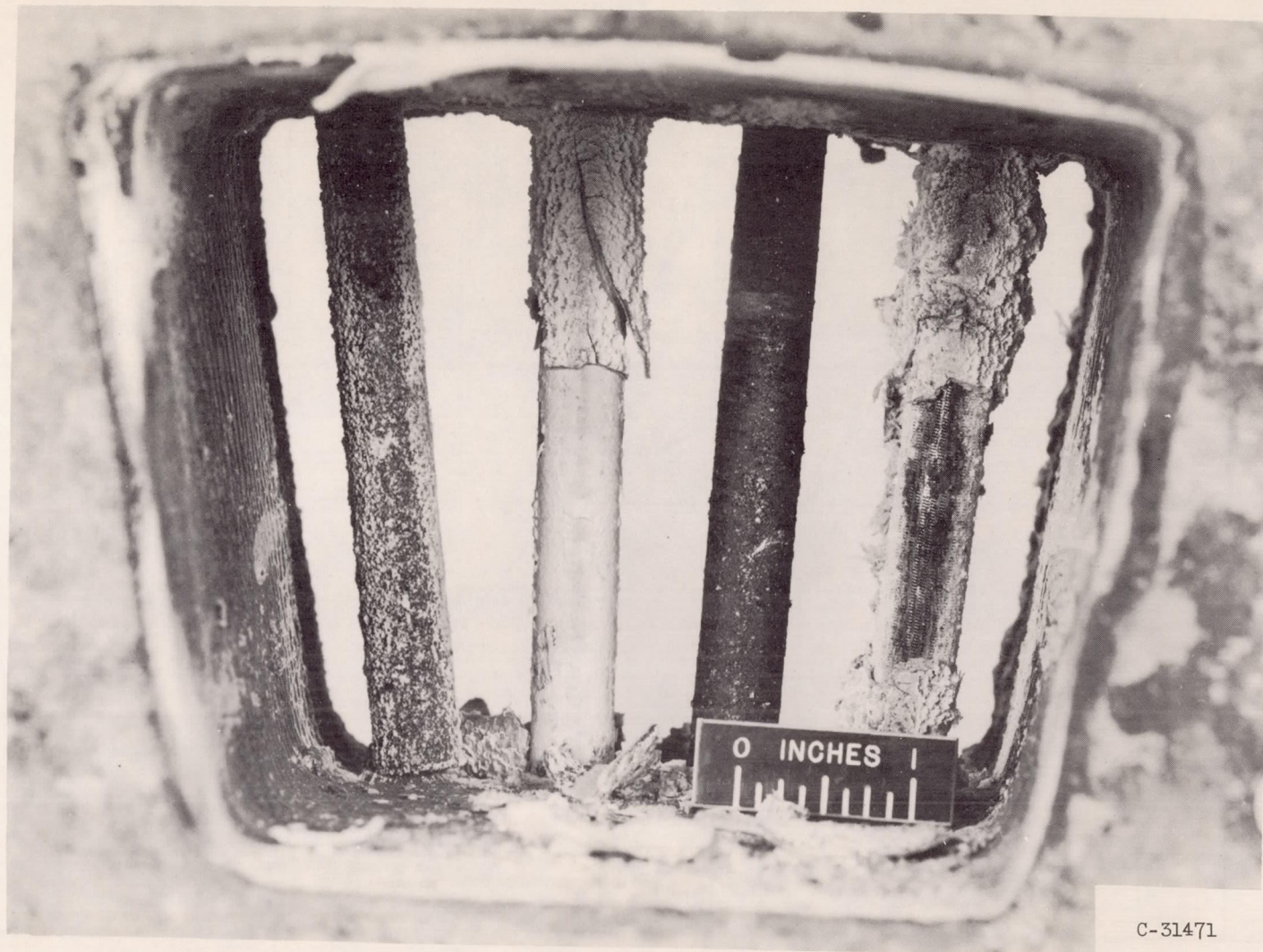
Figure 11. - Concluded. Deposits on special tubes at outlet of model 6 combustor.
