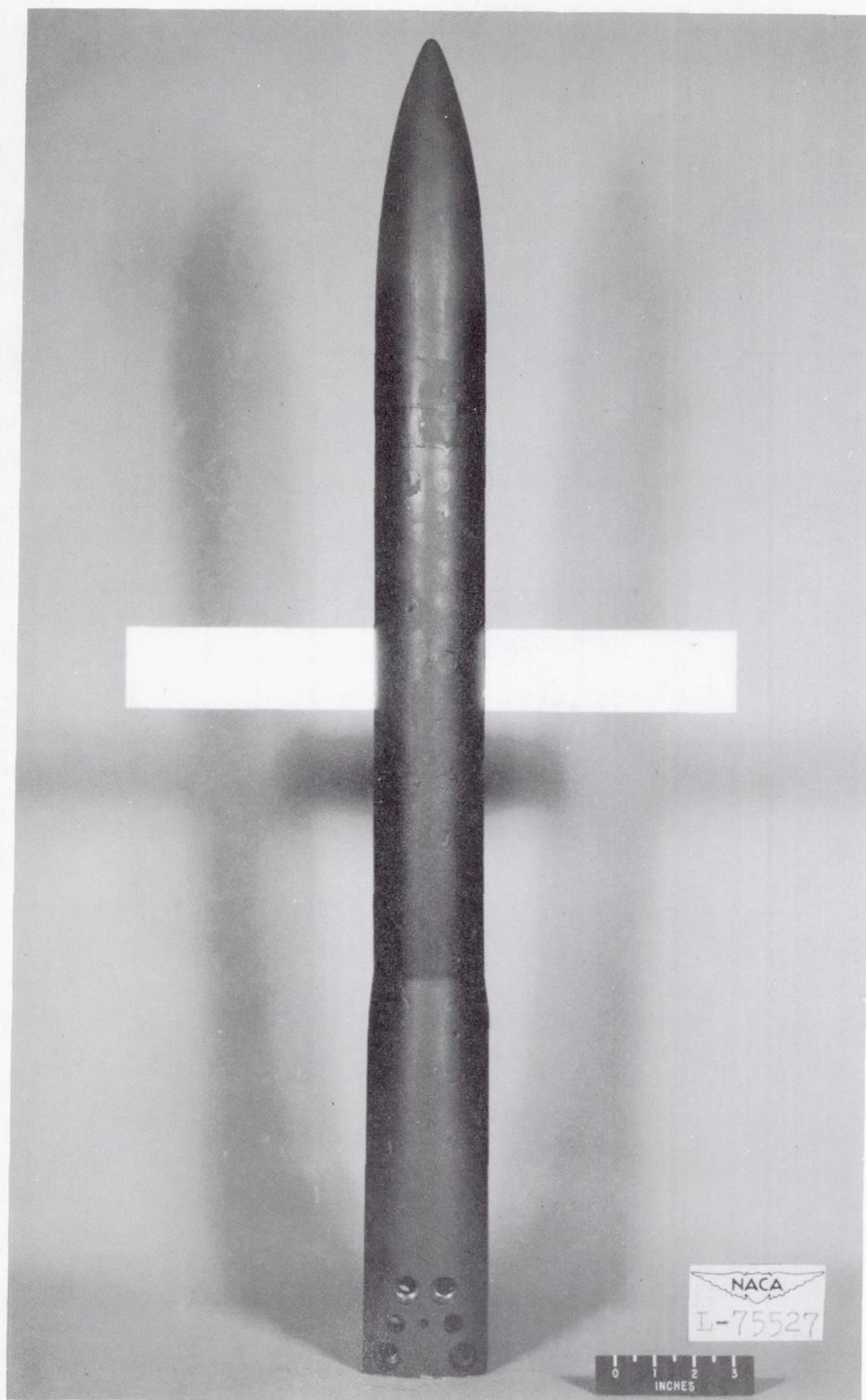
Figure 2.- Wind-tunnel flutter wing and fuselage.
