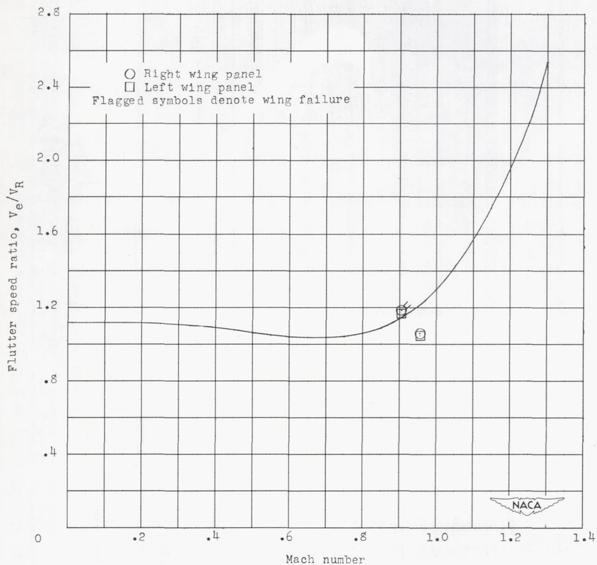
Figure 8.- Comparison of flutter-speed ratio at beginning of flutter and at wing failure.
