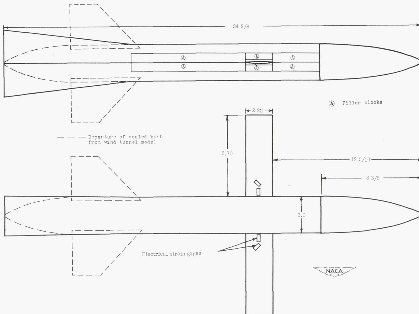
Figure 3.- Flutter-wing model and fuselage. All dimensions are in inches.
