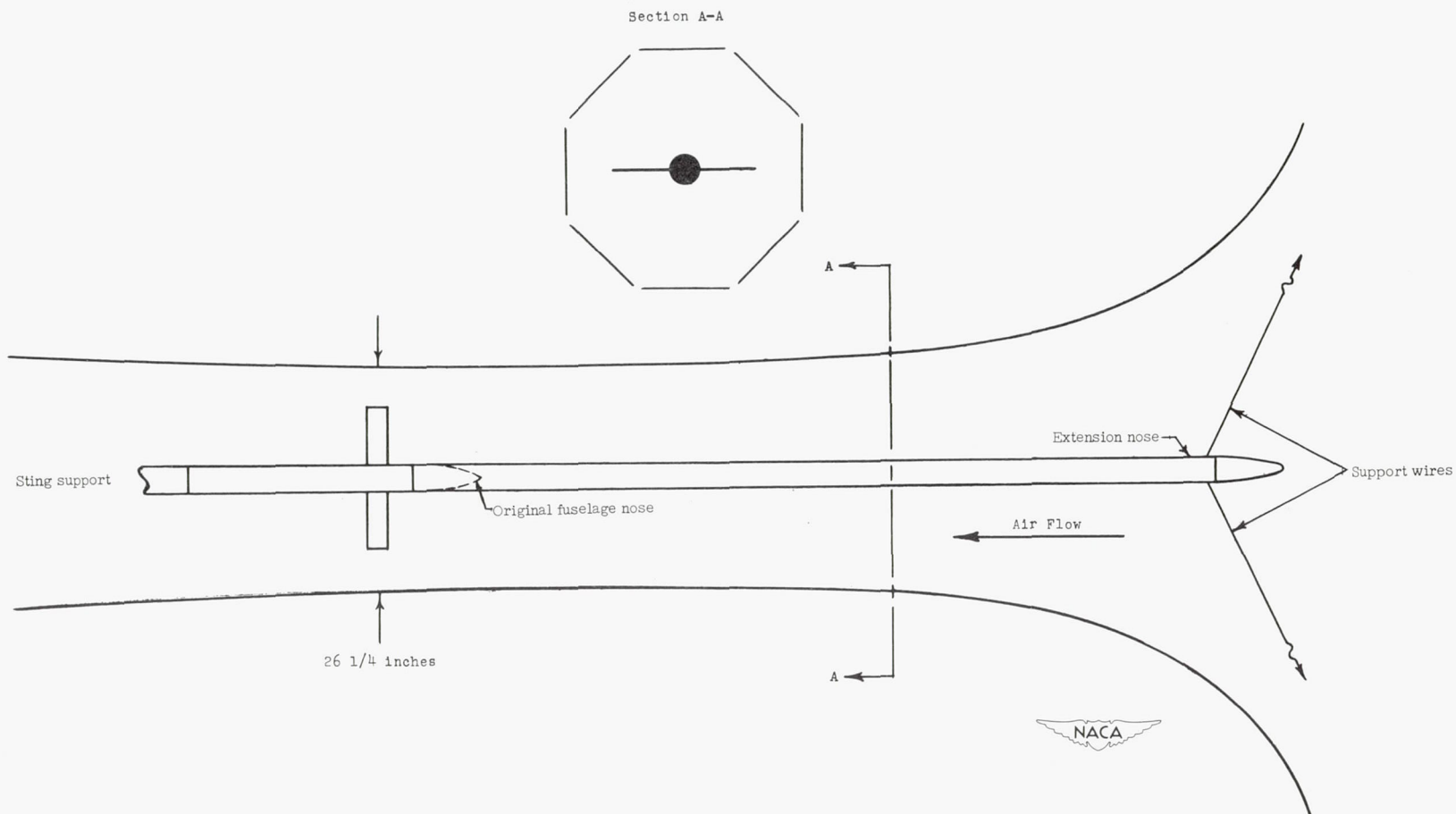
Figure 1.- Plan view of Langley transonic blowdown tunnel with flutter model installed.
