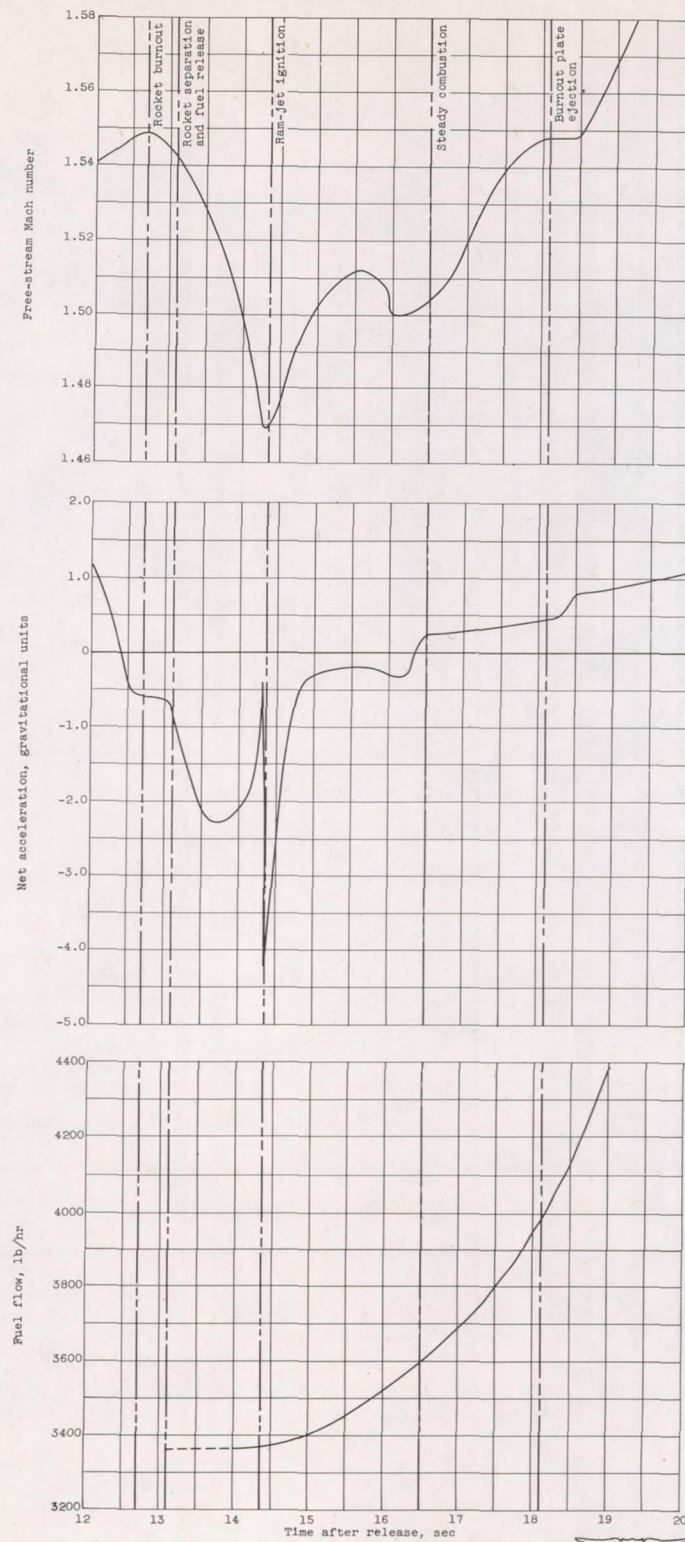
Figure 8. - Concluded. Detailed time history of ram-jet engine, covering sequence from burnout of booster rocket to steady ram-jet combustion.
