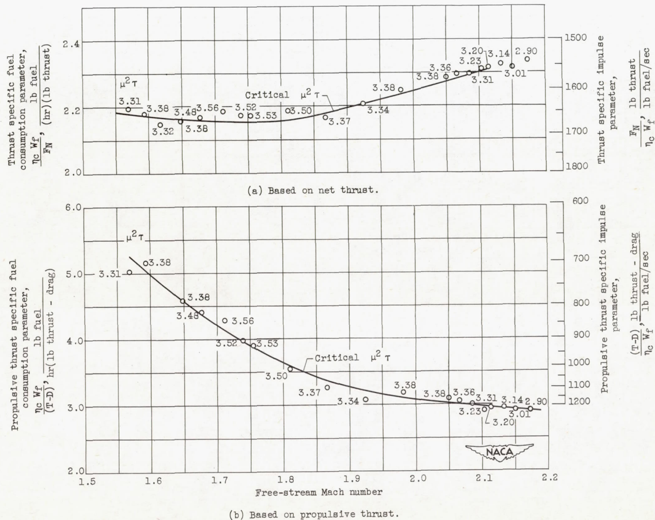
Figure 16. - Specific fuel consumption and specific impulse for model F ram-jet engine with indicated values of \mu^2 \tau .
