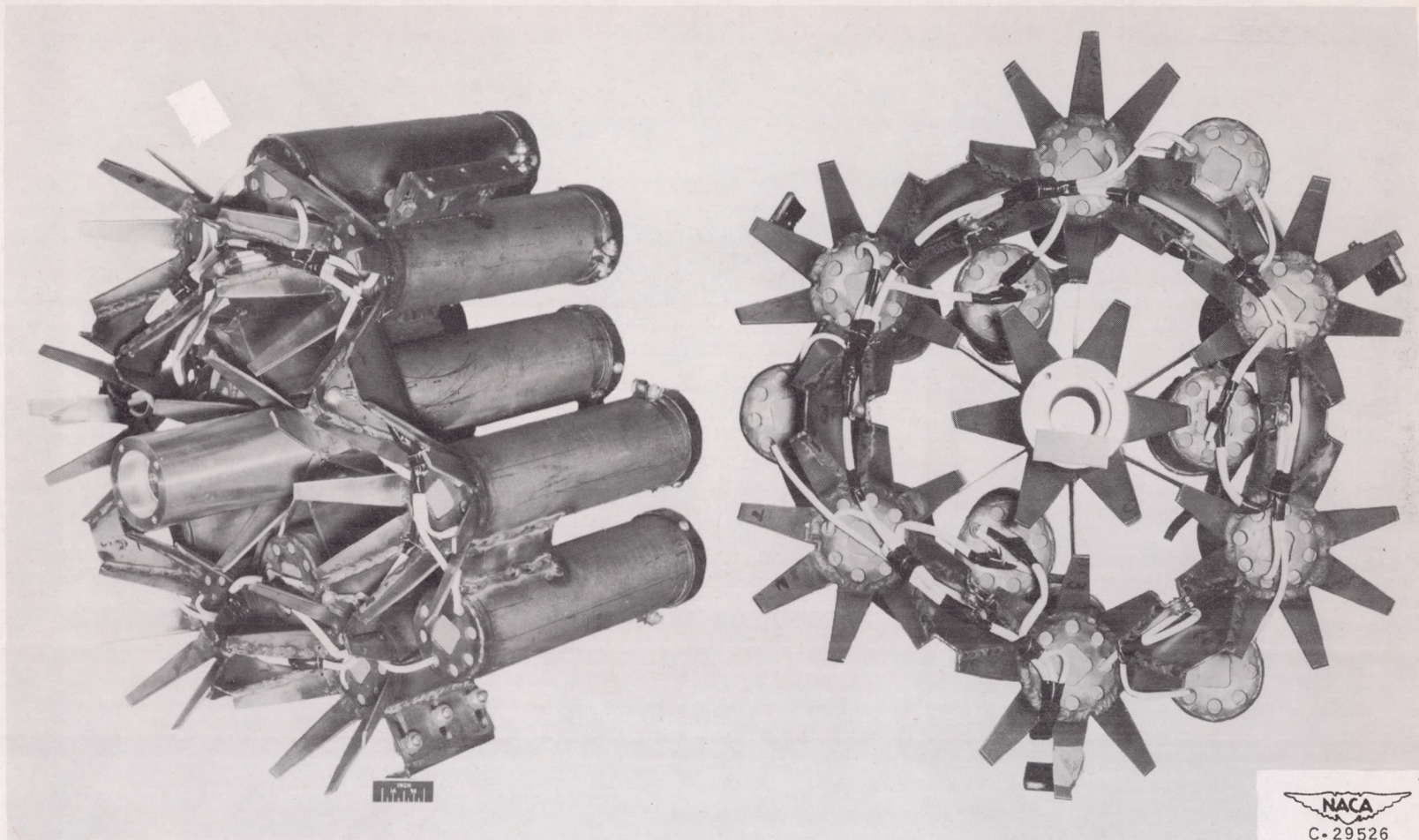
Figure 5. - Star-type flame holder and flare case combination used in model F ram-jet engine.
