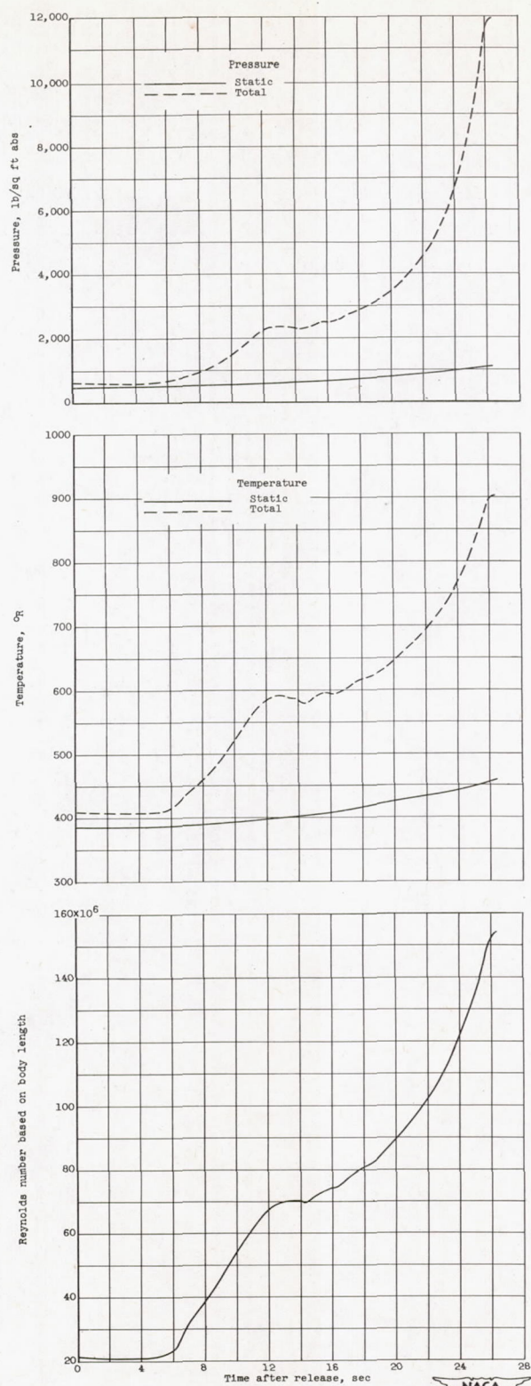
Figure 10. - Time histories of rocket-engineered model F ram-jet engine.
