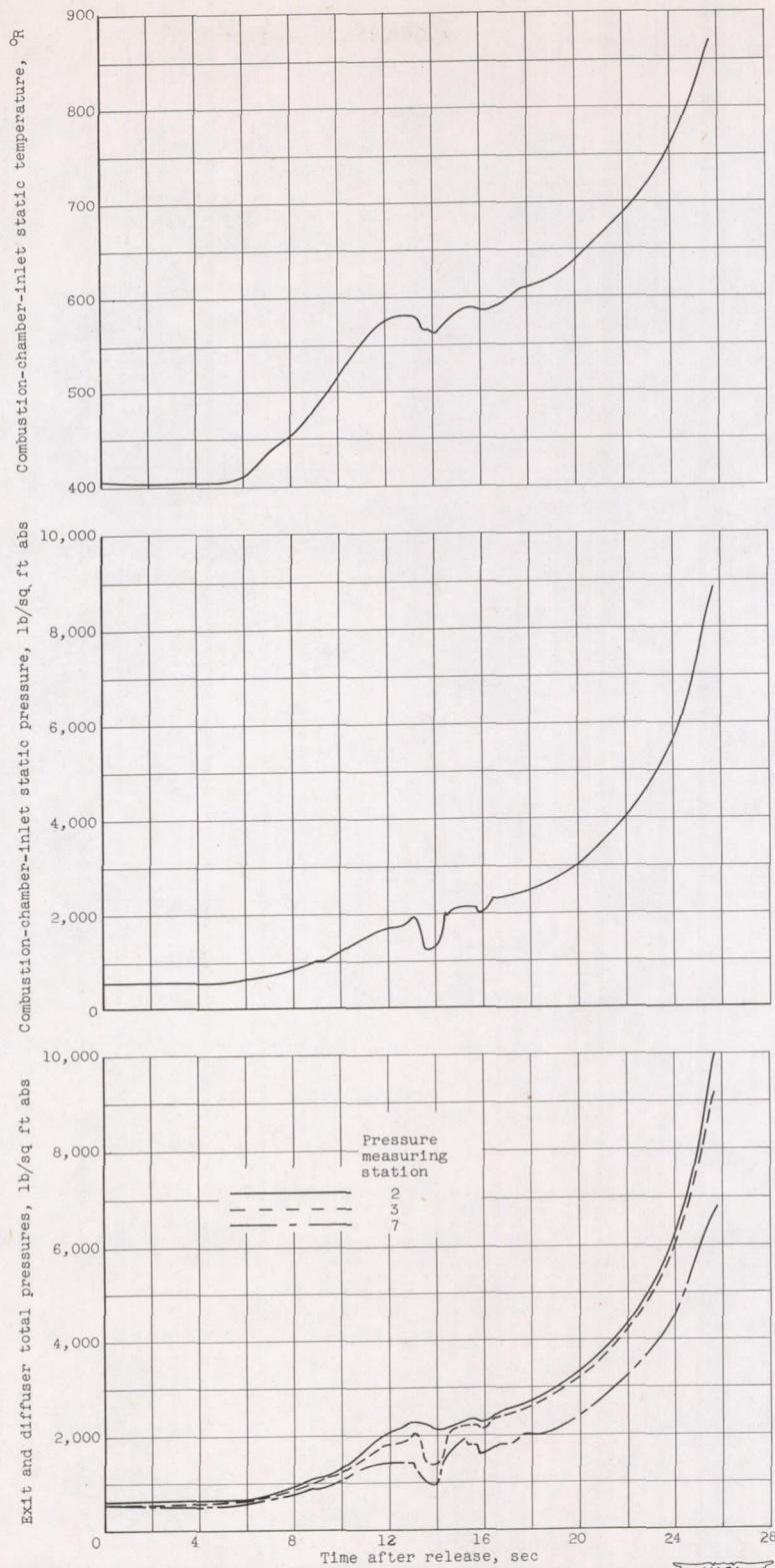
Figure 10. - Continued. Time histories of rocket-boostered model F ram-jet engine.
