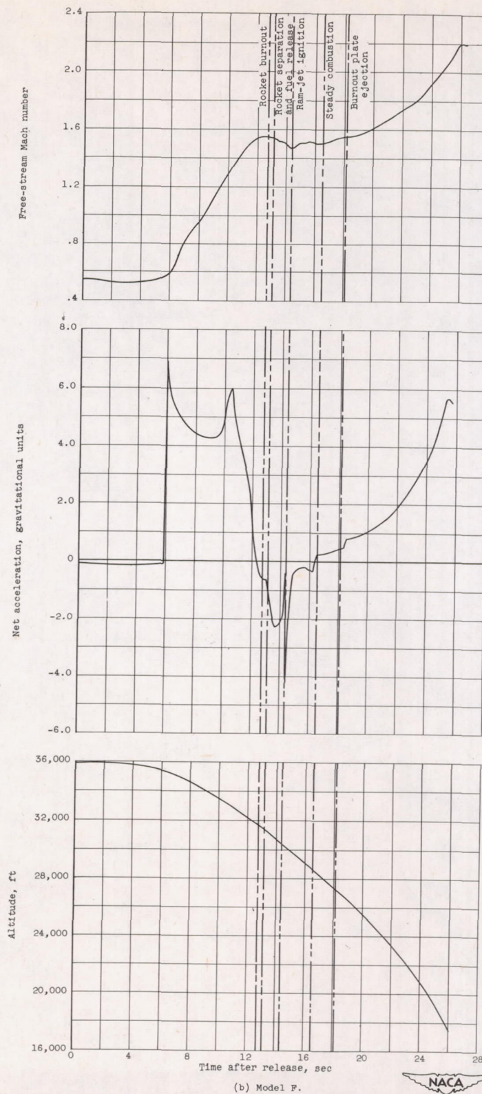
Figure 9. - Concluded. Over-all time history of rocket-boosted ram-jet engine.
