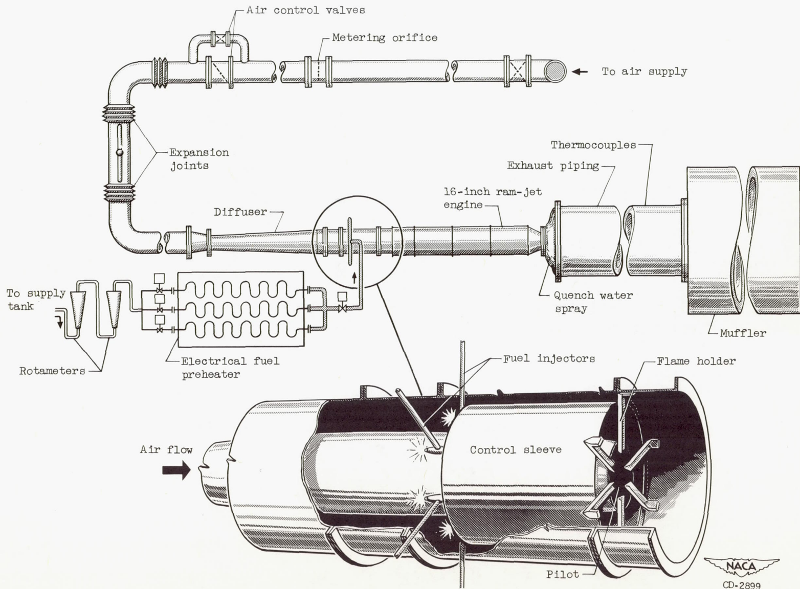
Figure 1. - Installation of 16-inch ram-jet engine.
