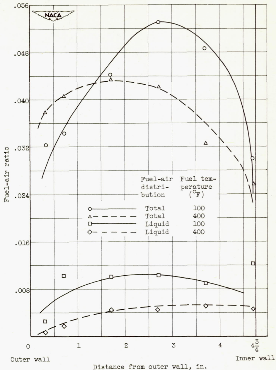
Figure 10. - Concluded. Total and liquid fuel-air distributions for MIL-F-5624A grade JP-4 fuel. Over-all fuel-air ratio, 0.037.
