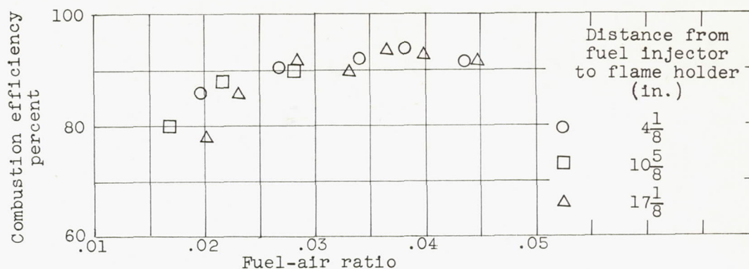
Figure 7. - Comparison of combustion efficiencies for three injector distances upstream of the flame holders for cold MIL-F-5624A grade JP-4 fuel and fuel injectors at midposition of annulus.
