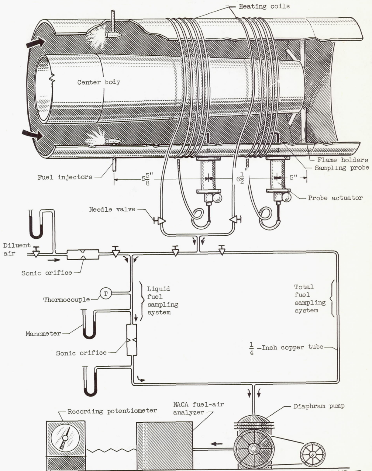
Figure 5. - Sketch of total fuel-air and liquid fuel-air sampling system.
