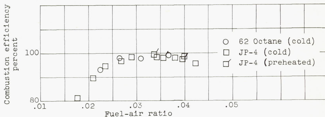
Figure 8. - Effect of fuel type and fuel temperature on combustion efficiency with a 1\frac{1}{2} -inch-diameter fuel-mixing control sleeve and fuel injectors 17\frac{1}{8} inches upstream of flame holders. Fuel, MIL-F-5624A grade JP-4 and 62-octane gasoline.
