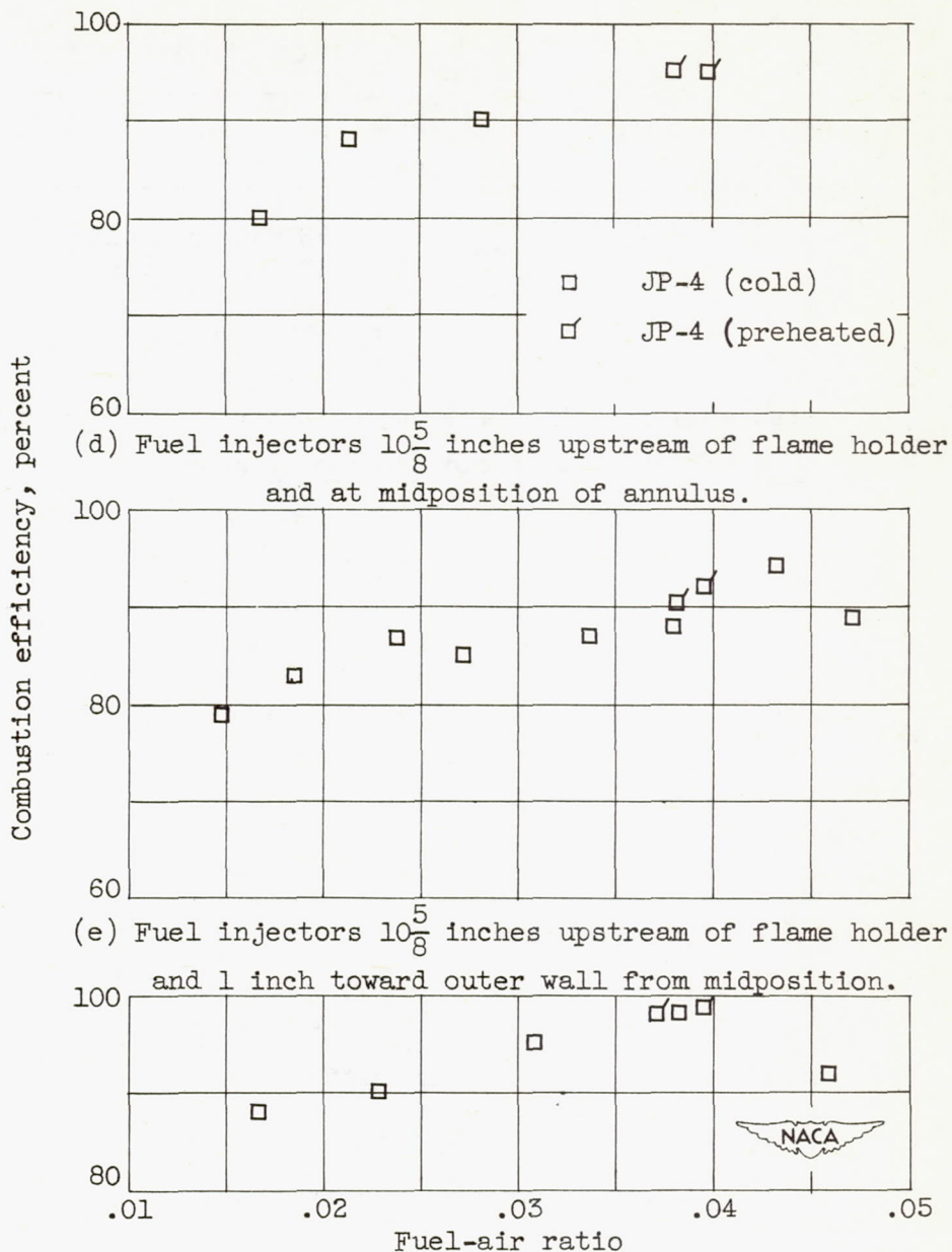
Figure 6. - Continued. Effect of fuel type, fuel temperature, and fuel-injector radial position on combustion efficiency. Fuel, MIL-F-5624A grade JP-4 and 62-octane gasoline.
