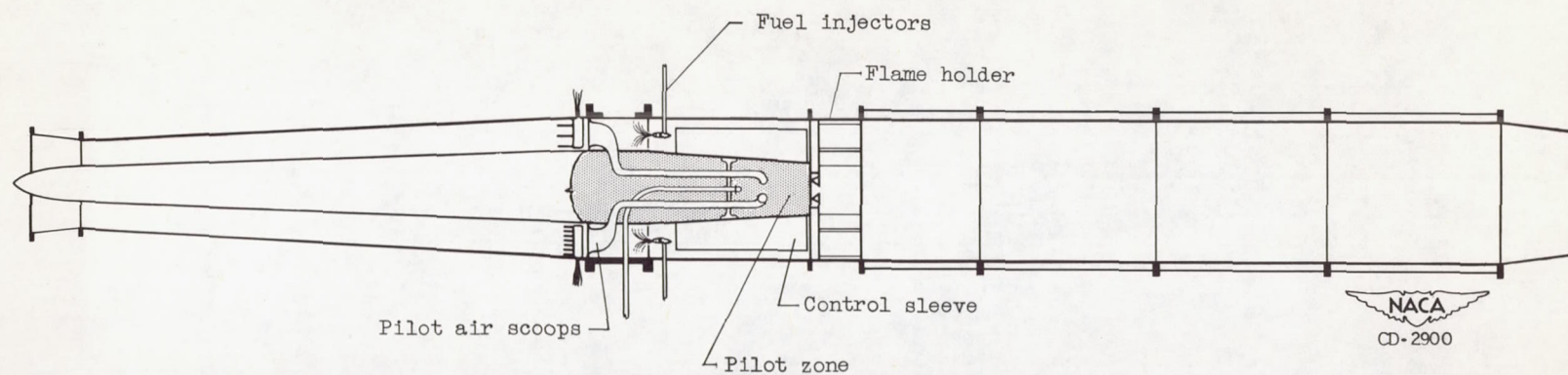
Figure 2. - Sketch of 16-inch ram-jet engine showing position of fuel injectors, flame holder, and mixing control sleeve.
