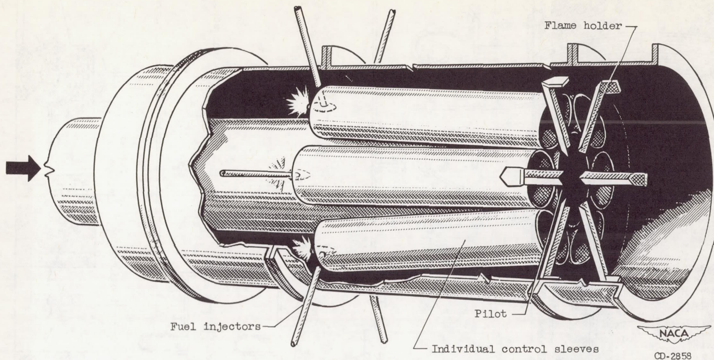
Figure 4. - Installation of six individual fuel-mixing control sleeves between fuel injectors and flame holder.
