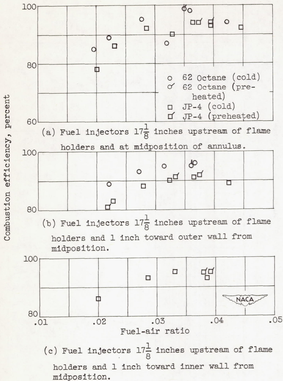
Figure 6. - Effect of fuel type, fuel temperature, and fuel-injector radial position on combustion efficiency. Fuel, MIL-F-5624A grade JP-4 and 62-octane gasoline.
