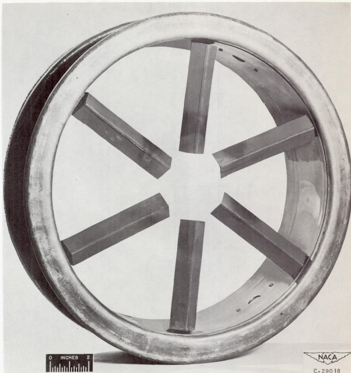
Figure 3. - Flame-holder configuration showing radial V-gutter, upstream face.
