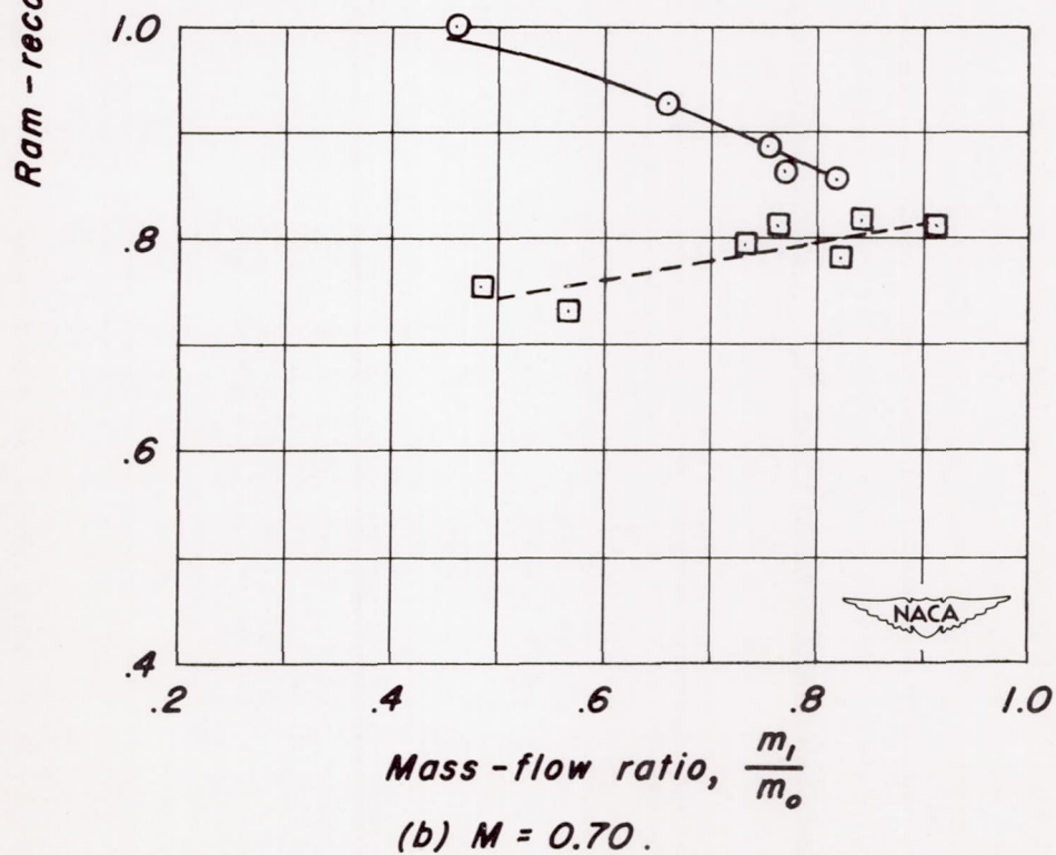
Figure 7.—Typical variations of ram-recovery ratio at the inlet with mass-flow ratio.
