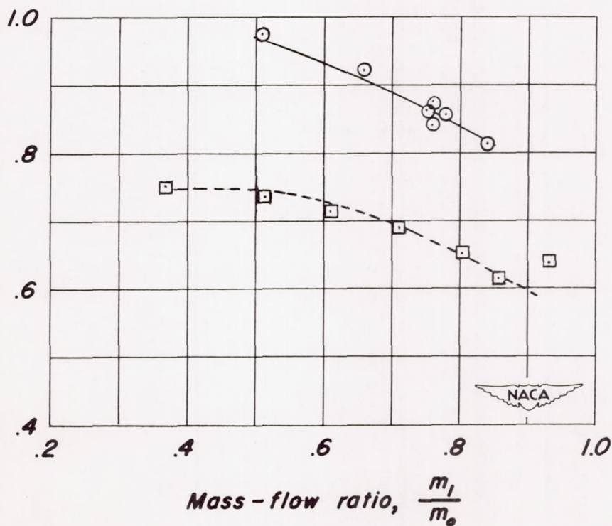
Figure 8.—Typical variation of ram-recovery ratio at the compressor face with mass-flow ratio.
