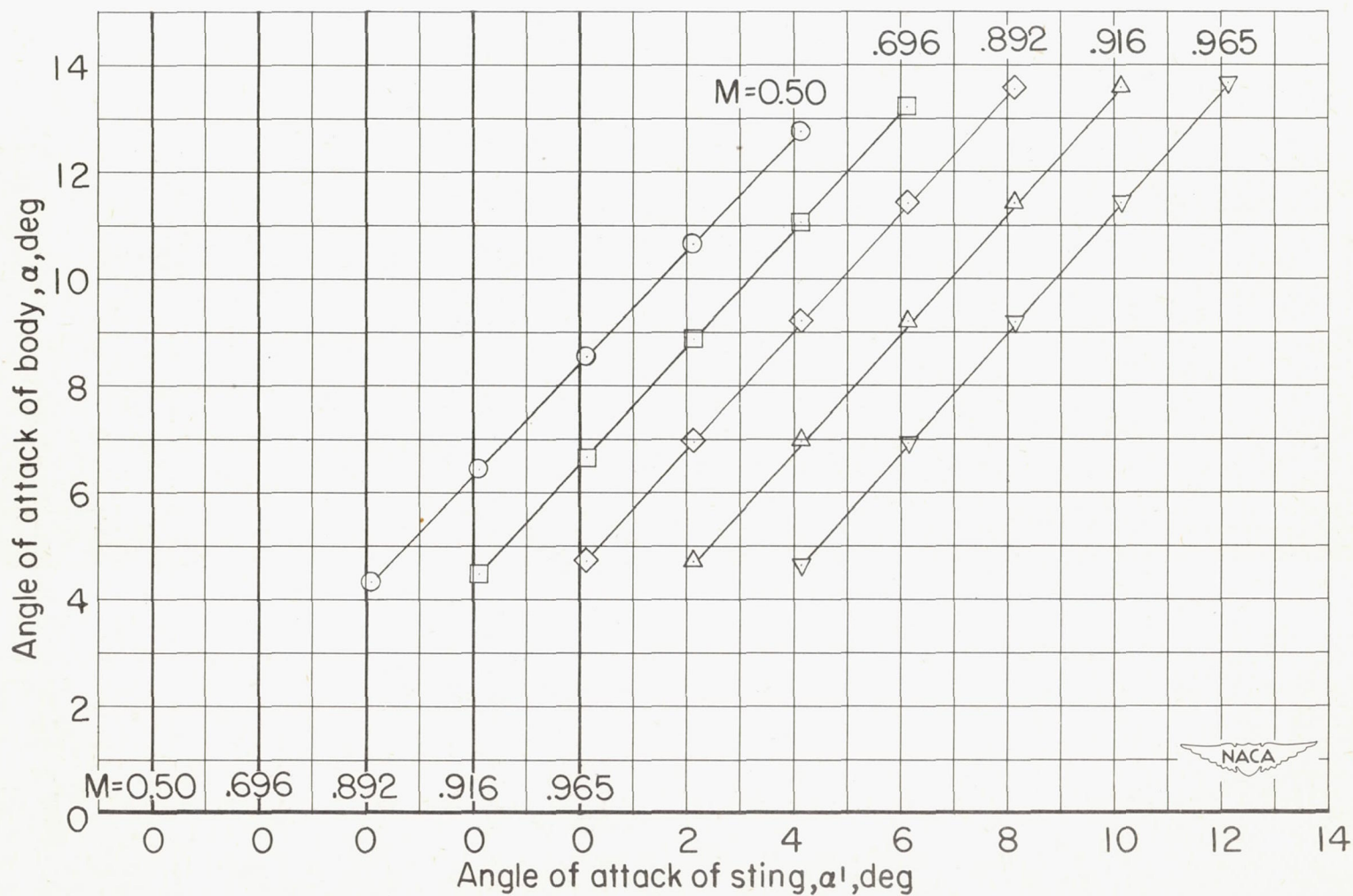
Figure 12.- Variation of angle of attack of body with angle of attack of sting. Wing-body configuration; h_t = 0.333\frac{b}{2} ; i = 3^\circ .
