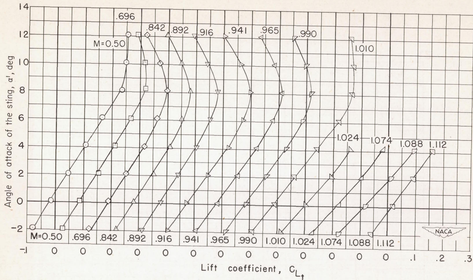
Figure 5.- Variation of the angle of attack of the sting with the horizontal-tail lift coefficient in presence of the wing-body configuration. h_t = 0.333 \frac{b}{2} ; i = 0^\circ .
