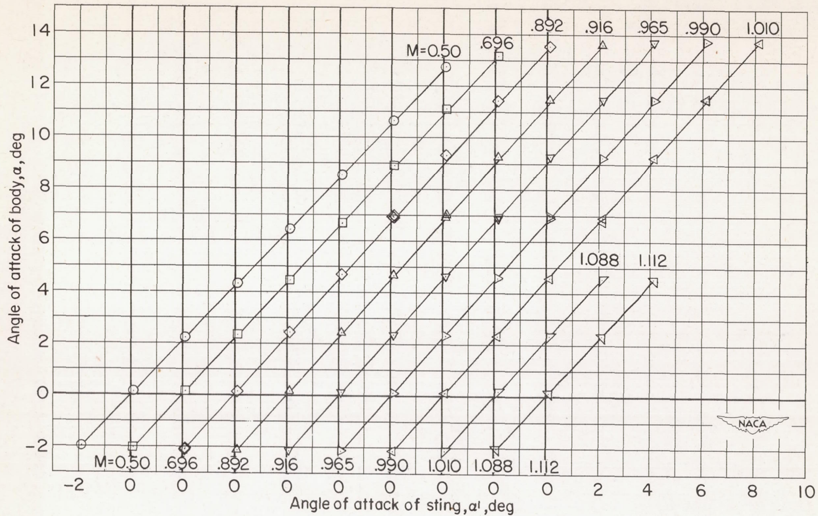
Figure 11.- Variation of angle of attack of body with angle of attack of sting. Wing-body configuration; h_t = 0.333\frac{b}{2} ; i = 0^\circ .
