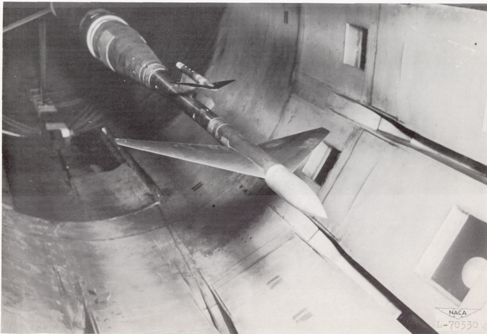
Figure 2.- Model as tested in the Langley 8-foot transonic tunnel.
