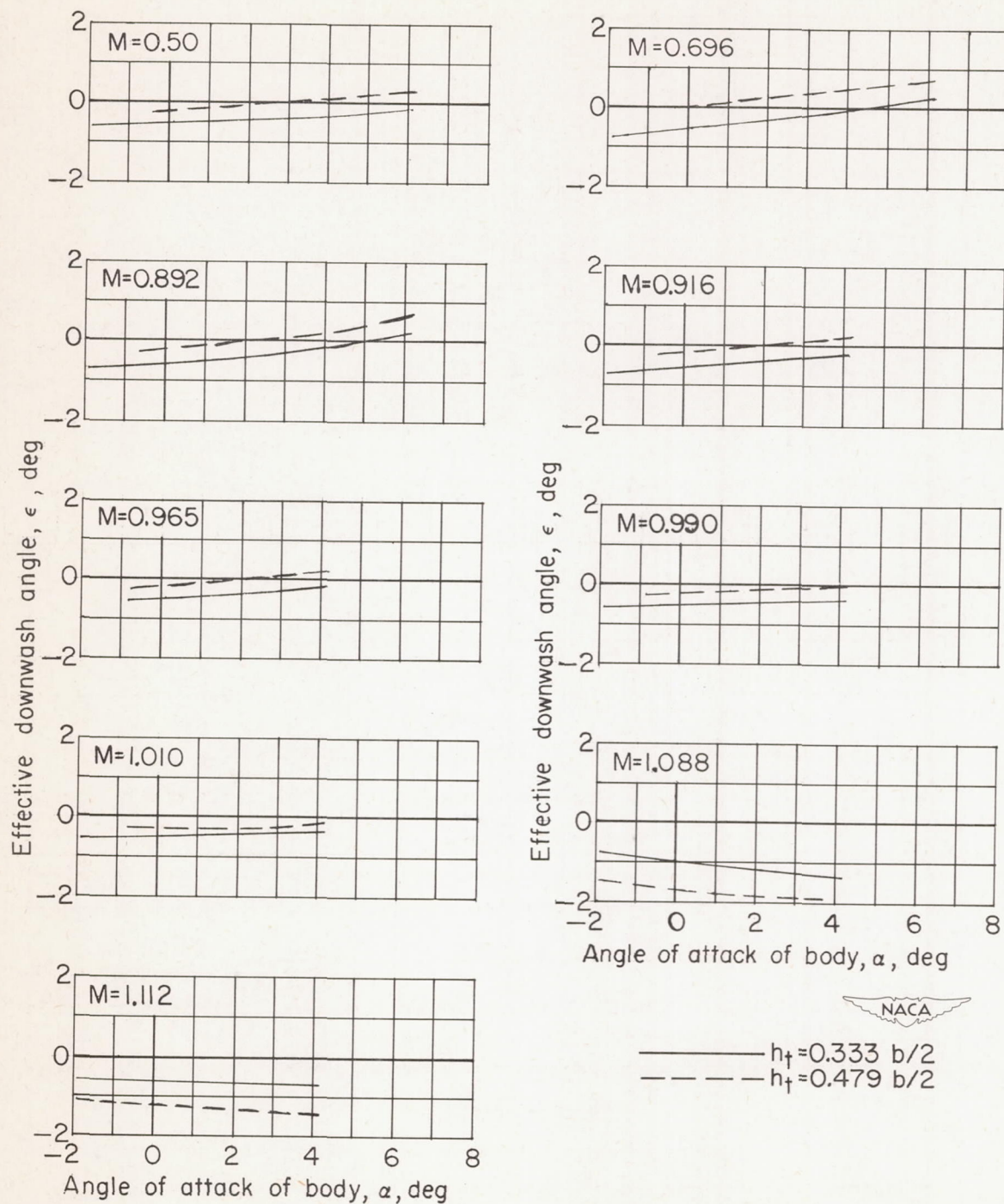
Figure 19.- Variation with angle of attack of body of the effective downwash angle for the body alone.
