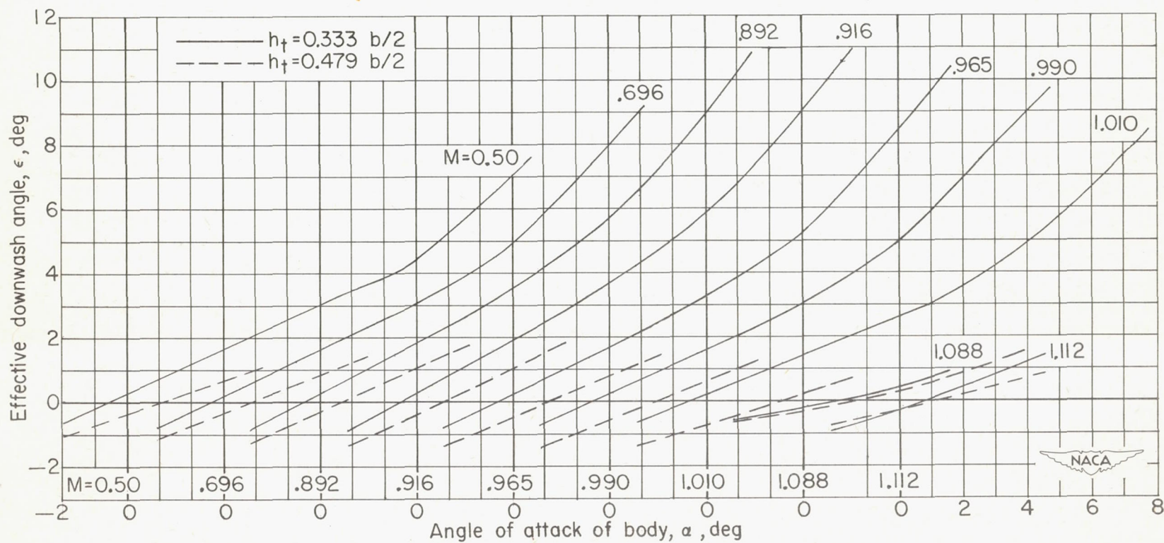
Figure 18.- Variation with angle of attack of body of the effective downwash angle for the wing-body configuration.
