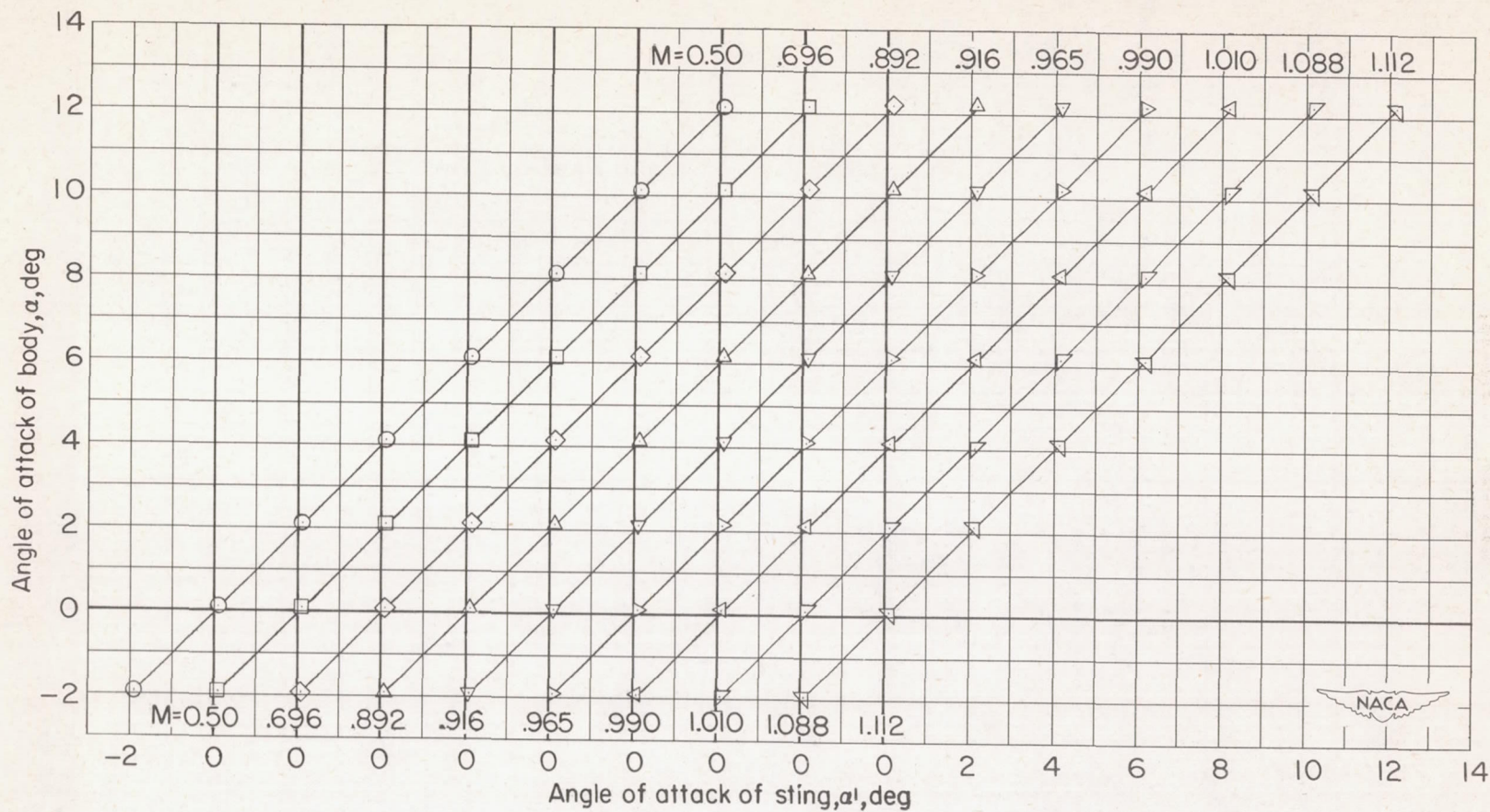
Figure 15.- Variation of angle of attack of body with angle of attack of sting. Body alone; h_t = 0.333\frac{b}{2} ; i = 0^\circ .
