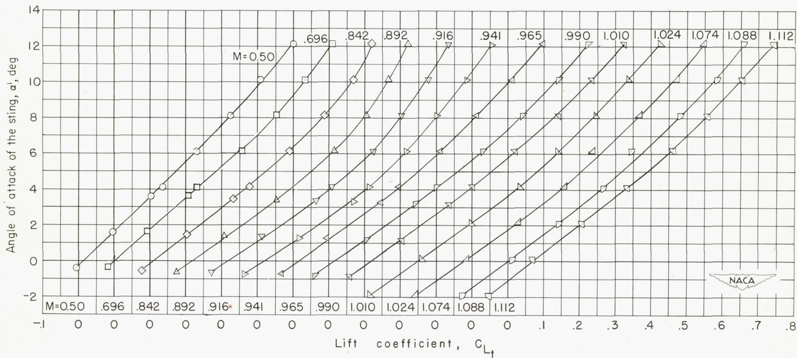
Figure 10.- Variation of the angle of attack of the sting with the horizontal-tail lift coefficient in presence of the body alone.
