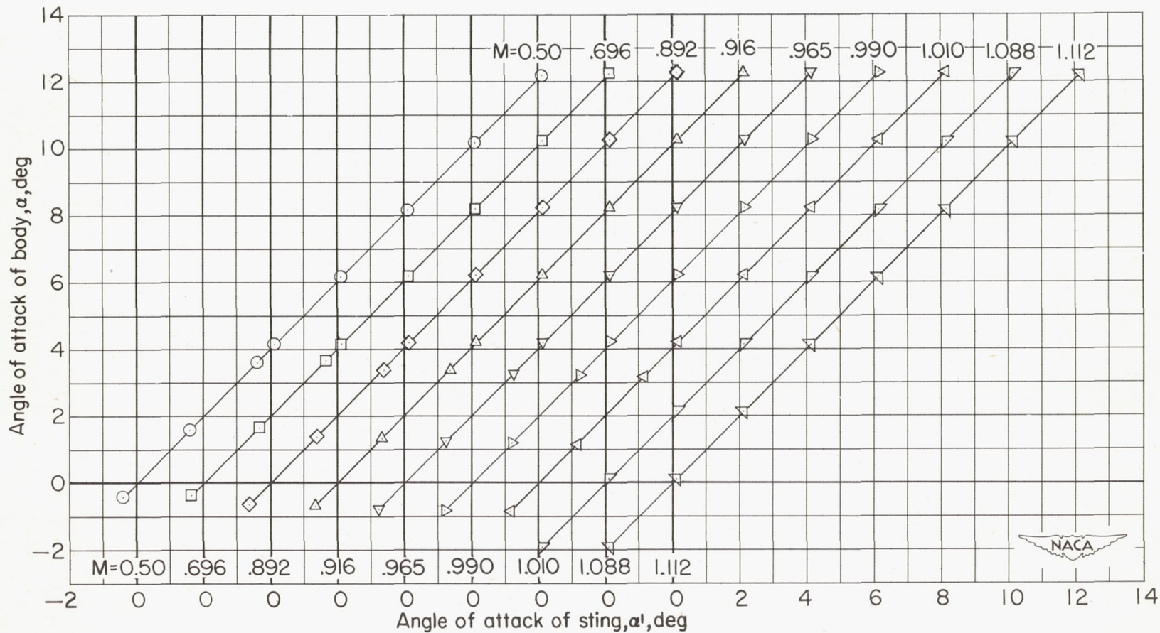
Figure 16.- Variation of angle of attack of body with angle of attack of sting. Body alone; h_t = 0.479 \frac{b}{2} ; i = 0^\circ .
