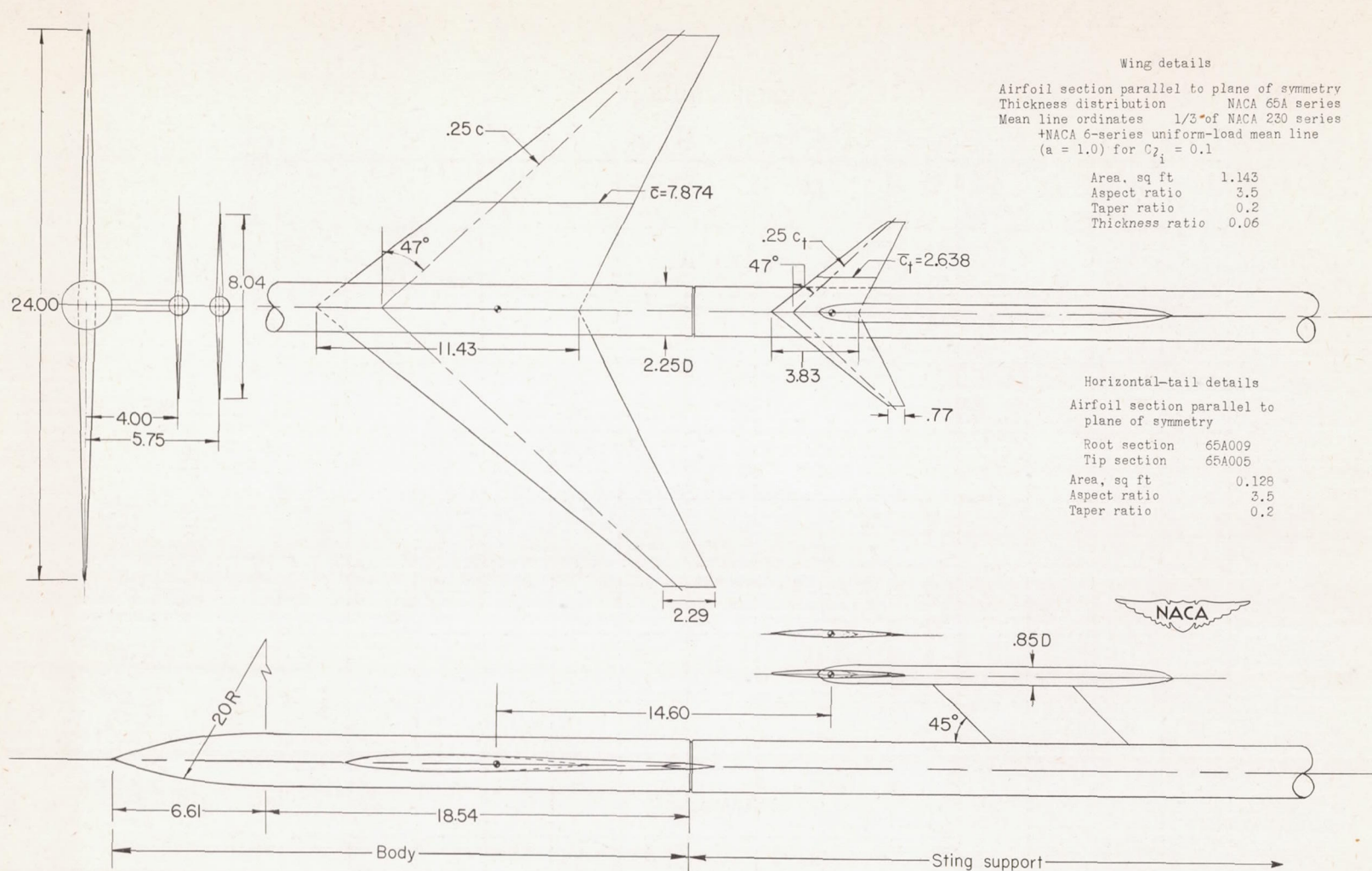
Figure 3.- Model details. All dimensions are in inches.
