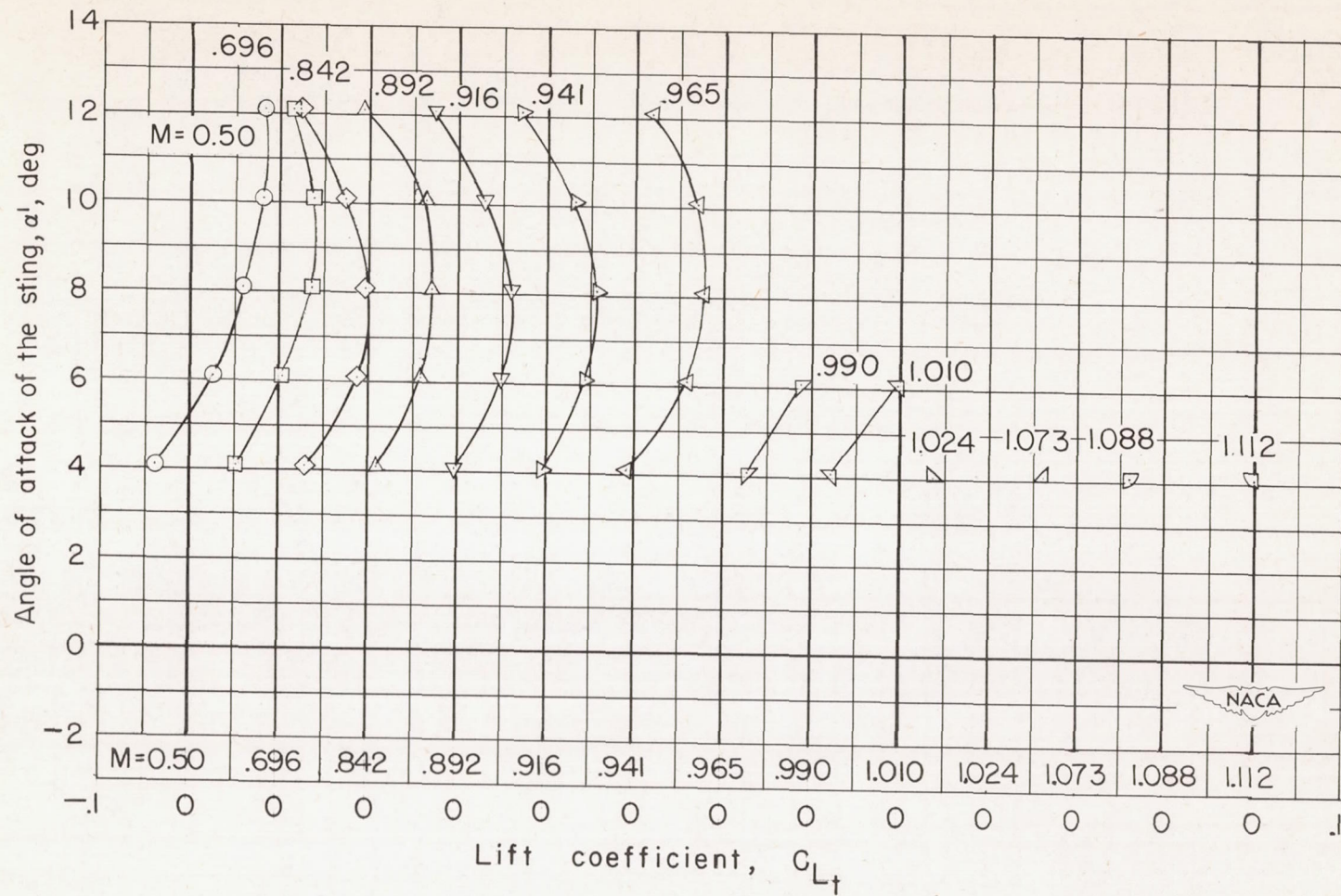
Figure 7.- Variation of the angle of attack of the sting with the horizontal-tail lift coefficient in presence of the wing-body configuration. h_t = 0.333 \frac{b}{2} ; i = -3^\circ .
