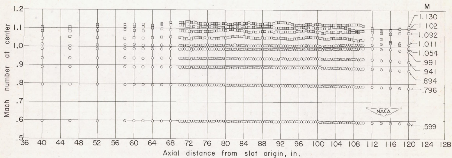
Figure 1.- Mach number distributions along the center of the test section.
