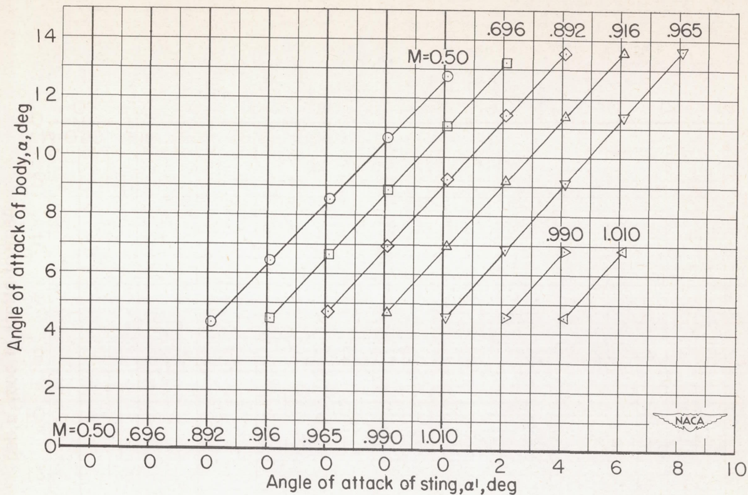
Figure 13.- Variation of angle of attack of body with angle of attack of sting. Wing-body configuration; h_t = 0.333 \frac{b}{2} ; i = -3^\circ .
