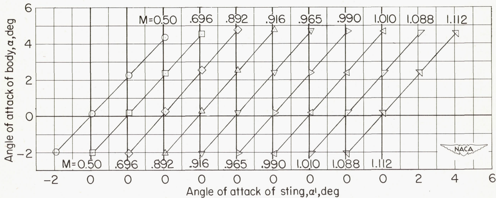
Figure 14.- Variation of angle of attack of body with angle of attack of sting. Wing-body configuration; h_t = 0.479 \frac{b}{2} ; i = 0^\circ .
