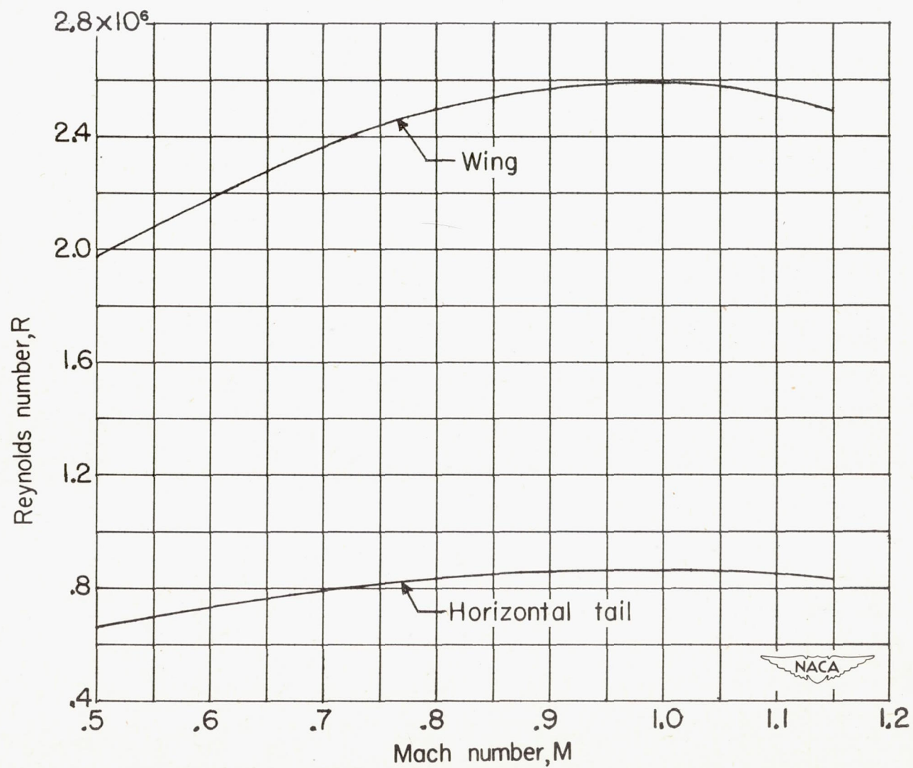
Figure 4.- Variation with Mach number of test Reynolds number.
