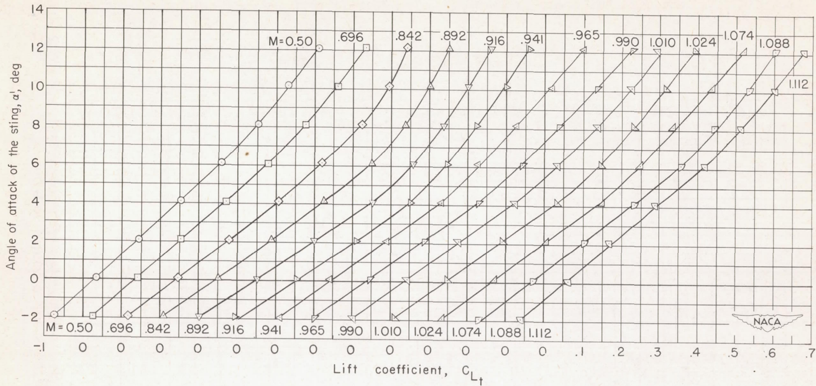
Figure 9.- Variation of the angle of attack of the sting with the horizontal-tail lift coefficient in presence of the body alone.
