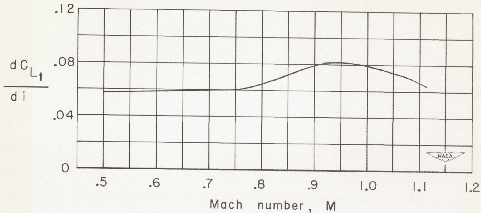
Figure 17.- Variation of the horizontal-tail lift-curve slope with Mach number in presence of the wing-body configuration. \alpha' = 4^\circ .
