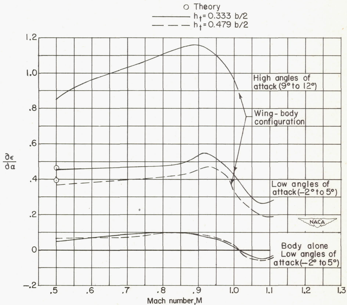
Figure 20.- Variation with Mach number of the effective downwash derivative for the wing-body and body alone configurations.
