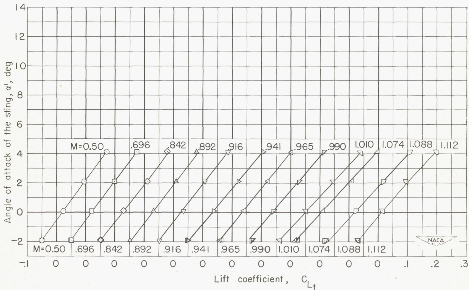
Figure 8.- Variation of the angle of attack of the sting with the horizontal-tail lift coefficient in presence of the wing-body configuration. h_t = 0.479 \frac{b}{2} ; i = 0^\circ .
