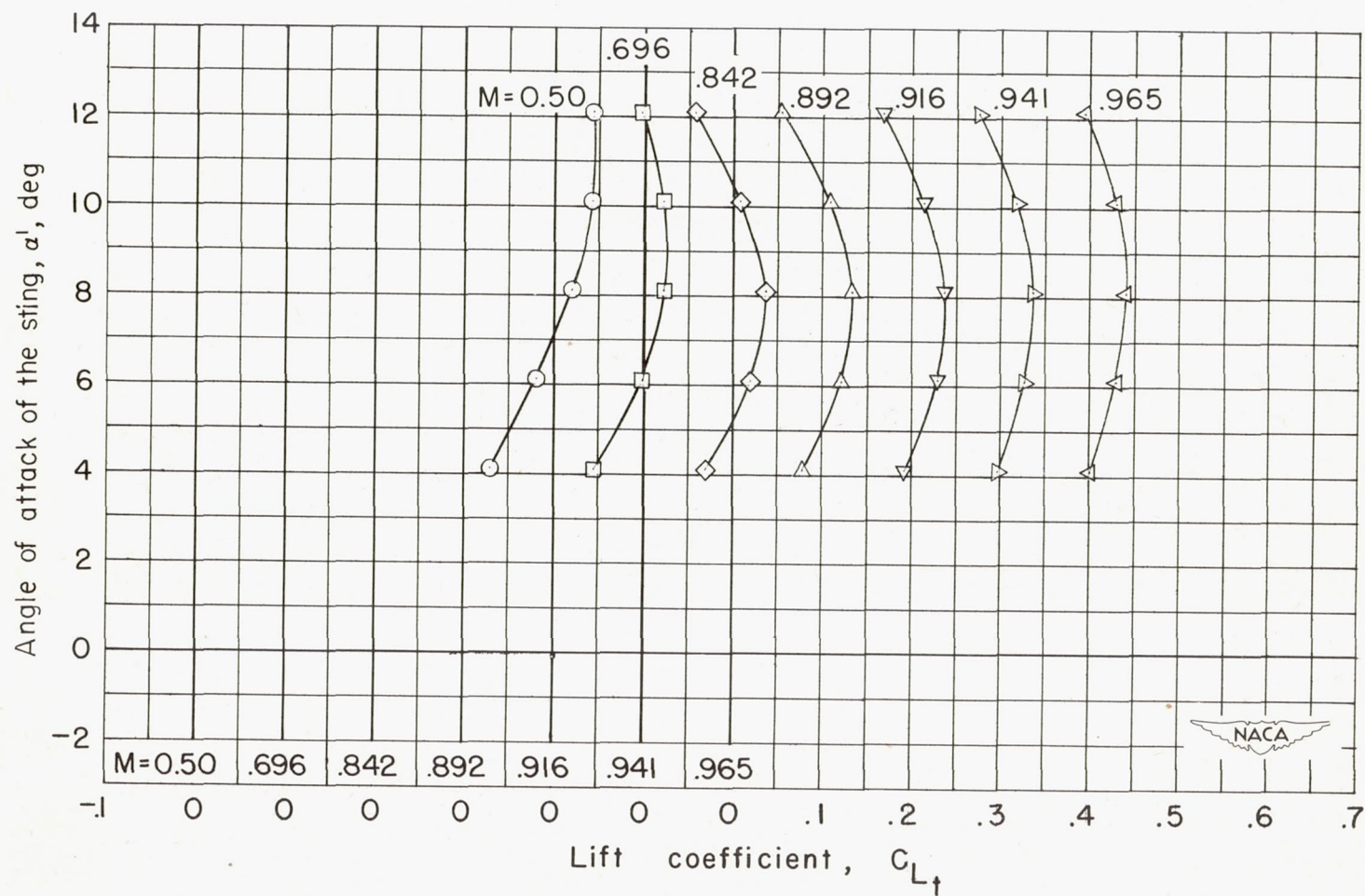
Figure 6.- Variation of the angle of attack of the sting with the horizontal-tail lift coefficient in presence of the wing-body configuration. h_t = 0.333\frac{b}{2} ; i = 3^\circ .
