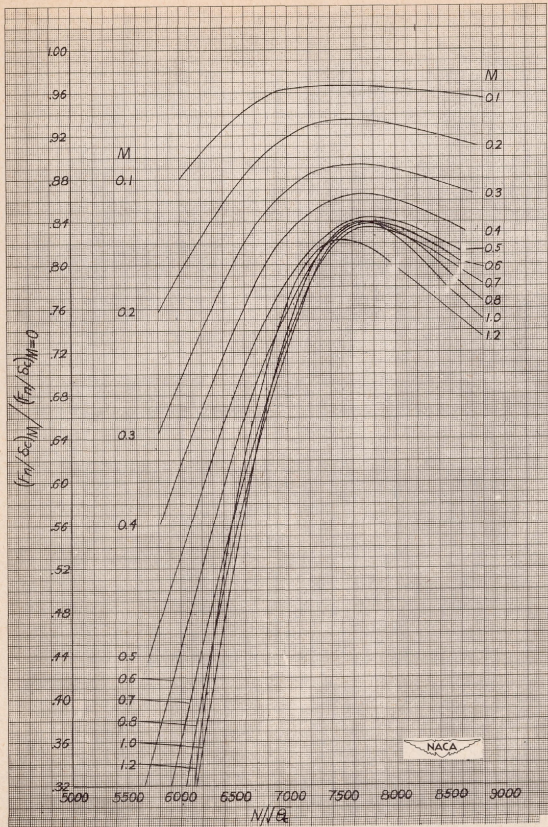
Figure 5.- Factor for correcting engine thrust for various flight Mach numbers.
