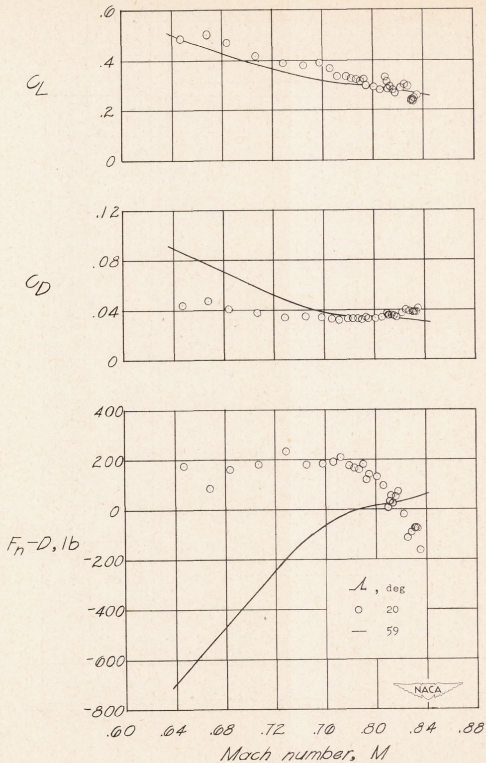
Figure 12.- Comparison of performance of 20° and 59° sweptback configurations in unaccelerated flight at an altitude of about 42,000 feet.
