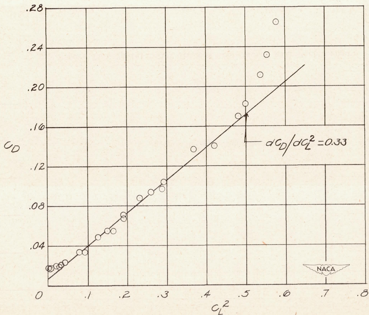
Figure 10.- Typical plot for determination of induced drag factor. M = 0.80 .
