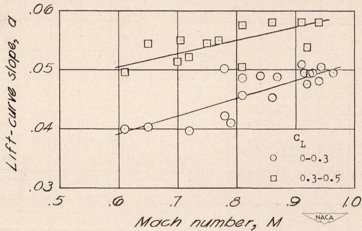
Figure 7.- Variation of lift-curve slope with Mach number.
