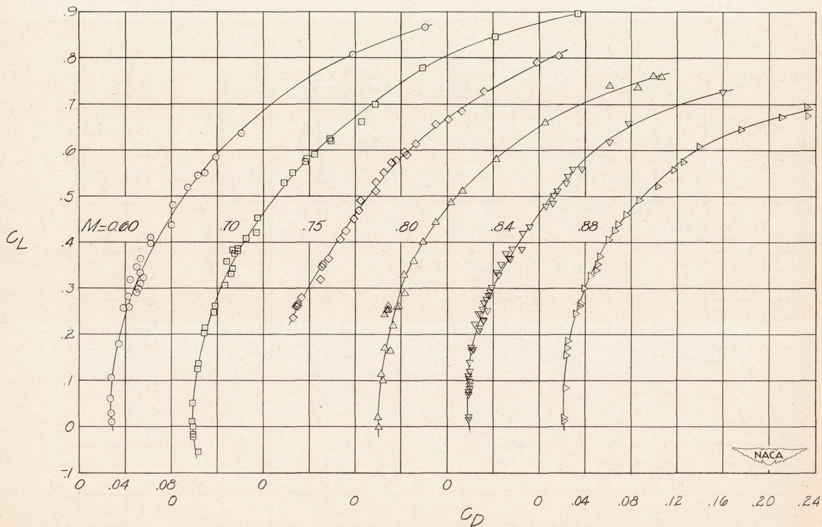
Figure 8.- Variation of drag coefficient with lift coefficient for various constant Mach numbers.
