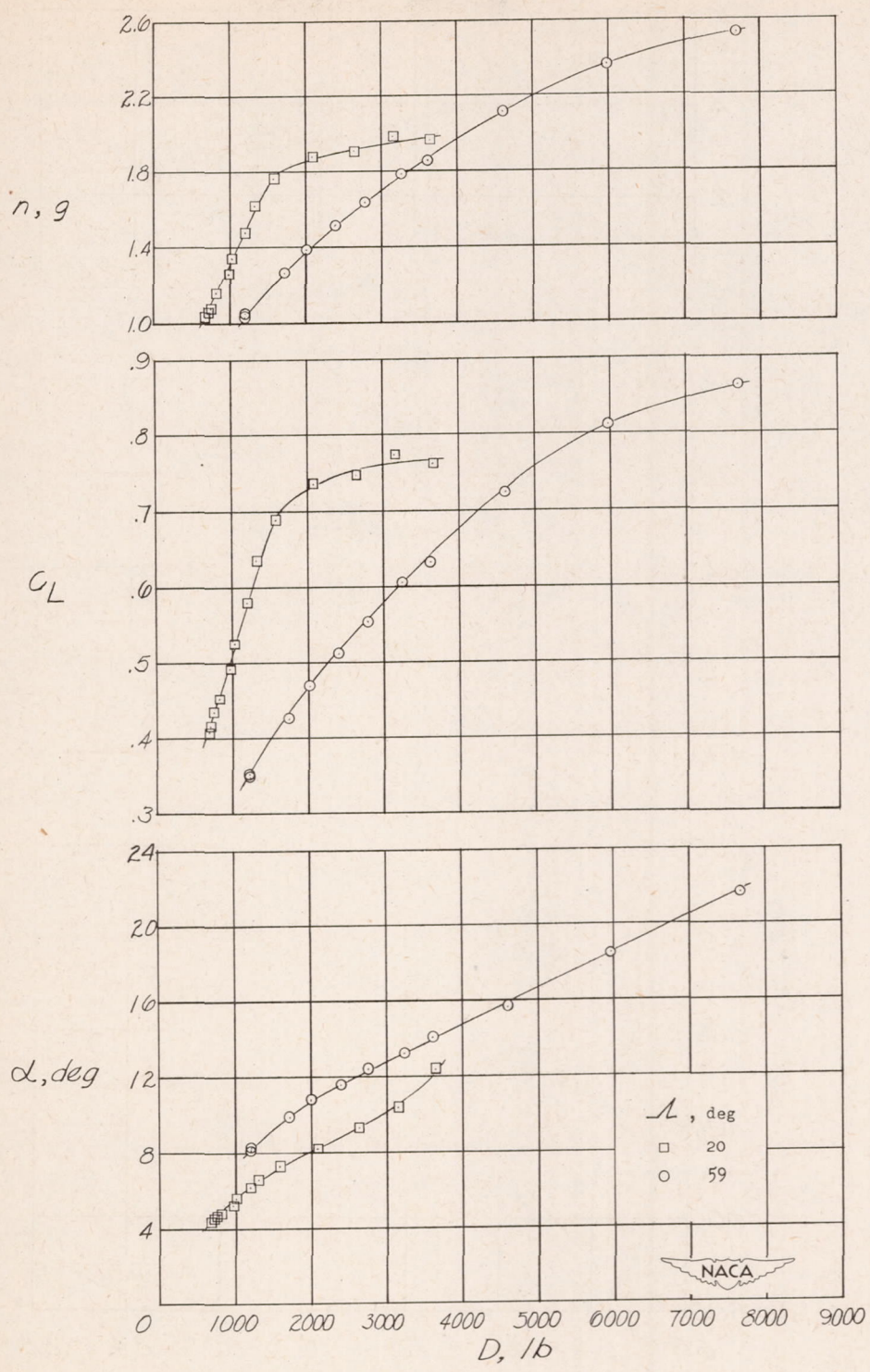
Figure 13.- Comparison of performance of 20° and 59° sweptback configurations in pull-ups at a Mach number of 0.74 and an altitude of 42,000 feet.
