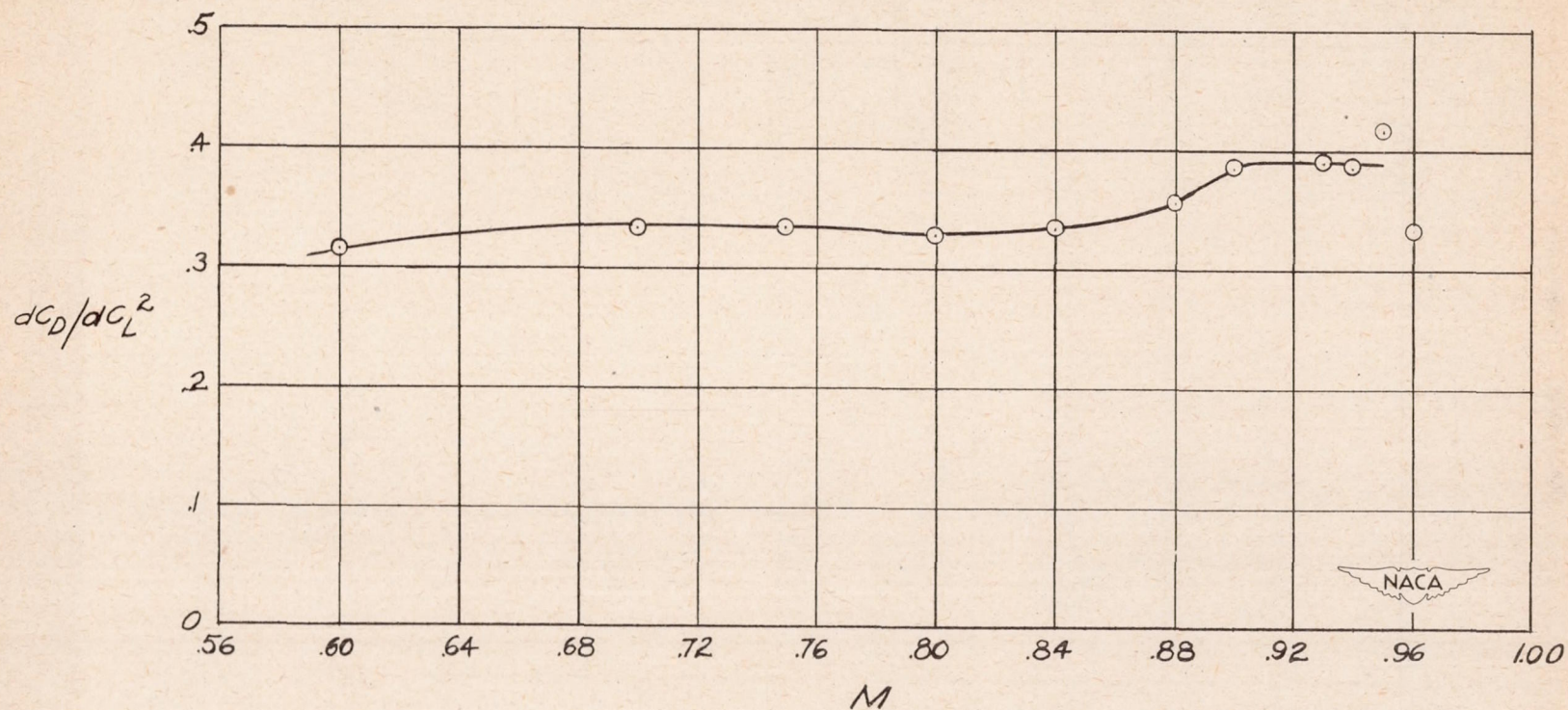
Figure 11.- Variation of induced drag factor with Mach number. C_L range 0.2 - 0.6.
