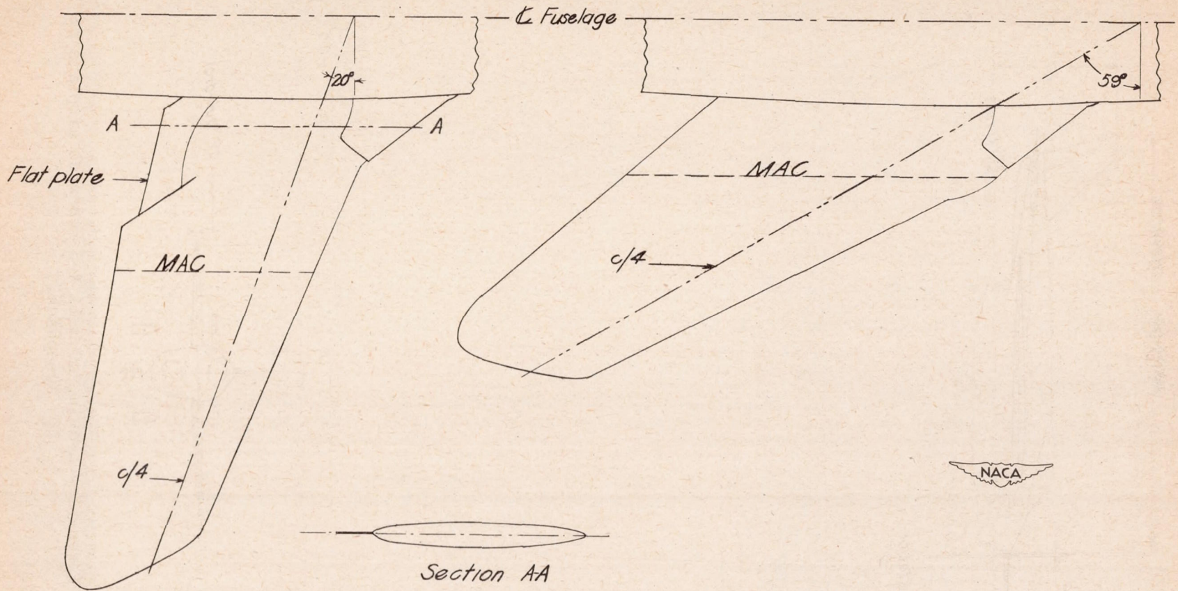
Figure 3.- Sketch showing differences in wing plan form between the 20° and 59° sweptback configurations.
