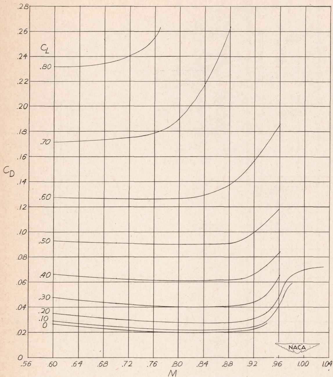
Figure 9.- Variation of drag coefficient with Mach number for various constant lift coefficients.
