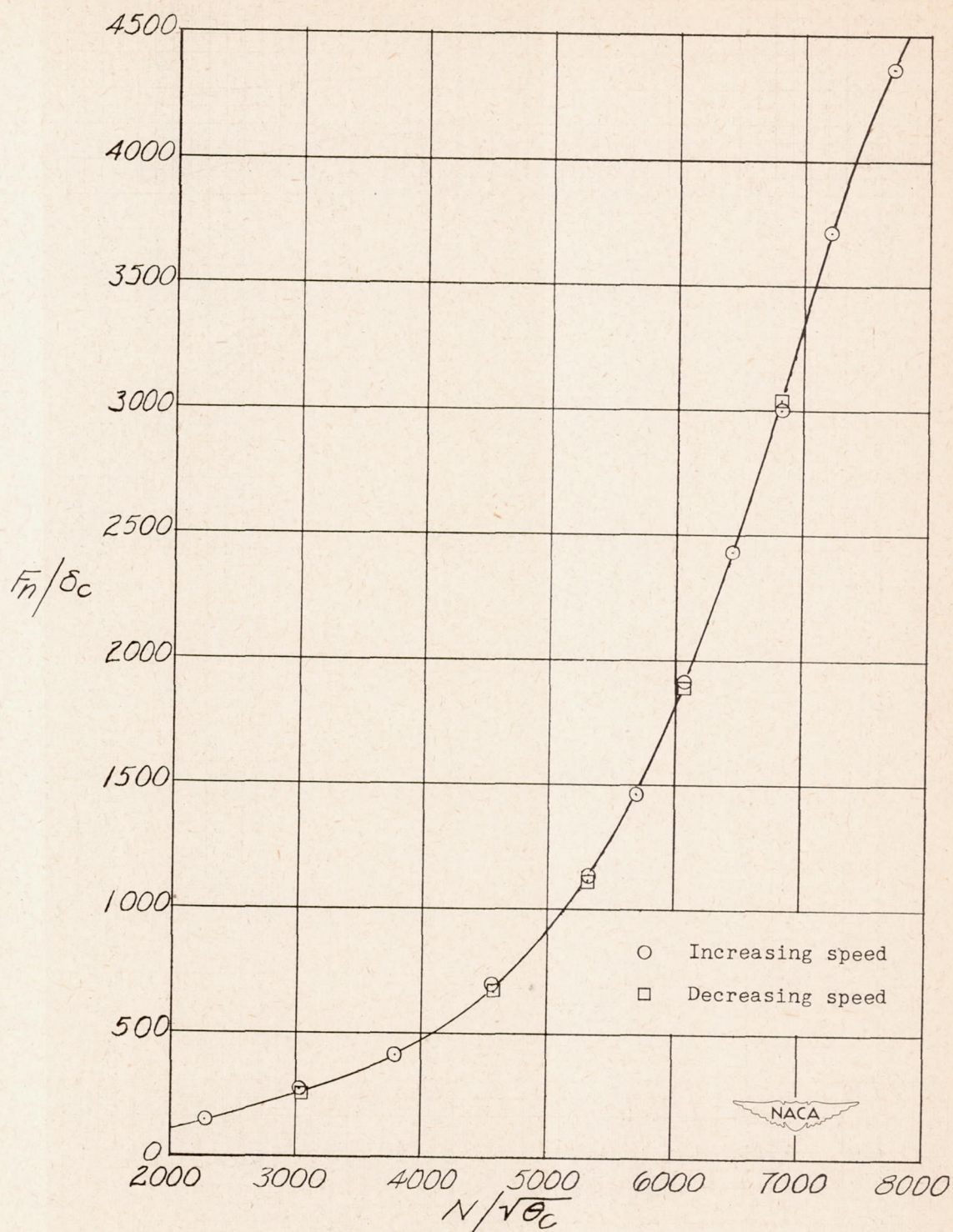
Figure 4.- Variation of normalized engine thrust with normalized engine speed.
